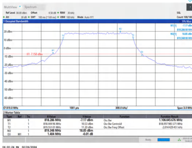
Band26-1.4MHz-16QAM-26740-6RB#0
