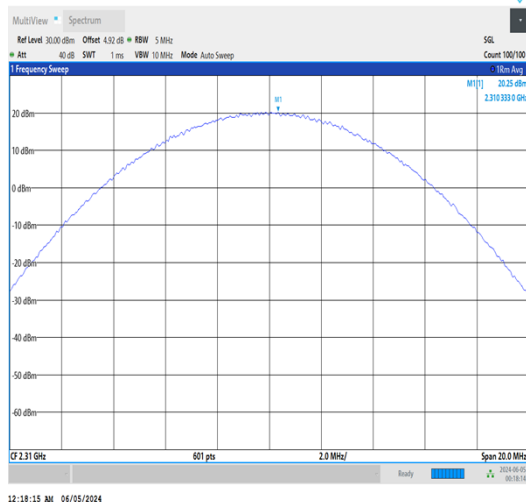
Band30-10MHz-QPSK-27710-1RB#24-PASS
