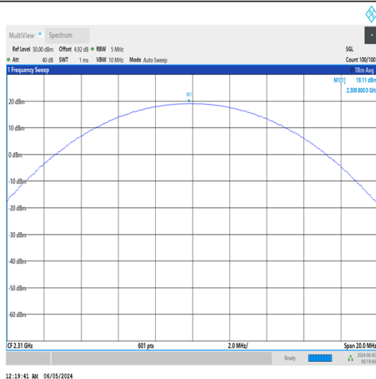
Band30-10MHz-QPSK-27710-25RB#12-PASS
