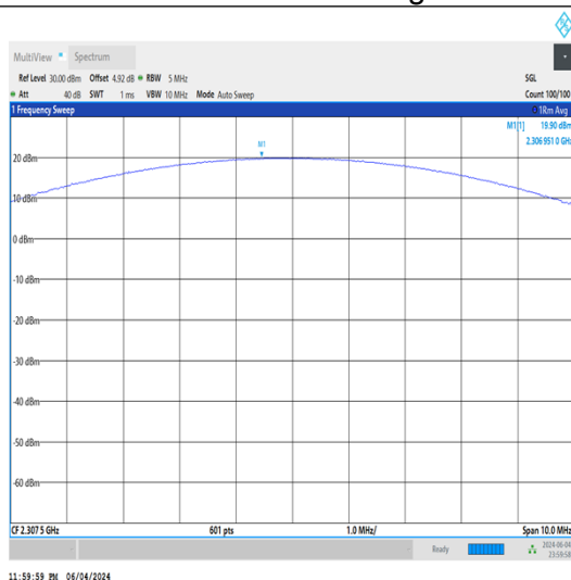
Band30-5MHz-QPSK-27685-12RB#6-PASS
