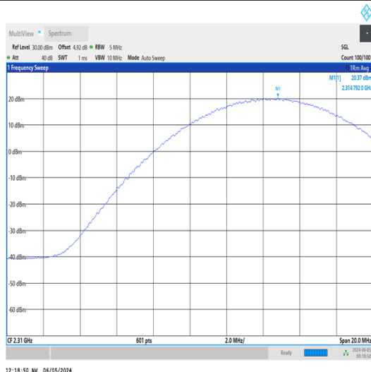
Band30-10MHz-QPSK-27710-1RB#49-PASS
