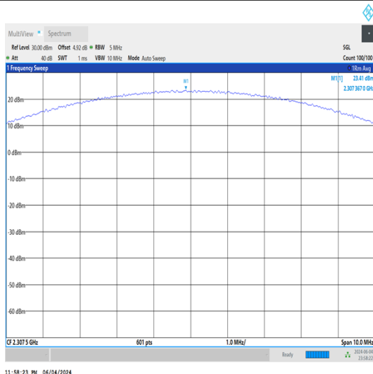
Band30-5MHz-QPSK-27685-1RB#12-PASS
