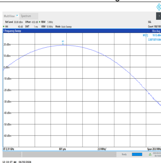
Band30-10MHz-QPSK-27710-25RB#0-PASS
