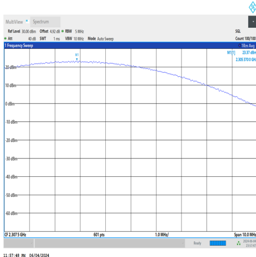
Band30-5MHz-QPSK-27685-1RB#0-PASS
