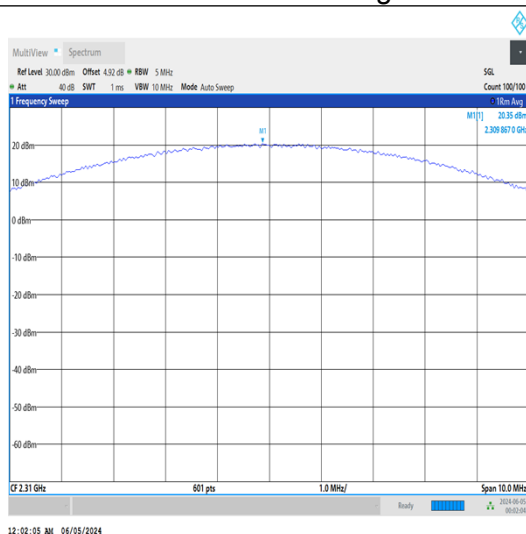
Band30-5MHz-QPSK-27710-1RB#12-PASS
