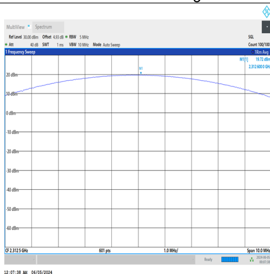
Band30-5MHz-QPSK-27735-12RB#6-PASS
