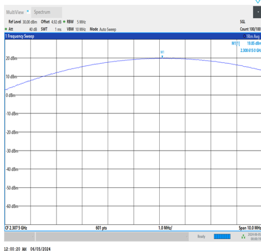
Band30-5MHz-QPSK-27685-12RB#13-PASS
