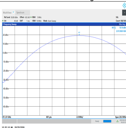
Band30-10MHz-QPSK-27710-25RB#25-PASS
