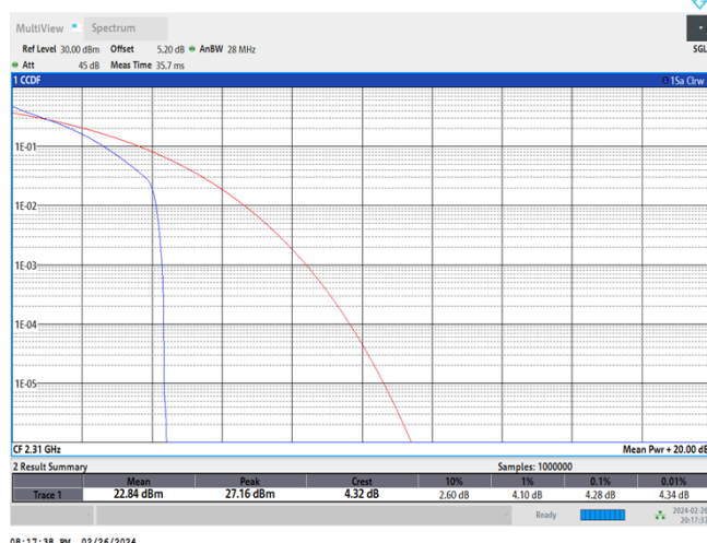
Band30-10MHz-QPSK-27710-50RB#0
