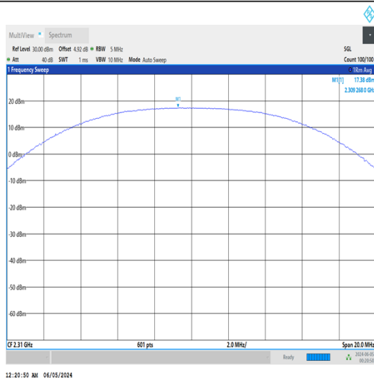
Band30-10MHz-QPSK-27710-50RB#0-PASS
