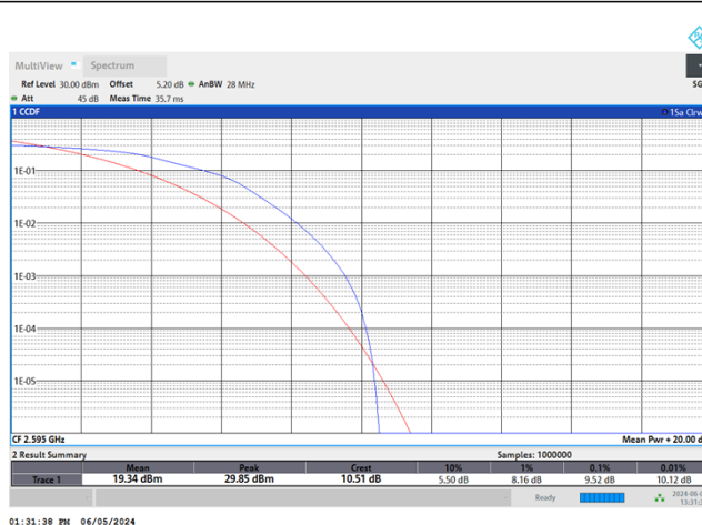
Band38-20MHz-QPSK-38000-100RB#0
