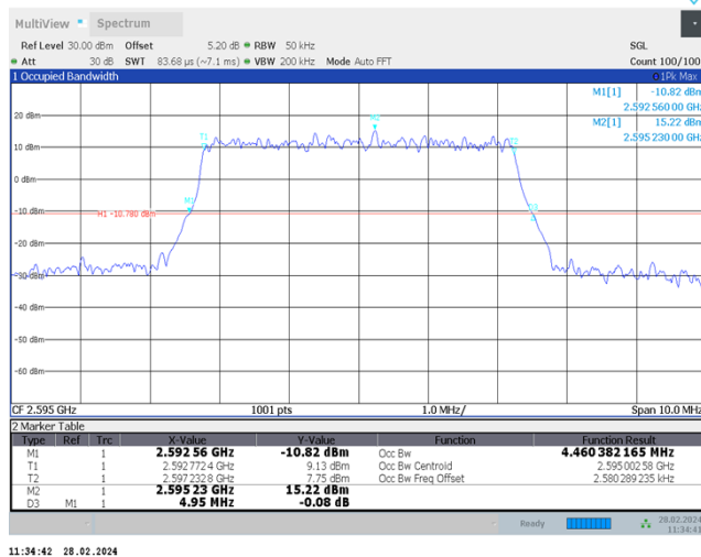
Band38-5MHz-16QAM-38000-25RB#0
