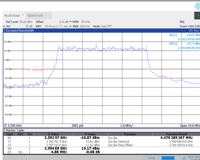
Band38-5MHz-QPSK-38000-25RB#0
