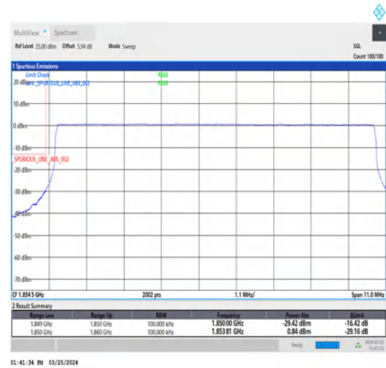
1-N2-15-10-L-6-CP-QPSK-Outer_Full-52@0-Ant1-1-seegraph-PASS-see graph
