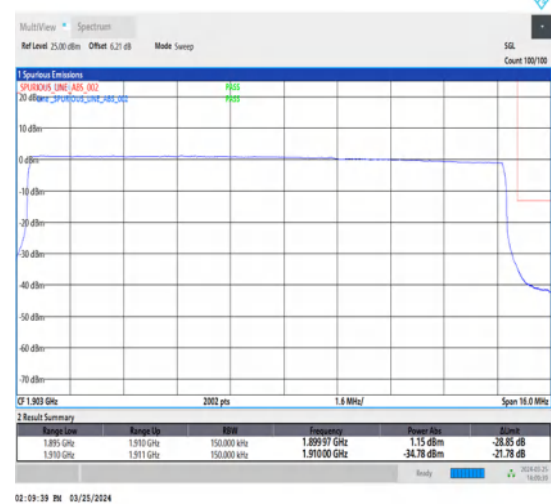
1-N2-15-15-H-6-CP-QPSK-Outer_Full-79@0-Ant1-1-seegraph-PASS-see graph
