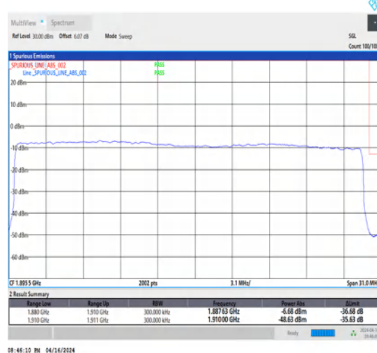
1-N2-15-30-H-6-CP-QPSK-Outer_Full-160@0-Ant1-1-seegraph-PASS-see graph
