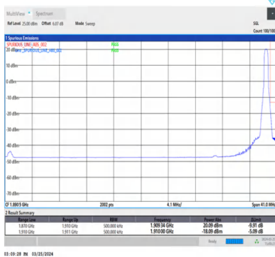
1-N2-15-40-H-5-CP-QPSK-Edge_1RB_Right-1@215-Ant1-1-seegraph-PASS-see graph
