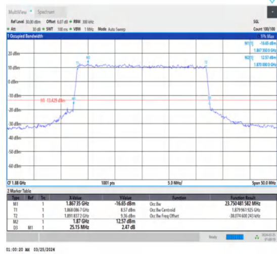
1-N2-15-25-M-6-CP-QPSK-Outet_Full-133@0-Ant1-23.75-25.150-≤25-PASS
