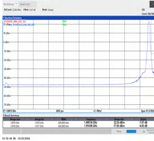
1-N2-15-40-H-2-DFT-PI2BPSK-Edge_1RB_Right-1@215-Ant1-1-seegraph-PASS-see graph
