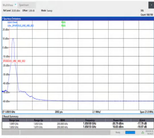
1-N2-15-20-L-1-DFT-PI2BPSK-Edge_1RB_Left-1@0-Ant1-1-seegraph-PASS-see graph
