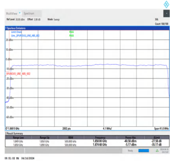
1-N2-15-40-L-3-DFT-PI2BPSK-Outer_Full-216@0-Ant1-1-seegraph-PASS-see graph
