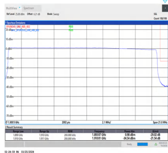
1-N2-15-20-H-6-CP-QPSK-Outer_Full-106@0-Ant1-1-seegraph-PASS-see graph
