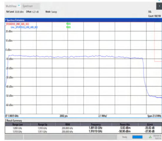
1-N2-15-20-H-3-DFT-PI2BPSK-Outer_Full-100@0-Ant1-1-seegraph-PASS-see graph
