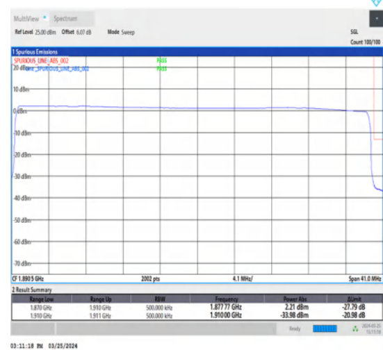
1-N2-15-40-H-6-CP-QPSK-Outer_Full-216@0-Ant1-1-seegraph-PASS-see graph
