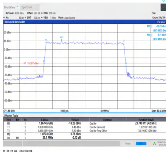
1-N2-15-25-M-9-CP-256QAM-Outer_Full-133@0- Ant1-23.746-25.100-≤25-PASS
