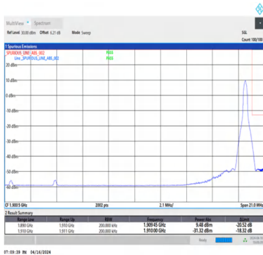
1-N2-15-20-H-5-CP-QPSK-Edge_1RB_Right-1@105-Ant1-1-seegraph-PASS-see graph
