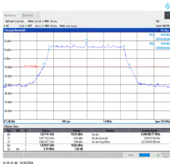
1-N2-15-5-M-3-DFT-16QAM-Outer_Full-25@0-Ant1- 4.508-5.140-≤5-PASS
