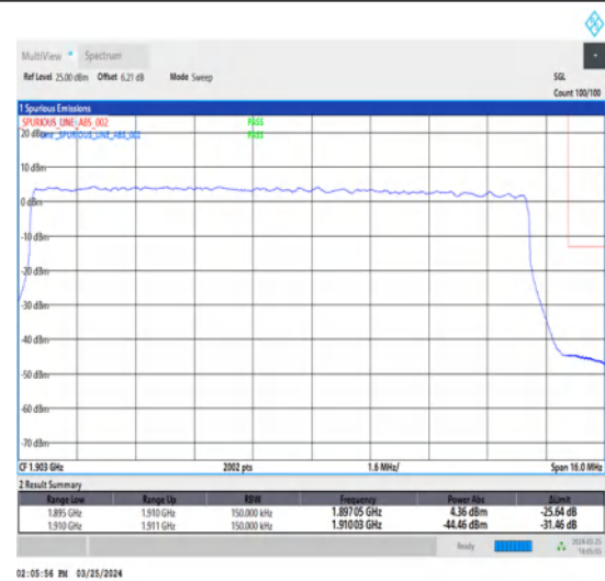
1-N2-15-15-H-3-DFT-PI2BPSK-Outer_Full-75@0-Ant1-1-seegraph-PASS-see graph
