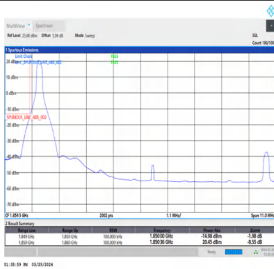
1-N2-15-10-L-1-DFT-PI2BPSK-Edge_1RB_Left-1@0-Ant1-1-seegraph-PASS-see graph
