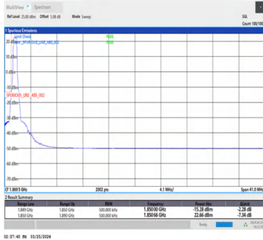
1-N2-15-40-L-1-DFT-PI2BPSK-Edge_1RB_Left-1@0-Ant1-1-seegraph-PASS-see graph
