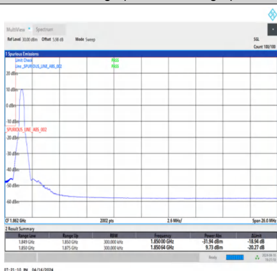
1-N2-15-25-L-4-CP-QPSK-Edge_1RB_Left-1@0-Ant1-1-seegraph-PASS-see graph
