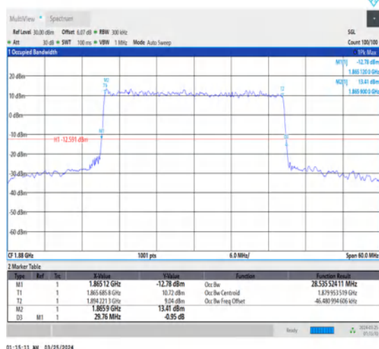
1-N2-15-30-M-3-DFT-16QAM-Outer_Full-160@0- Ant1-28.536-29.760-≤30-PASS
