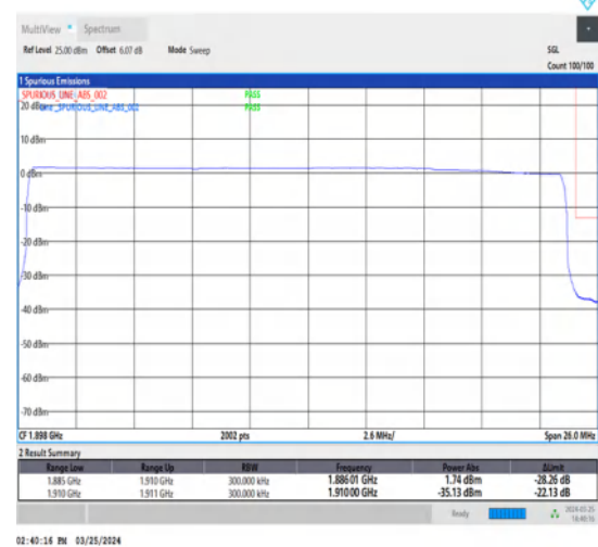
1-N2-15-25-H-6-CP-QPSK-Outer_Full-133@0-Ant1-1-seegraph-PASS-see graph
