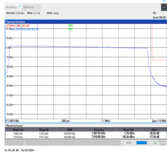
1-N2-15-10-H-6-CP-QPSK-Outer_Full-52@0-Ant1-1-seegraph-PASS-see graph
