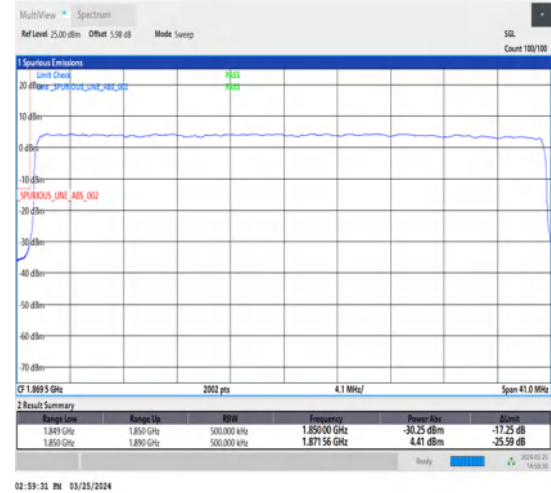
1-N2-15-40-L-3-DFT-PI2BPSK-Outer_Full-216@0-Ant1-1-seegraph-PASS-see graph
