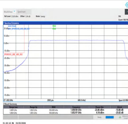
1-N2-15-5-L-6-CP-QPSK-Outer_Full-25@0-Ant1-1-seegraph-PASS-see graph
