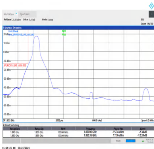
1-N2-15-5-L-4-CP-QPSK-Edge_1RB_Left-1@0-Ant1-1-seegraph-PASS-see graph
