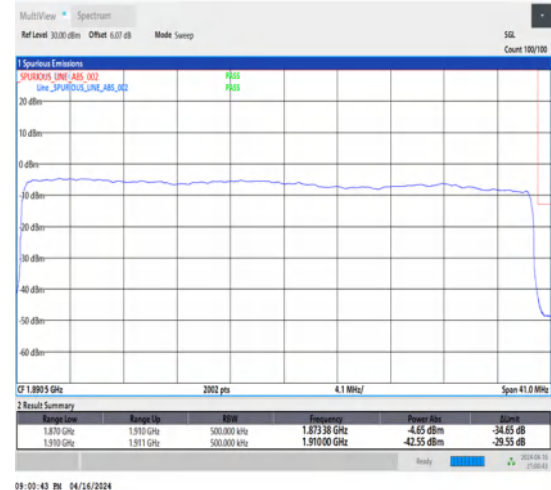
1-N2-15-40-H-3-DFT-PI2BPSK-Outer_Full-216@0-Ant1-1-seegraph-PASS-see graph
