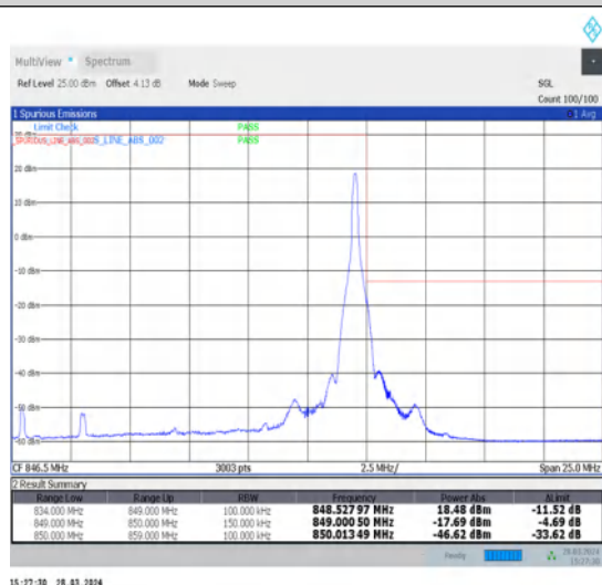
1-N5-15-15-H-5-CP-QPSK-Edge_1RB_Right-1@78-Ant1-1--PASS-see graph
