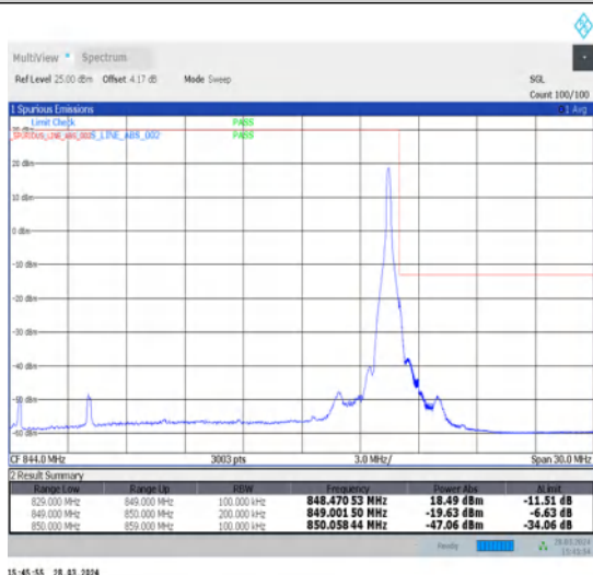
1-N5-15-20-H-5-CP-QPSK-Edge_1RB_Right-1@105-Ant1-1--PASS-see graph
