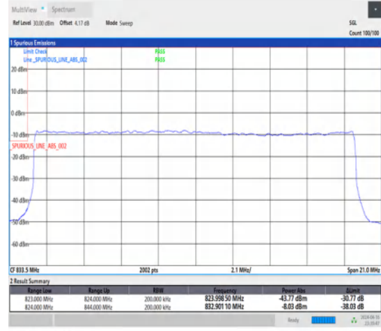
1-N5-15-20-L-3-DFT-PI2BPSK-Outer_Full-100@0-Ant1-1-seegraph-PASS-see graph
