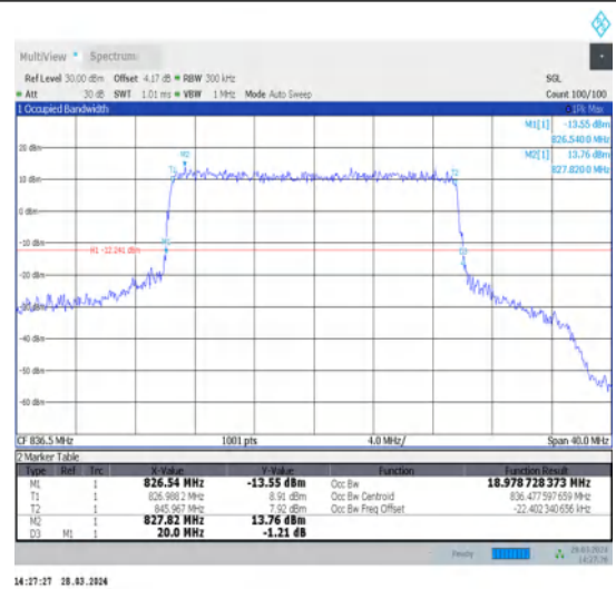
1-N5-15-20-M-7-CP-16QAM-Outer_Full-106@0-Ant1-18.979-20.000-≤20-PASS
