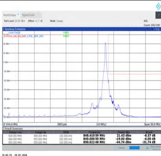
1-N5-15-20-H-2-DFT-PI2BPSK-Edge_1RB_Right-1@105-Ant1-1--PASS-see graph
