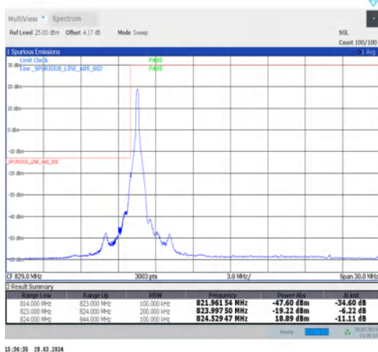
1-N5-15-20-L-4-CP-QPSK-Edge_1RB_Left-1@0-Ant1-1--PASS-see graph
