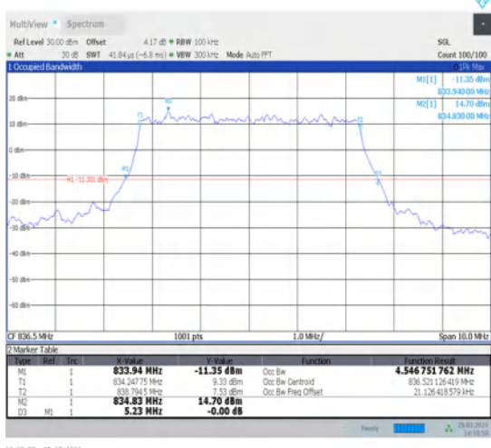
1-N5-15-5-M-7-CP-16QAM-Outer_Full-25@0-Ant1-4.547-5.230-≤5-PASS
