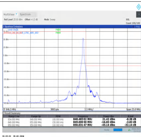
1-N5-15-15-H-2-DFT-PI2BPSK-Edge_1RB_Right-1@78-Ant1-1--PASS-see graph
