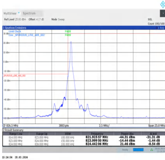
1-N5-15-15-L-1-DFT-PI2BPSK-Edge_1RB_Left-1@0-Ant1-1--PASS-see graph
