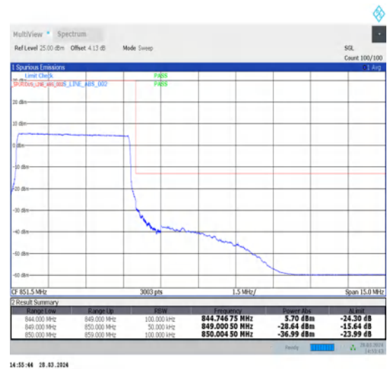
1-N5-15-5-H-6-CP-QPSK-Outer_Full-25@0-Ant1-1--PASS-see graph
