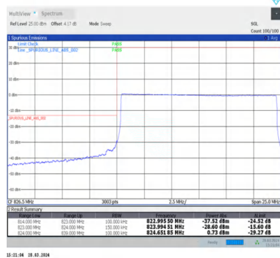
1-N5-15-15-L-6-CP-QPSK-Outer_Full-79@0-Ant1-1--PASS-see graph
