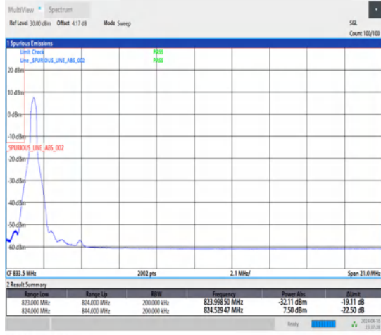
1-N5-15-20-L-1-DFT-PI2BPSK-Edge_1RB_Left-1@0-Ant1-1-seegraph-PASS-see graph
