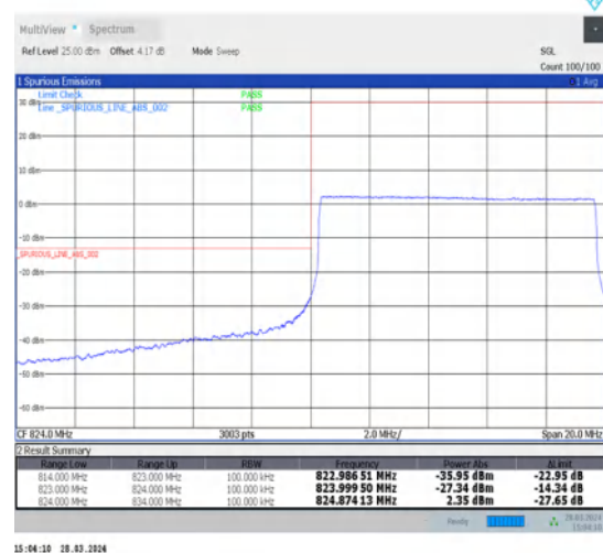
1-N5-15-10-L-6-CP-QPSK-Outer_Full-52@0-Ant1-1--PASS-see graph
