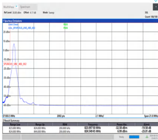
1-N5-15-20-L-4-CP-QPSK-Edge_1RB_Left-1@0-Ant1-1-seegraph-PASS-see graph
