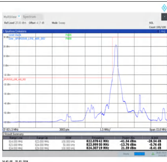
1-N5-15-5-L-1-DFT-PI2BPSK-Edge_1RB_Left-1@0-Ant1-1--PASS-see graph
