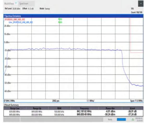
1-N5-15-10-H-3-DFT-PI2BPSK-Outer_Full-50@0-Ant1-1-seegraph-PASS-see graph
