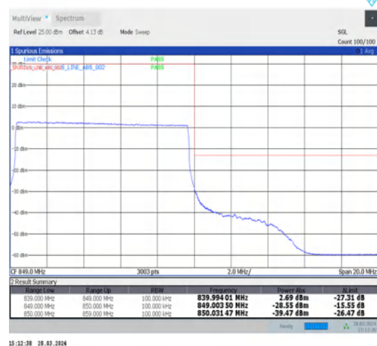
1-N5-15-10-H-6-CP-QPSK-Outer_Full-52@0-Ant1-1--PASS-see graph
