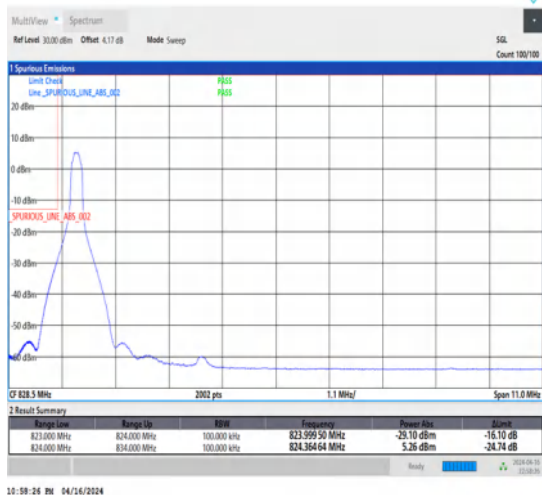
1-N5-15-10-L-1-DFT-PI2BPSK-Edge_1RB_Left-1@0-Ant1-1-seegraph-PASS-see graph
