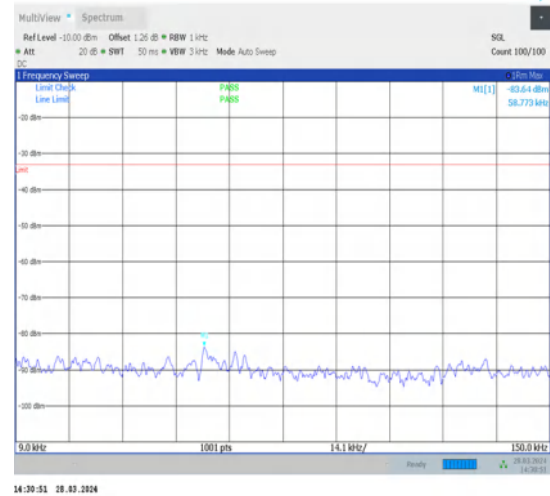
1-N5-15-20-M-1-DFT-PI2BPSK-Inner_1RB_Left- 1@1-0.009-0.15-Ant1-0.06--83.64--33-PASS
