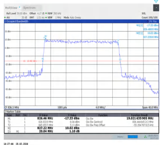
1-N5-15-20-M-9-CP-256QAM-Outer_Full-106@0-Ant1-19.022-20.040-≤20-PASS
