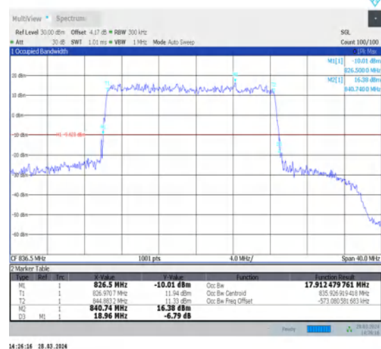
1-N5-15-20-M-1-DFT-QPSK-Outer_Full-100@0-Ant1-17.912-18.960-≤20-PASS
