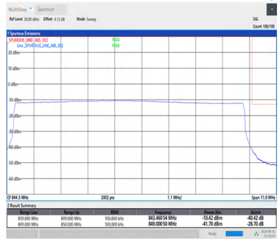
1-N5-15-10-H-6-CP-QPSK-Outer_Full-52@0-Ant1-1-seegraph-PASS-see graph
