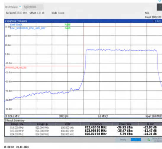
1-N5-15-10-L-3-DFT-PI2BPSK-Outer_Full-50@0-Ant1-1--PASS-see graph
