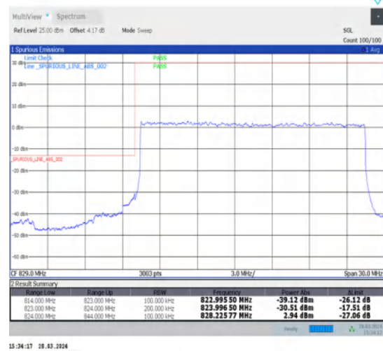
1-N5-15-20-L-3-DFT-PI2BPSK-Outer_Full-100@0-Ant1-1--PASS-see graph
