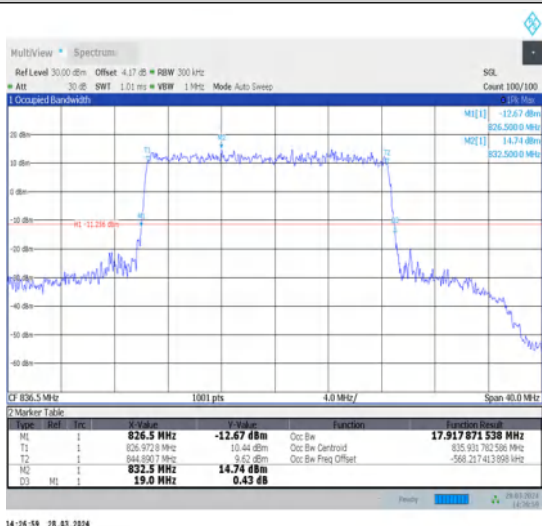
1-N5-15-20-M-4-DFT-64QAM-Outer_Full-100@0-Ant1-17.918-19.000-≤20-PASS
