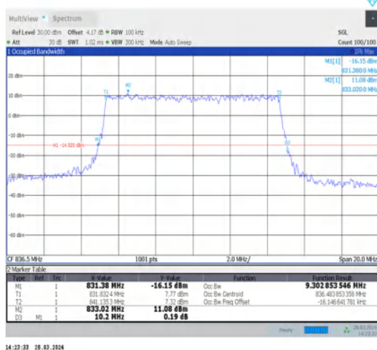
1-N5-15-10-M-6-CP-QPSK-Outer_Full-52@0-Ant1-9.303-10.200-≤10-PASS
