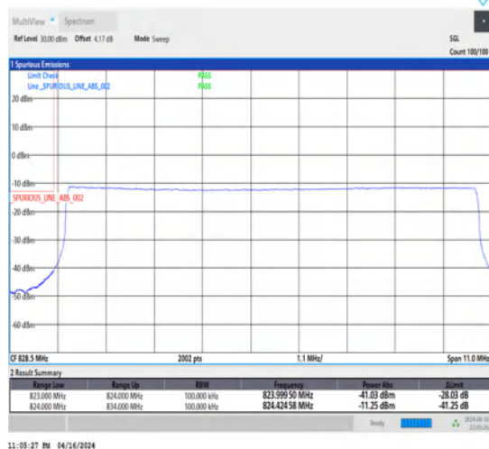
1-N5-15-10-L-6-CP-QPSK-Outer_Full-52@0-Ant1-1-seegraph-PASS-see graph
