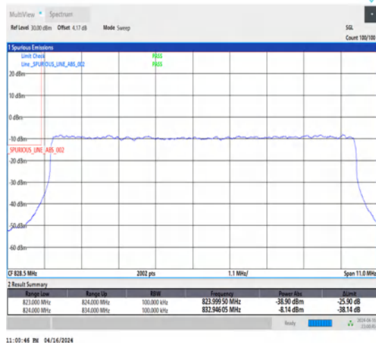
1-N5-15-10-L-3-DFT-PI2BPSK-Outer_Full-50@0-Ant1-1-seegraph-PASS-see graph
