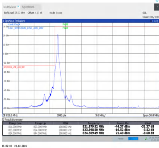
1-N5-15-20-L-1-DFT-PI2BPSK-Edge_1RB_Left-1@0-Ant1-1--PASS-see graph
