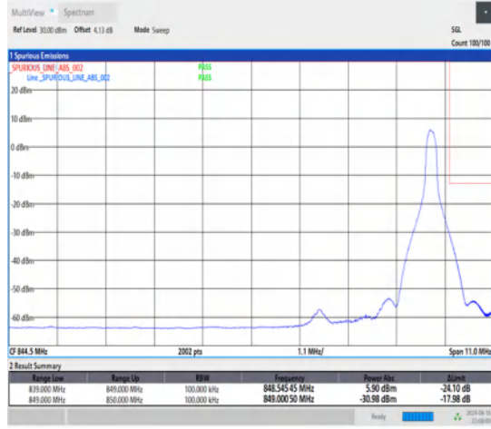
1-N5-15-10-H-2-DFT-PI2BPSK-Edge_1RB_Right-1@51-Ant1-1-seegraph-PASS-see graph
