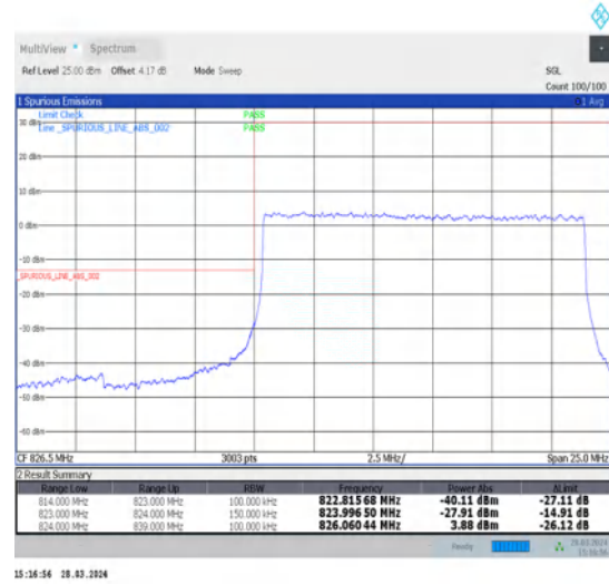
1-N5-15-15-L-3-DFT-PI2BPSK-Outer_Full-75@0-Ant1-1--PASS-see graph
