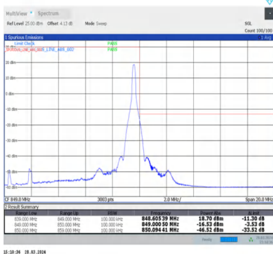
1-N5-15-10-H-5-CP-QPSK-Edge_1RB_Right-1@51-Ant1-1--PASS-see graph
