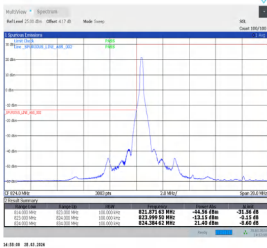
1-N5-15-10-L-1-DFT-PI2BPSK-Edge_1RB_Left-1@0-Ant1-1--PASS-see graph
