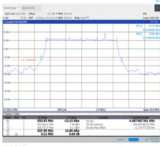
1-N5-15-5-M-8-CP-64QAM-Outer_Full-25@0-Ant1-4.487-5.120-≤5-PASS
