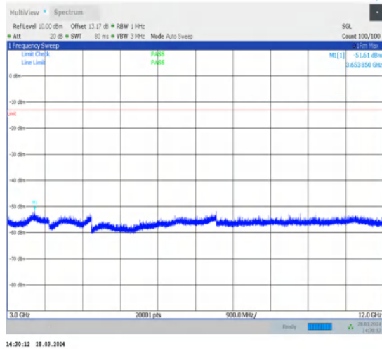
1-N5-15-20-L-1-DFT-PI2BPSK-Inner_1RB_Left- 1@1-3000-12000-Ant1-3653.85--51.61--13-PASS
