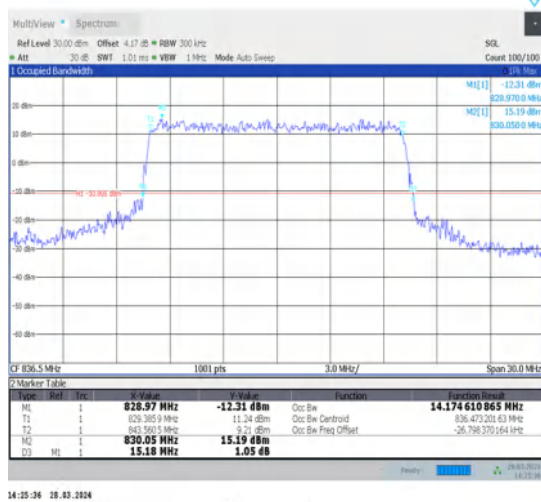
1-N5-15-15-M-7-CP-16QAM-Outer_Full-79@0-Ant1-14.175-15.180-≤15-PASS
