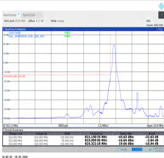
1-N5-15-5-L-4-CP-QPSK-Edge_1RB_Left-1@0-Ant1-1--PASS-see graph
