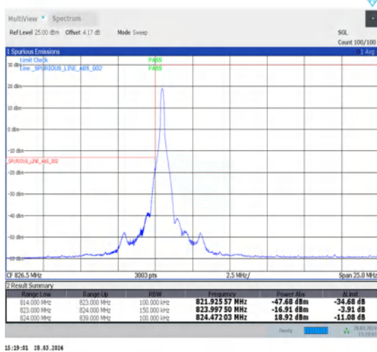
1-N5-15-15-L-4-CP-QPSK-Edge_1RB_Left-1@0-Ant1-1--PASS-see graph
