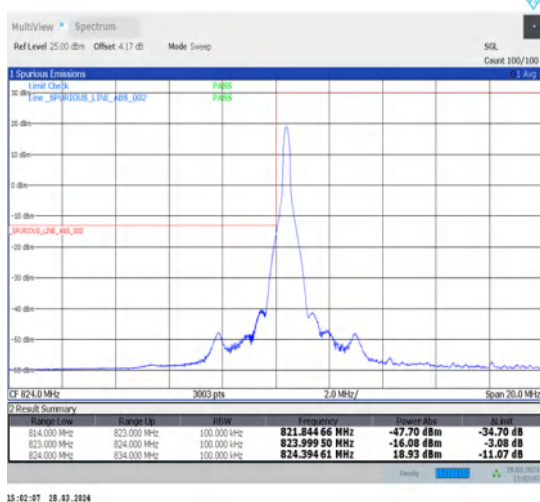
1-N5-15-10-L-4-CP-QPSK-Edge_1RB_Left-1@0-Ant1-1--PASS-see graph
