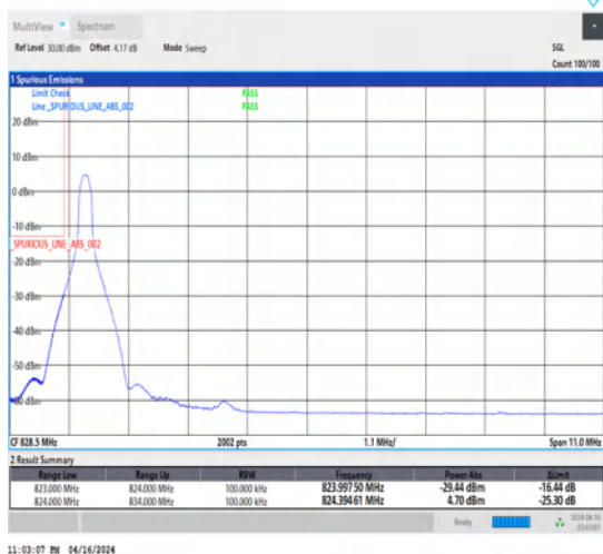
1-N5-15-10-L-4-CP-QPSK-Edge_1RB_Left-1@0-Ant1-1-seegraph-PASS-see graph
