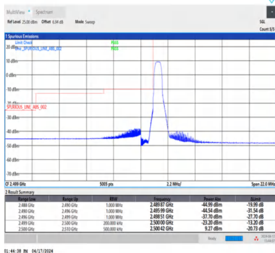
1-N7-15-10-L-4-CP-QPSK-Edge_1RB_Left-1@0-Ant1-1--PASS-see graph
