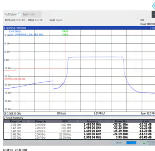
1-N7-15-5-L-6-CP-QPSK-Outer_Full-25@0-Ant1-1--PASS-see graph
