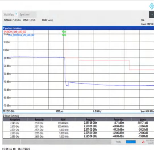
1-N7-15-25-H-6-CP-QPSK-Outer_Full-133@0-Ant1-1--PASS-see graph
