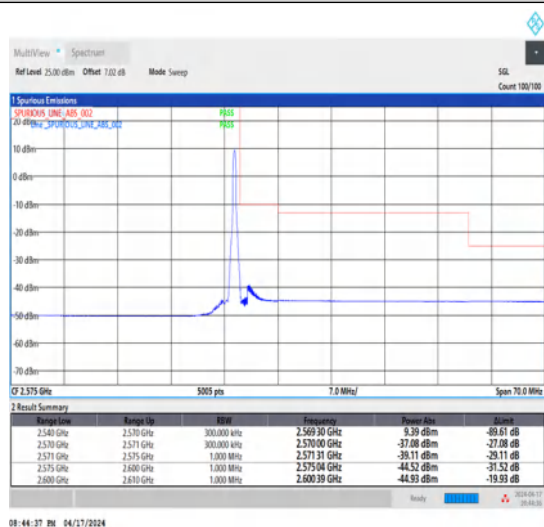
1-N7-15-30-H-5-CP-QPSK-Edge_1RB_Right-1@159-Ant1-1--PASS-see graph
