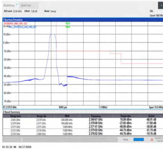
1-N7-15-5-H-2-DFT-PI2BPSK-Edge_1RB_Right-1@24-Ant1-1--PASS-see graph
