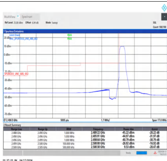
1-N7-15-5-L-1-DFT-PI2BPSK-Edge_1RB_Left-1@0-Ant1-1--PASS-see graph
