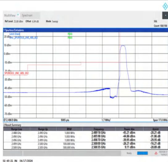
1-N7-15-5-L-4-CP-QPSK-Edge_1RB_Left-1@0-Ant1-1--PASS-see graph
