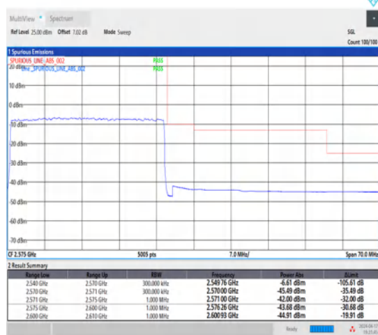
1-N7-15-30-H-3-DFT-PI2BPSK-Outer_Full-160@0-Ant1-1--PASS-see graph
