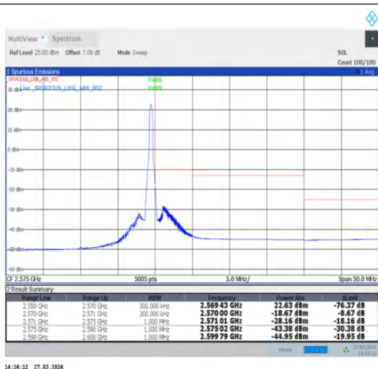
1-N7-15-20-H-2-DFT-PI2BPSK-Edge_1RB_Right-1@105-Ant1-1--PASS-see graph
