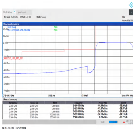
1-N7-15-5-L-6-CP-QPSK-Outer_Full-25@0-Ant1-1--PASS-see graph
