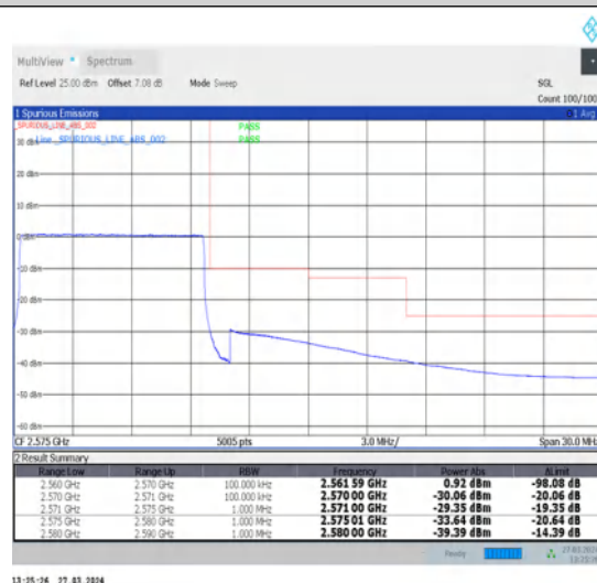
1-N7-15-10-H-6-CP-QPSK-Outer_Full-52@0-Ant1-1--PASS-see graph
