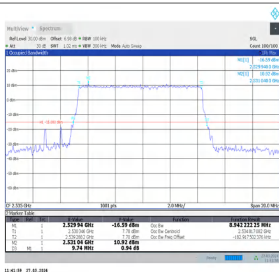
1-N7-15-10-M-4-DFT-64QAM-Outet_Full-50@0-Ant1-8.942-9.740-≤10-PASS
