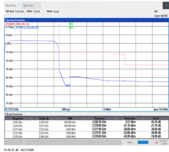
1-N7-15-5-H-3-DFT-PI2BPSK-Outer_Full-25@0-Ant1-1--PASS-see graph
