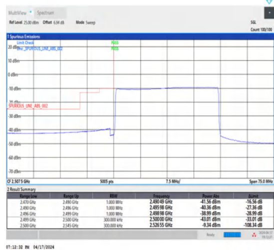
1-N7-15-30-L-6-CP-QPSK-Outer_Full-160@0-Ant1-1--PASS-see graph
