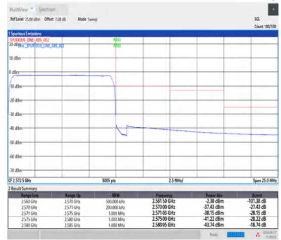
1-N7-15-10-H-6-CP-QPSK-Outer_Full-52@0-Ant1-1--PASS-see graph
