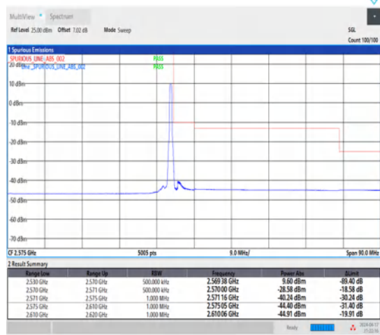
1-N7-15-40-H-5-CP-QPSK-Edge_1RB_Right-1@215-Ant1-1--PASS-see graph
