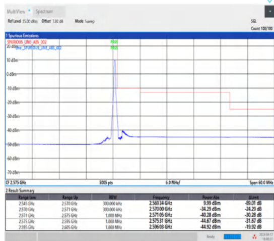
1-N7-15-25-H-2-DFT-PI2BPSK-Edge_1RB_Right-1@132-Ant1-1--PASS-see graph
