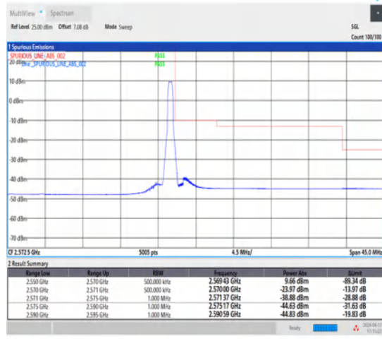
1-N7-15-20-H-5-CP-QPSK-Edge_1RB_Right-1@105-Ant1-1--PASS-see graph
