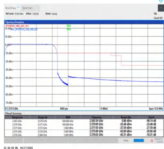
1-N7-15-5-H-6-CP-QPSK-Outer_Full-25@0-Ant1-1--PASS-see graph
