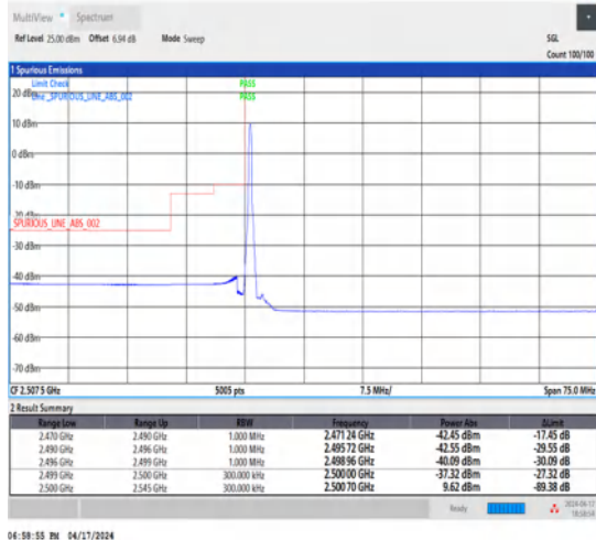
1-N7-15-30-L-1-DFT-PI2BPSK-Edge_1RB_Left-1@0-Ant1-1--PASS-see graph
