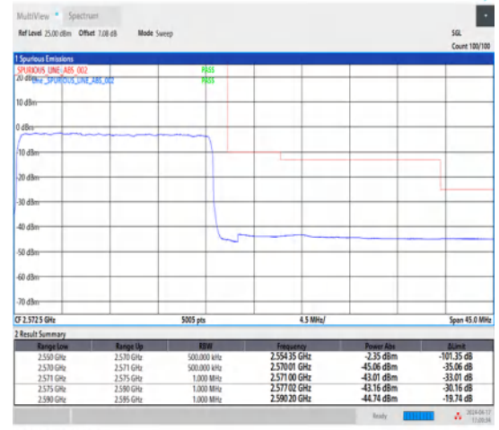
1-N7-15-20-H-3-DFT-PI2BPSK-Outer_Full-100@0-Ant1-1--PASS-see graph
