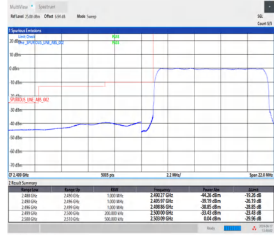
1-N7-15-10-L-3-DFT-PI2BPSK-Outer_Full-50@0-Ant1-1--PASS-see graph
