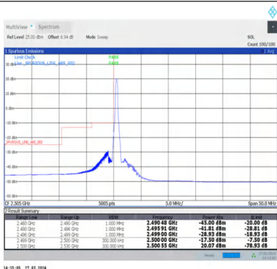
1-N7-15-20-L-4-CP-QPSK-Edge_1RB_Left-1@0-Ant1-1--PASS-see graph
