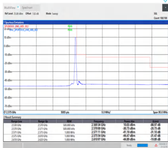
1-N7-15-40-H-2-DFT-PI2BPSK-Edge_1RB_Right-1@215-Ant1-1--PASS-see graph
