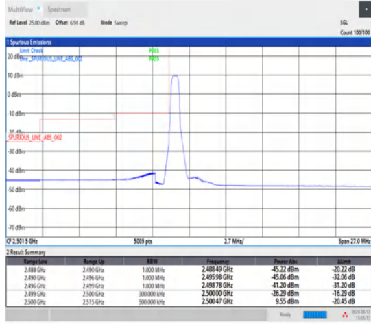
1-N7-15-15-L-1-DFT-PI2BPSK-Edge_1RB_Left-1@0-Ant1-1--PASS-see graph
