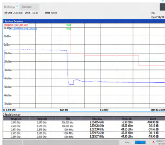
1-N7-15-25-H-3-DFT-PI2BPSK-Outer_Full-128@0-Ant1-1--PASS-see graph
