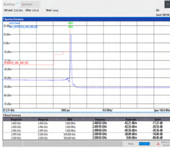
1-N7-15-40-L-1-DFT-PI2BPSK-Edge_1RB_Left-1@0-Ant1-1--PASS-see graph
