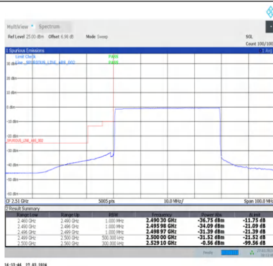
1-N7-15-40-L-6-CP-QPSK-Outer_Full-216@0-Ant1-1--PASS-see graph
