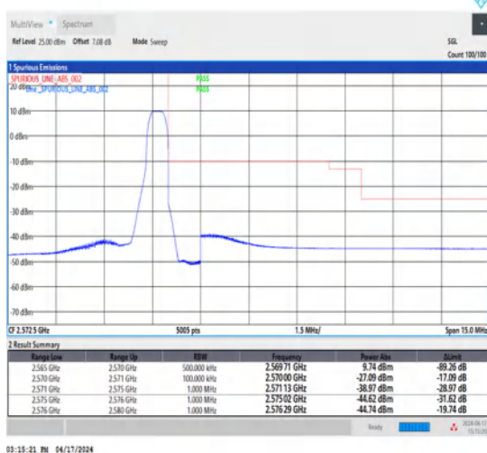
1-N7-15-5-H-5-CP-QPSK-Edge_1RB_Right-1@24-Ant1-1--PASS-see graph
