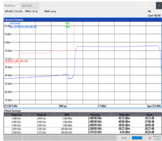
1-N7-15-15-L-6-CP-QPSK-Outer_Full-79@0-Ant1-1--PASS-see graph
