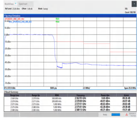
1-N7-15-10-H-3-DFT-PI2BPSK-Outer_Full-50@0-Ant1-1--PASS-see graph
