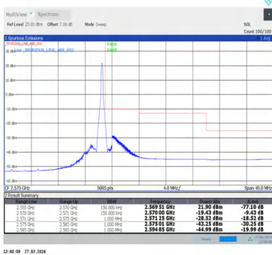
1-N7-15-15-H-2-DFT-PI2BPSK-Edge_1RB_Right-1@78-Ant1-1--PASS-see graph
