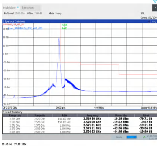
1-N7-15-15-H-5-CP-QPSK-Edge_1RB_Right-1@78-Ant1-1--PASS-see graph
