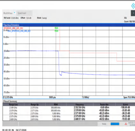
1-N7-15-30-H-6-CP-QPSK-Outer_Full-160@0-Ant1-1--PASS-see graph
