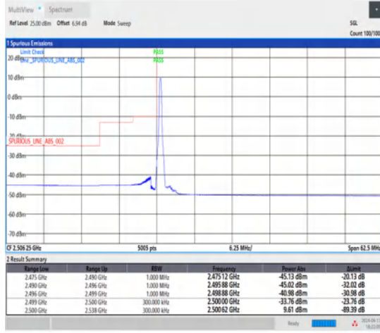
1-N7-15-25-L-1-DFT-PI2BPSK-Edge_1RB_Left-1@0-Ant1-1--PASS-see graph
