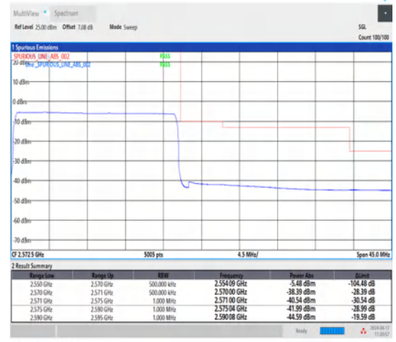
1-N7-15-20-H-6-CP-QPSK-Outer_Full-106@0-Ant1-1--PASS-see graph
