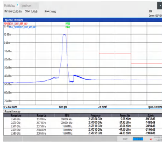
1-N7-15-10-H-5-CP-QPSK-Edge_1RB_Right-1@51-Ant1-1--PASS-see graph
