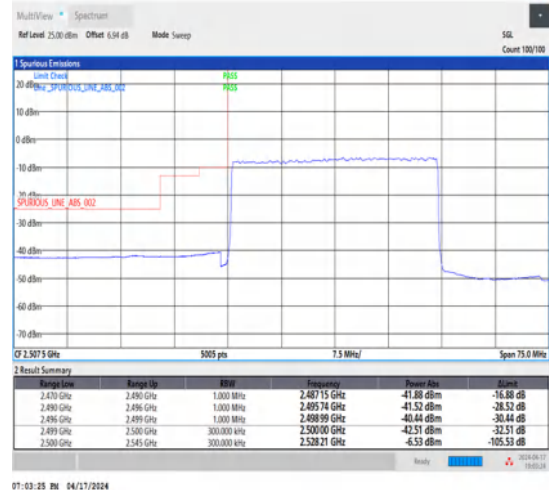
1-N7-15-30-L-3-DFT-PI2BPSK-Outer_Full-160@0-Ant1-1--PASS-see graph
