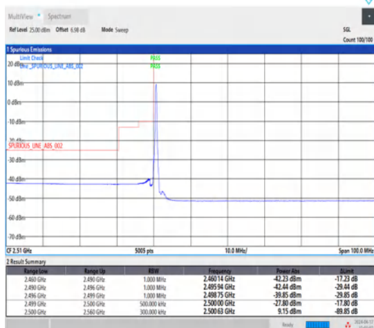
1-N7-15-40-L-4-CP-QPSK-Edge_1RB_Left-1@0-Ant1-1--PASS-see graph
