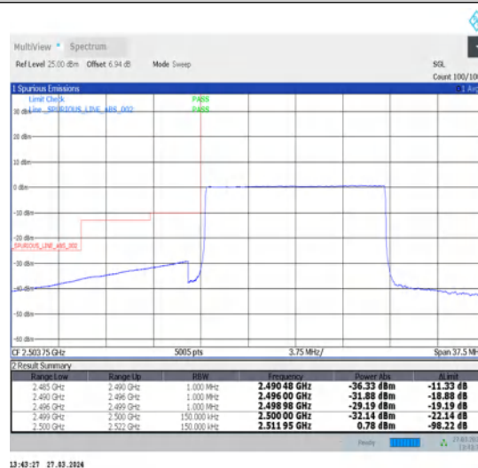
1-N7-15-15-L-6-CP-QPSK-Outer_Full-79@0-Ant1-1--PASS-see graph
