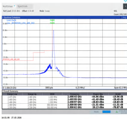
1-N7-15-25-L-4-CP-QPSK-Edge_1RB_Left-1@0-Ant1-1--PASS-see graph
