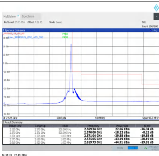
1-N7-15-40-H-2-DFT-PI2BPSK-Edge_1RB_Right-1@215-Ant1-1--PASS-see graph
