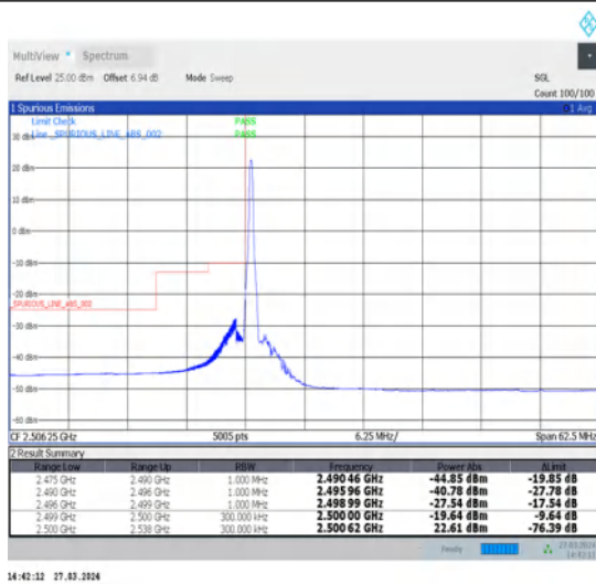
1-N7-15-25-L-1-DFT-PI2BPSK-Edge_1RB_Left-1@0-Ant1-1--PASS-see graph
