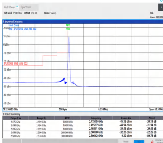
1-N7-15-25-L-4-CP-QPSK-Edge_1RB_Left-1@0-Ant1-1--PASS-see graph
