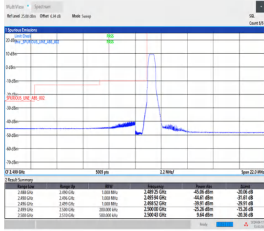
1-N7-15-10-L-1-DFT-PI2BPSK-Edge_1RB_Left-1@0-Ant1-1--PASS-see graph
