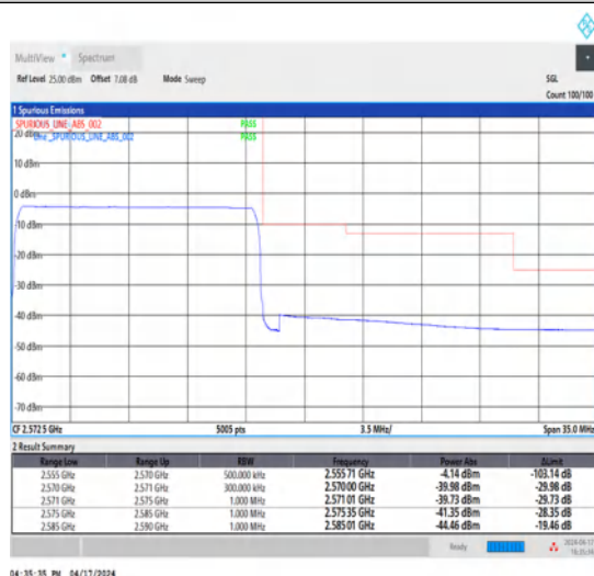
1-N7-15-15-H-6-CP-QPSK-Outer_Full-79@0-Ant1-1--PASS-see graph
