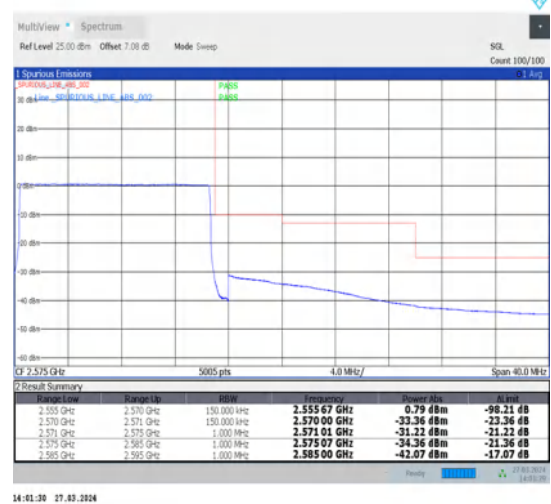
1-N7-15-15-H-6-CP-QPSK-Outer_Full-79@0-Ant1-1--PASS-see graph
