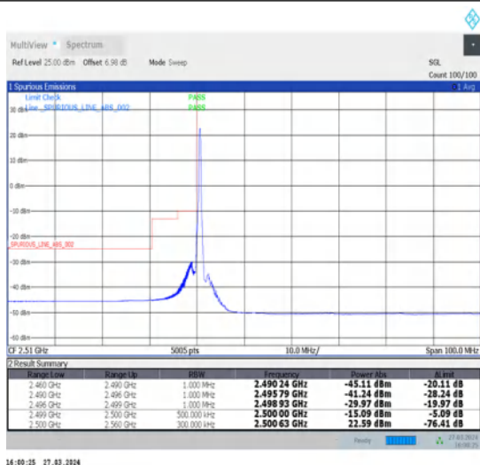
1-N7-15-40-L-1-DFT-PI2BPSK-Edge_1RB_Left-1@0-Ant1-1--PASS-see graph
