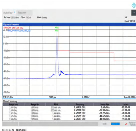
1-N7-15-25-H-5-CP-QPSK-Edge_1RB_Right-1@132-Ant1-1--PASS-see graph
