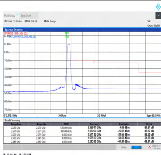
1-N7-15-15-H-5-CP-QPSK-Edge_1RB_Right-1@78-Ant1-1--PASS-see graph
