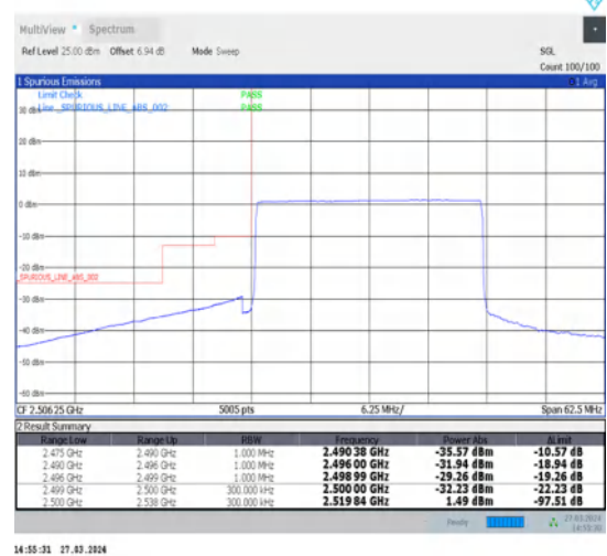
1-N7-15-25-L-6-CP-QPSK-Outer_Full-133@0-Ant1-1--PASS-see graph
