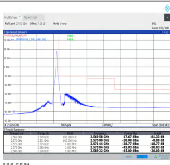
1-N7-15-10-H-5-CP-QPSK-Edge_1RB_Right-1@51-Ant1-1--PASS-see graph
