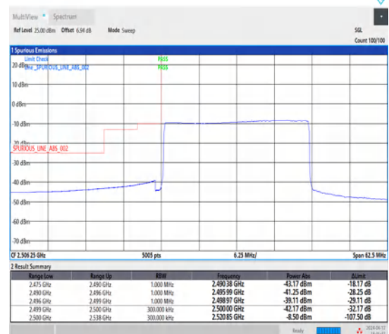
1-N7-15-25-L-6-CP-QPSK-Outer_Full-133@0-Ant1-1--PASS-see graph
