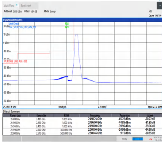
1-N7-15-15-L-4-CP-QPSK-Edge_1RB_Left-1@0-Ant1-1--PASS-see graph
