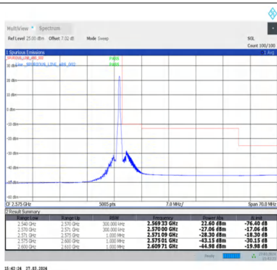
1-N7-15-30-H-2-DFT-PI2BPSK-Edge_1RB_Right-1@159-Ant1-1--PASS-see graph
