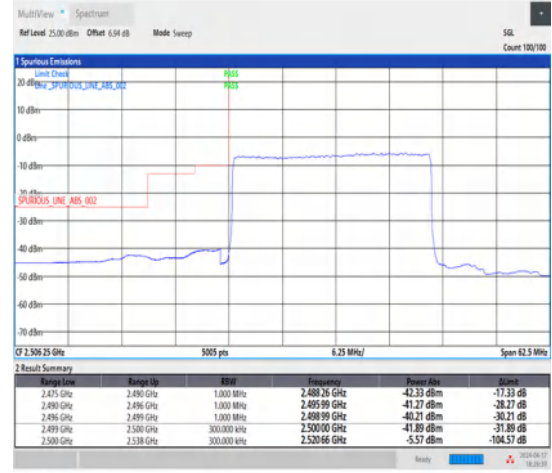
1-N7-15-25-L-3-DFT-PI2BPSK-Outer_Full-128@0-Ant1-1--PASS-see graph
