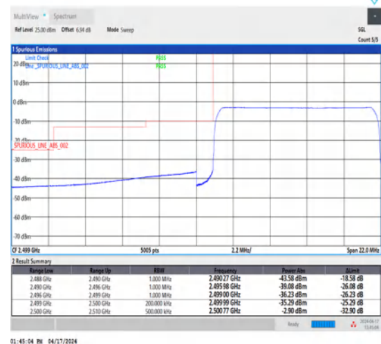
1-N7-15-10-L-6-CP-QPSK-Outer_Full-52@0-Ant1-1--PASS-see graph
