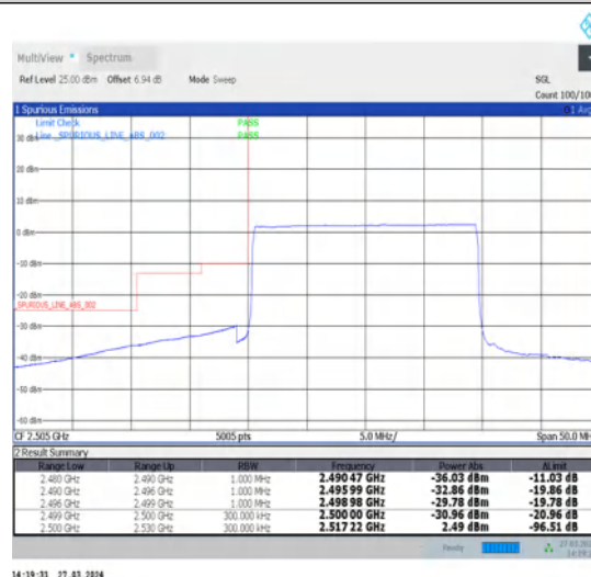
1-N7-15-20-L-6-CP-QPSK-Outer_Full-106@0-Ant1-1--PASS-see graph
