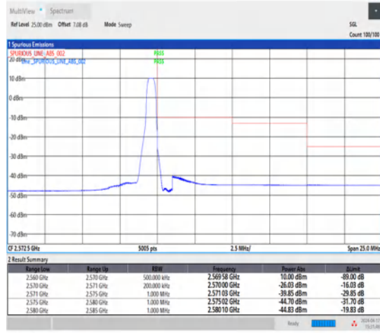
1-N7-15-10-H-2-DFT-PI2BPSK-Edge_1RB_Right-1@51-Ant1-1--PASS-see graph
