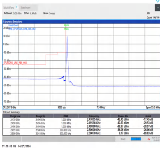
1-N7-15-30-L-4-CP-QPSK-Edge_1RB_Left-1@0-Ant1-1--PASS-see graph
