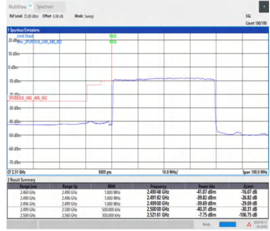
1-N7-15-40-L-3-DFT-PI2BPSK-Outer_Full-216@0-Ant1-1--PASS-see graph
