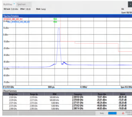
1-N7-15-20-H-2-DFT-PI2BPSK-Edge_1RB_Right-1@105-Ant1-1--PASS-see graph
