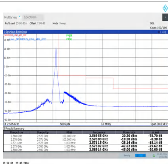
1-N7-15-10-H-2-DFT-PI2BPSK-Edge_1RB_Right-1@51-Ant1-1--PASS-see graph
