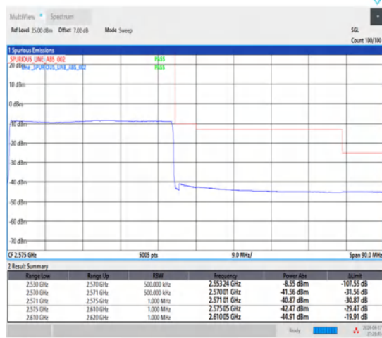
1-N7-15-40-H-6-CP-QPSK-Outer_Full-216@0-Ant1-1--PASS-see graph
