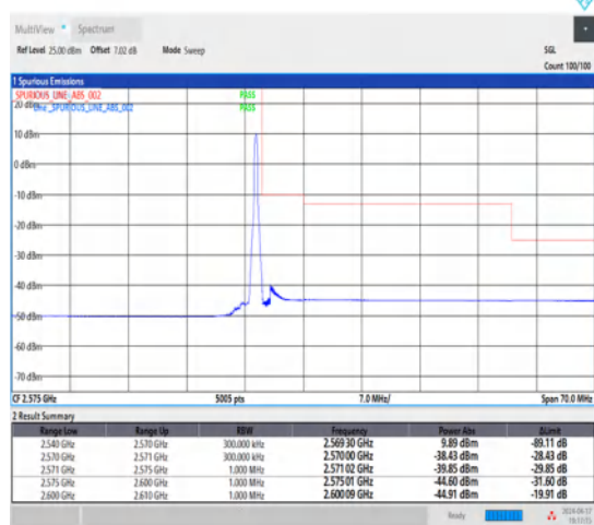
1-N7-15-30-H-2-DFT-PI2BPSK-Edge_1RB_Right-1@159-Ant1-1--PASS-see graph
