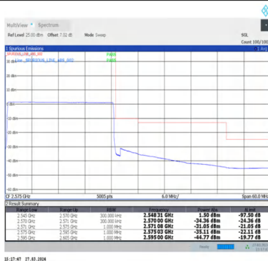
1-N7-15-25-H-6-CP-QPSK-Outer_Full-133@0-Ant1-1--PASS-see graph
