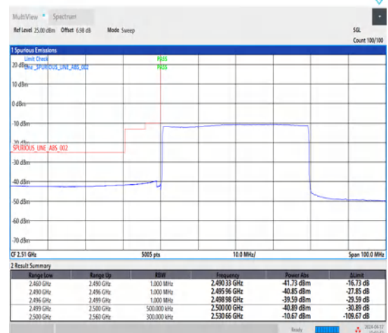
1-N7-15-40-L-6-CP-QPSK-Outer_Full-216@0-Ant1-1--PASS-see graph
