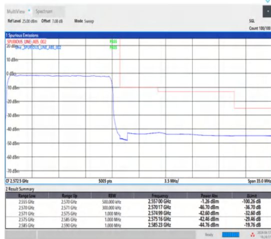
1-N7-15-15-H-3-DFT-PI2BPSK-Outer_Full-75@0-Ant1-1--PASS-see graph
