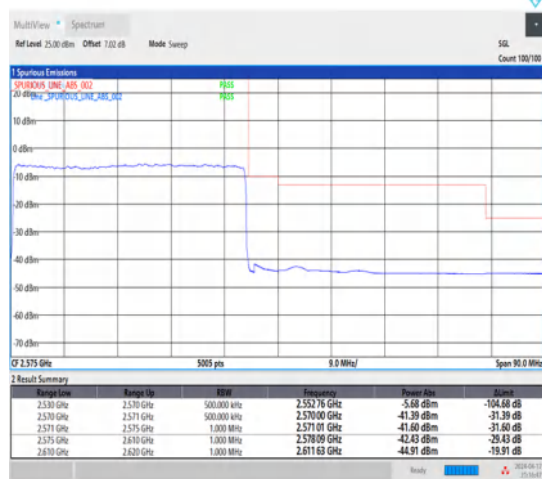
1-N7-15-40-H-3-DFT-PI2BPSK-Outer_Full-216@0-Ant1-1--PASS-see graph
