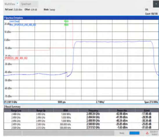
1-N7-15-15-L-3-DFT-PI2BPSK-Outer_Full-75@0-Ant1-1--PASS-see graph
