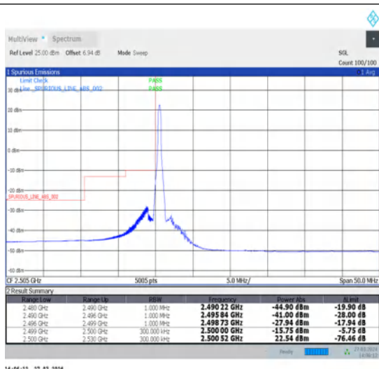
1-N7-15-20-L-1-DFT-PI2BPSK-Edge_1RB_Left-1@0-Ant1-1--PASS-see graph
