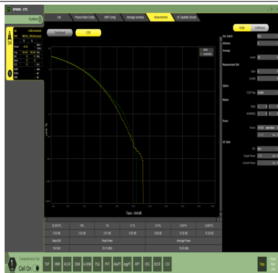
1-N12-15-15-L-15-CP-256QAM-Outer_Full-79@0- 18.78-18.78-19~27.5-PASS
