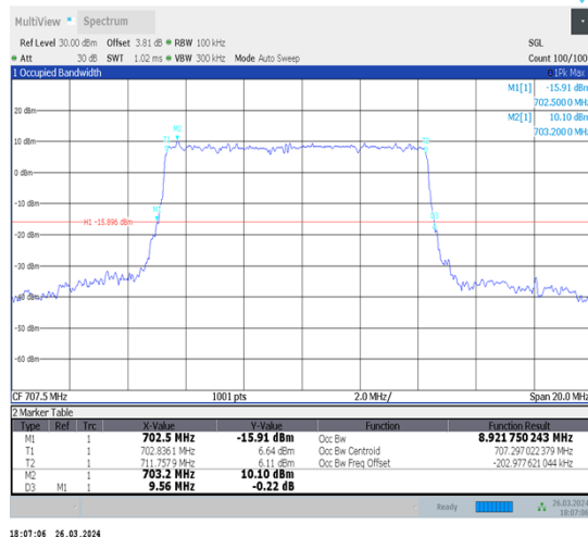
1-N12-15-10-M-5-DFT-256QAM-Outer_Full-50@0-Ant1-8.922-9.560-≤10-PASS
