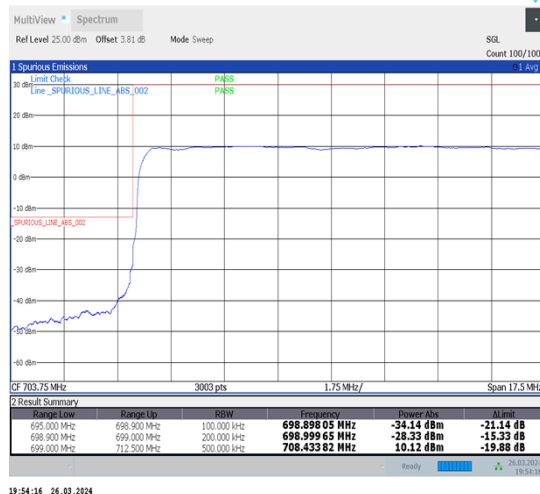
1-N12-15-15-L-3-DFT-PI2BPSK-Outer_Full-75@0-Ant1-1--PASS-see graph
