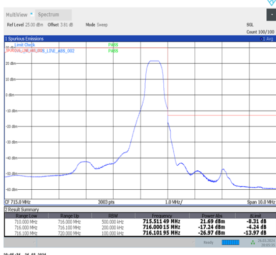
1-N12-15-15-H-2-DFT-PI2BPSK-Edge_1RB_Right-1@78-Ant1-1--PASS-see graph
