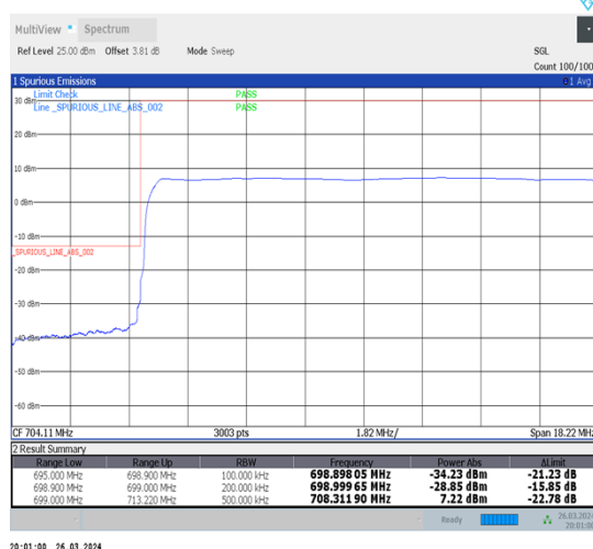
1-N12-15-15-L-6-CP-QPSK-Outer_Full-79@0-Ant1-1--PASS-see graph
