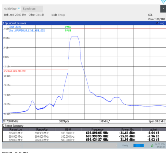
1-N12-15-10-L-1-DFT-PI2BPSK-Edge_1RB_Left-1@0-Ant1-1--PASS-see graph
