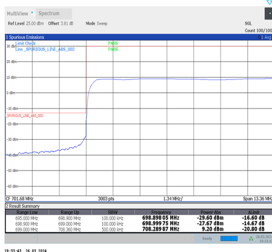
1-N12-15-10-L-6-CP-QPSK-Outer_Full-52@0-Ant1-1--PASS-see graph
