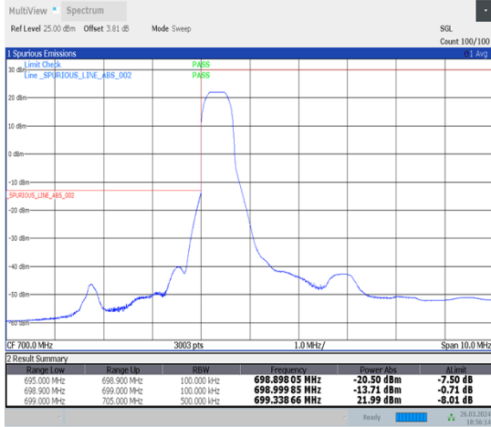
1-N12-15-5-L-1-DFT-PI2BPSK-Edge_1RB_Left-1@0-Ant1-1--PASS-see graph
