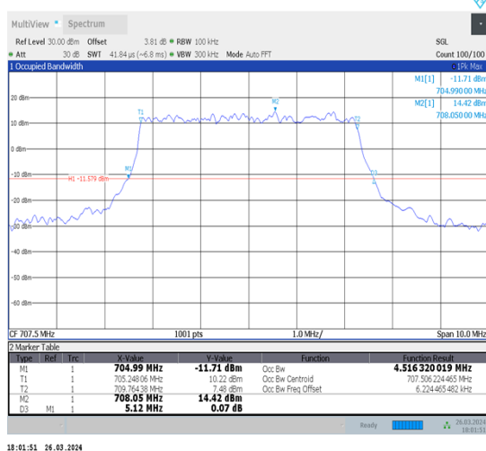
1-N12-15-5-M-7-CP-16QAM-Outer_Full-25@0-Ant1-4.516-5.120-≤5-PASS
