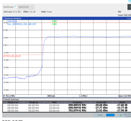
1-N12-15-10-L-3-DFT-PI2BPSK-Outer_Full-50@0-Ant1-1--PASS-see graph
