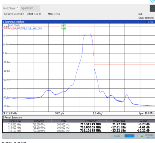
1-N12-15-10-H-2-DFT-PI2BPSK-Edge_1RB_Right-1@51-Ant1-1--PASS-see graph
