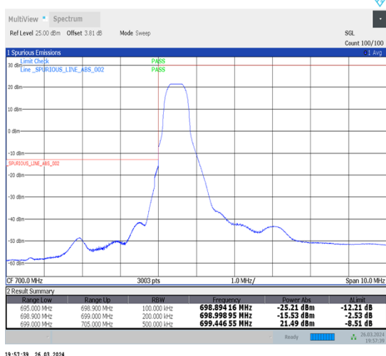
1-N12-15-15-L-4-CP-QPSK-Edge_1RB_Left-1@0-Ant1-1--PASS-see graph
