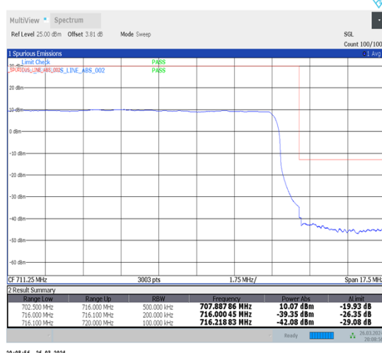
1-N12-15-15-H-3-DFT-PI2BPSK-Outer_Full-75@0-Ant1-1--PASS-see graph
