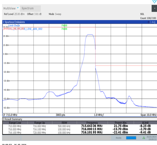
1-N12-15-5-H-2-DFT-PI2BPSK-Edge_1RB_Right-1@24-Ant1-1--PASS-see graph
