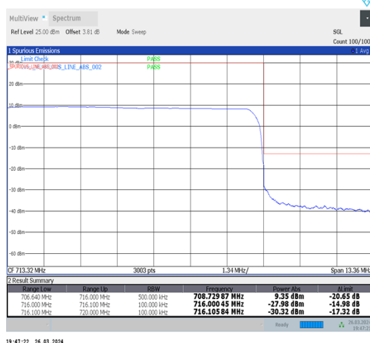
1-N12-15-10-H-6-CP-QPSK-Outer_Full-52@0-Ant1-1--PASS-see graph
