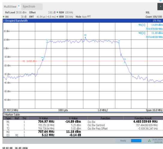
1-N12-15-5-M-9-CP-256QAM-Outer_Full-25@0-Ant1-4.486-5.120-≤5-PASS
