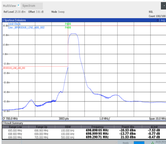
1-N12-15-5-L-4-CP-QPSK-Edge_1RB_Left-1@0-Ant1-1--PASS-see graph
