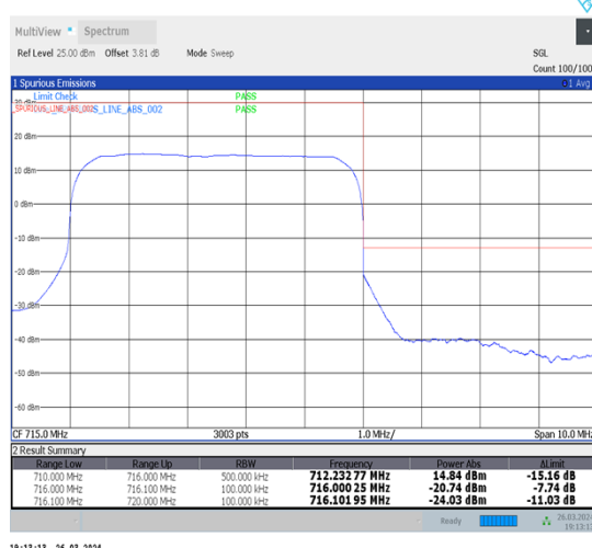
1-N12-15-5-H-3-DFT-PI2BPSK-Outer_Full-25@0-Ant1-1--PASS-see graph
