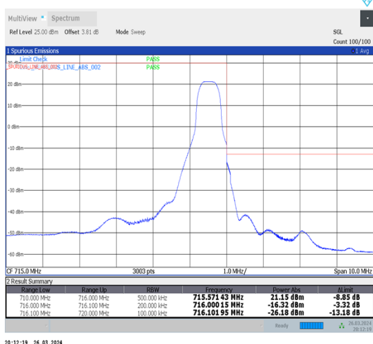
1-N12-15-15-H-5-CP-QPSK-Edge_1RB_Right-1@78-Ant1-1--PASS-see graph
