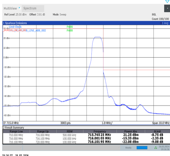
1-N12-15-5-H-5-CP-QPSK-Edge_1RB_Right-1@24-Ant1-1--PASS-see graph
