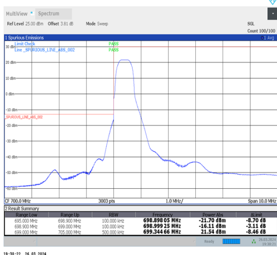
1-N12-15-10-L-4-CP-QPSK-Edge_1RB_Left-1@0-Ant1-1--PASS-see graph
