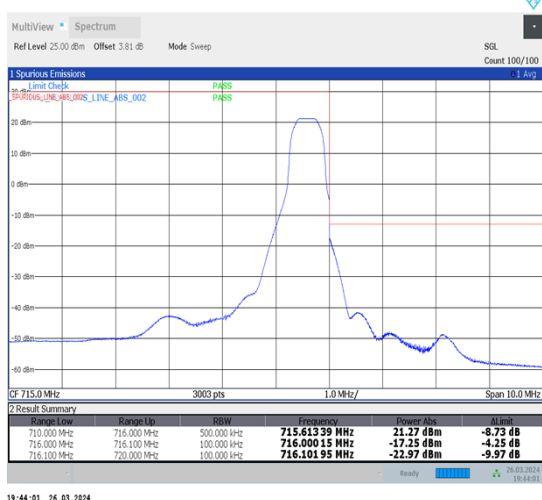
1-N12-15-10-H-5-CP-QPSK-Edge_1RB_Right-1@51-Ant1-1--PASS-see graph
