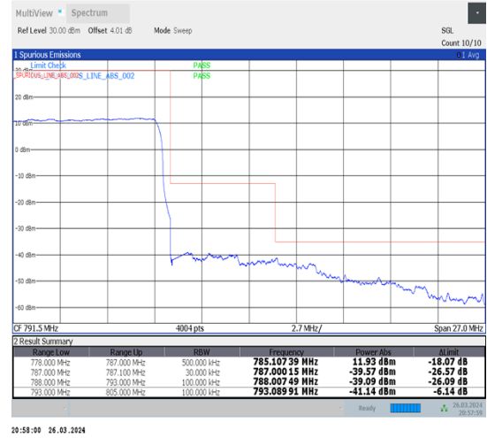
1-N13-15-10-H-3-DFT-PI2BPSK-Outer_Full-50@0-Ant1-1--PASS-see graph
