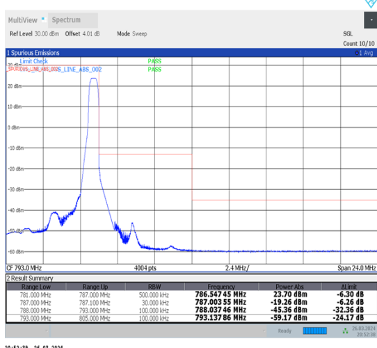
1-N13-15-5-H-2-DFT-PI2BPSK-Edge_1RB_Right-1@24-Ant1-1--PASS-see graph
