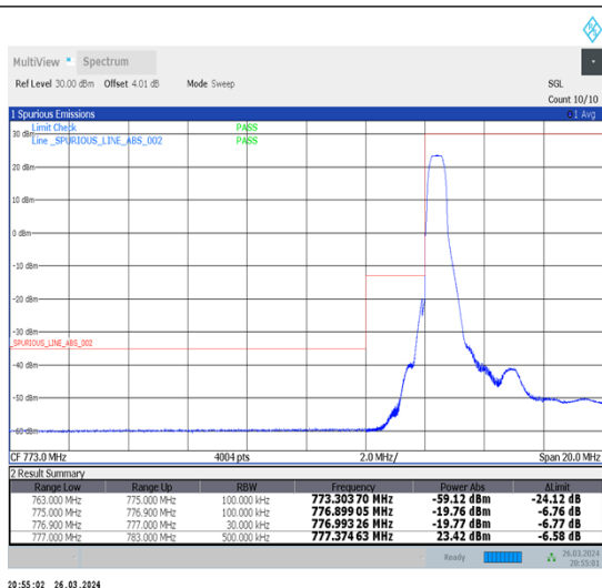
1-N13-15-10-L-1-DFT-PI2BPSK-Edge_1RB_Left-1@0-Ant1-1--PASS-see graph
