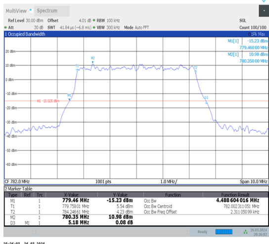
1-N13-15-5-M-9-CP-256QAM-Outer_Full-25@0- Ant1-4.489-5.180-≤5-PASS
