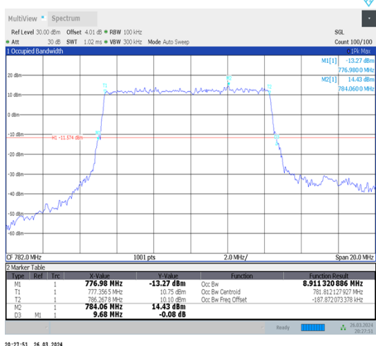
1-N13-15-10-M-2-DFT-PI2BPSK-Outer_Full-50@0- Ant1-8.911-9.680-≤10-PASS
