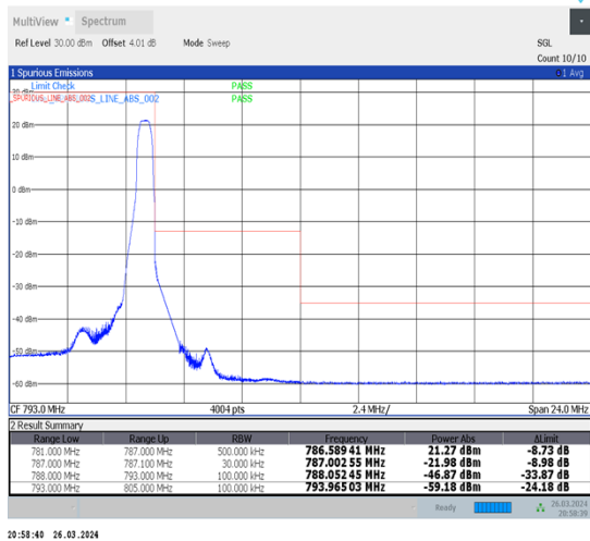
1-N13-15-10-H-5-CP-QPSK-Edge_1RB_Right-1@51-Ant1-1--PASS-see graph
