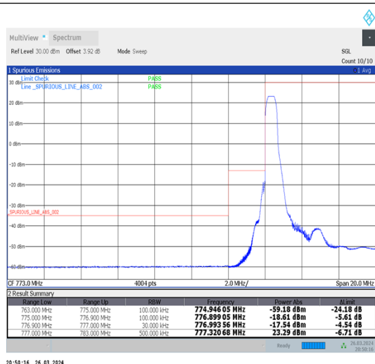
1-N13-15-5-L-1-DFT-PI2BPSK-Edge_1RB_Left-1@0-Ant1-1--PASS-see graph
