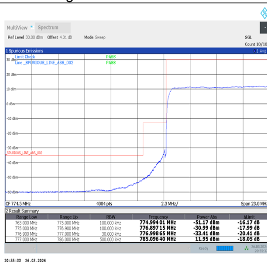
1-N13-15-10-L-3-DFT-PI2BPSK-Outer_Full-50@0-Ant1-1--PASS-see graph
