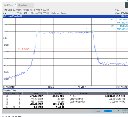
1-N13-15-10-M-5-DFT-256QAM-Outer_Full-50@0-Ant1-8.889-9.500-≤10-PASS
