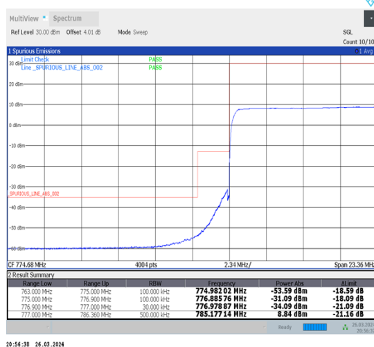
1-N13-15-10-L-6-CP-QPSK-Outer_Full-52@0-Ant1-1--PASS-see graph
