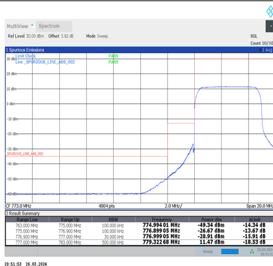
1-N13-15-5-L-6-CP-QPSK-Outer_Full-25@0-Ant1-1--PASS-see graph
