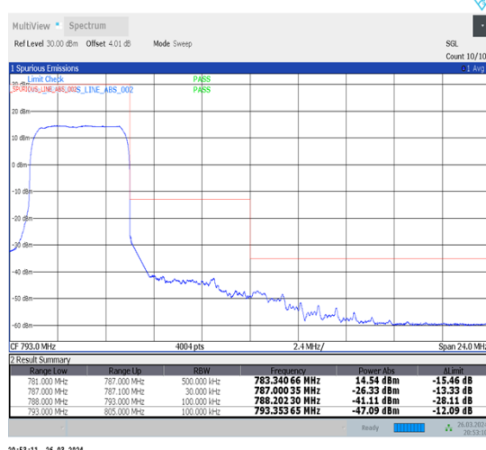
1-N13-15-5-H-3-DFT-PI2BPSK-Outer_Full-25@0-Ant1-1--PASS-see graph
