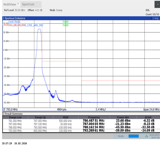
1-N13-15-10-H-2-DFT-PI2BPSK-Edge_1RB_Right-1@51-Ant1-1--PASS-see graph
