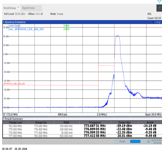
1-N13-15-10-L-4-CP-QPSK-Edge_1RB_Left-1@0-Ant1-1--PASS-see graph
