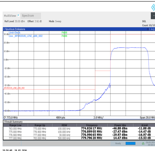
1-N13-15-5-L-3-DFT-PI2BPSK-Outer_Full-25@0-Ant1-1--PASS-see graph
