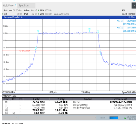
1-N13-15-10-M-4-DFT-64QAM-Outer_Full-50@0-Ant1-8.93-9.620-≤10-PASS
