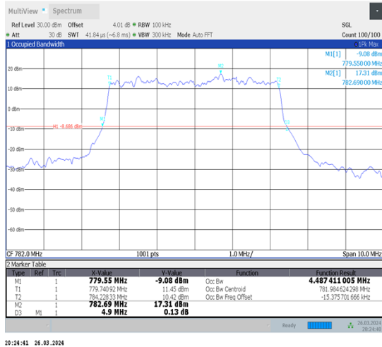
1-N13-15-5-M-1-DFT-QPSK-Outer_Full-25@0-Ant1-4.487-4.900-≤5-PASS
