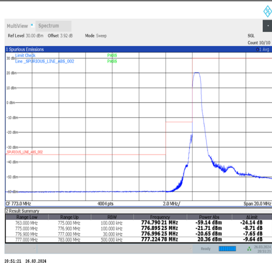
1-N13-15-5-L-4-CP-QPSK-Edge_1RB_Left-1@0-Ant1-1--PASS-see graph
