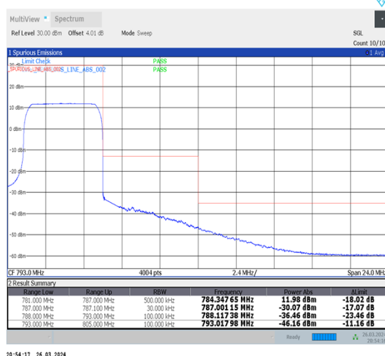
1-N13-15-5-H-6-CP-QPSK-Outer_Full-25@0-Ant1-1--PASS-see graph
