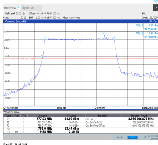
1-N13-15-10-M-3-DFT-16QAM-Outer_Full-50@0- Ant1-8.956-9.680-≤10-PASS
