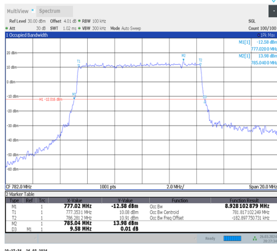
1-N13-15-10-M-1-DFT-QPSK-Outer_Full-50@0- Ant1-8.928-9.580-≤10-PASS
