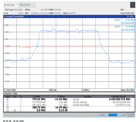
1-N13-15-5-M-4-DFT-64QAM-Outer_Full-25@0-Ant1-4.453-5.000-≤5-PASS
