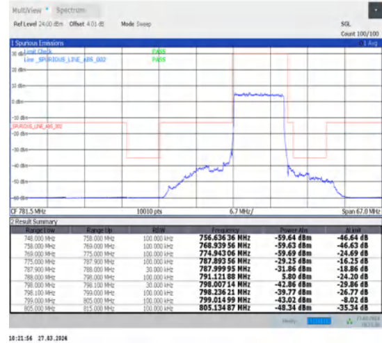
1-N14-15-10-L-3-DFT-PI2BPSK-Outer_Full-50@0-Ant1-1--PASS-see graph
