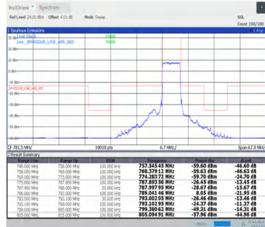
1-N14-15-5-L-3-DFT-PI2BPSK-Outer_Full-25@0-Ant1-1--PASS-see graph
