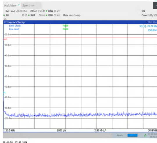
1-N14-15-10-L-1-DFT-PI2BPSK-Inner_1RB_Left- 1@1-0.15-30-Ant1-0.15--78.78--23-PASS
