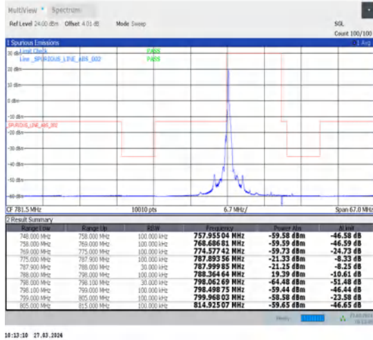
1-N14-15-10-L-1-DFT-PI2BPSK-Edge_1RB_Left-1@0-Ant1-1--PASS-see graph
