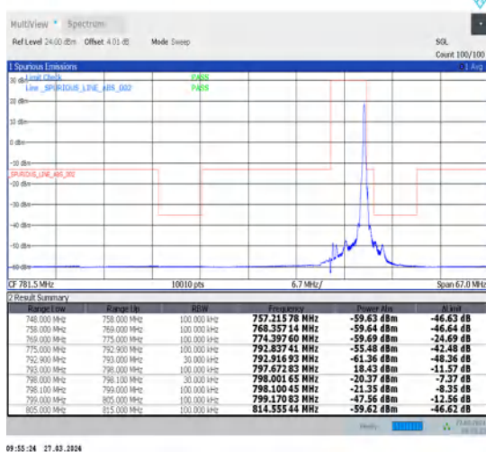
1-N14-15-5-H-5-CP-QPSK-Edge_1RB_Right-1@24-Ant1-1--PASS-see graph
