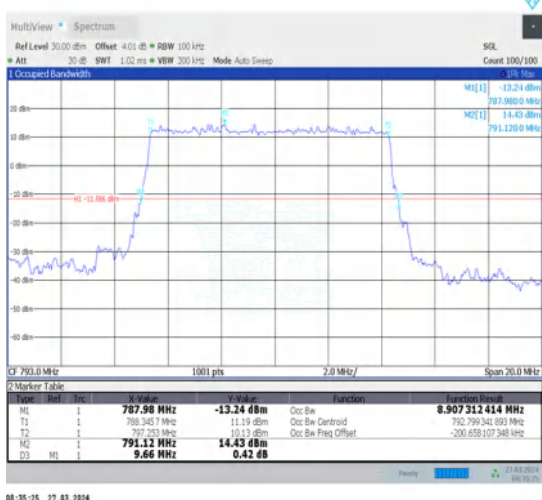
1-N14-15-10-M-2-DFT-PI2BPSK-Outer_Full-50@0-Ant1-8.907-9.660-≤10-PASS
