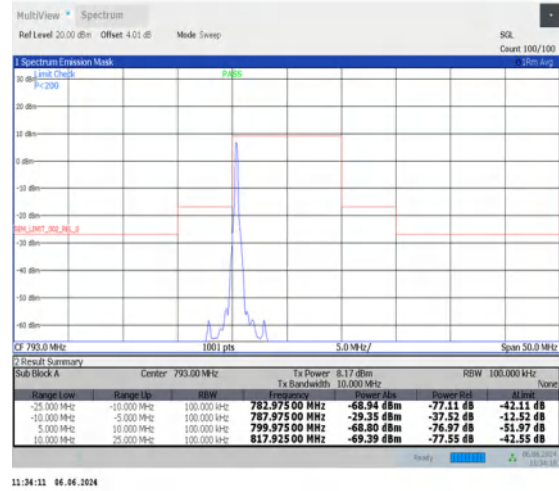
NTNV_N14_15_10_L_TID2_-25.00_-10.00_100.00_#1
