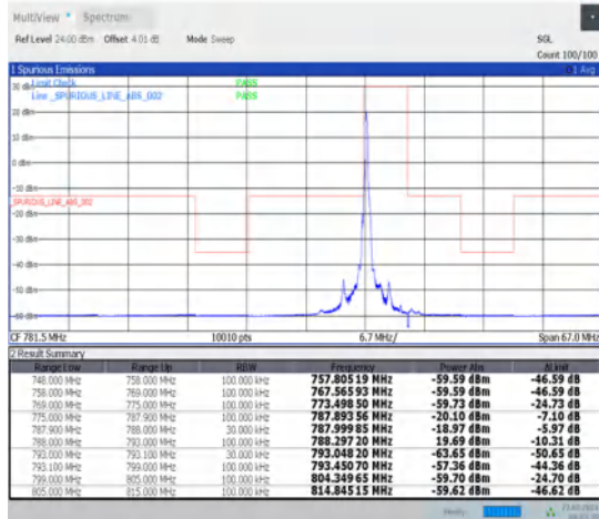
1-N14-15-5-L-1-DFT-PI2BPSK-Edge_1RB_Left-1@0-Ant1-1--PASS-see graph
