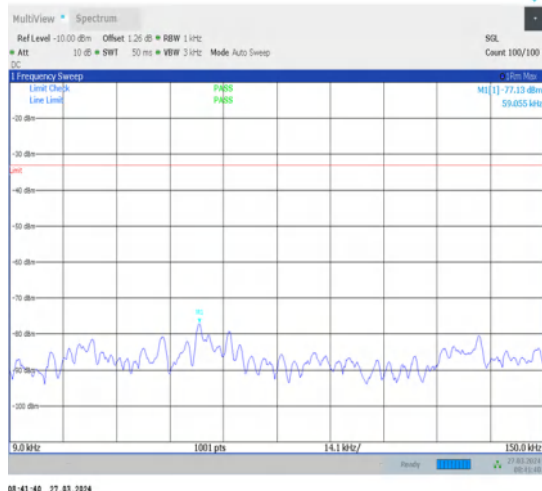
1-N14-15-10-L-1-DFT-PI2BPSK-Inner_1RB_Left- 1@1-0.009-0.15-Ant1-0.06--77.13--33-PASS
