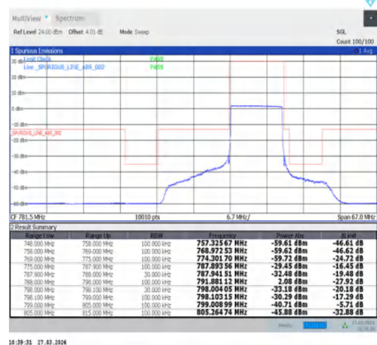
1-N14-15-10-L-6-CP-QPSK-Outer_Full-52@0-Ant1-1--PASS-see graph
