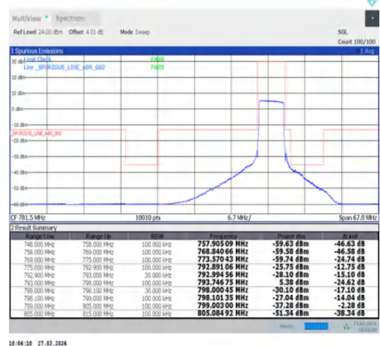
1-N14-15-5-H-6-CP-QPSK-Outer_Full-25@0-Ant1-1--PASS-see graph
