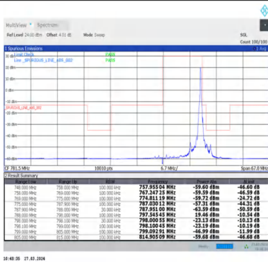
1-N14-15-10-H-2-DFT-PI2BPSK-Edge_1RB_Right-1@51-Ant1-1--PASS-see graph
