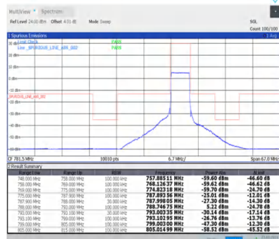
1-N14-15-5-L-6-CP-QPSK-Outer_Full-25@0-Ant1-1--PASS-see graph
