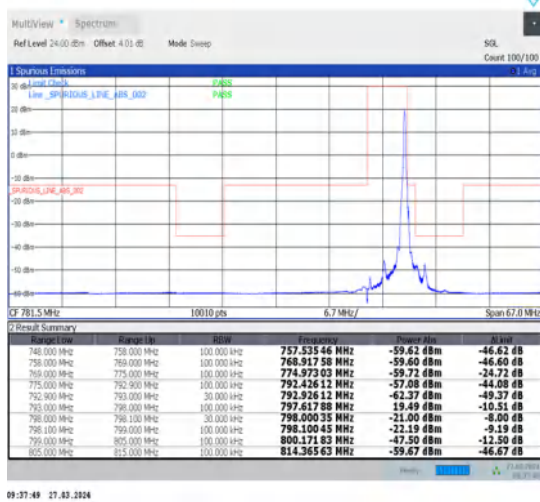
1-N14-15-5-H-2-DFT-PI2BPSK-Edge_1RB_Right-1@24-Ant1-1--PASS-see graph
