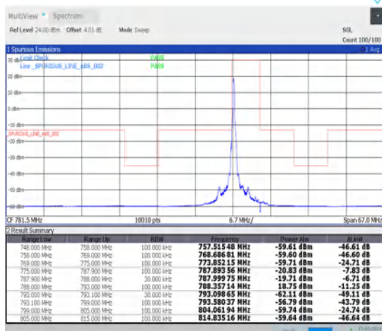
1-N14-15-5-L-4-CP-QPSK-Edge_1RB_Left-1@0-Ant1-1--PASS-see graph
