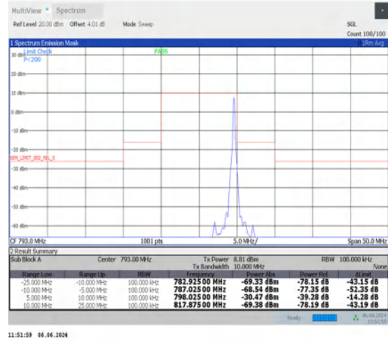
NTNV_N14_15_10_H_TID3_-25.00_-10.00_100.00_#1
