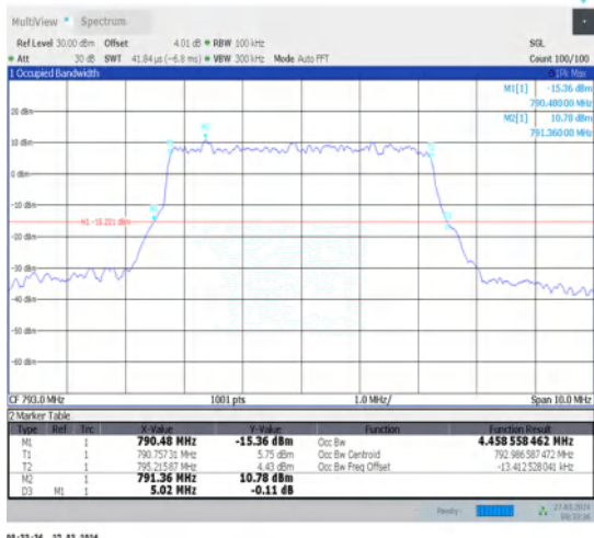
1-N14-15-5-M-9-CP-256QAM-Outer_Full-25@0-Ant1-4.459-5.020-≤5-PASS
