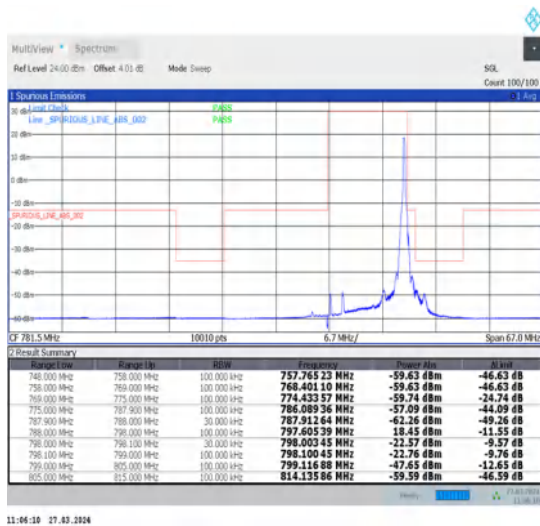
1-N14-15-10-H-5-CP-QPSK-Edge_1RB_Right-1@51-Ant1-1--PASS-see graph
