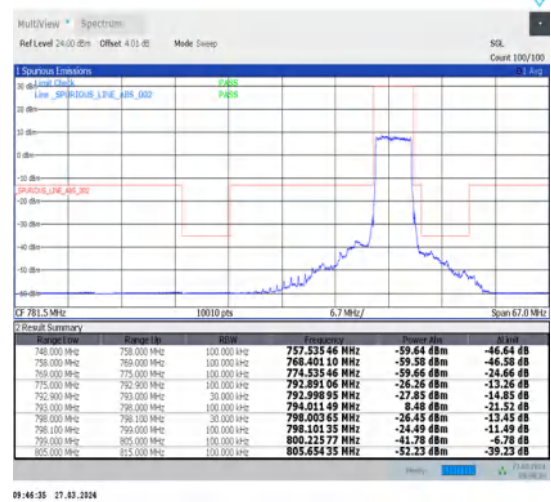
1-N14-15-5-H-3-DFT-PI2BPSK-Outer_Full-25@0-Ant1-1--PASS-see graph
