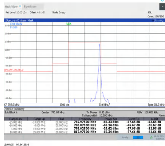
NTNV_N14_15_10_H_TID6_-25.00_-10.00_100.00_#1
