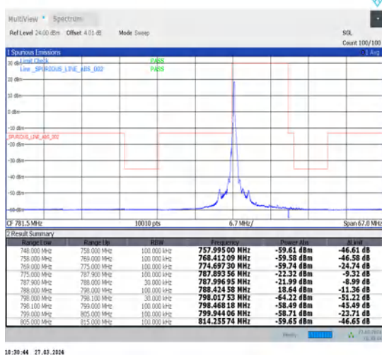
1-N14-15-10-L-4-CP-QPSK-Edge_1RB_Left-1@0-Ant1-1--PASS-see graph
