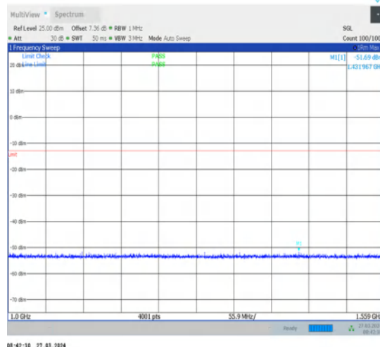
1-N14-15-10-L-1-DFT-PI2BPSK-Inner_1RB_Left- 1@1-1000-1559-Ant1-1431.97--51.69--13-PASS
