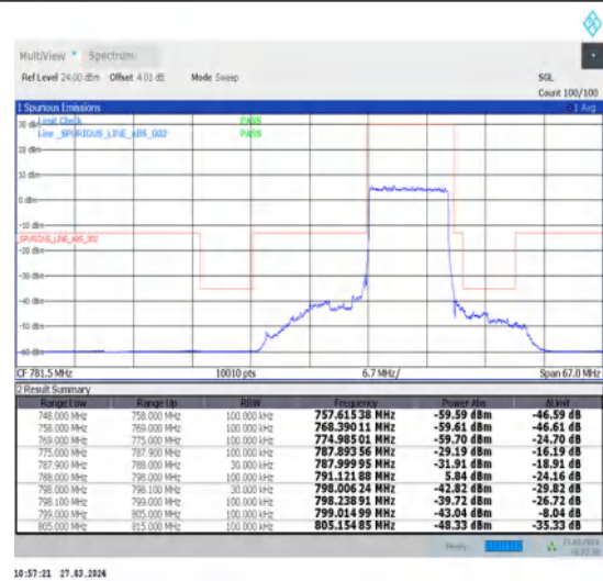
1-N14-15-10-H-3-DFT-PI2BPSK-Outer_Full-50@0-Ant1-1--PASS-see graph
