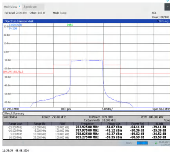
NTNV_N14_15_10_L_TID4_-25.00_-10.00_100.00_#1
