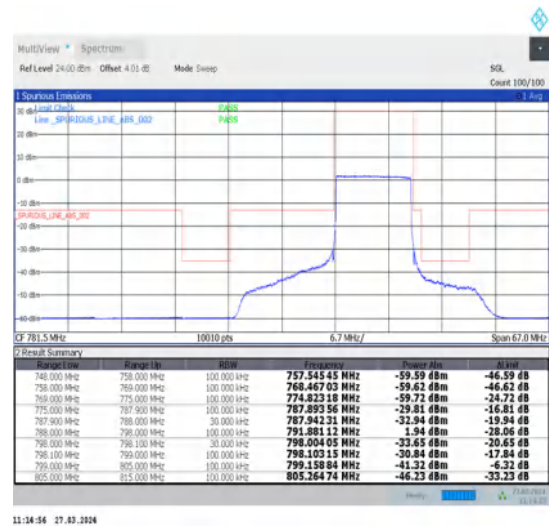
1-N14-15-10-H-6-CP-QPSK-Outer_Full-52@0-Ant1-1--PASS-see graph
