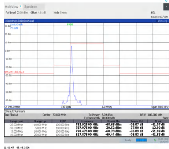
NTNV_N14_15_10_L_TID5_-25.00_-10.00_100.00_#1
