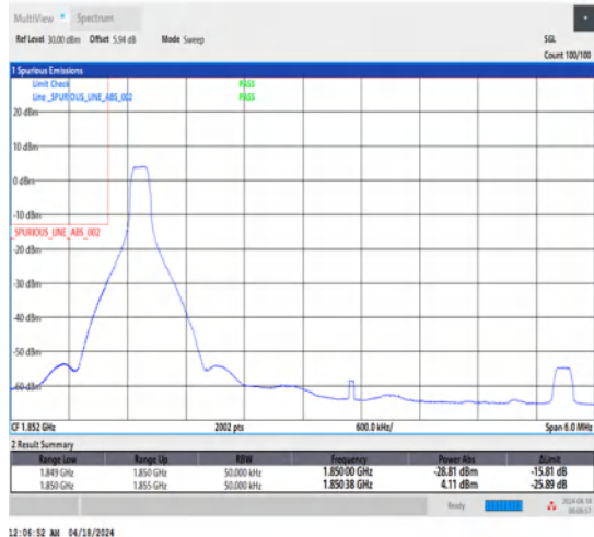
1-N25-15-5-L-4-CP-QPSK-Edge_1RB_Left-1@0-Ant1-1-seegraph-PASS-see graph
