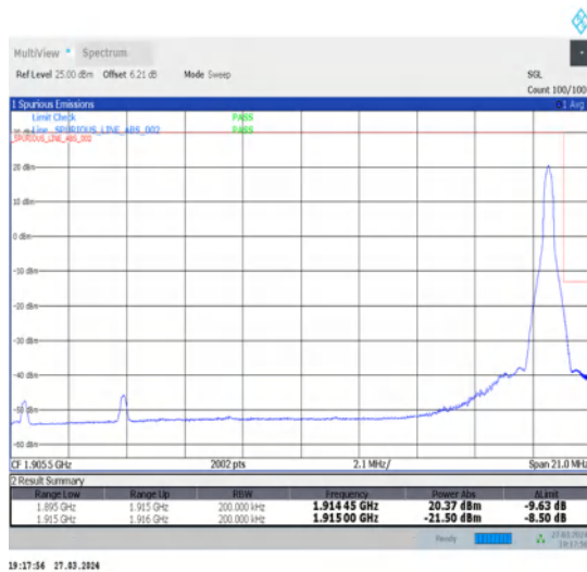
1-N25-15-20-H-5-CP-QPSK-Edge_1RB_Right-1@105-Ant1-1-seegraph-PASS-see graph
