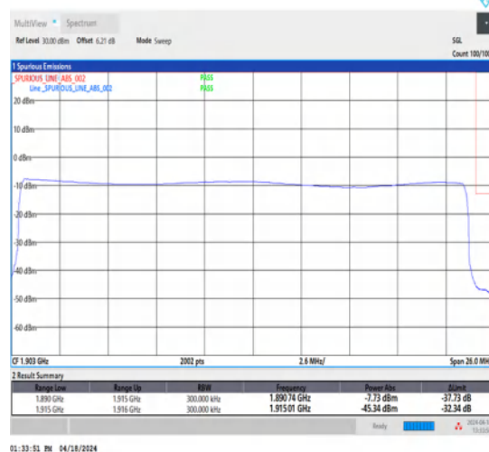
1-N25-15-25-H-6-CP-QPSK-Outer_Full-133@0-Ant1-1-seegraph-PASS-see graph
