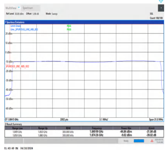
1-N25-15-30-L-6-CP-QPSK-Outer_Full-160@0-Ant1-1-seegraph-PASS-see graph
