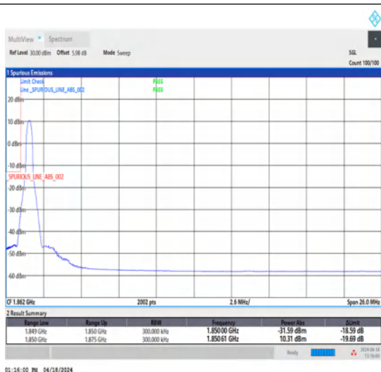
1-N25-15-25-L-1-DFT-PI2BPSK-Edge_1RB_Left-1@0-Ant1-1-seegraph-PASS-see graph
