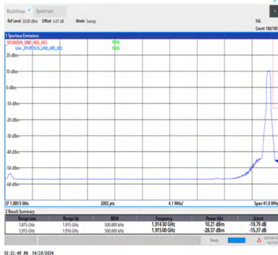
1-N25-15-40-H-5-CP-QPSK-Edge_1RB_Right-1@215-Ant1-1-seegraph-PASS-see graph
