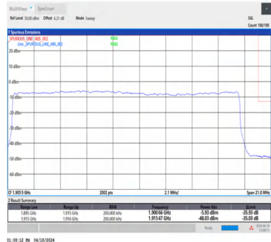
1-N25-15-20-H-3-DFT-PI2BPSK-Outer_Full-100@0-Ant1-1-seegraph-PASS-see graph
