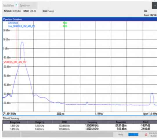
1-N25-15-10-L-4-CP-QPSK-Edge_1RB_Left-1@0-Ant1-1-seegraph-PASS-see graph
