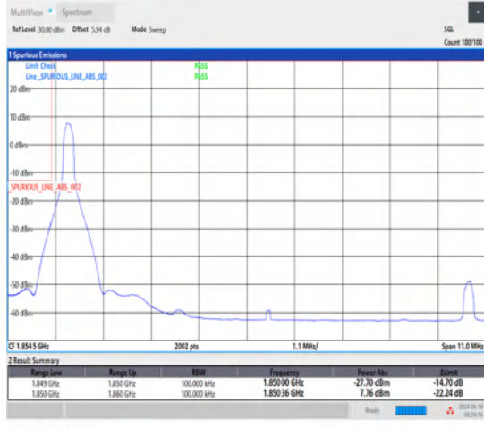
1-N25-15-10-L-1-DFT-PI2BPSK-Edge_1RB_Left-1@0-Ant1-1-seegraph-PASS-see graph
