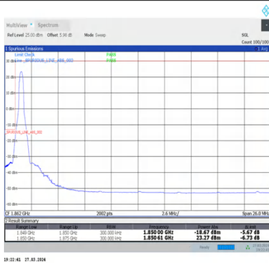
1-N25-15-25-L-1-DFT-PI2BPSK-Edge_1RB_Left-1@0-Ant1-1-seegraph-PASS-see graph
