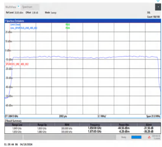
1-N25-15-30-L-3-DFT-PI2BPSK-Outer_Full-160@0-Ant1-1-seegraph-PASS-see graph
