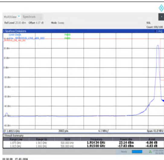
1-N25-15-40-H-2-DFT-PI2BPSK-Edge_1RB_Right-1@215-Ant1-1-seegraph-PASS-see graph
