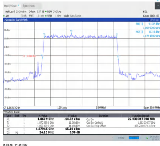
1-N25-15-25-M-2-DFT-PI2BPSK-Outer_Full-128@0-Ant1-22.93-24.150-≤25-PASS
