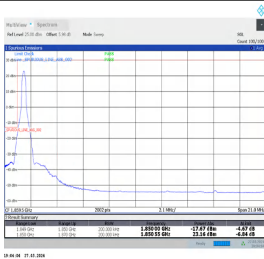
1-N25-15-20-L-1-DFT-PI2BPSK-Edge_1RB_Left-1@0-Ant1-1-seegraph-PASS-see graph
