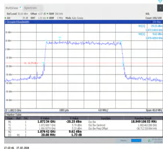
1-N25-15-20-M-9-CP-256QAM-Outet_Full-106@0-Ant1-18.949-20.080-≤20-PASS
