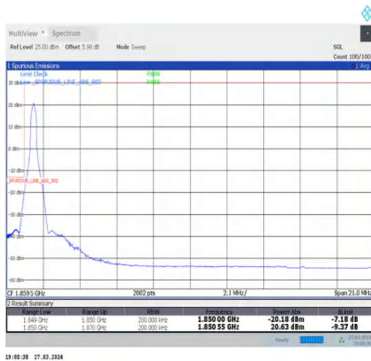
1-N25-15-20-L-4-CP-QPSK-Edge_1RB_Left-1@0-Ant1-1-seegraph-PASS-see graph
