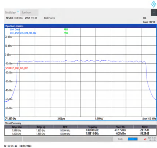
1-N25-15-15-L-3-DFT-PI2BPSK-Outer_Full-75@0-Ant1-1-seegraph-PASS-see graph
