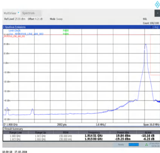
1-N25-15-15-H-5-CP-QPSK-Edge_1RB_Right-1@78-Ant1-1-seegraph-PASS-see graph
