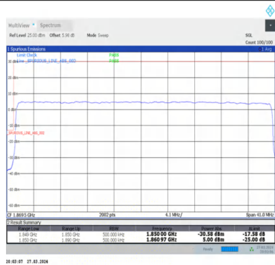
1-N25-15-40-L-3-DFT-PI2BPSK-Outer_Full-216@0-Ant1-1-seegraph-PASS-see graph
