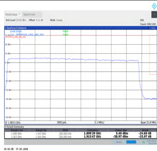
1-N25-15-20-H-3-DFT-PI2BPSK-Outer_Full-100@0-Ant1-1-seegraph-PASS-see graph
