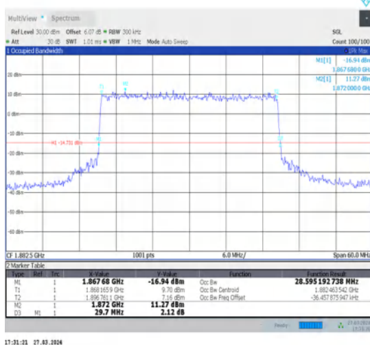
1-N25-15-30-M-6-CP-QPSK-Outer_Full-160@0-Ant1-28.598-29.700-≤30-PASS
