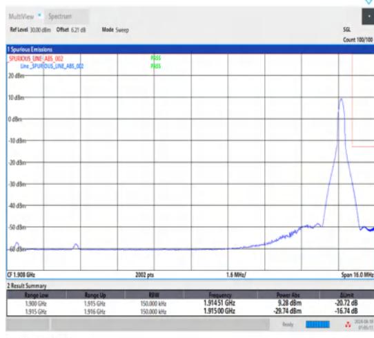
1-N25-15-15-H-5-CP-QPSK-Edge_1RB_Right-1@78-Ant1-1-seegraph-PASS-see graph
