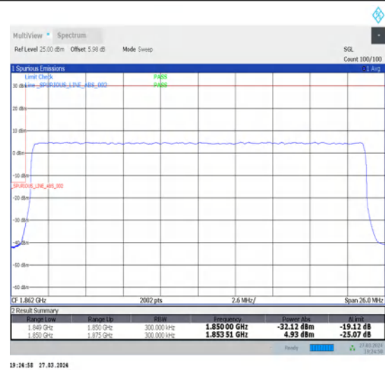
1-N25-15-25-L-3-DFT-PI2BPSK-Outer_Full-128@0-Ant1-1-seegraph-PASS-see graph
