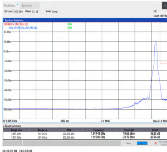
1-N25-15-20-H-2-DFT-PI2BPSK-Edge_1RB_Right-1@105-Ant1-1-seegraph-PASS-see graph
