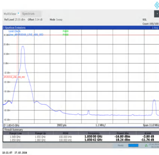
1-N25-15-10-L-4-CP-QPSK-Edge_1RB_Left-1@0-Ant1-1-seegraph-PASS-see graph
