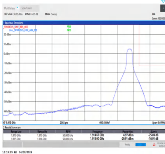
1-N25-15-5-H-5-CP-QPSK-Edge_1RB_Right-1@24-Ant1-1-seegraph-PASS-see graph
