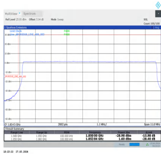
1-N25-15-10-L-6-CP-QPSK-Outer_Full-52@0-Ant1-1-seegraph-PASS-see graph
