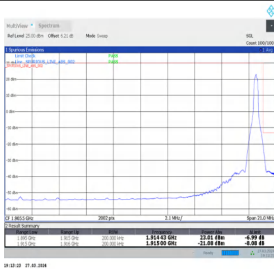
1-N25-15-20-H-2-DFT-PI2BPSK-Edge_1RB_Right-1@105-Ant1-1-seegraph-PASS-see graph
