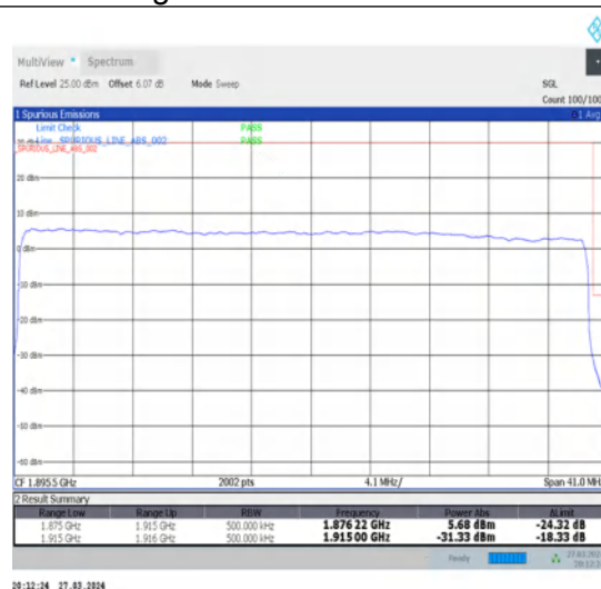
1-N25-15-40-H-3-DFT-PI2BPSK-Outer_Full-216@0-Ant1-1-seegraph-PASS-see graph
