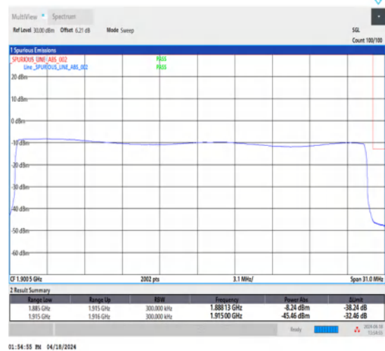
1-N25-15-30-H-6-CP-QPSK-Outer_Full-160@0-Ant1-1-seegraph-PASS-see graph
