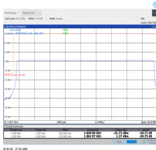
1-N25-15-15-L-6-CP-QPSK-Outer_Full-79@0-Ant1-1-seegraph-PASS-see graph
