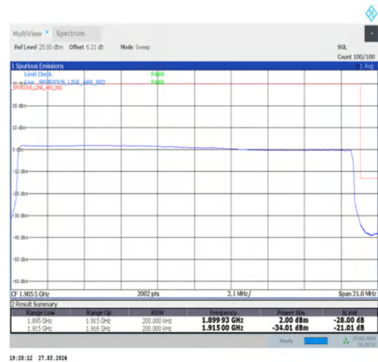
1-N25-15-20-H-6-CP-QPSK-Outer_Full-106@0-Ant1-1-seegraph-PASS-see graph
