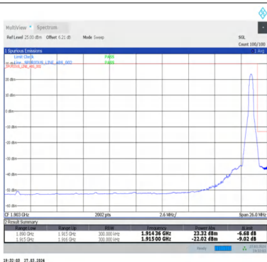
1-N25-15-25-H-2-DFT-PI2BPSK-Edge_1RB_Right-1@132-Ant1-1-seegraph-PASS-see graph
