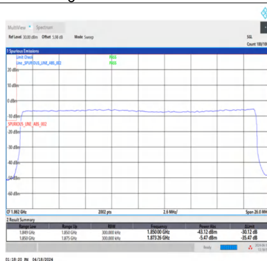
1-N25-15-25-L-3-DFT-PI2BPSK-Outer_Full-128@0-Ant1-1-seegraph-PASS-see graph
