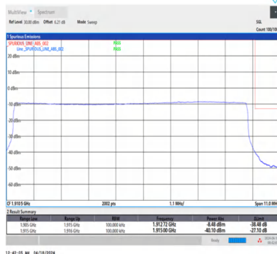
1-N25-15-10-H-6-CP-QPSK-Outer_Full-52@0-Ant1-1-seegraph-PASS-see graph
