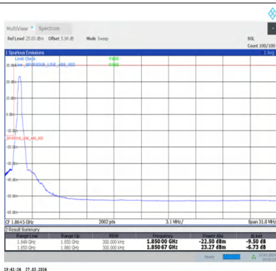
1-N25-15-30-L-1-DFT-PI2BPSK-Edge_1RB_Left-1@0-Ant1-1-seegraph-PASS-see graph
