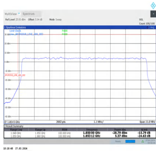
1-N25-15-10-L-3-DFT-PI2BPSK-Outer_Full-50@0-Ant1-1-seegraph-PASS-see graph
