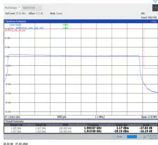
1-N25-15-10-H-6-CP-QPSK-Outer_Full-52@0-Ant1-1-seegraph-PASS-see graph
