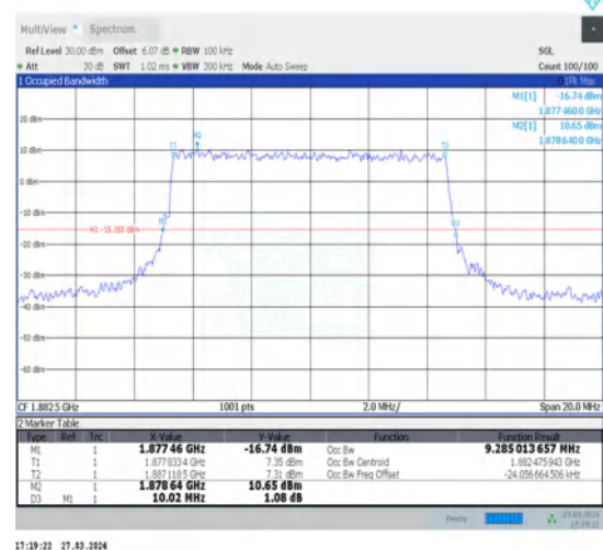
1-N25-15-10-M-7-CP-16QAM-Outer_Full-52@0-Ant1-9.285-10.020-≤10-PASS
