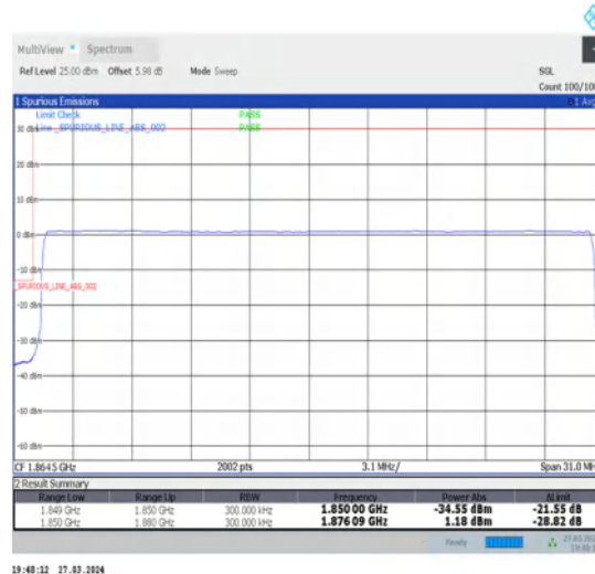
1-N25-15-30-L-6-CP-QPSK-Outer_Full-160@0-Ant1-1-seegraph-PASS-see graph
