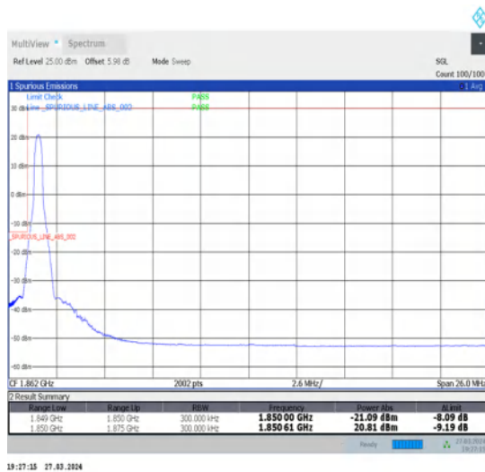
1-N25-15-25-L-4-CP-QPSK-Edge_1RB_Left-1@0-Ant1-1-seegraph-PASS-see graph
