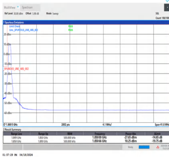
1-N25-15-40-L-1-DFT-PI2BPSK-Edge_1RB_Left-1@0-Ant1-1-seegraph-PASS-see graph
