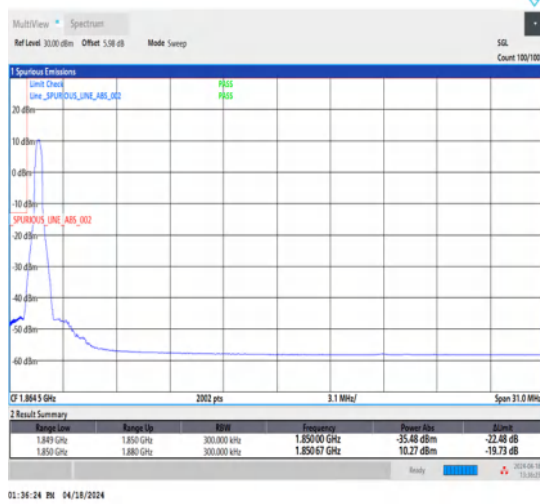
1-N25-15-30-L-1-DFT-PI2BPSK-Edge_1RB_Left-1@0-Ant1-1-seegraph-PASS-see graph
