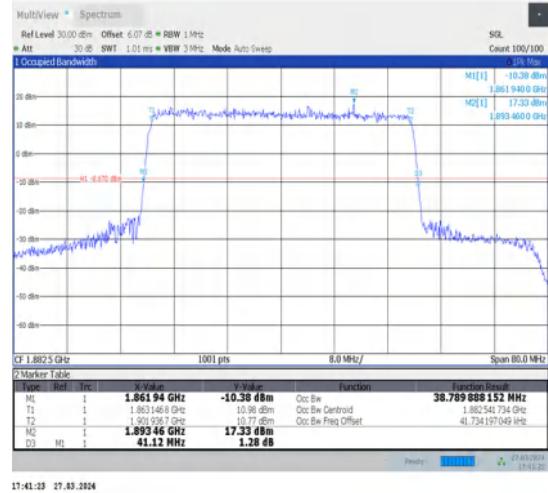
1-N25-15-40-M-4-DFT-64QAM-Outet_Full-216@0-Ant1-38.79-41.120-≤40-PASS
