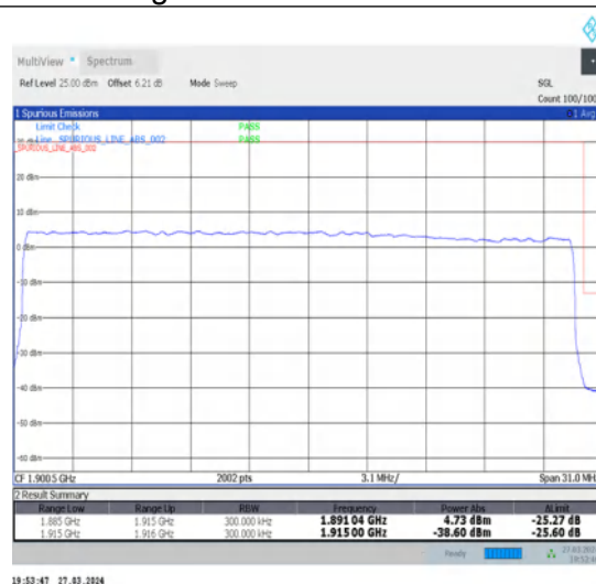
1-N25-15-30-H-3-DFT-PI2BPSK-Outer_Full-160@0-Ant1-1-seegraph-PASS-see graph
