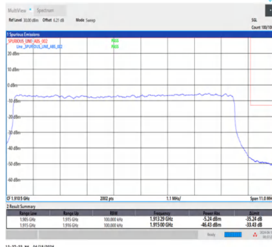
1-N25-15-10-H-3-DFT-PI2BPSK-Outer_Full-50@0-Ant1-1-seegraph-PASS-see graph
