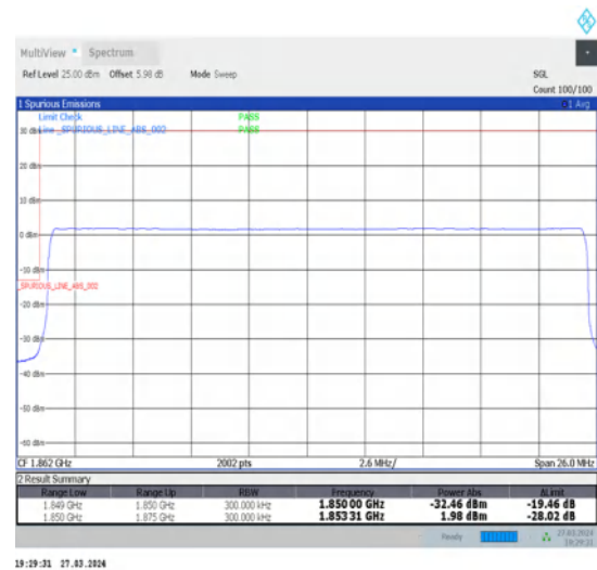
1-N25-15-25-L-6-CP-QPSK-Outer_Full-133@0-Ant1-1-seegraph-PASS-see graph
