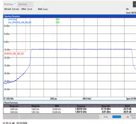
1-N25-15-5-L-6-CP-QPSK-Outer_Full-25@0-Ant1-1-seegraph-PASS-see graph
