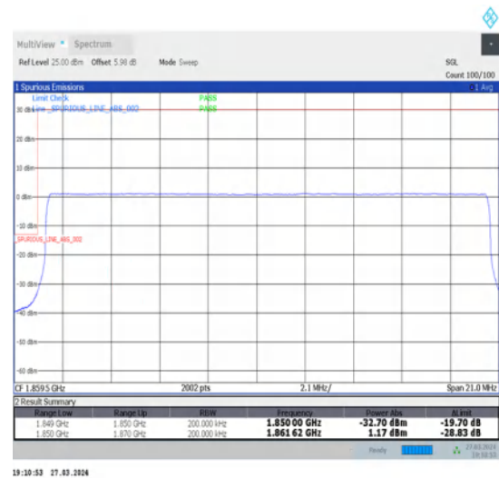
1-N25-15-20-L-6-CP-QPSK-Outer_Full-106@0-Ant1-1-seegraph-PASS-see graph
