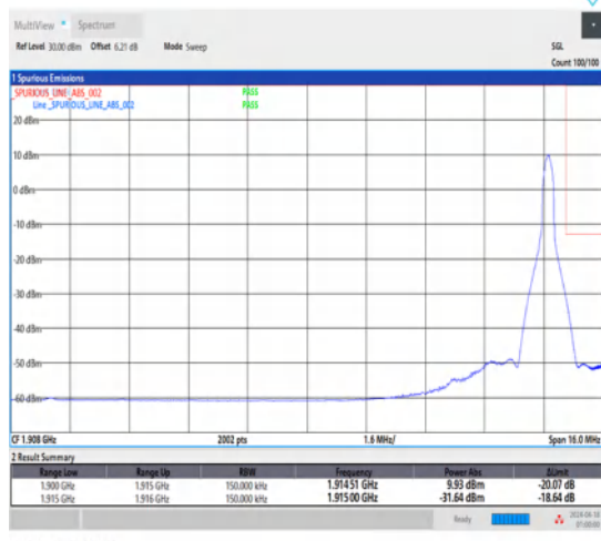
1-N25-15-15-H-2-DFT-PI2BPSK-Edge_1RB_Right-1@78-Ant1-1-seegraph-PASS-see graph
