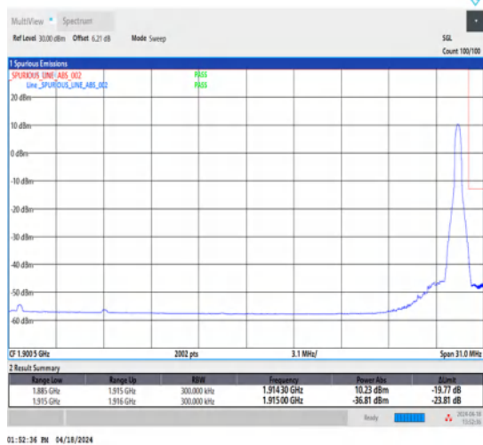
1-N25-15-30-H-5-CP-QPSK-Edge_1RB_Right-1@159-Ant1-1-seegraph-PASS-see graph
