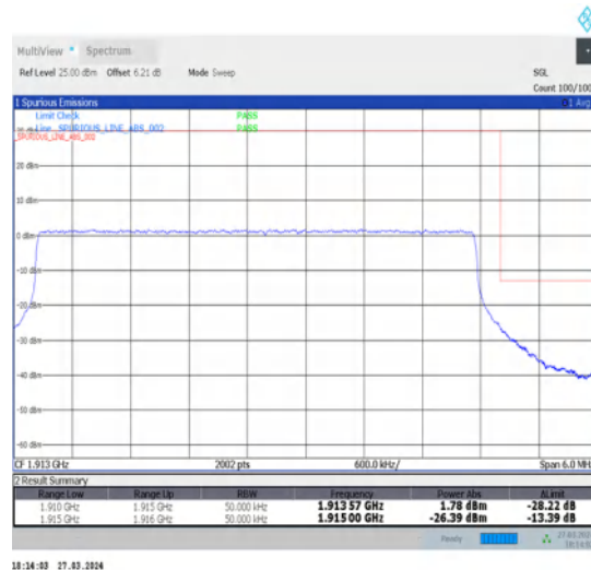
1-N25-15-5-H-6-CP-QPSK-Outer_Full-25@0-Ant1-1-seegraph-PASS-see graph
