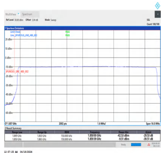
1-N25-15-15-L-6-CP-QPSK-Outer_Full-79@0-Ant1-1-seegraph-PASS-see graph
