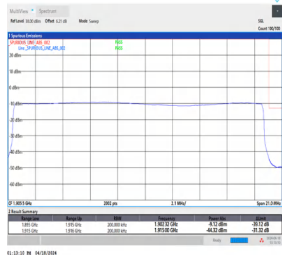
1-N25-15-20-H-6-CP-QPSK-Outer_Full-106@0-Ant1-1-seegraph-PASS-see graph
