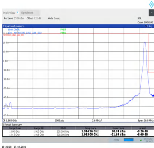
1-N25-15-25-H-5-CP-QPSK-Edge_1RB_Right-1@132-Ant1-1-seegraph-PASS-see graph
