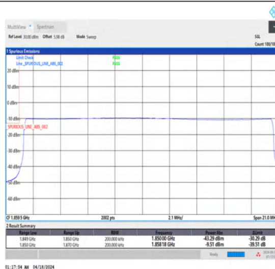
1-N25-15-20-L-6-CP-QPSK-Outer_Full-106@0-Ant1-1-seegraph-PASS-see graph
