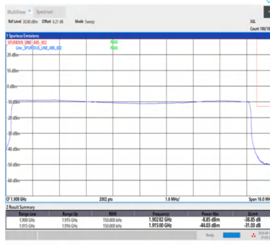
1-N25-15-15-H-6-CP-QPSK-Outer_Full-79@0-Ant1-1-seegraph-PASS-see graph
