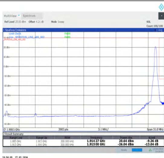
1-N25-15-30-H-5-CP-QPSK-Edge_1RB_Right-1@159-Ant1-1-seegraph-PASS-see graph
