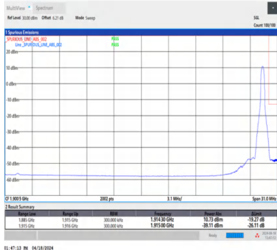
1-N25-15-30-H-2-DFT-PI2BPSK-Edge_1RB_Right-1@159-Ant1-1-seegraph-PASS-see graph
