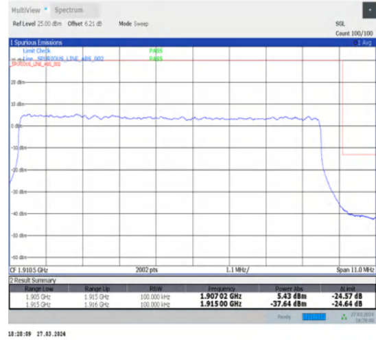
1-N25-15-10-H-3-DFT-PI2BPSK-Outer_Full-50@0-Ant1-1-seegraph-PASS-see graph
