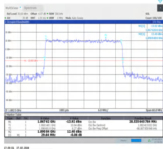
1-N25-15-30-M-3-DFT-16QAM-Outer_Full-160@0-Ant1-28.537-29.640-≤30-PASS
