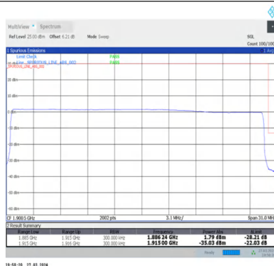
1-N25-15-30-H-6-CP-QPSK-Outer_Full-160@0-Ant1-1-seegraph-PASS-see graph
