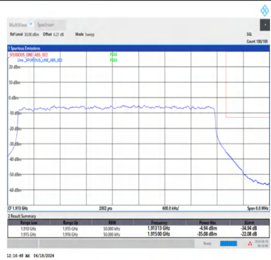
1-N25-15-5-H-3-DFT-PI2BPSK-Outer_Full-25@0-Ant1-1-seegraph-PASS-see graph
