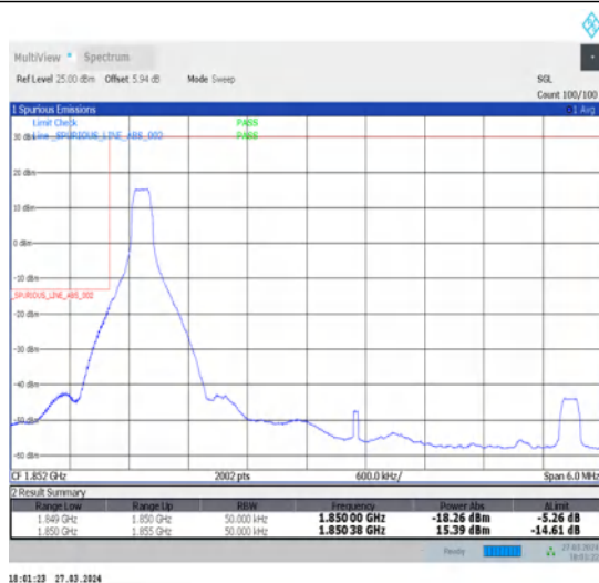
1-N25-15-5-L-4-CP-QPSK-Edge_1RB_Left-1@0-Ant1-1-seegraph-PASS-see graph
