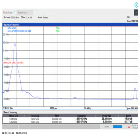
1-N25-15-15-L-4-CP-QPSK-Edge_1RB_Left-1@0-Ant1-1-seegraph-PASS-see graph
