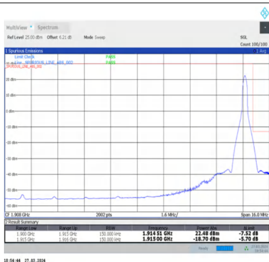
1-N25-15-15-H-2-DFT-PI2BPSK-Edge_1RB_Right-1@78-Ant1-1-seegraph-PASS-see graph
