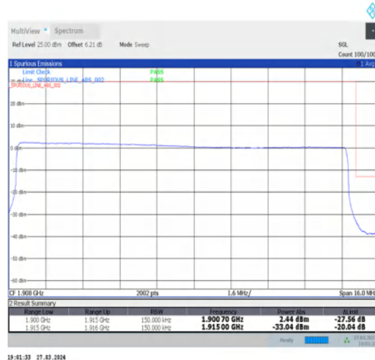
1-N25-15-15-H-6-CP-QPSK-Outer_Full-79@0-Ant1-1-seegraph-PASS-see graph
