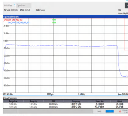
1-N25-15-25-H-3-DFT-PI2BPSK-Outer_Full-128@0-Ant1-1-seegraph-PASS-see graph
