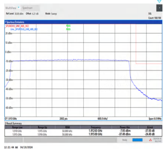
1-N25-15-5-H-6-CP-QPSK-Outer_Full-25@0-Ant1-1-seegraph-PASS-see graph
