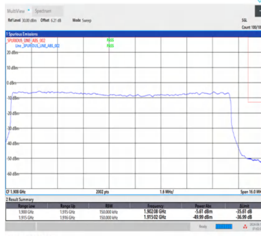
1-N25-15-15-H-3-DFT-PI2BPSK-Outer_Full-75@0-Ant1-1-seegraph-PASS-see graph
