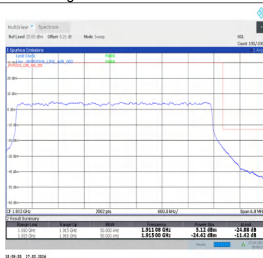
1-N25-15-5-H-3-DFT-PI2BPSK-Outer_Full-25@0-Ant1-1-seegraph-PASS-see graph
