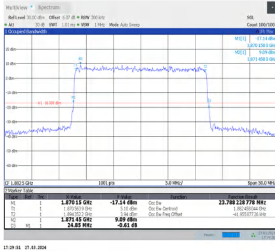
1-N25-15-25-M-9-CP-256QAM-Outer_Full-133@0-Ant1-23.788-24.850-≤25-PASS
