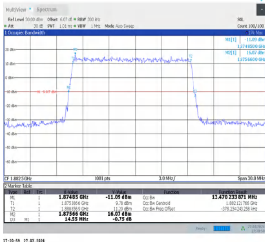
1-N25-15-15-M-3-DFT-16QAM-Outer_Full-75@0-Ant1-13.47-14.550-≤15-PASS
