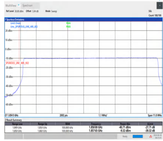
1-N25-15-10-L-6-CP-QPSK-Outer_Full-52@0-Ant1-1-seegraph-PASS-see graph
