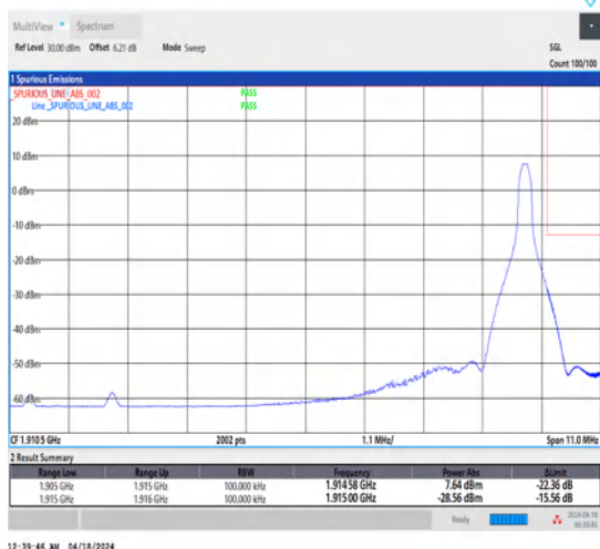
1-N25-15-10-H-5-CP-QPSK-Edge_1RB_Right-1@51-Ant1-1-seegraph-PASS-see graph
