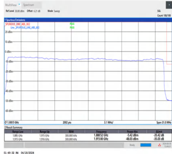
1-N25-15-30-H-3-DFT-PI2BPSK-Outer_Full-160@0-Ant1-1-seegraph-PASS-see graph
