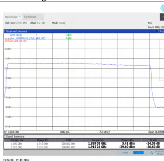
1-N25-15-25-H-3-DFT-PI2BPSK-Outer_Full-128@0-Ant1-1-seegraph-PASS-see graph
