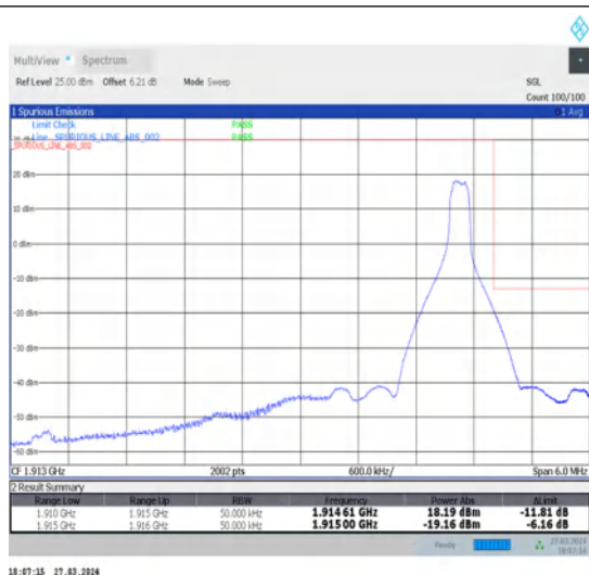
1-N25-15-5-H-2-DFT-PI2BPSK-Edge_1RB_Right-1@24-Ant1-1-seegraph-PASS-see graph
