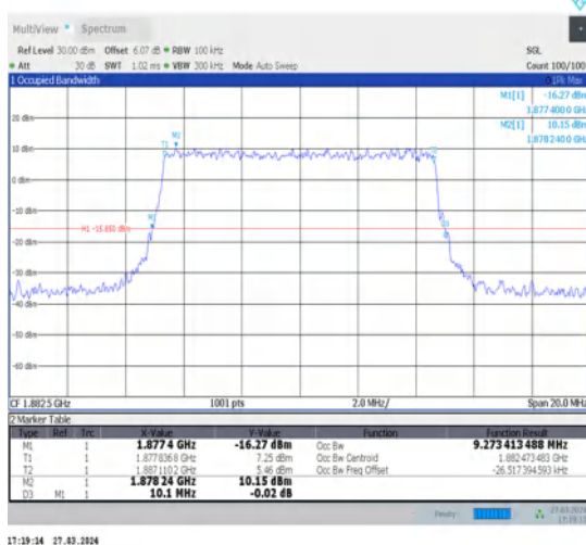
1-N25-15-10-M-6-CP-QPSK-Outer_Full-52@0-Ant1-9.273-10.100-≤10-PASS
