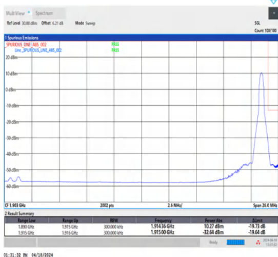
1-N25-15-25-H-5-CP-QPSK-Edge_1RB_Right-1@132-Ant1-1-seegraph-PASS-see graph
