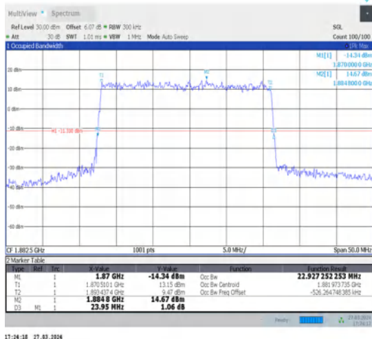
1-N25-15-25-M-1-DFT-QPSK-Outer_Full-128@0-Ant1-22.927-23.950-≤25-PASS
