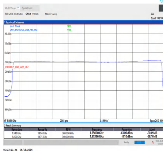
1-N25-15-25-L-6-CP-QPSK-Outer_Full-133@0-Ant1-1-seegraph-PASS-see graph
