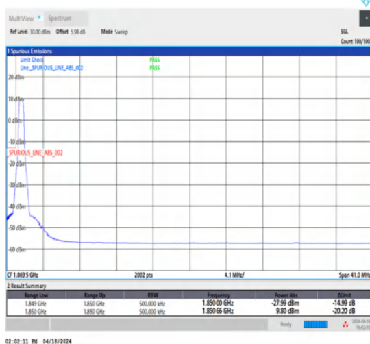
1-N25-15-40-L-4-CP-QPSK-Edge_1RB_Left-1@0-Ant1-1-seegraph-PASS-see graph
