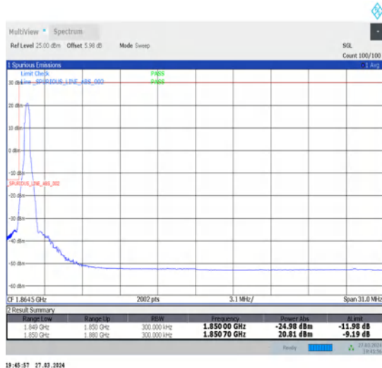
1-N25-15-30-L-4-CP-QPSK-Edge_1RB_Left-1@0-Ant1-1-seegraph-PASS-see graph
