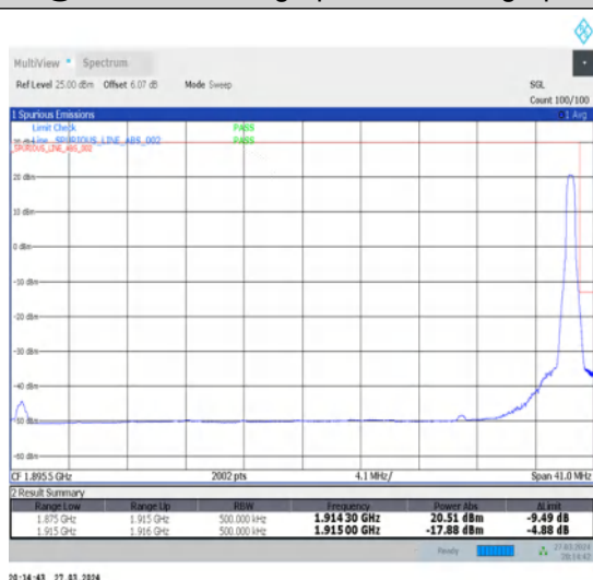
1-N25-15-40-H-5-CP-QPSK-Edge_1RB_Right-1@215-Ant1-1-seegraph-PASS-see graph
