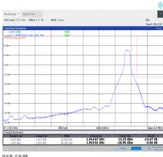
1-N25-15-5-H-5-CP-QPSK-Edge_1RB_Right-1@24-Ant1-1-seegraph-PASS-see graph
