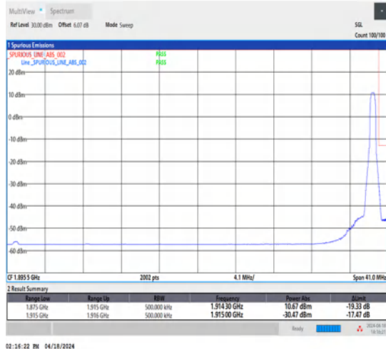
1-N25-15-40-H-2-DFT-PI2BPSK-Edge_1RB_Right-1@215-Ant1-1-seegraph-PASS-see graph
