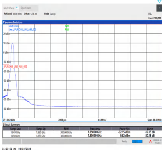
1-N25-15-25-L-4-CP-QPSK-Edge_1RB_Left-1@0-Ant1-1-seegraph-PASS-see graph
