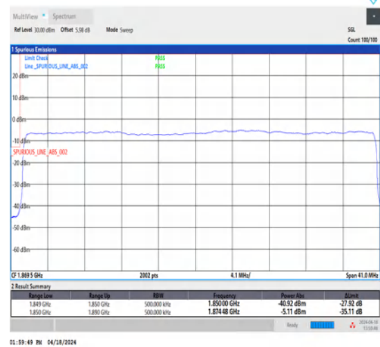
1-N25-15-40-L-3-DFT-PI2BPSK-Outer_Full-216@0-Ant1-1-seegraph-PASS-see graph
