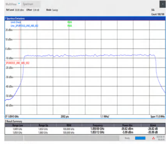
1-N25-15-10-L-3-DFT-PI2BPSK-Outer_Full-50@0-Ant1-1-seegraph-PASS-see graph
