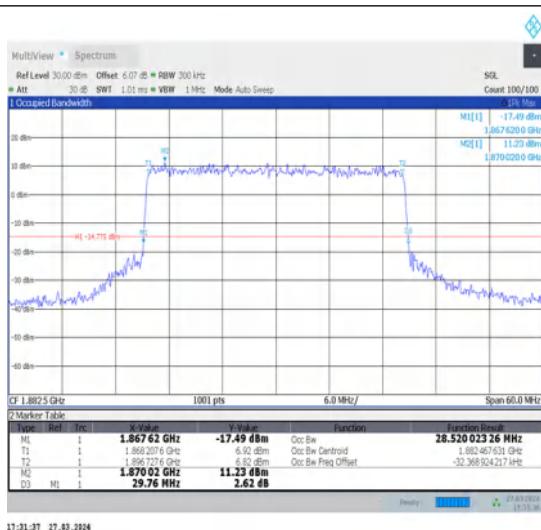
1-N25-15-30-M-8-CP-64QAM-Outer_Full-160@0-Ant1-28.521-29.760-≤30-PASS
