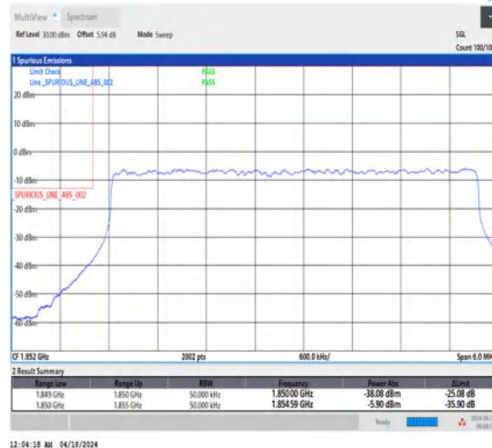
1-N25-15-5-L-3-DFT-PI2BPSK-Outer_Full-25@0-Ant1-1-seegraph-PASS-see graph
