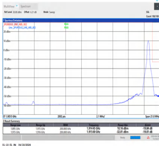
1-N25-15-20-H-5-CP-QPSK-Edge_1RB_Right-1@105-Ant1-1-seegraph-PASS-see graph
