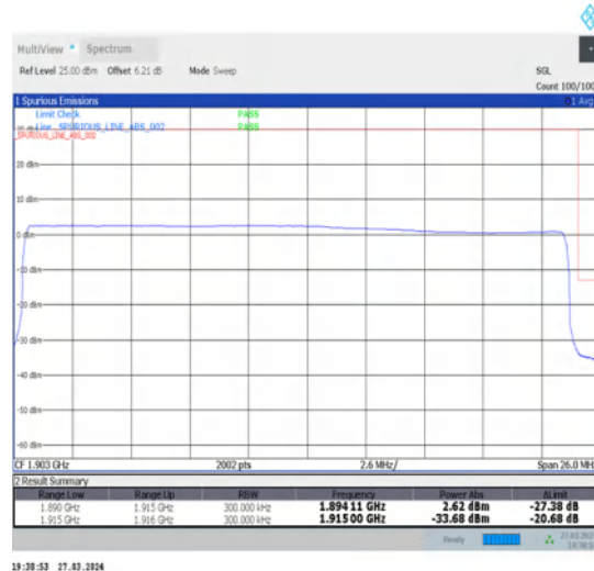
1-N25-15-25-H-6-CP-QPSK-Outer_Full-133@0-Ant1-1-seegraph-PASS-see graph
