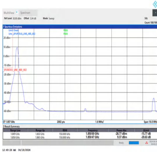
1-N25-15-15-L-1-DFT-PI2BPSK-Edge_1RB_Left-1@0-Ant1-1-seegraph-PASS-see graph
