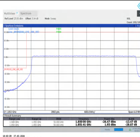
1-N25-15-5-L-6-CP-QPSK-Outer_Full-25@0-Ant1-1-seegraph-PASS-see graph
