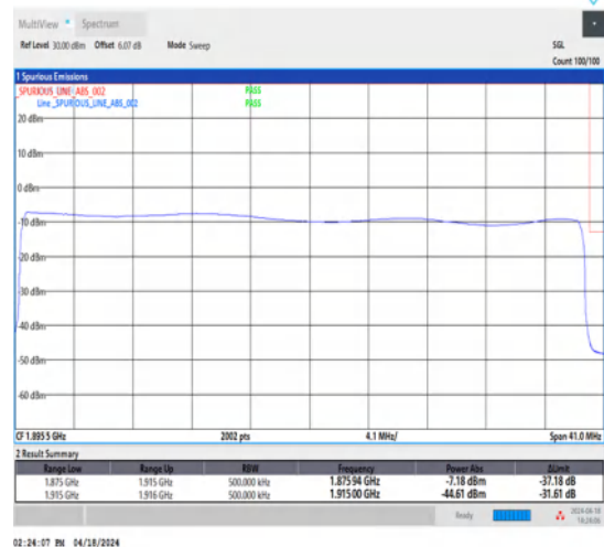
1-N25-15-40-H-6-CP-QPSK-Outer_Full-216@0-Ant1-1-seegraph-PASS-see graph
