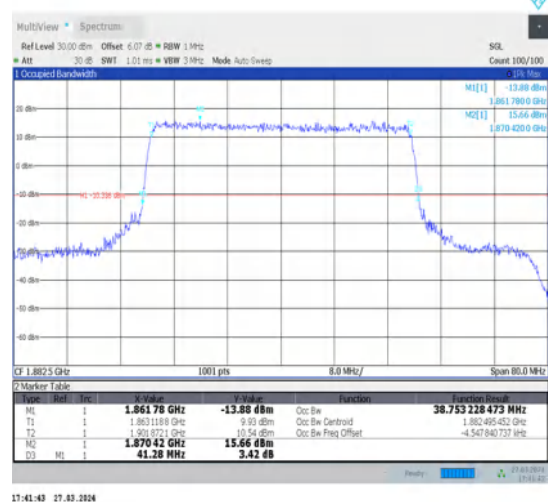
1-N25-15-40-M-6-CP-QPSK-Outet_Full-216@0-Ant1-38.753-41.280-≤40-PASS
