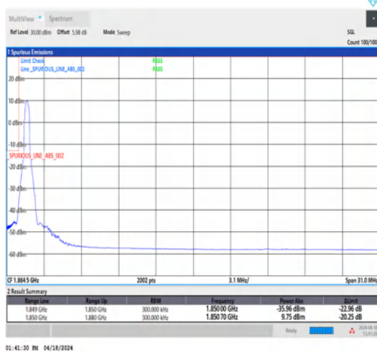
1-N25-15-30-L-4-CP-QPSK-Edge_1RB_Left-1@0-Ant1-1-seegraph-PASS-see graph
