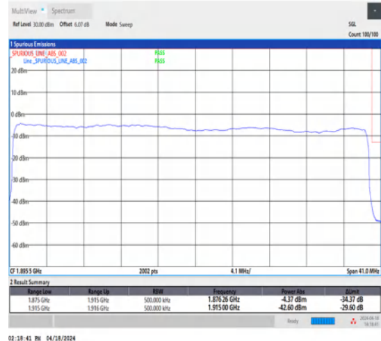
1-N25-15-40-H-3-DFT-PI2BPSK-Outer_Full-216@0-Ant1-1-seegraph-PASS-see graph
