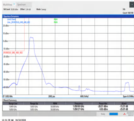
1-N25-15-5-L-1-DFT-PI2BPSK-Edge_1RB_Left-1@0-Ant1-1-seegraph-PASS-see graph
