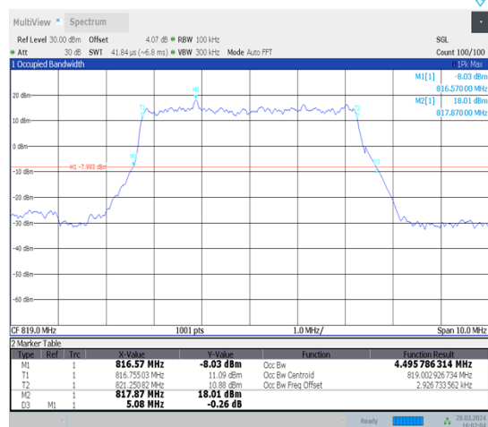
1-N26-814-824-15-5-M-2-DFT-PI2BPSK-Outer_Full-25@0-Ant1-4.496-5.080-≤5-PASS
