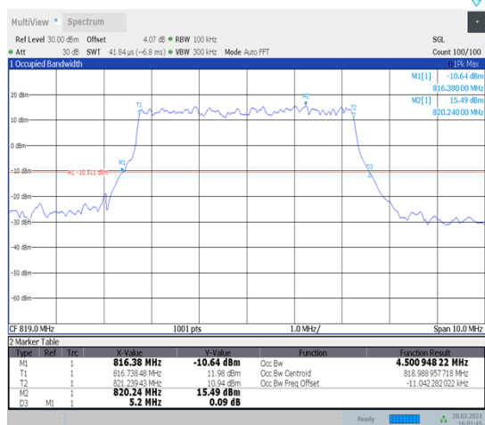
1-N26-814-824-15-5-M-1-DFT-QPSK-Outer_Full-25@0-Ant1-4.501-5.200-≤5-PASS
