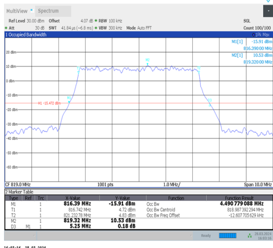
1-N26-814-824-15-5-M-9-CP-256QAM-Outer_Full-25@0-Ant1-4.491-5.250-≤5-PASS
