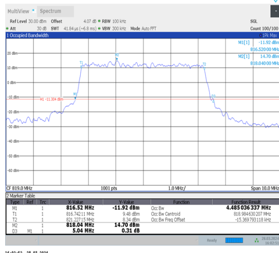
1-N26-814-824-15-5-M-6-CP-QPSK-Outer_Full-25@0-Ant1-4.485-5.040-≤5-PASS
