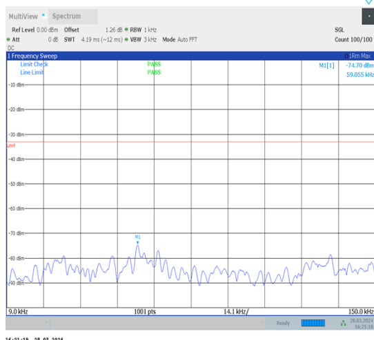
1-N26-814-824-15-10-M-1-DFT-PI2BPSK- Inner_1RB_Left-1@1-0.009-0.15-Ant1-0.06--74.70-- 33-PASS
