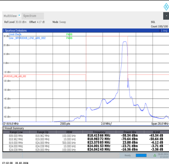
1-N26-814-824-15-5-H-2-DFT-PI2BPSK-Edge_1RB_Right-1@24-Ant1-1--PASS-see graph
