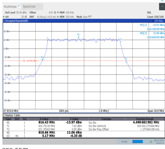
1-N26-814-824-15-5-M-5-DFT-256QAM-Outer_Full-25@0-Ant1-4.499-5.170-≤5-PASS
