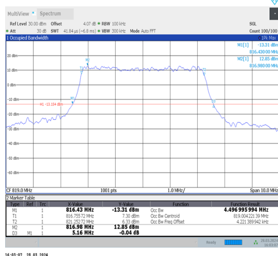
1-N26-814-824-15-5-M-8-CP-64QAM-Outer_Full-25@0-Ant1-4.497-5.160-≤5-PASS
