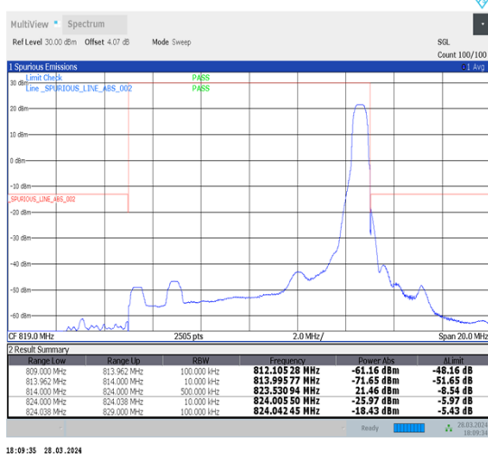
1-N26-814-824-15-10-H-5-CP-QPSK-Edge_1RB_Right-1@51-Ant1-1--PASS-see graph
