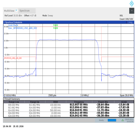
1-N26-814-824-15-10-H-3-DFT-PI2BPSK-Outer_Full-50@0-Ant1-1--PASS-see graph
