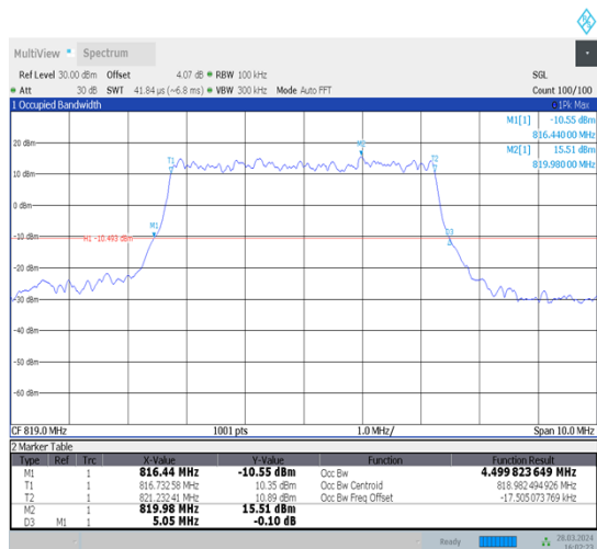
1-N26-814-824-15-5-M-1-DFT-QPSK-Outer_Full-25@0-Ant1-4.501-5.200-≤5-PASS
