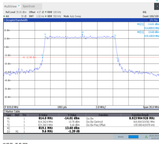
1-N26-814-824-15-10-M-1-DFT-QPSK-Outer_Full-50@0-Ant1-8.924-9.600-≤10-PASS
