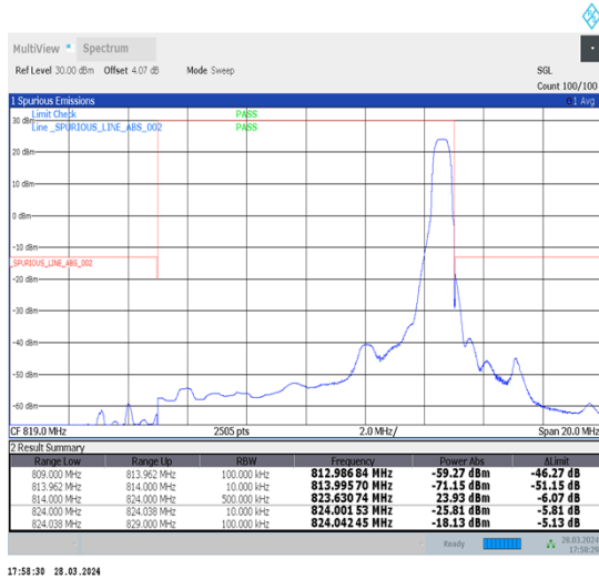
1-N26-814-824-15-10-H-2-DFT-PI2BPSK-Edge_1RB_Right-1@51-Ant1-1--PASS-see graph
