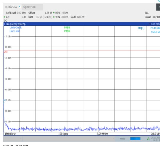
1-N26-814-824-15-10-M-1-DFT-PI2BPSK- Inner_1RB_Left-1@1-0.15-30-Ant1-0.15--73.40--23- PASS
