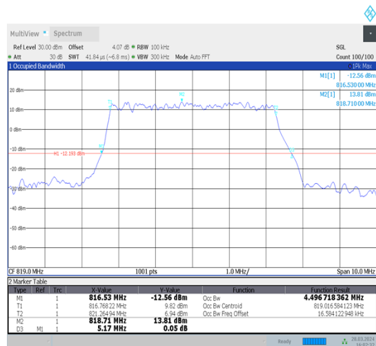
1-N26-814-824-15-5-M-2-DFT-PI2BPSK-Outer_Full-25@0-Ant1-4.496-5.080-≤5-PASS
