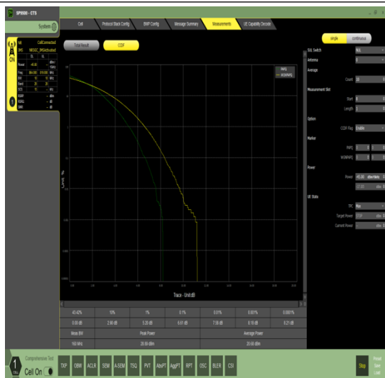
1-N26-814-824-15-10-L-14-DFT-256QAM-Outer_Full-50@0-20.61-20.61-19~27.5-PASS
