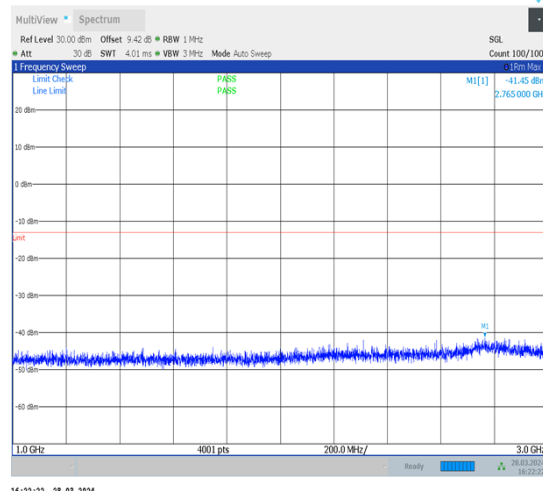
1-N26-814-824-15-10-M-1-DFT-PI2BPSK- Inner_1RB_Left-1@1-1000-3000-Ant1-2765.00-- 41.45--13-PASS
