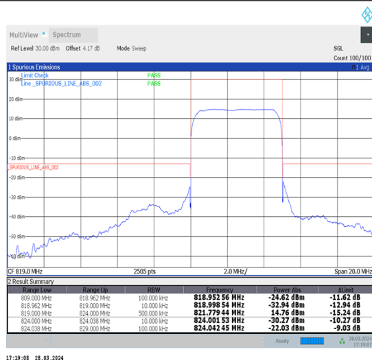
1-N26-814-824-15-5-H-3-DFT-PI2BPSK-Outer_Full-25@0-Ant1-1--PASS-see graph
