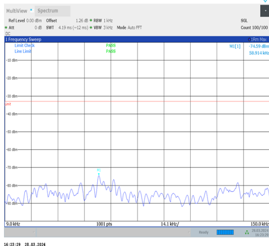
1-N26-814-824-15-10-H-1-DFT-PI2BPSK- Inner_1RB_Left-1@1-0.009-0.15-Ant1-0.06--74.59-- 33-PASS
