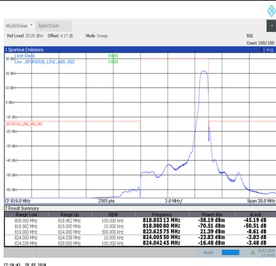
1-N26-814-824-15-5-H-5-CP-QPSK-Edge_1RB_Right-1@24-Ant1-1--PASS-see graph
