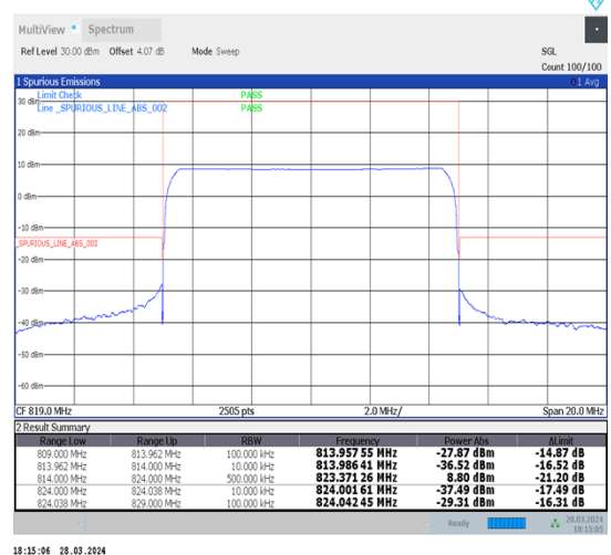
1-N26-814-824-15-10-H-6-CP-QPSK-Outer_Full-52@0-Ant1-1--PASS-see graph
