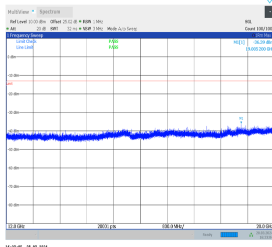
1-N26-814-824-15-10-M-1-DFT-PI2BPSK- Inner_1RB_Left-1@1-12000-20000-Ant1-19005.20-- 36.39--13-PASS
