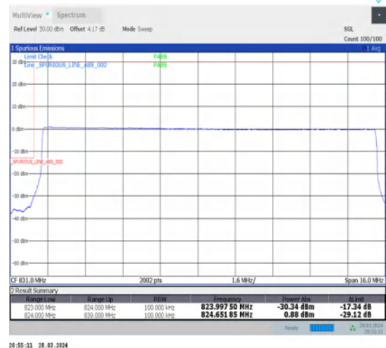
1-N26-824-849-15-15-L-6-CP-QPSK-Outer_Full-79@0-Ant1-1-seegraph-PASS-see graph
