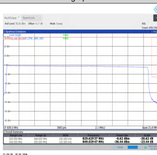
1-N26-824-849-15-20-H-3-DFT-PI2BPSK-Outer_Full-100@0-Ant1-1-seegraph-PASS-see graph
