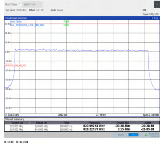
1-N26-824-849-15-20-L-3-DFT-PI2BPSK-Outer_Full-100@0-Ant1-1-seegraph-PASS-see graph
