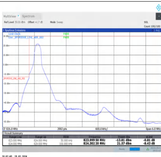
1-N26-824-849-15-5-L-1-DFT-PI2BPSK-Edge_1RB_Left-1@0-Ant1-1-seegraph-PASS-see graph
