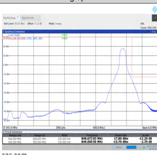
1-N26-824-849-15-5-H-5-CP-QPSK-Edge_1RB_Right-1@24-Ant1-1-seegraph-PASS-see graph
