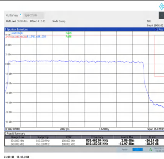
1-N26-824-849-15-15-H-3-DFT-PI2BPSK-Outer_Full-75@0-Ant1-1-seegraph-PASS-see graph
