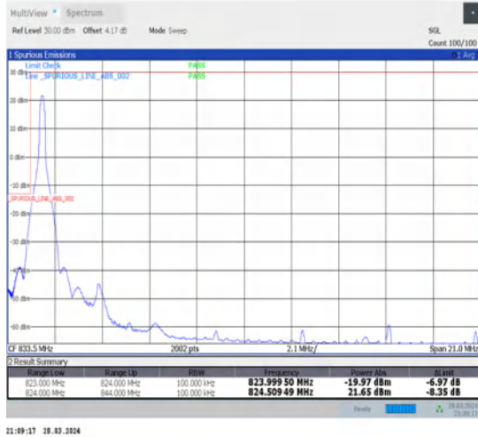
1-N26-824-849-15-20-L-1-DFT-PI2BPSK-Edge_1RB_Left-1@0-Ant1-1-seegraph-PASS-see graph
