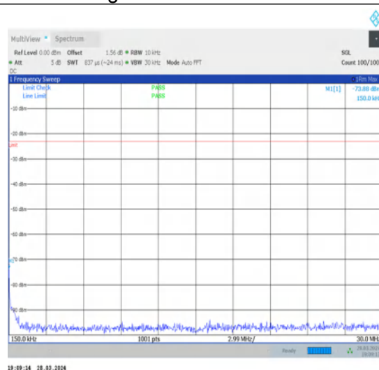
1-N26-824-849-15-20-H-1-DFT-PI2BPSK- Inner_1RB_Left-1@1-0.15-30-Ant1-0.15--73.88--23- PASS
