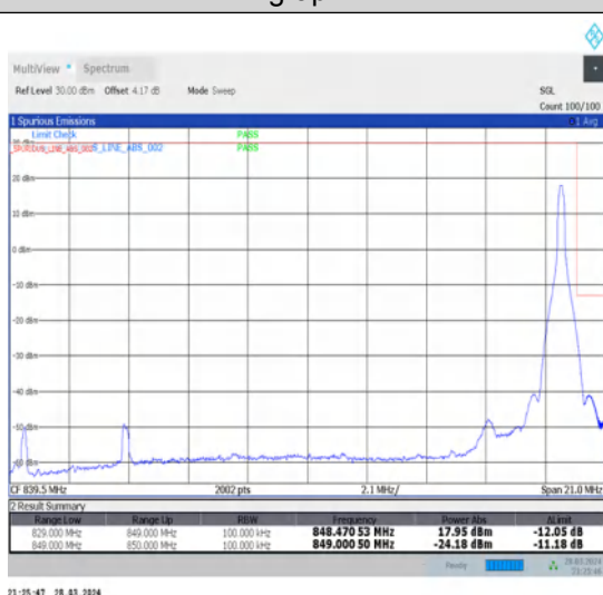
1-N26-824-849-15-20-H-5-CP-QPSK-Edge_1RB_Right-1@105-Ant1-1-seegraph-PASS-see graph
