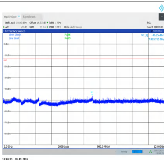
1-N26-824-849-15-20-L-1-DFT-PI2BPSK- Inner_1RB_Left-1@1-3000-12000-Ant1-7965.75-- 46.25--13-PASS
