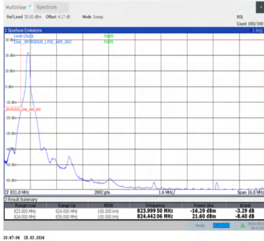
1-N26-824-849-15-15-L-1-DFT-PI2BPSK-Edge_1RB_Left-1@0-Ant1-1-seegraph-PASS-see graph
