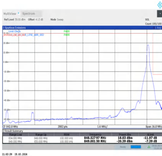
1-N26-824-849-15-15-H-5-CP-QPSK-Edge_1RB_Right-1@78-Ant1-1-seegraph-PASS-see graph
