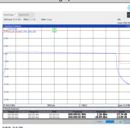
1-N26-824-849-15-10-H-3-DFT-PI2BPSK-Outer_Full-50@0-Ant1-1-seegraph-PASS-see graph
