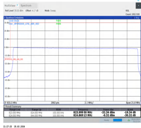
1-N26-824-849-15-20-L-6-CP-QPSK-Outer_Full-106@0-Ant1-1-seegraph-PASS-see graph
