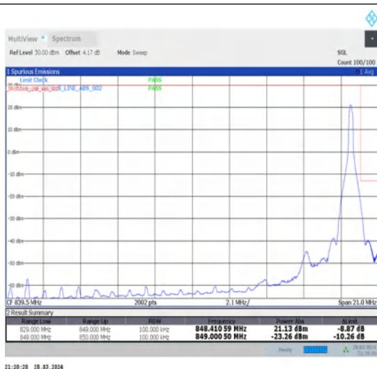
1-N26-824-849-15-20-H-2-DFT-PI2BPSK-Edge_1RB_Right-1@105-Ant1-1-seegraph-PASS-see graph
