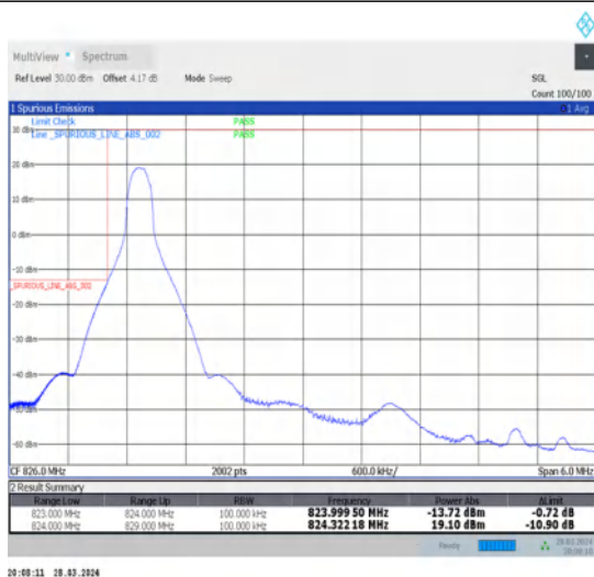
1-N26-824-849-15-5-L-4-CP-QPSK-Edge_1RB_Left-1@0-Ant1-1-seegraph-PASS-see graph
