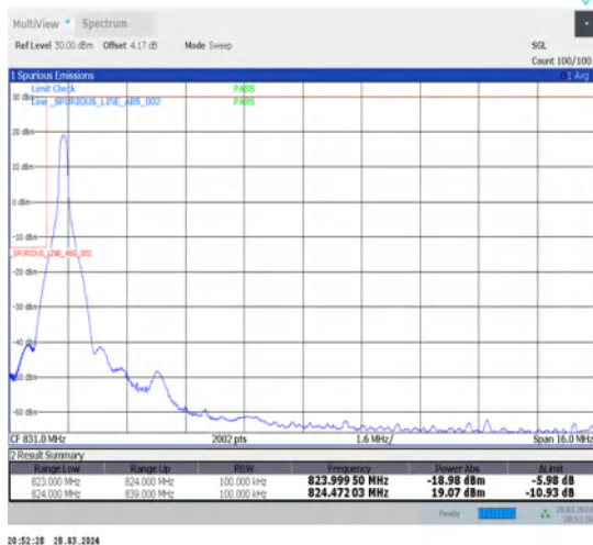
1-N26-824-849-15-15-L-4-CP-QPSK-Edge_1RB_Left-1@0-Ant1-1-seegraph-PASS-see graph
