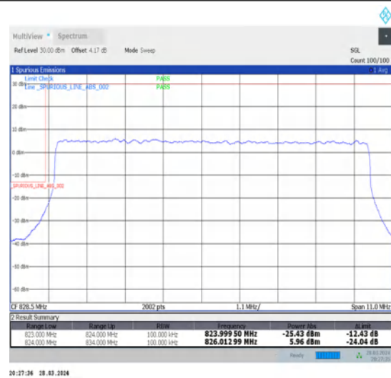
1-N26-824-849-15-10-L-3-DFT-PI2BPSK-Outer_Full-50@0-Ant1-1-seegraph-PASS-see graph
