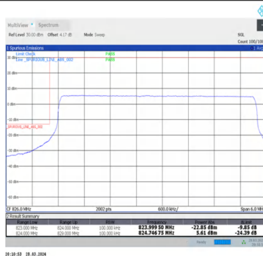
1-N26-824-849-15-5-L-6-CP-QPSK-Outer_Full-25@0-Ant1-1-seegraph-PASS-see graph
