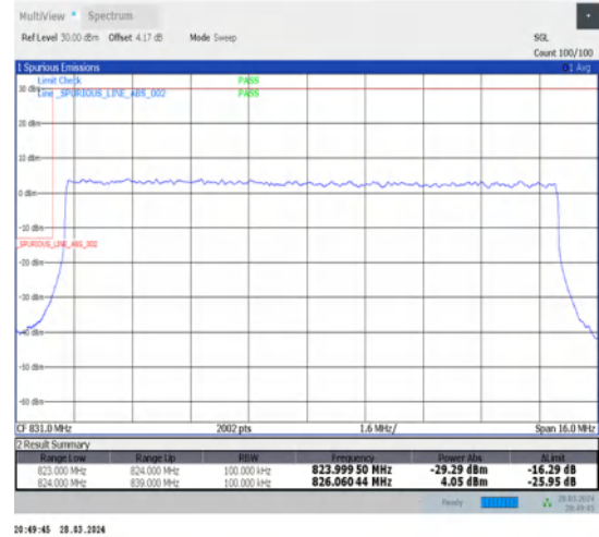
1-N26-824-849-15-15-L-3-DFT-PI2BPSK-Outer_Full-75@0-Ant1-1-seegraph-PASS-see graph
