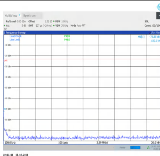
1-N26-824-849-15-20-M-1-DFT-PI2BPSK- Inner_1RB_Left-1@1-0.15-30-Ant1-0.15--73.35--23- PASS
