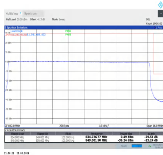
1-N26-824-849-15-15-H-3-DFT-PI2BPSK-Outer_Full-75@0-Ant1-1-seegraph-PASS-see graph
