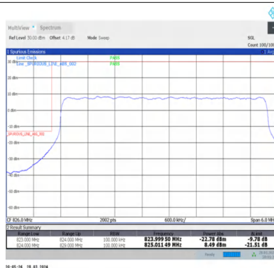
1-N26-824-849-15-5-L-3-DFT-PI2BPSK-Outer_Full-25@0-Ant1-1-seegraph-PASS-see graph
