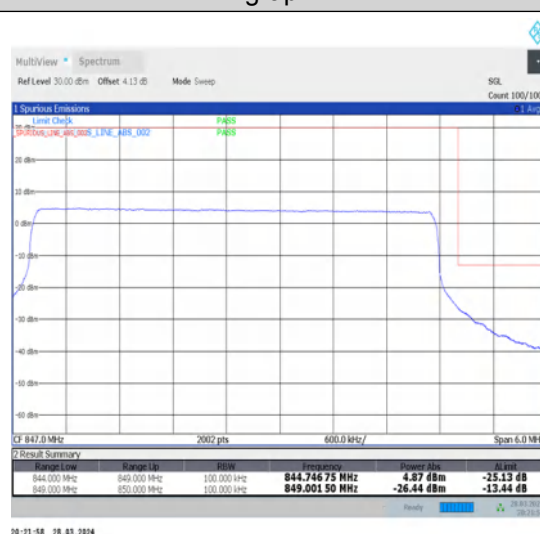
1-N26-824-849-15-5-H-6-CP-QPSK-Outer_Full-25@0-Ant1-1-seegraph-PASS-see graph
