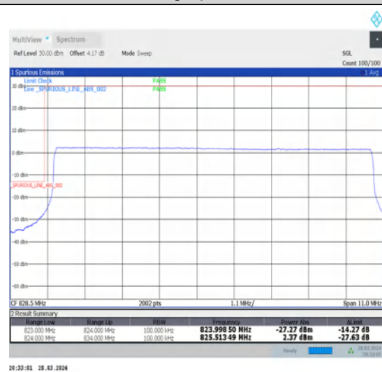
1-N26-824-849-15-10-L-6-CP-QPSK-Outer_Full-52@0-Ant1-1-seegraph-PASS-see graph
