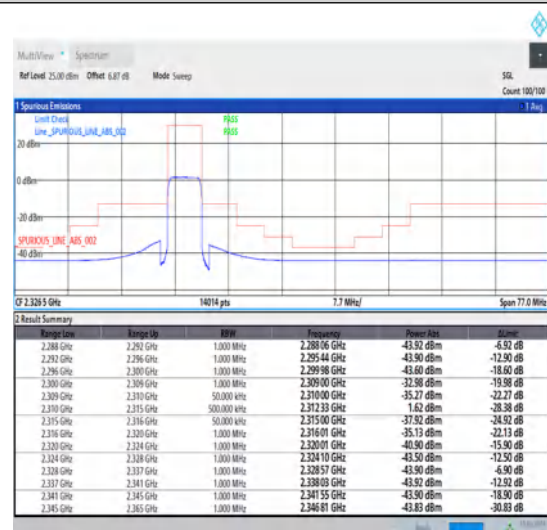
1-N30-15-5-H-6-CP-QPSK-Outer_Full-25@0-Ant1-1--PASS-see graph
