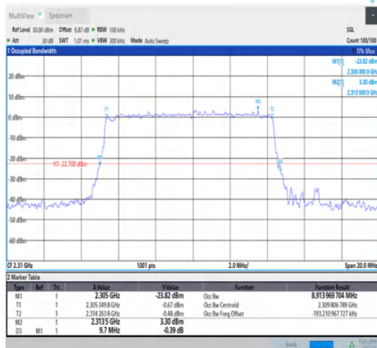
1-N30-15-10-M-1-DFT-QPSK-Outer_Full-50@0- Ant1-8.914-9.700-≤10-PASS
