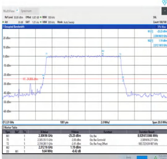
1-N30-15-10-M-4-DFT-64QAM-Outer_Full-50@0- Ant1-8.93-9.640-≤10-PASS
