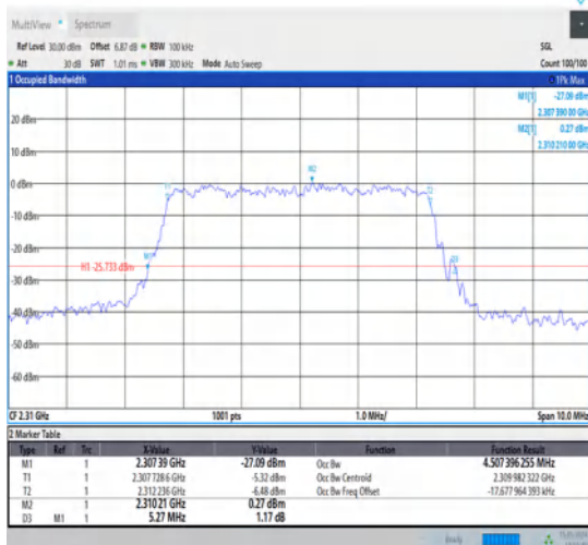
1-N30-15-5-M-9-CP-256QAM-Outer_Full-25@0- Ant1-4.507-5.270-≤5-PASS
