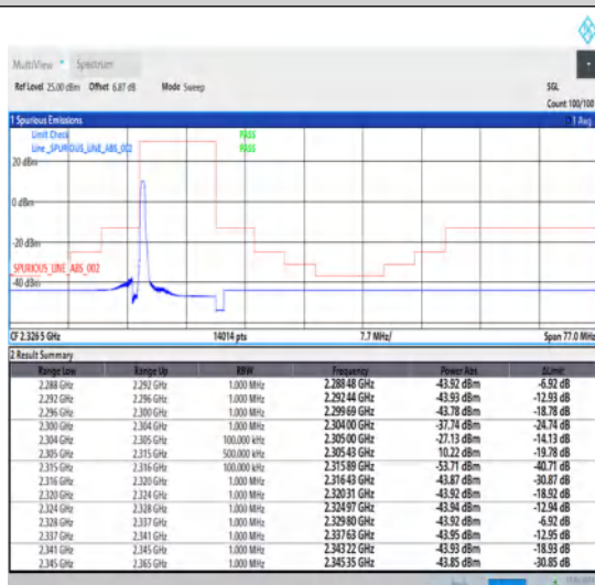
1-N30-15-10-L-4-CP-QPSK-Edge_1RB_Left-1@0-Ant1-1--PASS-see graph
