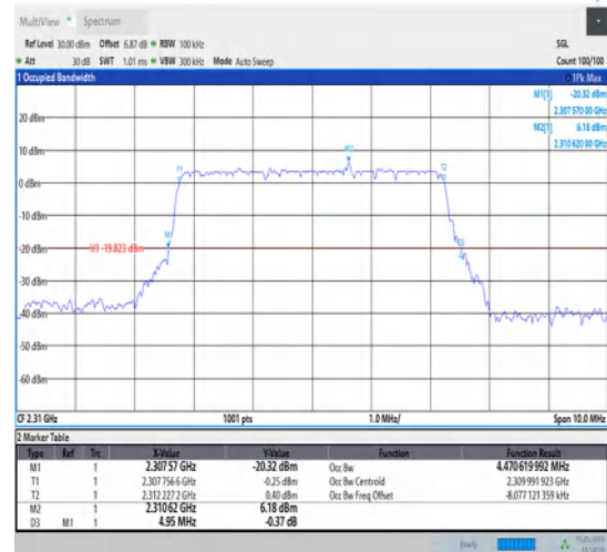
1-N30-15-5-M-4-DFT-64QAM-Outer_Full-25@0-Ant1-4.471-4.950-≤5-PASS
