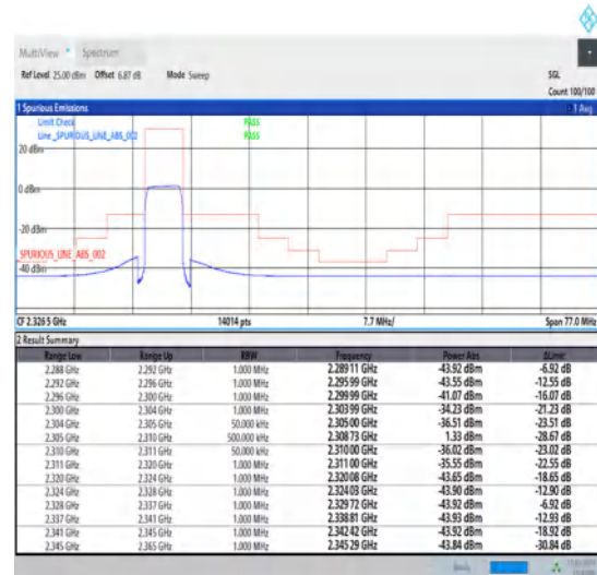
1-N30-15-5-L-6-CP-QPSK-Outer_Full-25@0-Ant1-1--PASS-see graph
