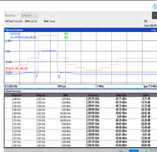
1-N30-15-10-H-3-DFT-PI2BPSK-Outer_Full-50@0-Ant1-1--PASS-see graph
