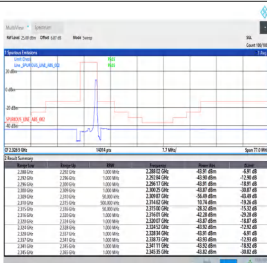
1-N30-15-5-H-5-CP-QPSK-Edge_1RB_Right-1@24-Ant1-1--PASS-see graph
