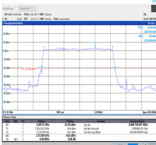
1-N30-15-10-M-2-DFT-PI2BPSK-Outer_Full-50@0- Ant1-8.907-9.480-≤10-PASS
