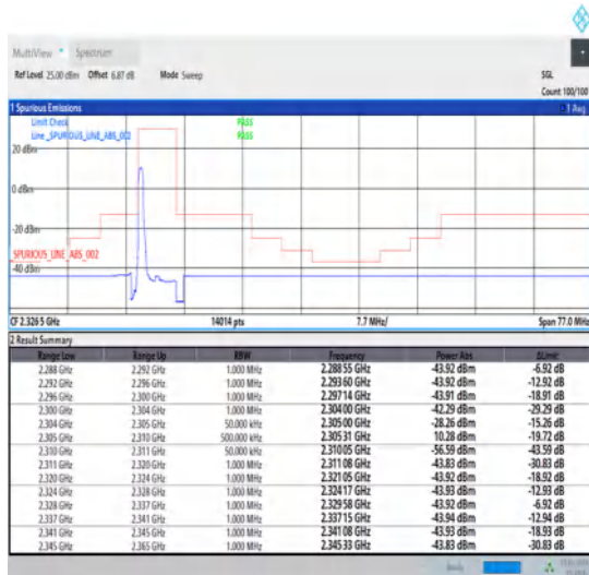
1-N30-15-5-L-4-CP-QPSK-Edge_1RB_Left-1@0-Ant1-1--PASS-see graph
