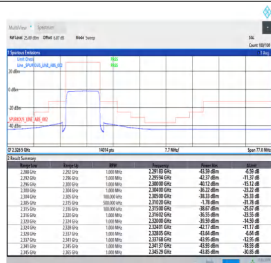
1-N30-15-10-H-6-CP-QPSK-Outer_Full-52@0-Ant1-1--PASS-see graph
