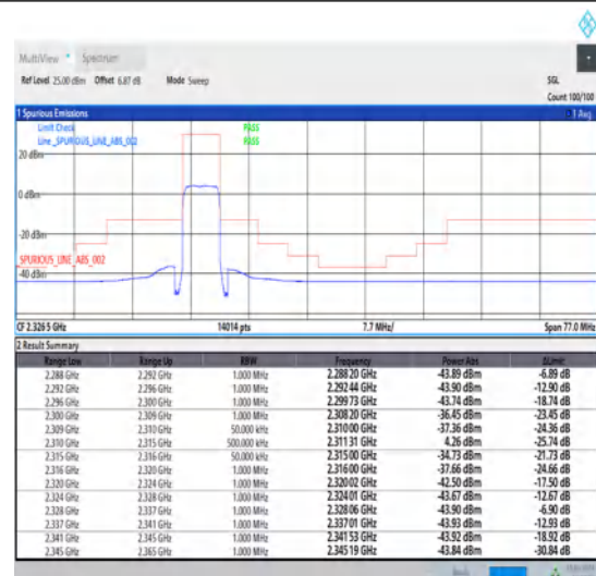
1-N30-15-5-H-3-DFT-PI2BPSK-Outer_Full-25@0-Ant1-1--PASS-see graph
