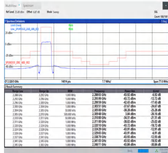
1-N30-15-5-L-3-DFT-PI2BPSK-Outer_Full-25@0-Ant1-1--PASS-see graph
