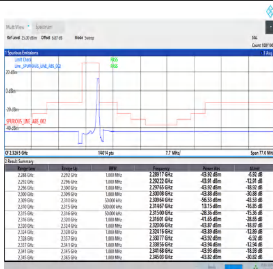
1-N30-15-5-H-2-DFT-PI2BPSK-Edge_1RB_Right-1@24-Ant1-1--PASS-see graph
