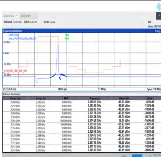
1-N30-15-10-H-2-DFT-PI2BPSK-Edge_1RB_Right-1@51-Ant1-1--PASS-see graph
