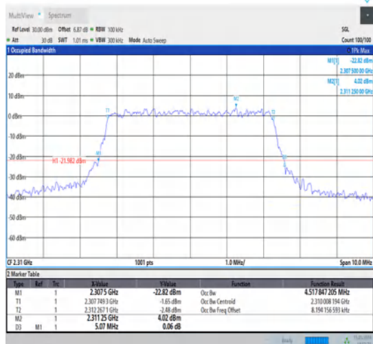
1-N30-15-5-M-6-CP-QPSK-Outer_Full-25@0-Ant1-4.518-5.070-≤5-PASS
