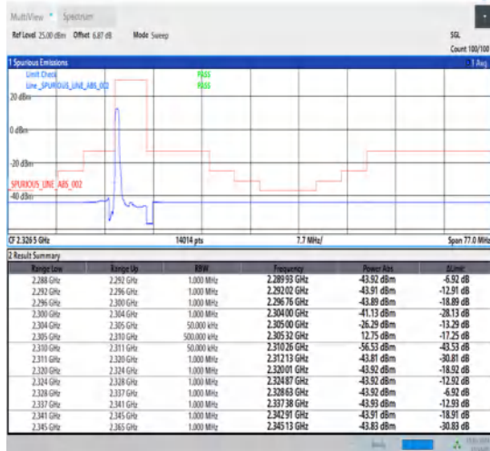
1-N30-15-5-L-1-DFT-PI2BPSK-Edge_1RB_Left-1@0-Ant1-1--PASS-see graph
