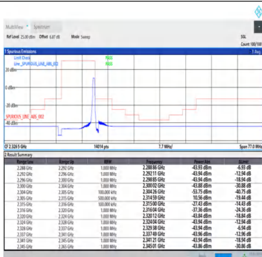
1-N30-15-10-H-5-CP-QPSK-Edge_1RB_Right-1@51-Ant1-1--PASS-see graph
