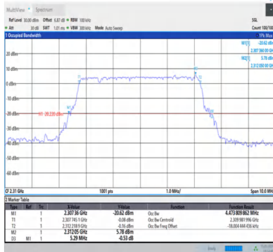
1-N30-15-5-M-3-DFT-16QAM-Outer_Full-25@0-Ant1-4.474-5.290-≤5-PASS
