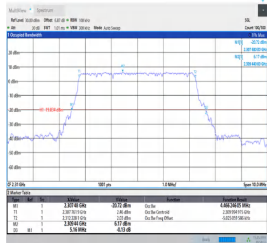
1-N30-15-5-M-2-DFT-PI2BPSK-Outer_Full-25@0-Ant1-4.466-5.160-≤5-PASS
