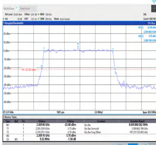
1-N30-15-10-M-3-DFT-16QAM-Outer_Full-50@0- Ant1-8.946-9.520-≤10-PASS
