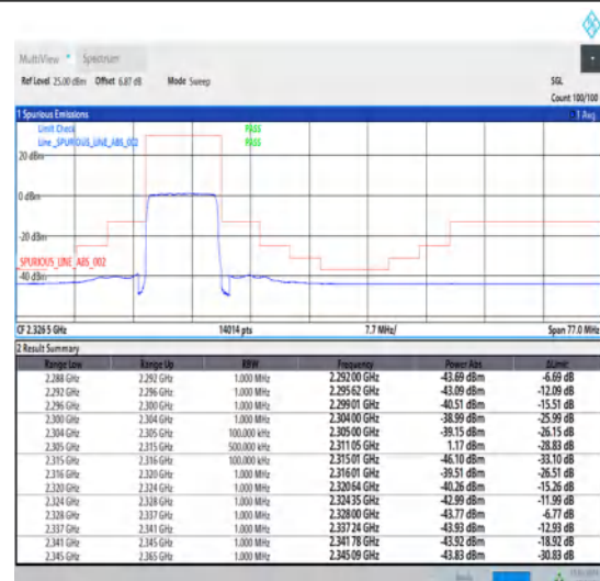
1-N30-15-10-L-3-DFT-PI2BPSK-Outer_Full-50@0-Ant1-1--PASS-see graph
