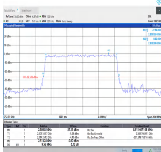
1-N30-15-10-M-5-DFT-256QAM-Outer_Full-50@0- Ant1-8.911-9.560-≤10-PASS
