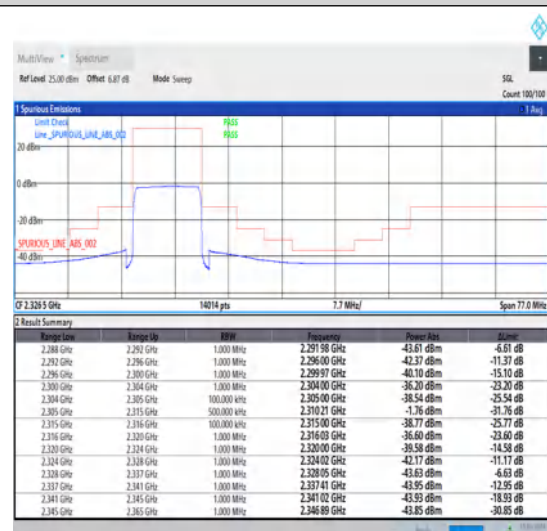
1-N30-15-10-L-6-CP-QPSK-Outer_Full-52@0-Ant1-1--PASS-see graph
