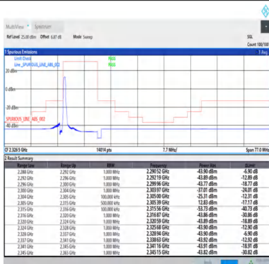
1-N30-15-10-L-1-DFT-PI2BPSK-Edge_1RB_Left-1@0-Ant1-1--PASS-see graph
