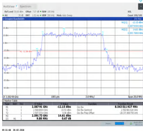
1-N41-30-10-M-2-DFT-PI2BPSK-Outter_Full-24@0- Ant1-8.544-9.880-≤10-PASS
