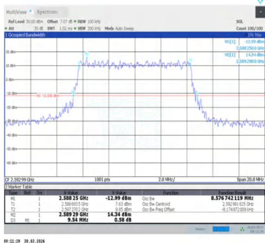
1-N41-30-10-M-1-DFT-QPSK-Outter_Full-24@0- Ant1-8.577-9.540-≤10-PASS
