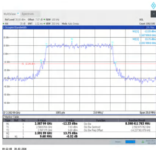
1-N41-30-10-M-4-DFT-64QAM-Outter_Full-24@0- Ant1-8.598-9.680-≤10-PASS
