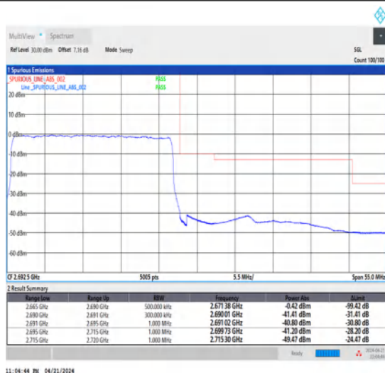
1-N41-30-25-H-3-DFT-PI2BPSK-Outer_Full-64@0-Ant1-1--PASS-see graph
