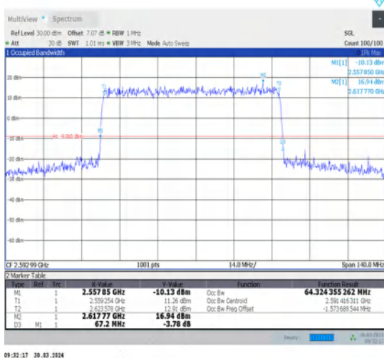
1-N41-30-70-M-3-DFT-16QAM-Outter_Full-180@0-Ant1-64.324-67.200-≤70-PASS
