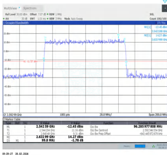
1-N41-30-100-M-4-DFT-64QAM-Outer_Full-270@0-Ant1-96.286-99.800-≤100-PASS
