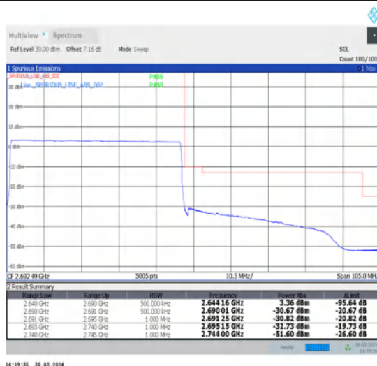
1-N41-30-50-H-6-CP-QPSK-Outer_Full-133@0-Ant1-1--PASS-see graph
