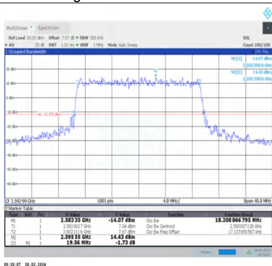
1-N41-30-20-M-8-CP-64QAM-Outer_Full-51@0- Ant1-18.209-19.560-≤20-PASS
