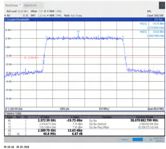
1-N41-30-40-M-9-CP-256QAM-Outer_Full-106@0-Ant1-38.071-40.800-≤40-PASS
