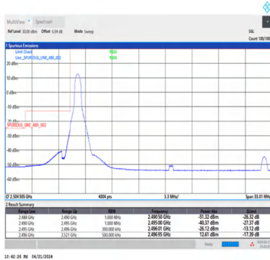
1-N41-30-25-L-1-DFT-PI2BPSK-Edge_1RB_Left-1@0-Ant1-1--PASS-see graph
