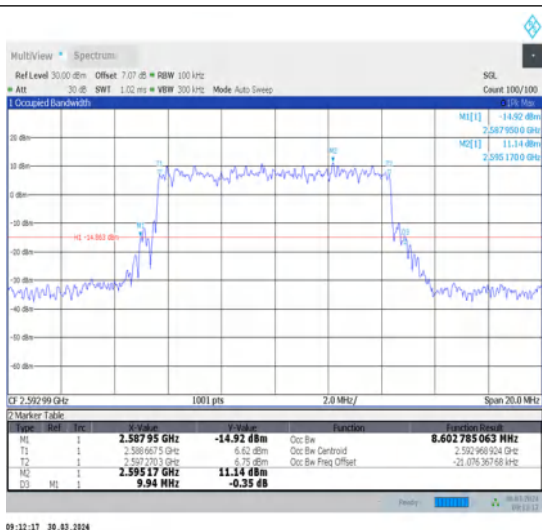
1-N41-30-10-M-5-DFT-256QAM-Outer_Full-24@0-Ant1-8.603-9.940-≤10-PASS
