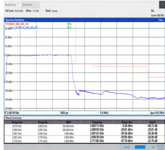
1-N41-30-20-H-3-DFT-PI2BPSK-Outer_Full-50@0-Ant1-1--PASS-see graph
