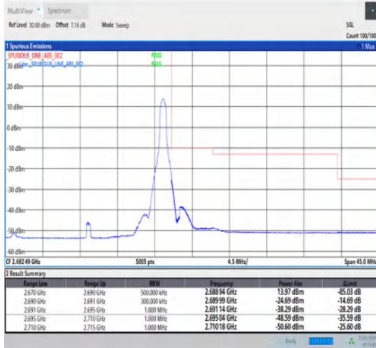
1-N41-30-20-H-2-DFT-PI2BPSK-Edge_1RB_Right-1@50-Ant1-1--PASS-see graph
