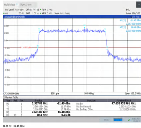
1-N41-30-50-M-8-CP-64QAM-Outer_Full-133@0-Ant1-47.656-50.300-≤50-PASS
