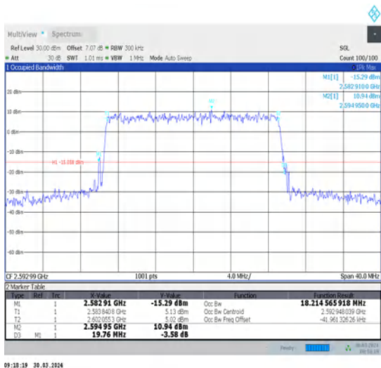
1-N41-30-20-M-9-CP-256QAM-Outer_Full-51@0- Ant1-18.215-19.760-≤20-PASS
