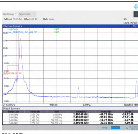
1-N41-30-60-L-1-DFT-PI2BPSK-Edge_1RB_Left-1@0-Ant1-1--PASS-see graph
