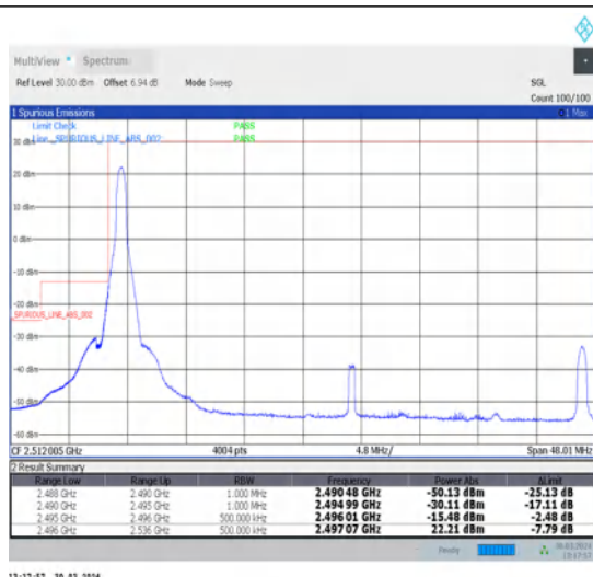
1-N41-30-40-L-1-DFT-PI2BPSK-Edge_1RB_Left-1@0-Ant1-1--PASS-see graph
