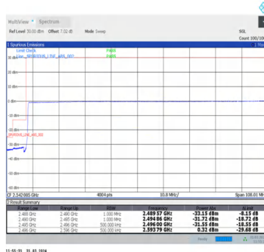
1-N41-30-100-L-6-CP-QPSK-Outer_Full-273@0-Ant1-1--PASS-see graph
