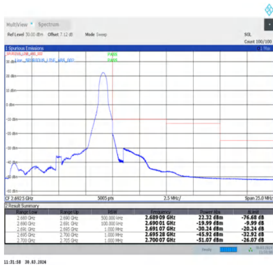
1-N41-30-10-H-5-CP-QPSK-Edge_1RB_Right-1@23-Ant1-1--PASS-see graph
