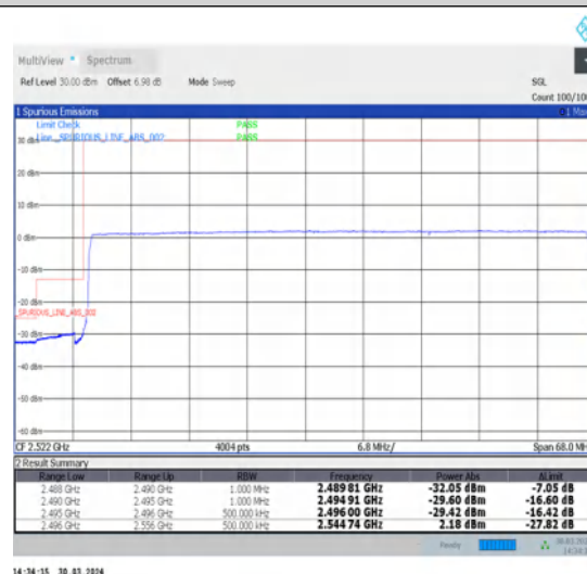
1-N41-30-60-L-6-CP-QPSK-Outer_Full-162@0-Ant1-1--PASS-see graph
