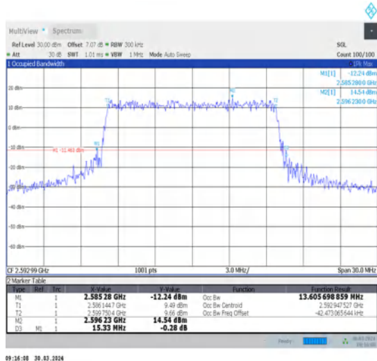
1-N41-30-15-M-7-CP-16QAM-Outer_Full-38@0-Ant1-13.606-15.330-≤15-PASS
