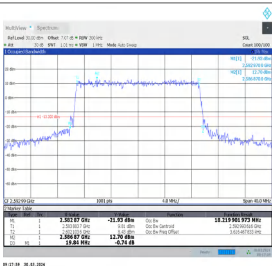
1-N41-30-20-M-7-CP-16QAM-Outer_Full-51@0- Ant1-18.22-19.840-≤20-PASS
