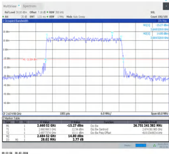
1-N41-30-30-H-1-DFT-QPSK-Outer_Full-75@0-Ant1-26.752-28.020-≤30-PASS
