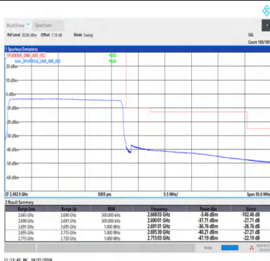
1-N41-30-25-H-6-CP-QPSK-Outer_Full-65@0-Ant1-1--PASS-see graph
