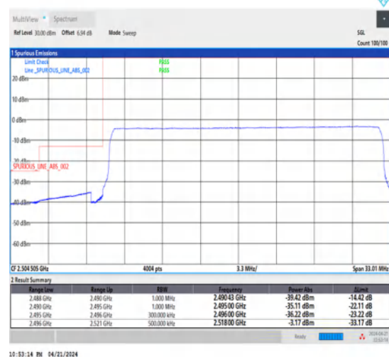
1-N41-30-25-L-6-CP-QPSK-Outer_Full-65@0-Ant1-1--PASS-see graph
