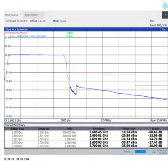
1-N41-30-10-H-6-CP-QPSK-Outer_Full-24@0-Ant1-1--PASS-see graph
