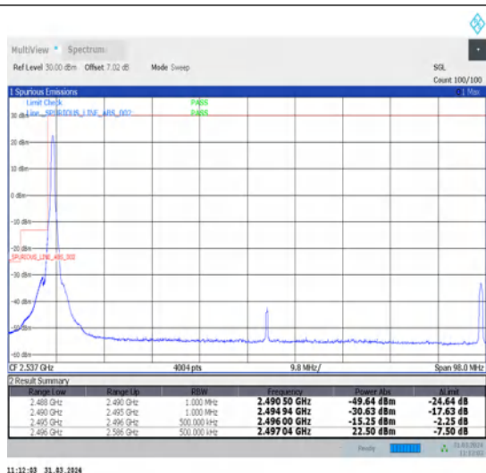
1-N41-30-90-L-1-DFT-PI2BPSK-Edge_1RB_Left-1@0-Ant1-1--PASS-see graph
