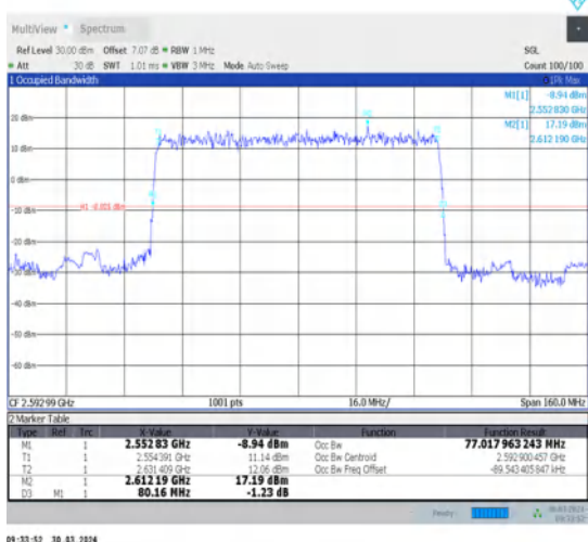
1-N41-30-80-M-2-DFT-PI2BPSK-Outer_Full-216@0-Ant1-77.018-80.160-≤80-PASS
