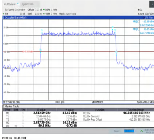
1-N41-30-100-M-2-DFT-PI2BPSK-Outer_Full-270@0-Ant1-96.345-99.800-≤100-PASS
