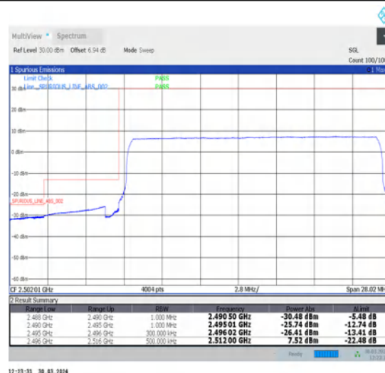
1-N41-30-20-L-6-CP-QPSK-Outer_Full-51@0-Ant1-1--PASS-see graph
