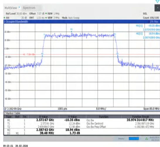
1-N41-30-40-M-3-DFT-16QAM-Outer_Full-100@0- Ant1-35.974-38.480-≤40-PASS
