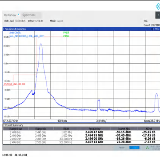
1-N41-30-30-L-1-DFT-PI2BPSK-Edge_1RB_Left-1@0-Ant1-1--PASS-see graph
