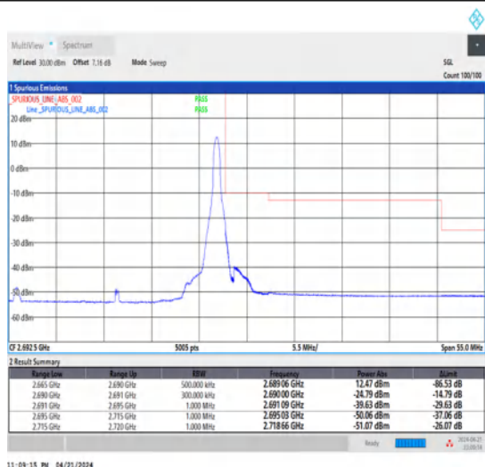
1-N41-30-25-H-5-CP-QPSK-Edge_1RB_Right-1@64-Ant1-1--PASS-see graph
