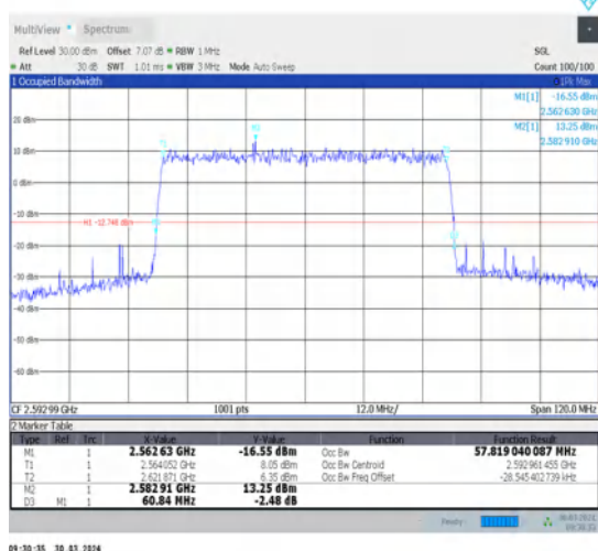
1-N41-30-60-M-9-CP-256QAM-Outer_Full-162@0-Ant1-57.819-60.840-≤60-PASS
