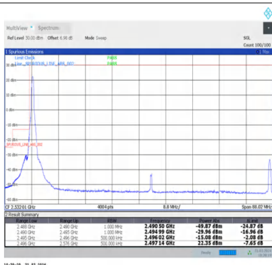
1-N41-30-80-L-1-DFT-PI2BPSK-Edge_1RB_Left-1@0-Ant1-1--PASS-see graph
