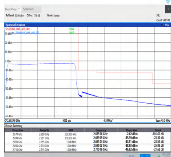
1-N41-30-20-H-6-CP-QPSK-Outer_Full-51@0-Ant1-1--PASS-see graph
