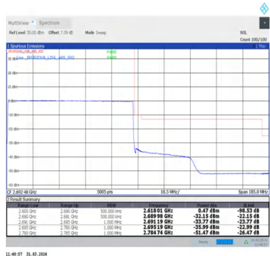
1-N41-30-90-H-6-CP-QPSK-Outer_Full-245@0-Ant1-1--PASS-see graph
