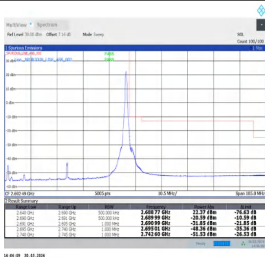
1-N41-30-50-H-2-DFT-PI2BPSK-Edge_1RB_Right-1@132-Ant1-1--PASS-see graph
