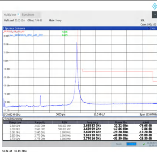
1-N41-30-80-H-2-DFT-PI2BPSK-Edge_1RB_Right-1@216-Ant1-1--PASS-see graph
