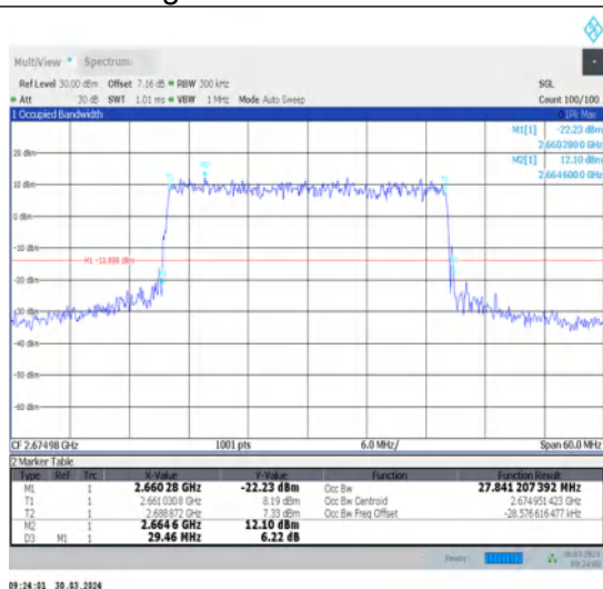
1-N41-30-30-H-6-CP-QPSK-Outer_Full-78@0-Ant1-27.843-29.460-≤30-PASS
