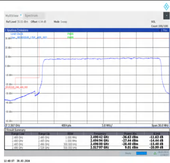
1-N41-30-30-L-3-DFT-PI2BPSK-Outer_Full-75@0-Ant1-1--PASS-see graph
