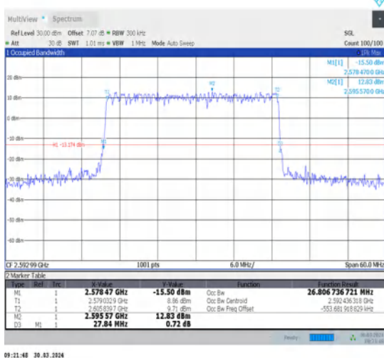
1-N41-30-30-M-4-DFT-64QAM-Outer_Full-75@0-Ant1-26.808-27.840-≤30-PASS
