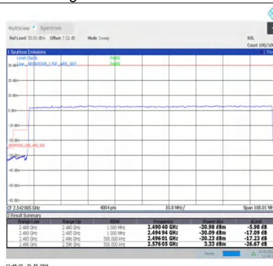
1-N41-30-100-L-3-DFT-PI2BPSK-Outer_Full-270@0-Ant1-1--PASS-see graph
