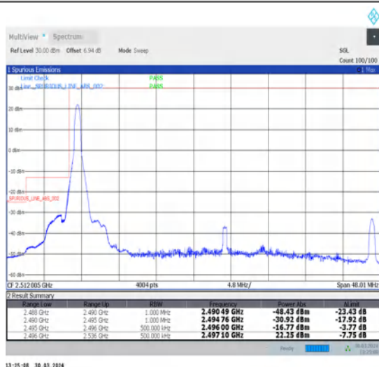
1-N41-30-40-L-4-CP-QPSK-Edge_1RB_Left-1@0-Ant1-1--PASS-see graph
