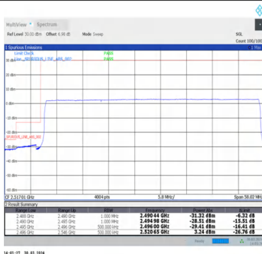
1-N41-30-50-L-6-CP-QPSK-Outer_Full-133@0-Ant1-1--PASS-see graph
