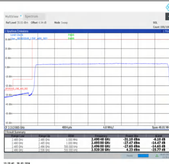
1-N41-30-40-L-6-CP-QPSK-Outer_Full-106@0-Ant1-1--PASS-see graph
