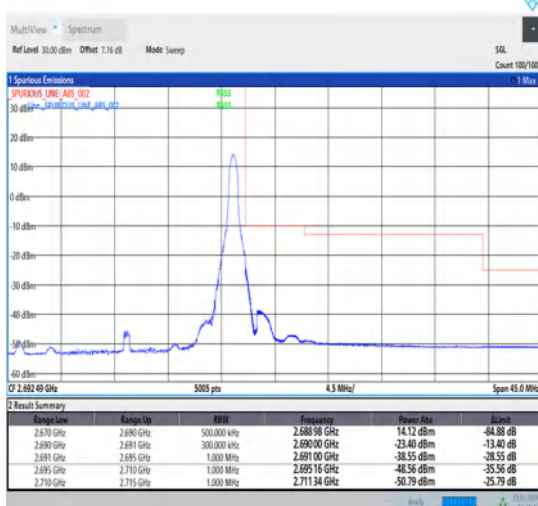
1-N41-30-20-H-5-CP-QPSK-Edge_1RB_Right-1@50-Ant1-1--PASS-see graph
