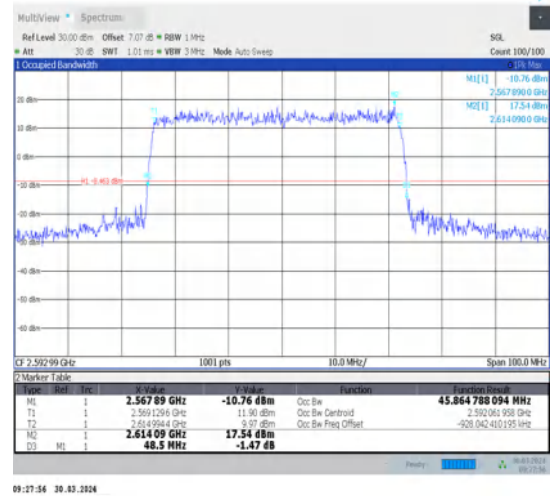
1-N41-30-50-M-4-DFT-64QAM-Outer_Full-128@0-Ant1-45.865-48.500-≤50-PASS
