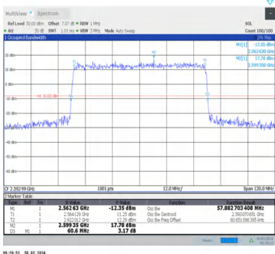
1-N41-30-60-M-4-DFT-64QAM-Outer_Full-162@0-Ant1-57.883-60.600-≤60-PASS
