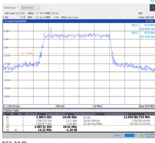
1-N41-30-15-M-3-DFT-16QAM-Outer_Full-36@0-Ant1-12.939-14.220-≤15-PASS
