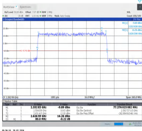
1-N41-30-80-M-3-DFT-16QAM-Outer_Full-216@0-Ant1-77.376-80.000-≤80-PASS
