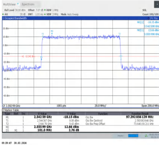
1-N41-30-100-M-6-CP-QPSK-Outer_Full-273@0-Ant1-97.393-101.000-≤100-PASS
