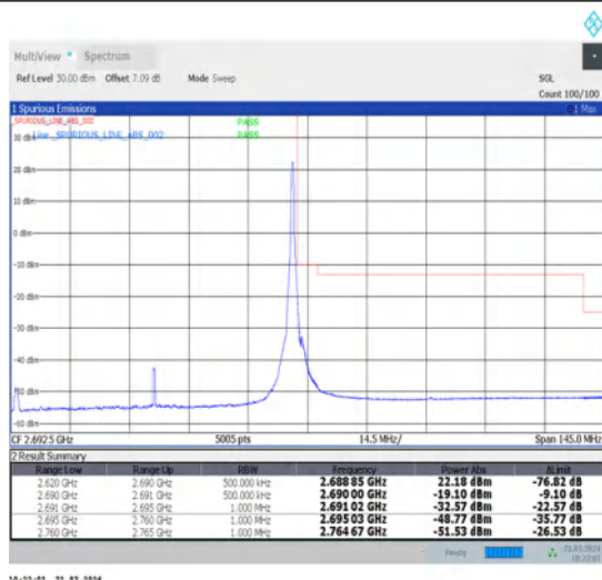
1-N41-30-70-H-2-DFT-PI2BPSK-Edge_1RB_Right-1@188-Ant1-1--PASS-see graph
