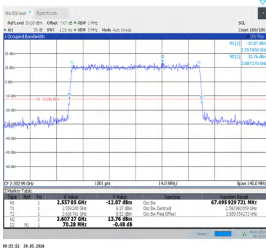
1-N41-30-70-M-7-CP-16QAM-Outer_Full-189@0-Ant1-67.496-70.280-≤70-PASS
