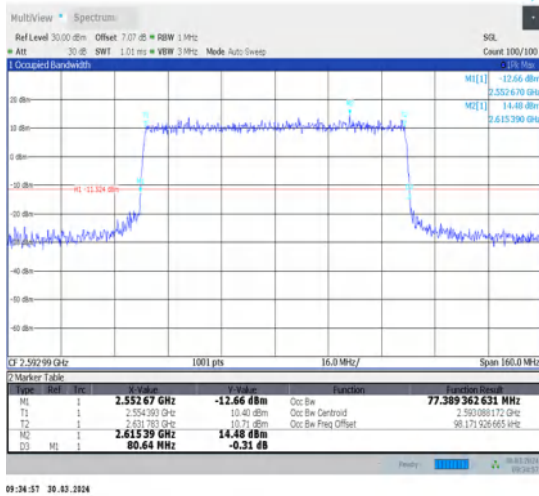
1-N41-30-80-M-8-CP-64QAM-Outer_Full-217@0-Ant1-77.389-80.640-≤80-PASS
