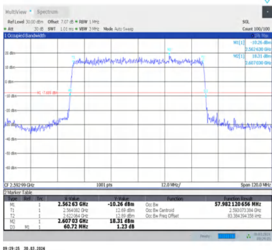
1-N41-30-60-M-2-DFT-PI2BPSK-Outer_Full-162@0-Ant1-57.982-60.720-≤60-PASS
