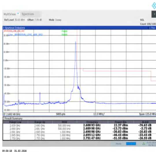
1-N41-30-60-H-5-CP-QPSK-Edge_1RB_Right-1@161-Ant1-1--PASS-see graph
