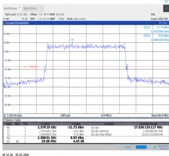
1-N41-30-30-M-9-CP-256QAM-Outer_Full-78@0-Ant1-27.838-29.580-≤30-PASS
