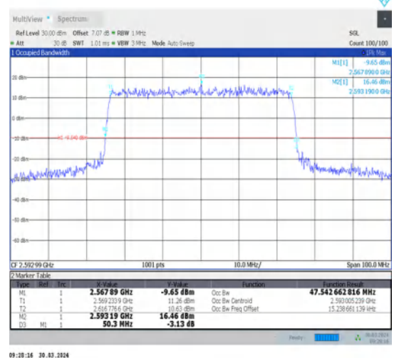
1-N41-30-50-M-6-CP-QPSK-Outer_Full-133@0-Ant1-47.543-50.300-≤50-PASS
