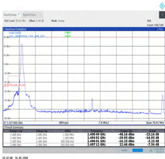
1-N41-30-70-L-4-CP-QPSK-Edge_1RB_Left-1@0-Ant1-1--PASS-see graph
