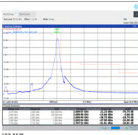
1-N41-30-15-H-2-DFT-PI2BPSK-Edge_1RB_Right-1@37-Ant1-1--PASS-see graph
