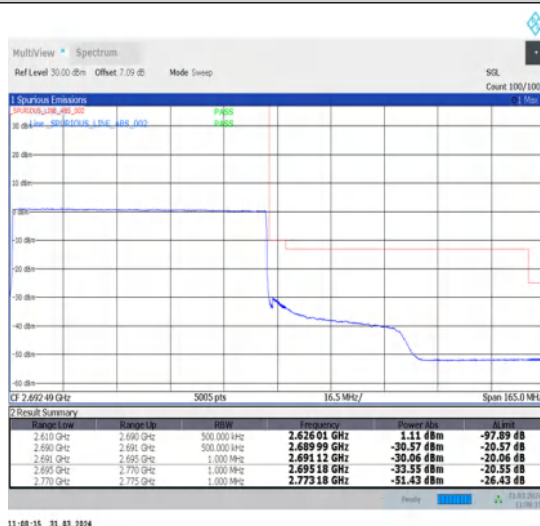
1-N41-30-80-H-6-CP-QPSK-Outer_Full-217@0-Ant1-1--PASS-see graph
