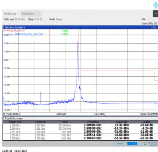
1-N41-30-90-H-5-CP-QPSK-Edge_1RB_Right-1@244-Ant1-1--PASS-see graph
