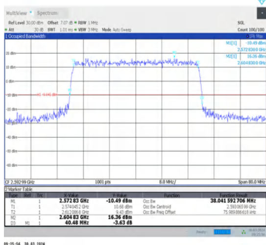
1-N41-30-40-M-7-CP-16QAM-Outer_Full-106@0-Ant1-38.042-40.480-≤40-PASS
