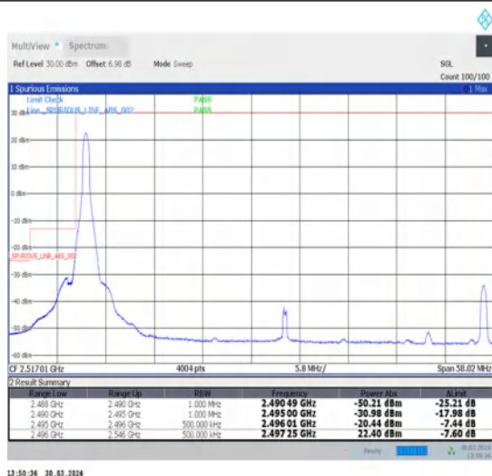
1-N41-30-50-L-1-DFT-PI2BPSK-Edge_1RB_Left-1@0-Ant1-1--PASS-see graph
