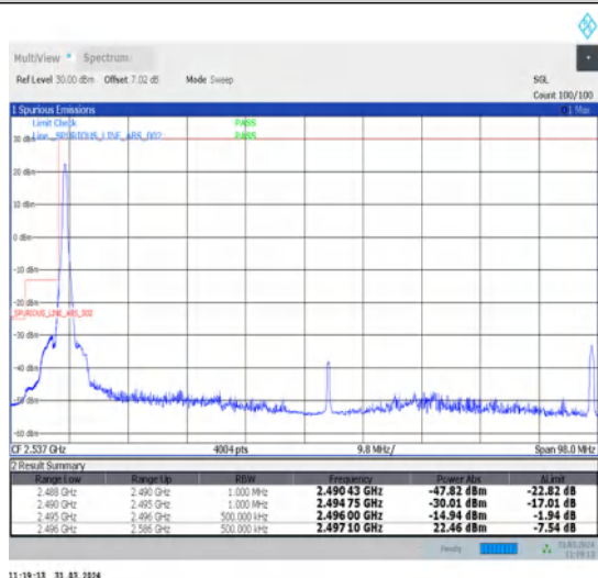
1-N41-30-90-L-4-CP-QPSK-Edge_1RB_Left-1@0-Ant1-1--PASS-see graph
