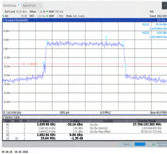
1-N41-30-30-H-9-CP-256QAM-Outer_Full-78@0- Ant1-27.77-29.640-≤30-PASS
