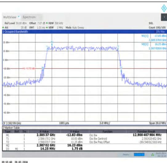
1-N41-30-15-M-4-DFT-64QAM-Outer_Full-36@0-Ant1-12.9-14.250-≤15-PASS
