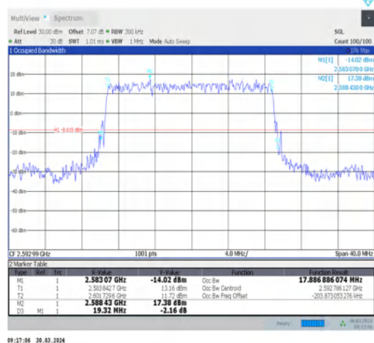
1-N41-30-20-M-2-DFT-PI2BPSK-Outet_Full-50@0-Ant1-17.887-19.320-≤20-PASS
