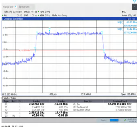
1-N41-30-60-M-8-CP-64QAM-Outer_Full-162@0-Ant1-57.796-60.960-≤60-PASS
