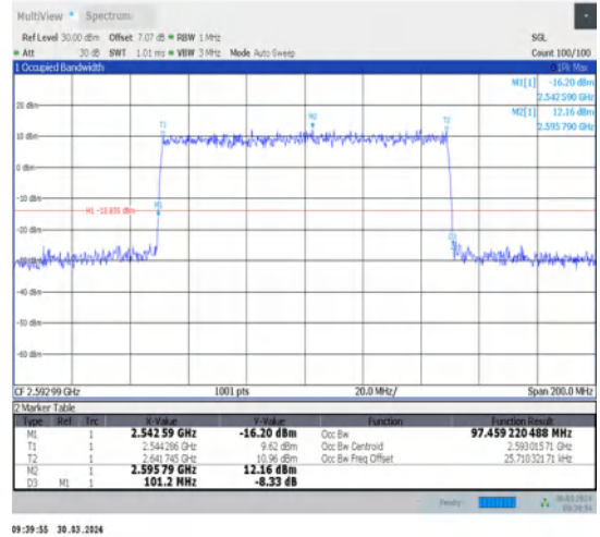
1-N41-30-100-M-7-CP-16QAM-Outer_Full-273@0-Ant1-97.459-101.200-≤100-PASS
