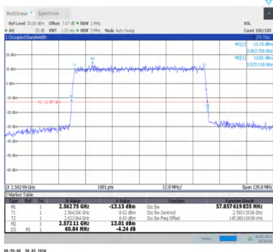
1-N41-30-60-M-5-DFT-256QAM-Outer_Full-162@0-Ant1-57.858-60.840-≤60-PASS
