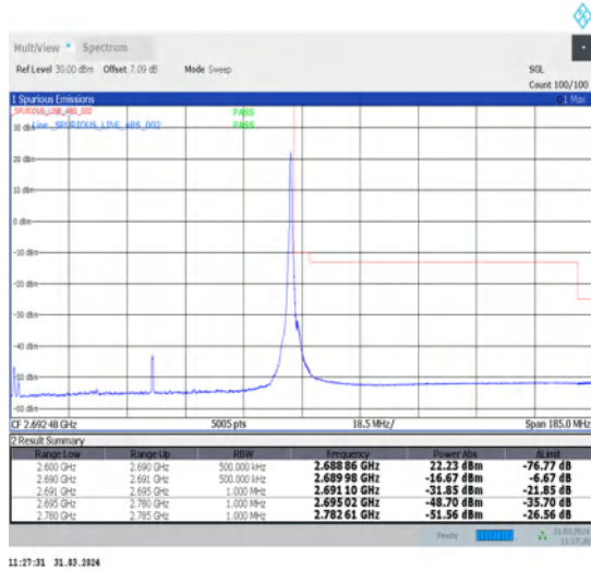
1-N41-30-90-H-2-DFT-PI2BPSK-Edge_1RB_Right-1@244-Ant1-1--PASS-see graph
