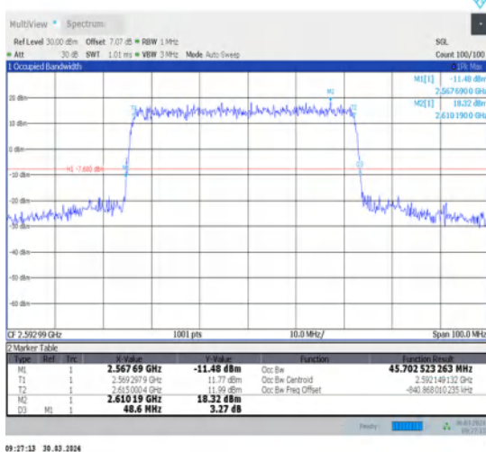
1-N41-30-50-M-1-DFT-QPSK-Outer_Full-128@0-Ant1-45.703-48.600-≤50-PASS
