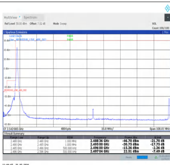
1-N41-30-100-L-1-DFT-PI2BPSK-Edge_1RB_Left-1@0-Ant1-1--PASS-see graph
