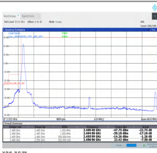
1-N41-30-60-L-4-CP-QPSK-Edge_1RB_Left-1@0-Ant1-1--PASS-see graph
