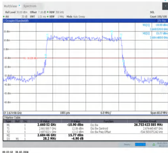
1-N41-30-30-H-2-DFT-PI2BPSK-Outer_Full-75@0-Ant1-26.755-28.200-≤30-PASS
