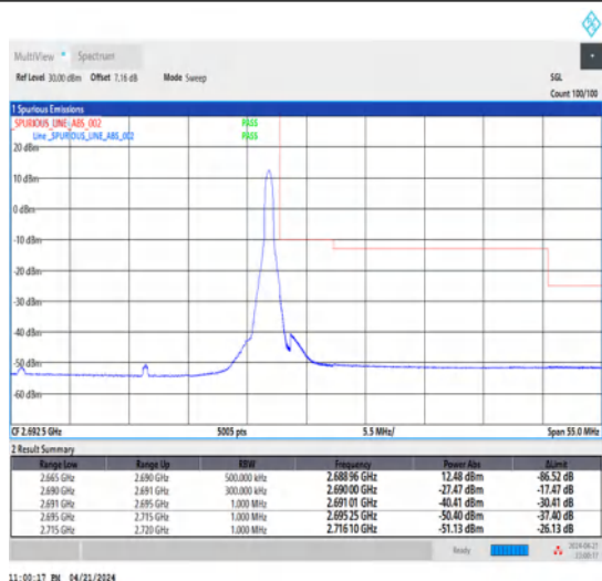
1-N41-30-25-H-2-DFT-PI2BPSK-Edge_1RB_Right-1@64-Ant1-1--PASS-see graph
