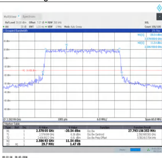
1-N41-30-30-M-7-CP-16QAM-Outer_Full-78@0-Ant1-27.781-29.700-≤30-PASS
