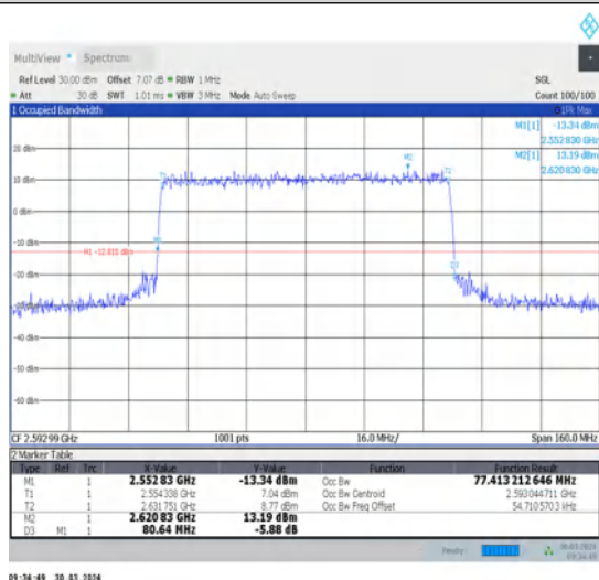
1-N41-30-80-M-7-CP-16QAM-Outer_Full-217@0-Ant1-77.413-80.640-≤80-PASS
