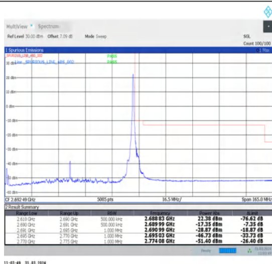
1-N41-30-80-H-5-CP-QPSK-Edge_1RB_Right-1@216-Ant1-1--PASS-see graph
