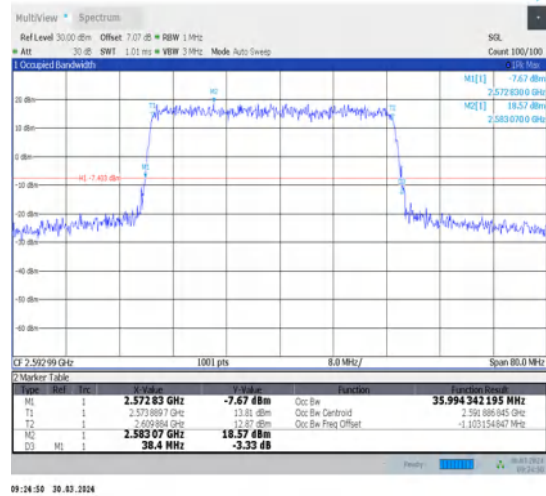
1-N41-30-40-M-1-DFT-QPSK-Outer_Full-100@0- Ant1-35.994-38.400-≤40-PASS
