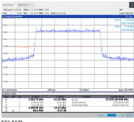
1-N41-30-60-M-6-CP-QPSK-Outer_Full-162@0-Ant1-57.87-60.600-≤60-PASS
