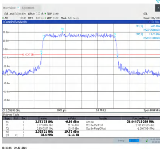
1-N41-30-40-M-2-DFT-PI2BPSK-Outer_Full-100@0- Ant1-36.045-38.400-≤40-PASS
