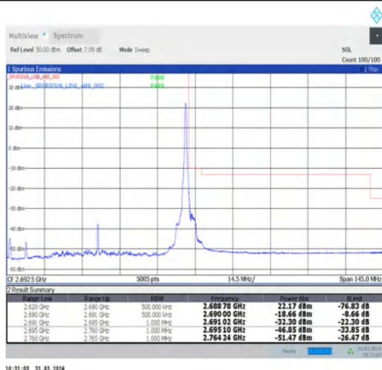
1-N41-30-70-H-5-CP-QPSK-Edge_1RB_Right-1@188-Ant1-1--PASS-see graph
