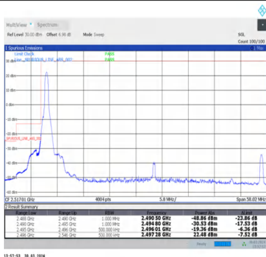
1-N41-30-50-L-4-CP-QPSK-Edge_1RB_Left-1@0-Ant1-1--PASS-see graph
