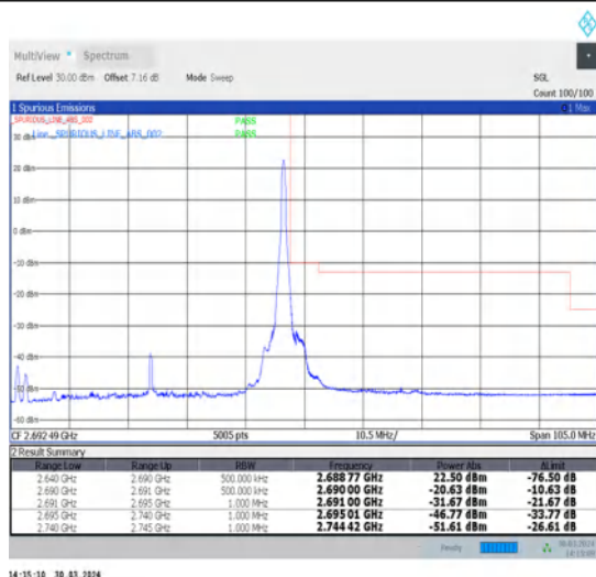
1-N41-30-50-H-5-CP-QPSK-Edge_1RB_Right-1@132-Ant1-1--PASS-see graph
