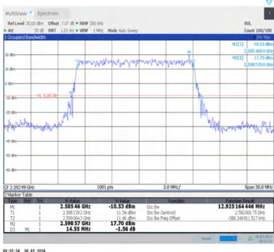
1-N41-30-15-M-2-DFT-PI2BPSK-Outer_Full-36@0-Ant1-12.925-14.550-≤15-PASS
