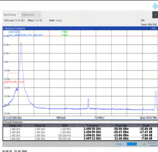
1-N41-30-70-L-1-DFT-PI2BPSK-Edge_1RB_Left-1@0-Ant1-1--PASS-see graph
