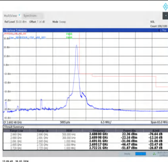
1-N41-30-30-H-5-CP-QPSK-Edge_1RB_Right-1@77-Ant1-1--PASS-see graph
