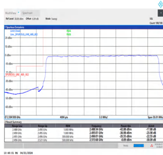
1-N41-30-25-L-3-DFT-PI2BPSK-Outer_Full-64@0-Ant1-1--PASS-see graph
