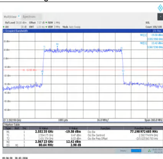
1-N41-30-80-M-5-DFT-256QAM-Outer_Full-216@0-Ant1-77.199-80.640-≤80-PASS
