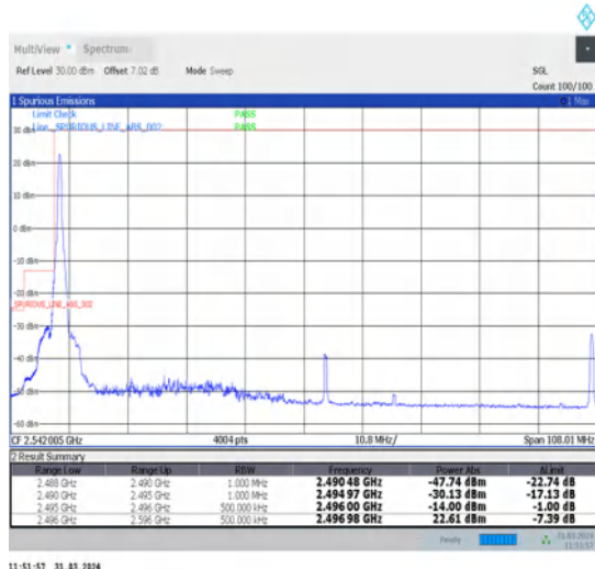
1-N41-30-100-L-4-CP-QPSK-Edge_1RB_Left-1@0-Ant1-1--PASS-see graph
