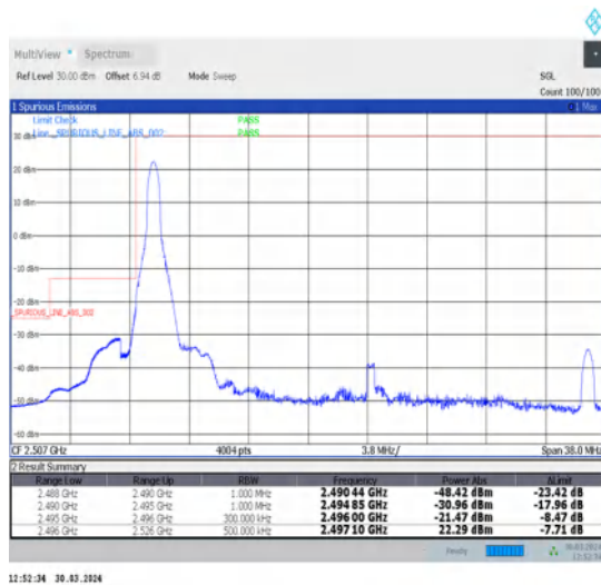
1-N41-30-30-L-4-CP-QPSK-Edge_1RB_Left-1@0-Ant1-1--PASS-see graph
