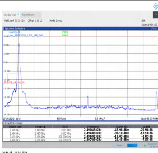
1-N41-30-80-L-4-CP-QPSK-Edge_1RB_Left-1@0-Ant1-1--PASS-see graph
