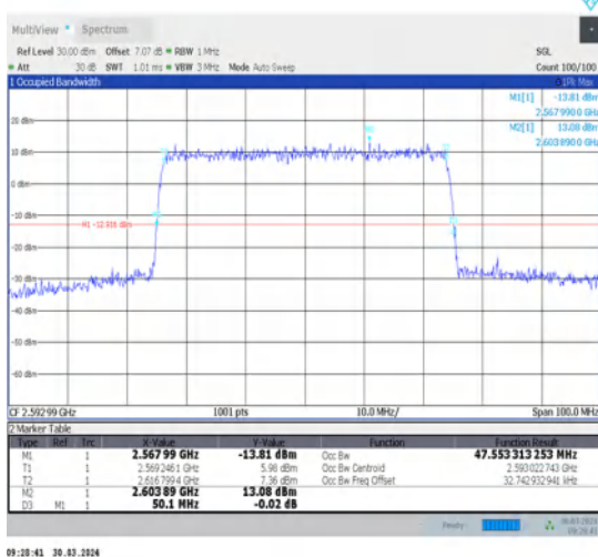
1-N41-30-50-M-9-CP-256QAM-Outer_Full-133@0-Ant1-47.553-50.100-≤50-PASS
