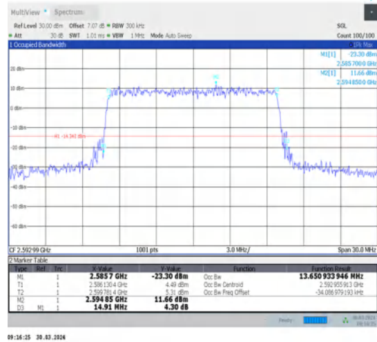
1-N41-30-15-M-9-CP-256QAM-Outet_Full-38@0-Ant1-13.651-14.910-≤15-PASS
