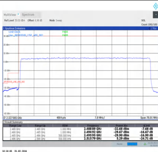
1-N41-30-70-L-3-DFT-PI2BPSK-Outer_Full-180@0-Ant1-1--PASS-see graph
