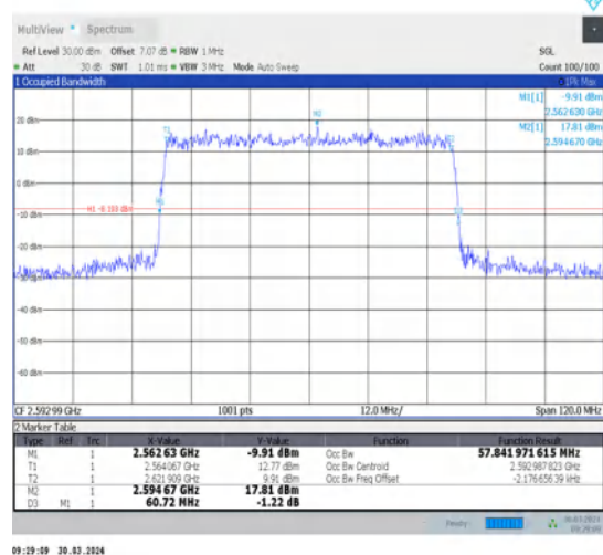
1-N41-30-60-M-1-DFT-QPSK-Outer_Full-162@0-Ant1-57.842-60.720-≤60-PASS
