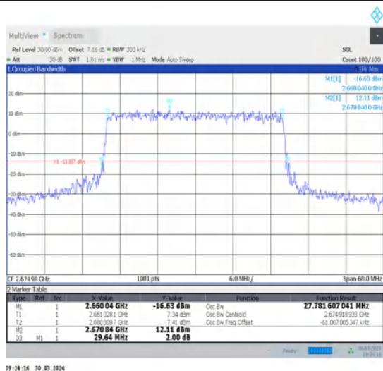
1-N41-30-30-H-8-CP-64QAM-Outer_Full-78@0-Ant1-27.784-29.640-≤30-PASS
