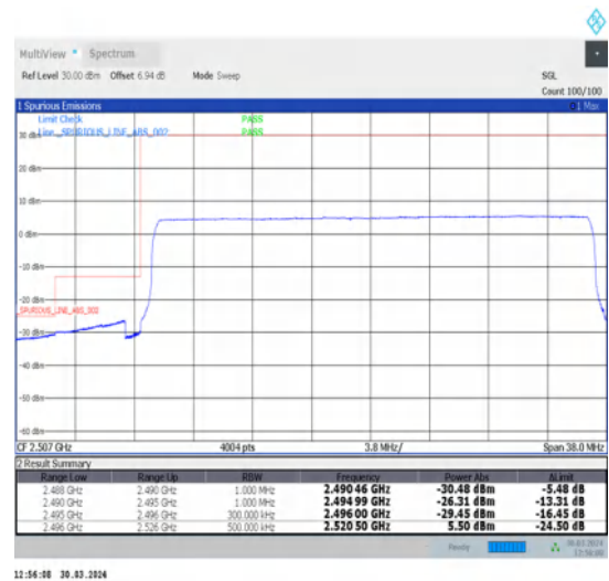
1-N41-30-30-L-6-CP-QPSK-Outer_Full-78@0-Ant1-1--PASS-see graph
