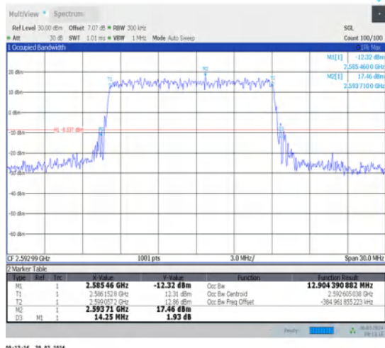
1-N41-30-15-M-1-DFT-QPSK-Outer_Full-36@0-Ant1-12.904-14.250-≤15-PASS
