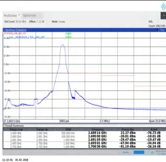
1-N41-30-10-H-2-DFT-PI2BPSK-Edge_1RB_Right-1@23-Ant1-1--PASS-see graph
