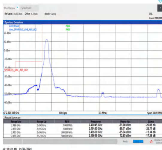
1-N41-30-25-L-4-CP-QPSK-Edge_1RB_Left-1@0-Ant1-1--PASS-see graph
