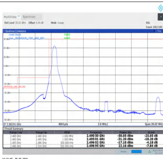
1-N41-30-20-L-1-DFT-PI2BPSK-Edge_1RB_Left-1@0-Ant1-1--PASS-see graph
