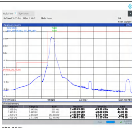
1-N41-30-15-L-1-DFT-PI2BPSK-Edge_1RB_Left-1@0-Ant1-1--PASS-see graph
