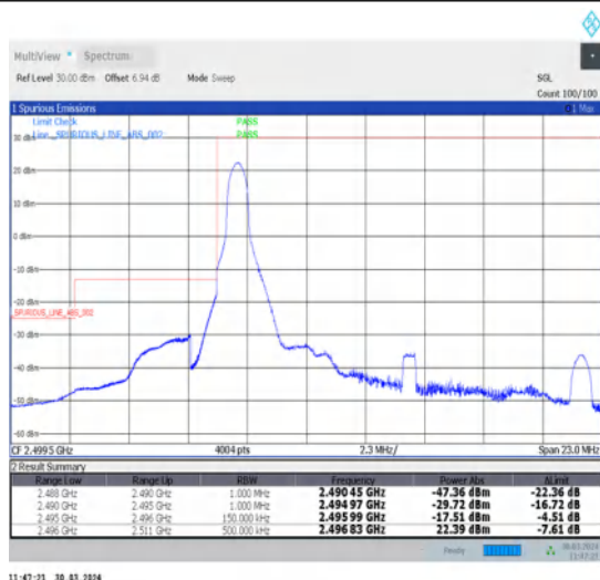
1-N41-30-15-L-4-CP-QPSK-Edge_1RB_Left-1@0-Ant1-1--PASS-see graph
