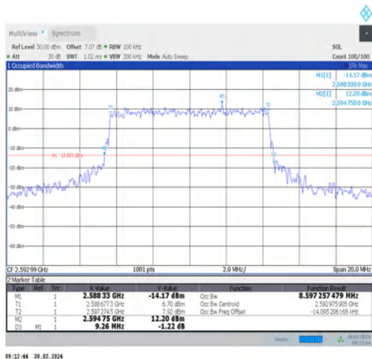
1-N41-30-10-M-8-CP-64QAM-Outer_Full-24@0-Ant1-8.597-9.260-≤10-PASS
