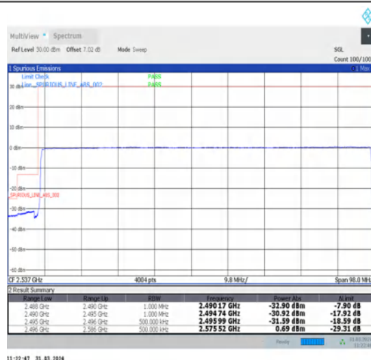
1-N41-30-90-L-6-CP-QPSK-Outer_Full-245@0-Ant1-1--PASS-see graph
