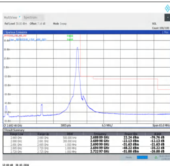
1-N41-30-30-H-2-DFT-PI2BPSK-Edge_1RB_Right-1@77-Ant1-1--PASS-see graph
