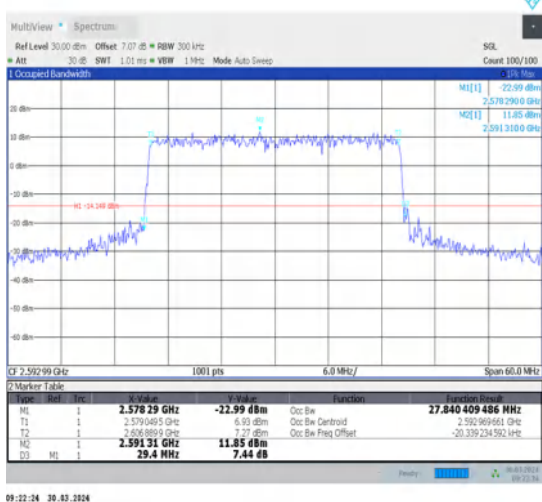
1-N41-30-30-M-8-CP-64QAM-Outer_Full-78@0-Ant1-27.844-29.400-≤30-PASS
