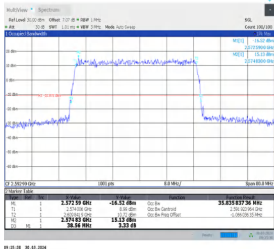
1-N41-30-40-M-5-DFT-256QAM-Outer_Full-100@0-Ant1-35.836-38.560-≤40-PASS
