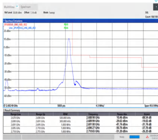
1-N41-30-20-H-5-CP-QPSK-Edge_1RB_Right-1@50-Ant1-1--PASS-see graph
