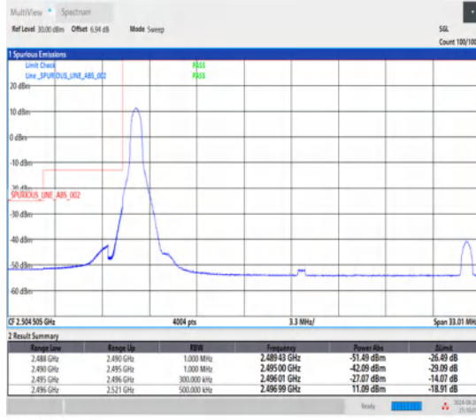
1-N41-30-25-L-1-DFT-PI2BPSK-Edge_1RB_Left-1@0-Ant1-1--PASS-see graph
