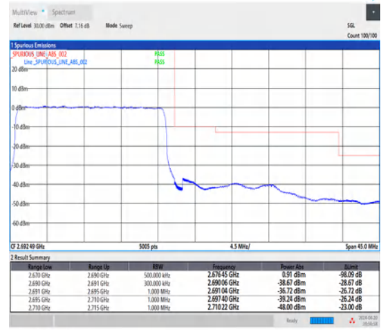
1-N41-30-20-H-3-DFT-PI2BPSK-Outer_Full-50@0-Ant1-1--PASS-see graph
