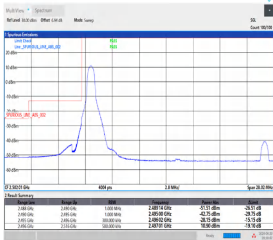
1-N41-30-20-L-1-DFT-PI2BPSK-Edge_1RB_Left-1@0-Ant1-1--PASS-see graph
