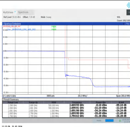
1-N41-30-100-H-6-CP-QPSK-Outer_Full-273@0-Ant1-1--PASS-see graph
