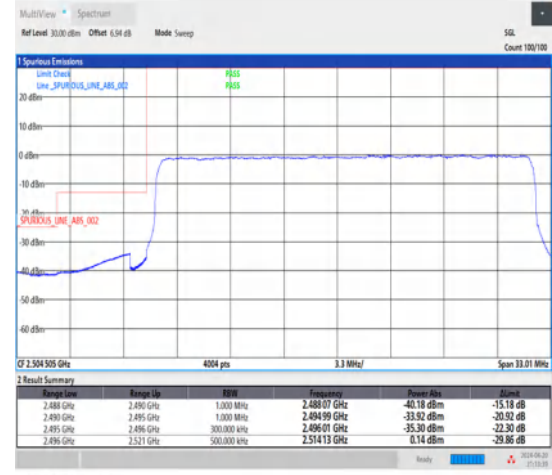
1-N41-30-25-L-3-DFT-PI2BPSK-Outer_Full-64@0-Ant1-1--PASS-see graph
