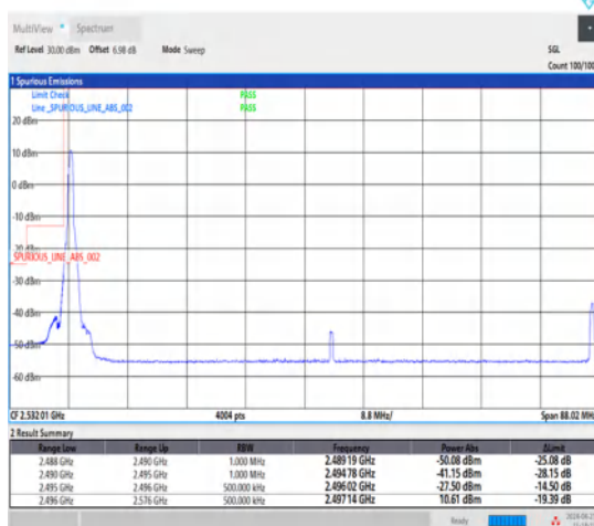
1-N41-30-80-L-4-CP-QPSK-Edge_1RB_Left-1@0-Ant1-1--PASS-see graph
