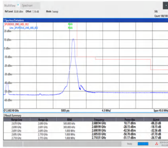
1-N41-30-20-H-2-DFT-PI2BPSK-Edge_1RB_Right-1@50-Ant1-1--PASS-see graph
