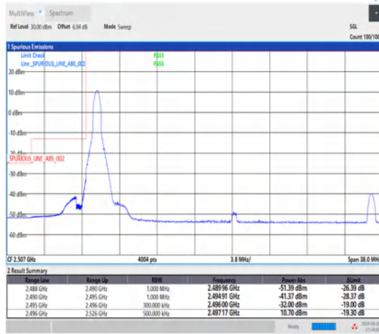
1-N41-30-30-L-4-CP-QPSK-Edge_1RB_Left-1@0-Ant1-1--PASS-see graph
