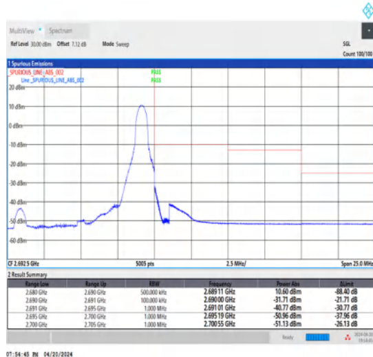
1-N41-30-10-H-5-CP-QPSK-Edge_1RB_Right-1@23-Ant1-1--PASS-see graph
