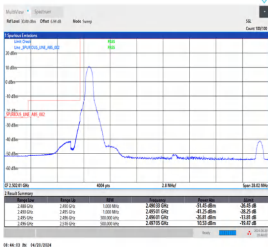
1-N41-30-20-L-4-CP-QPSK-Edge_1RB_Left-1@0-Ant1-1--PASS-see graph
