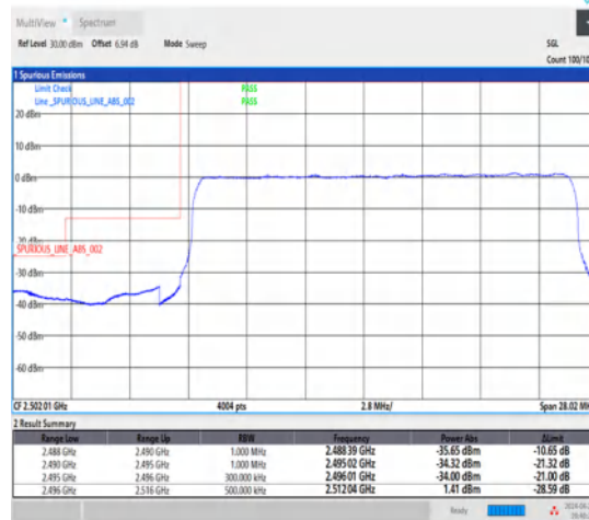
1-N41-30-20-L-3-DFT-PI2BPSK-Outer_Full-50@0-Ant1-1--PASS-see graph
