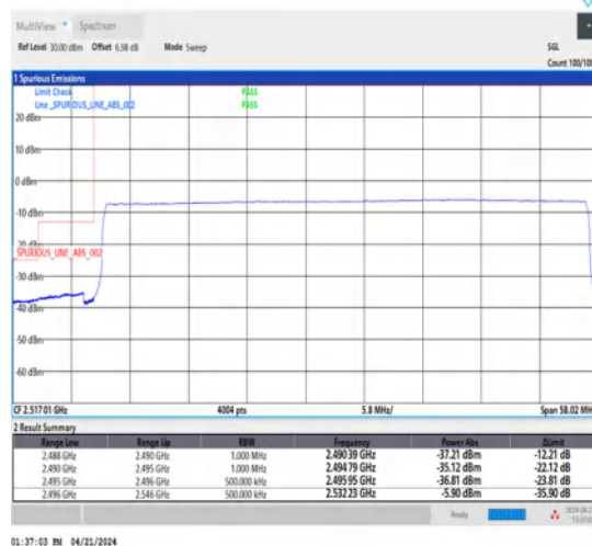
1-N41-30-50-L-6-CP-QPSK-Outer_Full-133@0-Ant1-1--PASS-see graph
