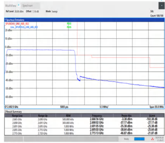
1-N41-30-25-H-6-CP-QPSK-Outer_Full-65@0-Ant1-1--PASS-see graph
