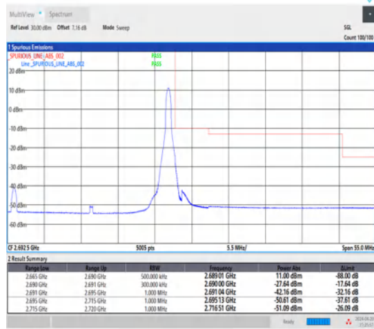
1-N41-30-25-H-2-DFT-PI2BPSK-Edge_1RB_Right-1@64-Ant1-1--PASS-see graph
