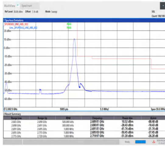
1-N41-30-25-H-5-CP-QPSK-Edge_1RB_Right-1@64-Ant1-1--PASS-see graph
