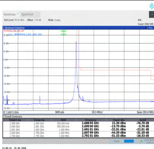
1-N41-30-100-H-2-DFT-PI2BPSK-Edge_1RB_Right-1@272-Ant1-1--PASS-see graph
