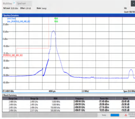
1-N41-30-15-L-1-DFT-PI2BPSK-Edge_1RB_Left-1@0-Ant1-1--PASS-see graph
