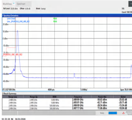
1-N41-30-70-L-1-DFT-PI2BPSK-Edge_1RB_Left-1@0-Ant1-1--PASS-see graph
