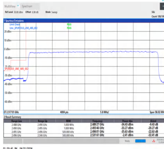
1-N41-30-50-L-3-DFT-PI2BPSK-Outer_Full-128@0-Ant1-1--PASS-see graph
