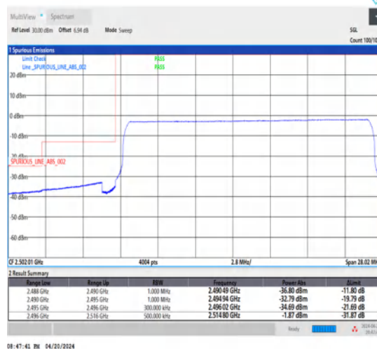
1-N41-30-20-L-6-CP-QPSK-Outer_Full-51@0-Ant1-1--PASS-see graph
