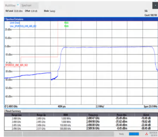
1-N41-30-15-L-6-CP-QPSK-Outer_Full-38@0-Ant1-1--PASS-see graph
