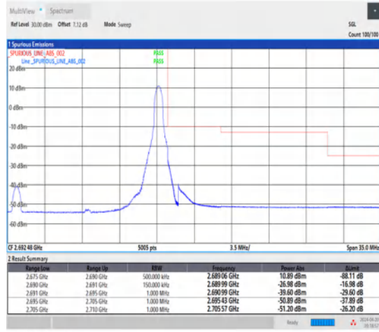
1-N41-30-15-H-2-DFT-PI2BPSK-Edge_1RB_Right-1@37-Ant1-1--PASS-see graph
