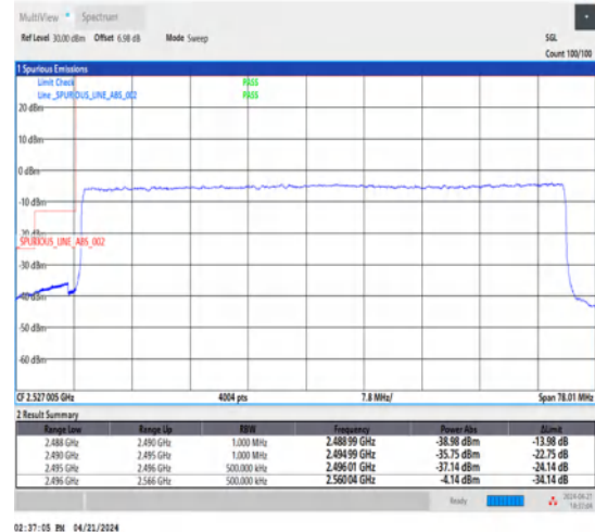
1-N41-30-70-L-3-DFT-PI2BPSK-Outer_Full-180@0-Ant1-1--PASS-see graph
