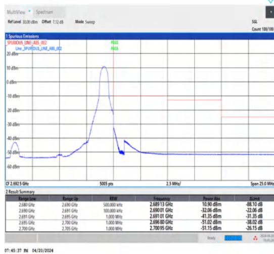
1-N41-30-10-H-2-DFT-PI2BPSK-Edge_1RB_Right-1@23-Ant1-1--PASS-see graph
