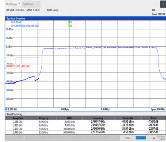
1-N41-30-30-L-3-DFT-PI2BPSK-Outer_Full-75@0-Ant1-1--PASS-see graph
