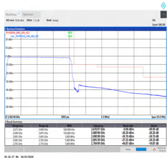
1-N41-30-15-H-6-CP-QPSK-Outer_Full-38@0-Ant1-1--PASS-see graph
