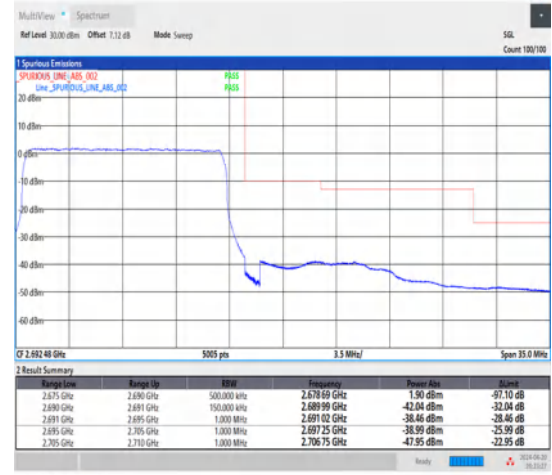
1-N41-30-15-H-3-DFT-PI2BPSK-Outer_Full-36@0-Ant1-1--PASS-see graph
