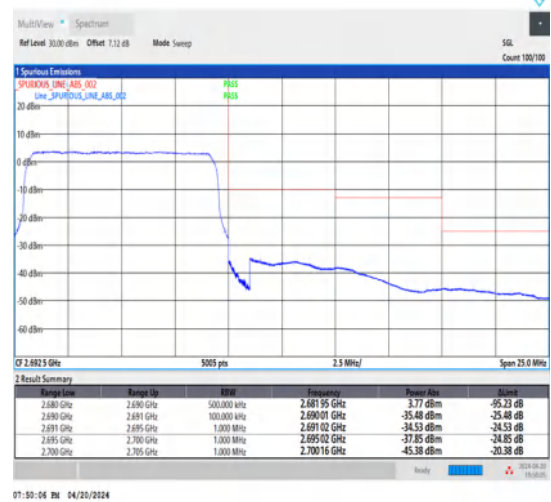
1-N41-30-10-H-3-DFT-PI2BPSK-Outer_Full-24@0-Ant1-1--PASS-see graph
