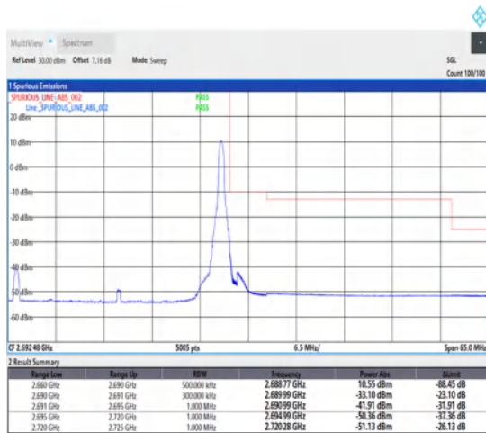
1-N41-30-30-H-2-DFT-PI2BPSK-Edge_1RB_Right-1@77-Ant1-1--PASS-see graph
