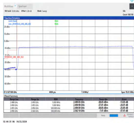
1-N41-30-70-L-6-CP-QPSK-Outer_Full-189@0-Ant1-1--PASS-see graph
