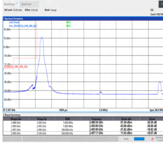
1-N41-30-30-L-1-DFT-PI2BPSK-Edge_1RB_Left-1@0-Ant1-1--PASS-see graph
