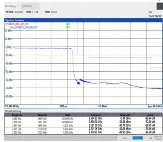
1-N41-30-30-H-3-DFT-PI2BPSK-Outer_Full-75@0-Ant1-1--PASS-see graph
