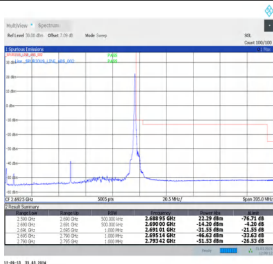
1-N41-30-100-H-5-CP-QPSK-Edge_1RB_Right-1@272-Ant1-1--PASS-see graph
