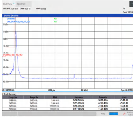
1-N41-30-80-L-1-DFT-PI2BPSK-Edge_1RB_Left-1@0-Ant1-1--PASS-see graph
