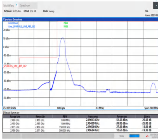
1-N41-30-15-L-4-CP-QPSK-Edge_1RB_Left-1@0-Ant1-1--PASS-see graph
