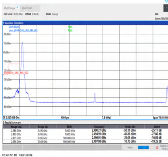
1-N41-30-70-L-4-CP-QPSK-Edge_1RB_Left-1@0-Ant1-1--PASS-see graph
