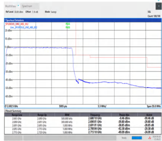
1-N41-30-25-H-3-DFT-PI2BPSK-Outer_Full-64@0-Ant1-1--PASS-see graph
