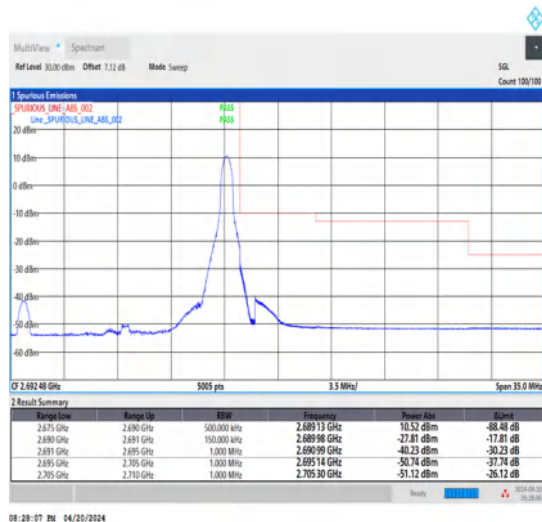
1-N41-30-15-H-5-CP-QPSK-Edge_1RB_Right-1@37-Ant1-1--PASS-see graph
