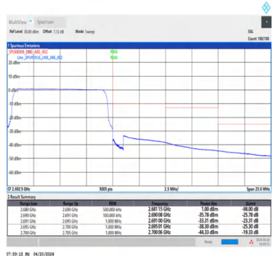
1-N41-30-10-H-6-CP-QPSK-Outer_Full-24@0-Ant1-1--PASS-see graph
