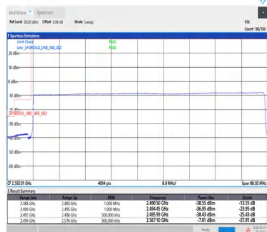
1-N41-30-80-L-6-CP-QPSK-Outer_Full-217@0-Ant1-1--PASS-see graph
