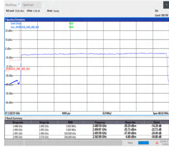
1-N41-30-80-L-3-DFT-PI2BPSK-Outer_Full-216@0-Ant1-1--PASS-see graph
