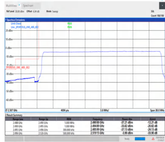
1-N41-30-30-L-6-CP-QPSK-Outer_Full-78@0-Ant1-1--PASS-see graph
