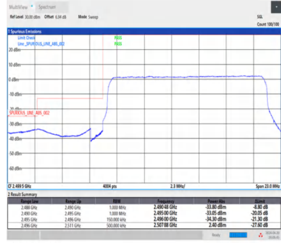
1-N41-30-15-L-3-DFT-PI2BPSK-Outer_Full-36@0-Ant1-1--PASS-see graph
