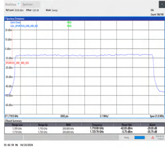
1-N66-15-20-L-3-DFT-PI2BPSK-Outer_Full-100@0-Ant1-1-seegraph-PASS-see graph
