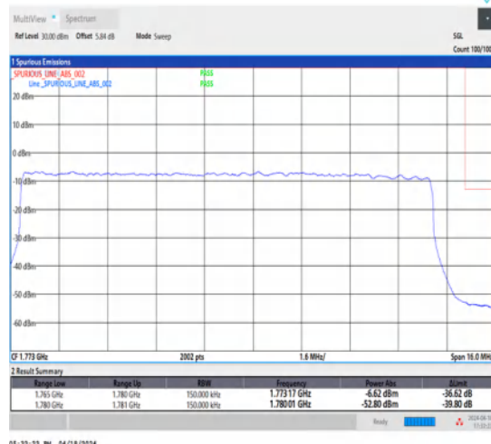
1-N66-15-15-H-3-DFT-PI2BPSK-Outer_Full-75@0-Ant1-1-seegraph-PASS-see graph
