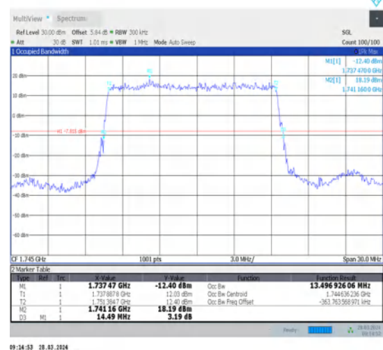
1-N66-15-15-M-2-DFT-PI2BPSK-Outer_Full-75@0-Ant1-13.497-14.490-≤15-PASS
