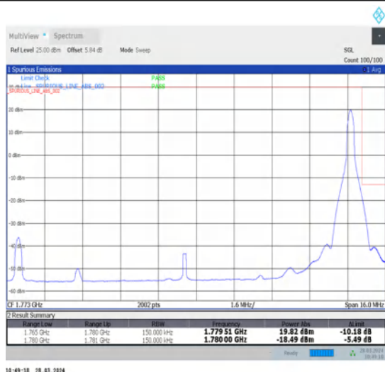
1-N66-15-15-H-5-CP-QPSK-Edge_1RB_Right-1@78-Ant1-1-seegraph-PASS-see graph
