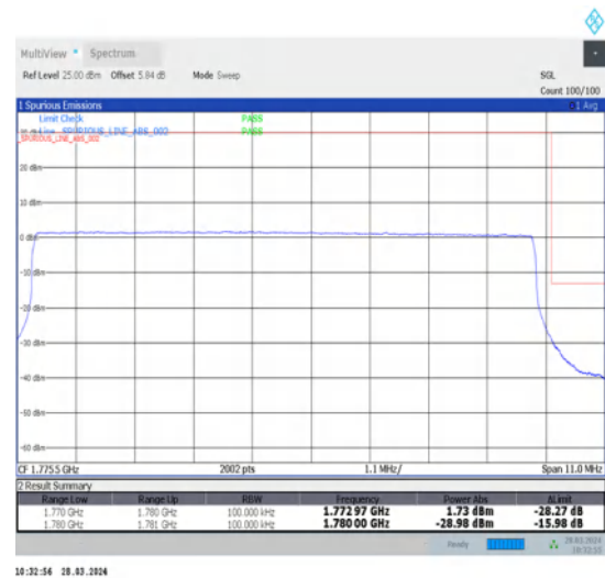
1-N66-15-10-H-6-CP-QPSK-Outer_Full-52@0-Ant1-1-seegraph-PASS-see graph
