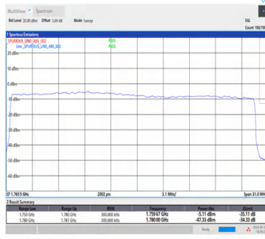
1-N66-15-30-H-3-DFT-PI2BPSK-Outer_Full-160@0-Ant1-1-seegraph-PASS-see graph
