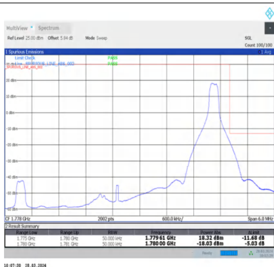
1-N66-15-5-H-2-DFT-PI2BPSK-Edge_1RB_Right-1@24-Ant1-1-seegraph-PASS-see graph
