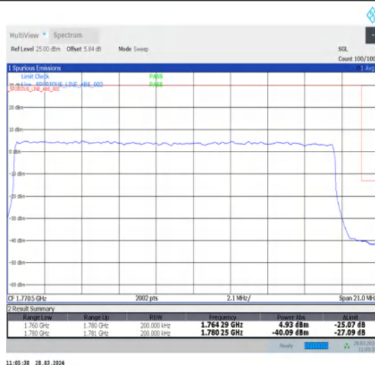
1-N66-15-20-H-3-DFT-PI2BPSK-Outer_Full-100@0-Ant1-1-seegraph-PASS-see graph
