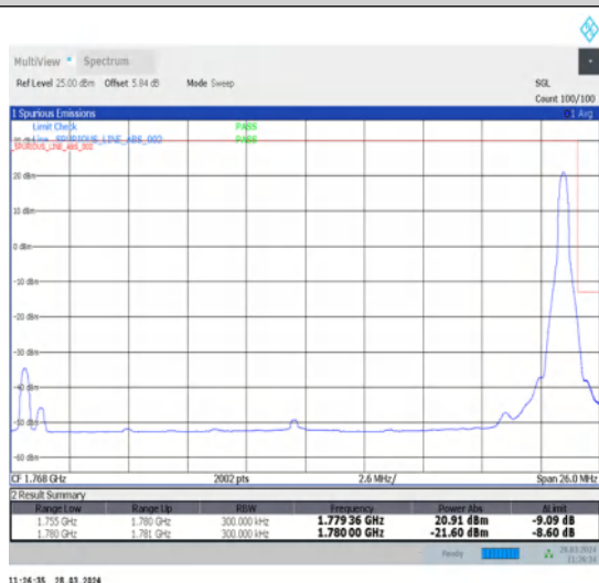
1-N66-15-25-H-5-CP-QPSK-Edge_1RB_Right-1@132-Ant1-1-seegraph-PASS-see graph
