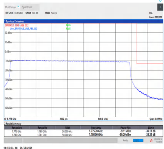
1-N66-15-5-H-6-CP-QPSK-Outer_Full-25@0-Ant1-1-seegraph-PASS-see graph
