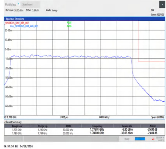
1-N66-15-5-H-3-DFT-PI2BPSK-Outer_Full-25@0-Ant1-1-seegraph-PASS-see graph
