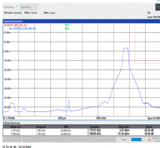
1-N66-15-5-H-5-CP-QPSK-Edge_1RB_Right-1@24-Ant1-1-seegraph-PASS-see graph
