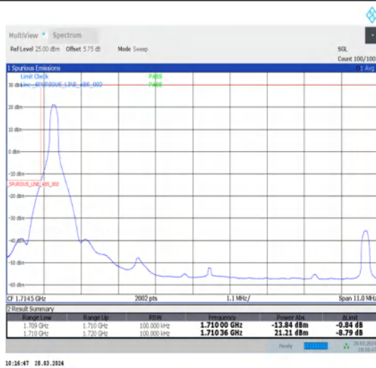
1-N66-15-10-L-1-DFT-PI2BPSK-Edge_1RB_Left-1@0-Ant1-1-seegraph-PASS-see graph
