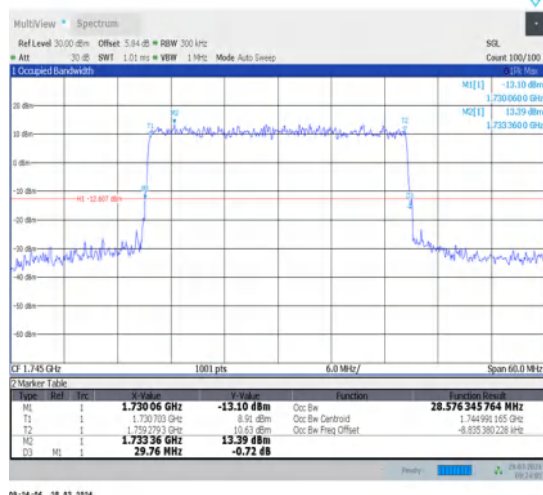
1-N66-15-30-M-1-DFT-QPSK-Outer_Full-160@0-Ant1-28.577-29.760-≤30-PASS
