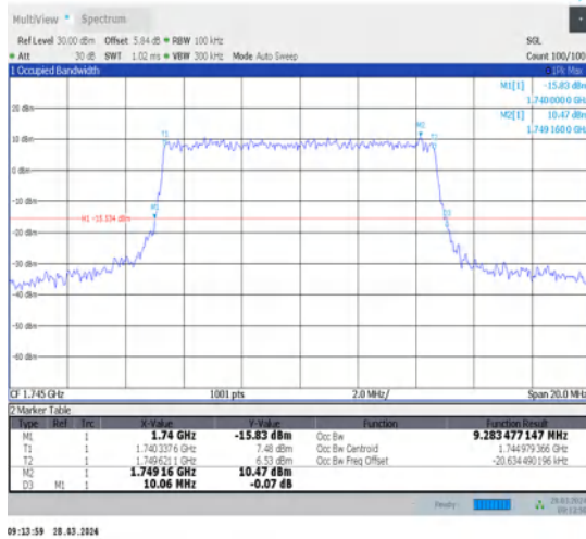
1-N66-15-10-M-8-CP-64QAM-Outer_Full-52@0-Ant1-9.283-10.060-≤10-PASS
