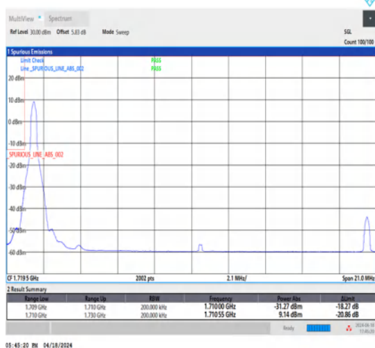
1-N66-15-20-L-4-CP-QPSK-Edge_1RB_Left-1@0-Ant1-1-seegraph-PASS-see graph
