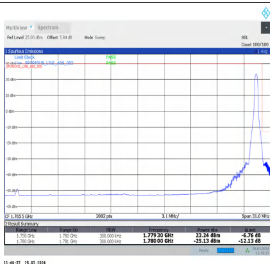
1-N66-15-30-H-2-DFT-PI2BPSK-Edge_1RB_Right-1@159-Ant1-1-seegraph-PASS-see graph
