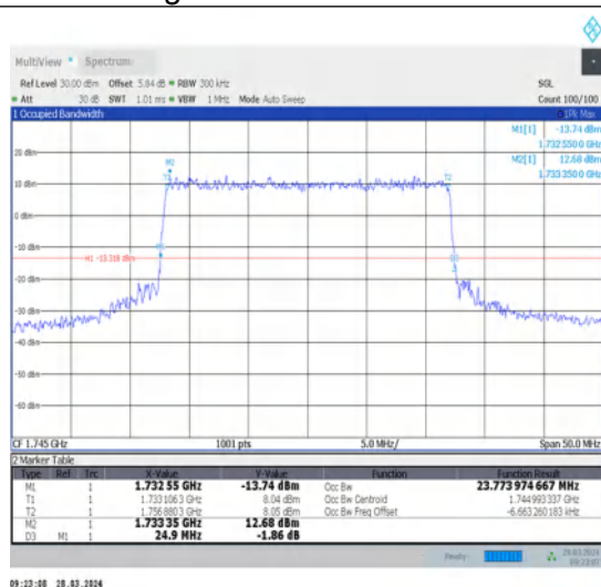
1-N66-15-25-M-6-CP-QPSK-Outer_Full-133@0-Ant1-23.774-24.900-≤25-PASS
