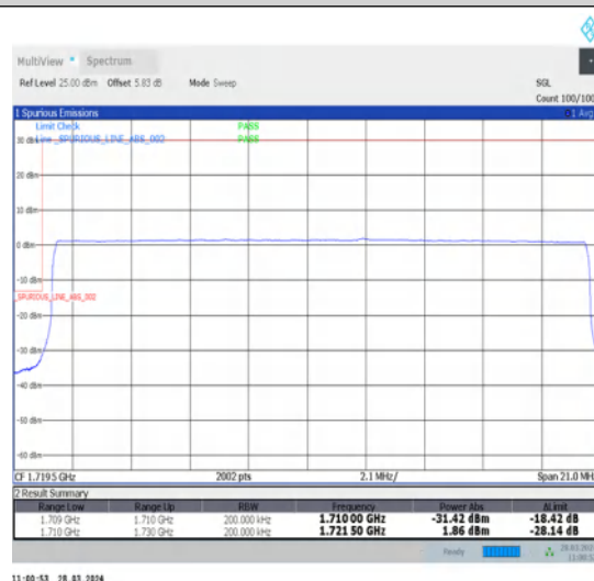
1-N66-15-20-L-6-CP-QPSK-Outer_Full-106@0-Ant1-1-seegraph-PASS-see graph
