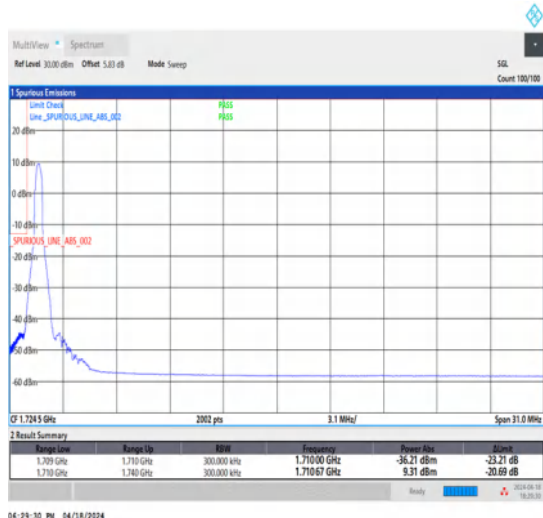
1-N66-15-30-L-4-CP-QPSK-Edge_1RB_Left-1@0-Ant1-1-seegraph-PASS-see graph
