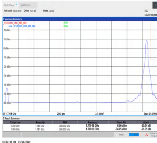
1-N66-15-20-H-2-DFT-PI2BPSK-Edge_1RB_Right-1@105-Ant1-1-seegraph-PASS-see graph
