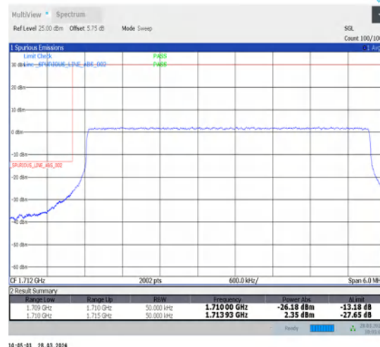
1-N66-15-5-L-6-CP-QPSK-Outer_Full-25@0-Ant1-1-seegraph-PASS-see graph
