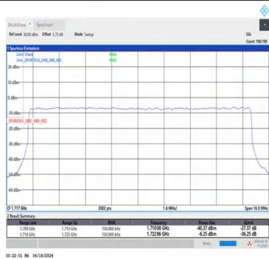
1-N66-15-15-L-3-DFT-PI2BPSK-Outer_Full-75@0-Ant1-1-seegraph-PASS-see graph
