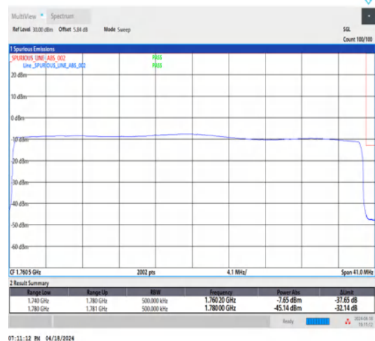
1-N66-15-40-H-6-CP-QPSK-Outer_Full-216@0-Ant1-1-seegraph-PASS-see graph
