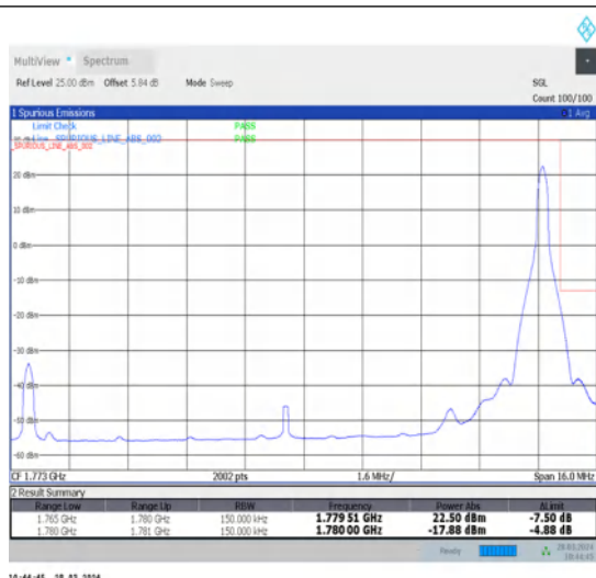
1-N66-15-15-H-2-DFT-PI2BPSK-Edge_1RB_Right-1@78-Ant1-1-seegraph-PASS-see graph
