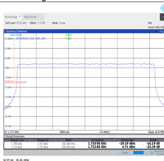
1-N66-15-15-L-3-DFT-PI2BPSK-Outer_Full-75@0-Ant1-1-seegraph-PASS-see graph
