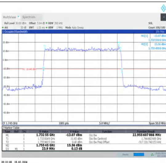
1-N66-15-25-M-1-DFT-QPSK-Outter_Full-128@0-Ant1-22.956-23.900-≤25-PASS
