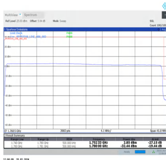
1-N66-15-40-H-6-CP-QPSK-Outer_Full-216@0-Ant1-1-seegraph-PASS-see graph
