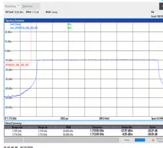
1-N66-15-5-L-6-CP-QPSK-Outer_Full-25@0-Ant1-1-seegraph-PASS-see graph
