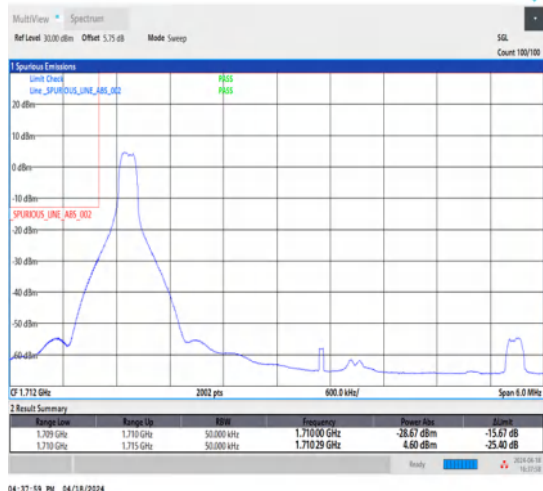
1-N66-15-5-L-1-DFT-PI2BPSK-Edge_1RB_Left-1@0-Ant1-1-seegraph-PASS-see graph
