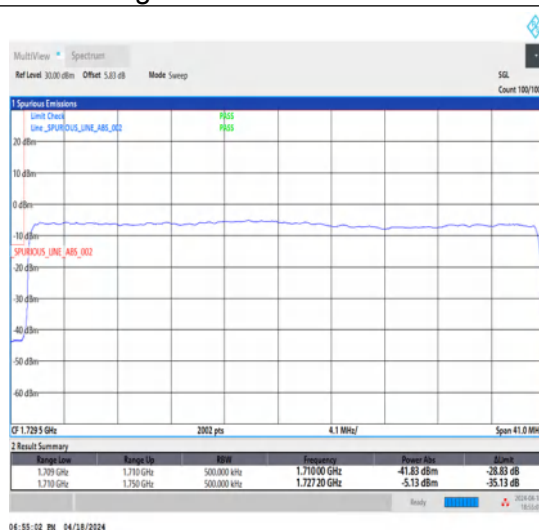
1-N66-15-40-L-3-DFT-PI2BPSK-Outer_Full-216@0-Ant1-1-seegraph-PASS-see graph
