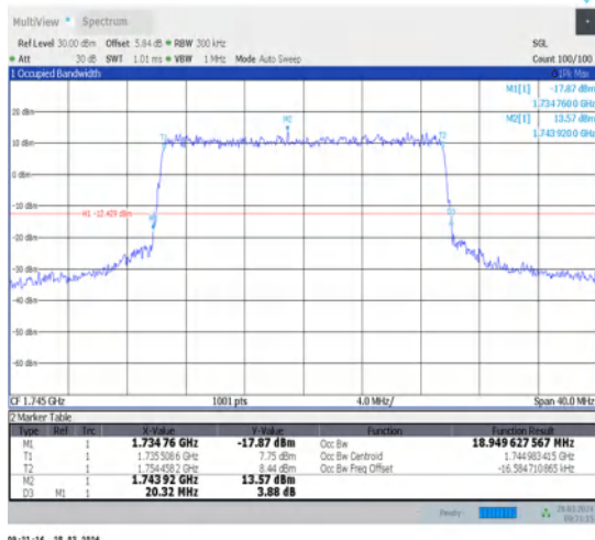
1-N66-15-20-M-7-CP-16QAM-Outer_Full-106@0-Ant1-18.95-20.320-≤20-PASS
