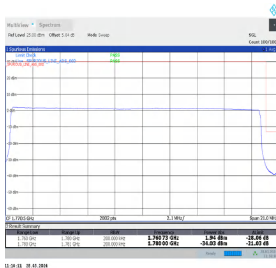
1-N66-15-20-H-6-CP-QPSK-Outer_Full-106@0-Ant1-1-seegraph-PASS-see graph
