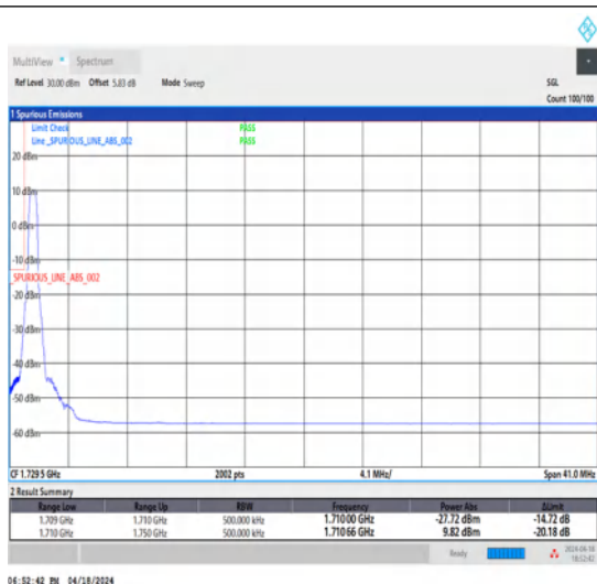
1-N66-15-40-L-1-DFT-PI2BPSK-Edge_1RB_Left-1@0-Ant1-1-seegraph-PASS-see graph
