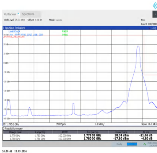
1-N66-15-10-H-5-CP-QPSK-Edge_1RB_Right-1@51-Ant1-1-seegraph-PASS-see graph
