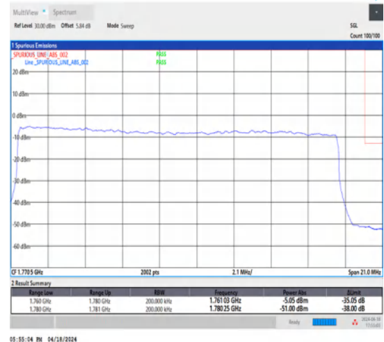
1-N66-15-20-H-3-DFT-PI2BPSK-Outer_Full-100@0-Ant1-1-seegraph-PASS-see graph
