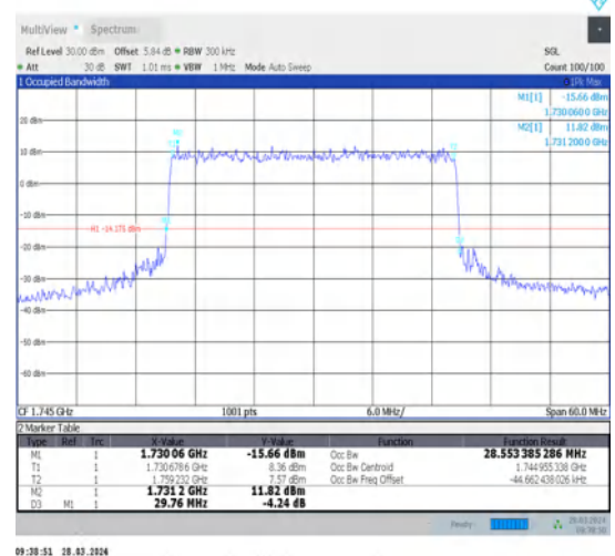
1-N66-15-30-M-7-CP-16QAM-Outer_Full-160@0-Ant1-28.554-29.760-≤30-PASS
