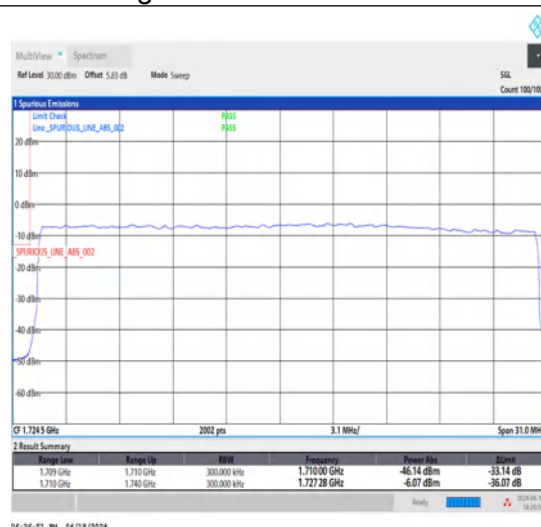
1-N66-15-30-L-3-DFT-PI2BPSK-Outer_Full-160@0-Ant1-1-seegraph-PASS-see graph
