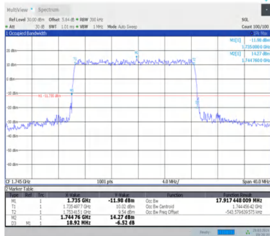
1-N66-15-20-M-3-DFT-16QAM-Outer_Full-100@0-Ant1-17.917-18.920-≤20-PASS
