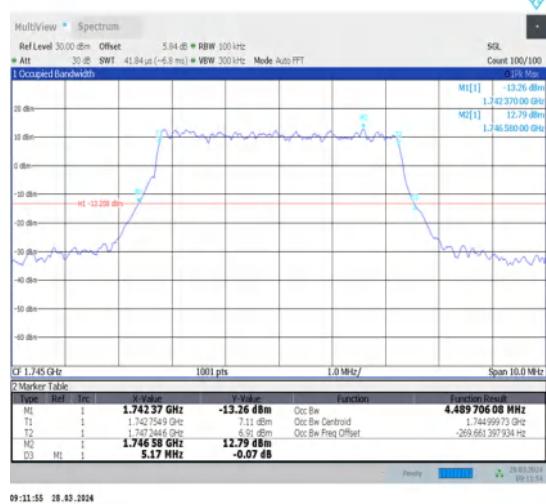
1-N66-15-5-M-8-CP-64QAM-Outer_Full-25@0-Ant1-4.49-5.170-≤5-PASS
