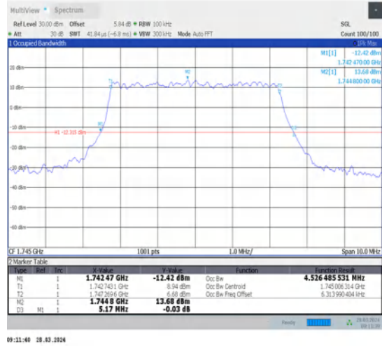
1-N66-15-5-M-6-CP-QPSK-Outer_Full-25@0-Ant1-4.526-5.170-≤5-PASS
