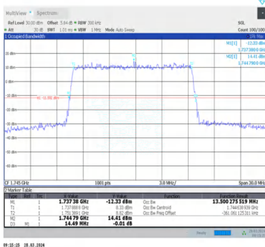
1-N66-15-15-M-5-DFT-256QAM-Outer_Full-75@0-Ant1-13.5-14.490-≤15-PASS
