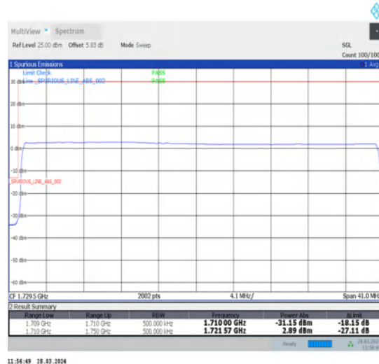
1-N66-15-40-L-6-CP-QPSK-Outer_Full-216@0-Ant1-1-seegraph-PASS-see graph
