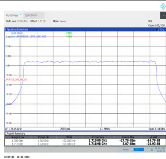
1-N66-15-10-L-3-DFT-PI2BPSK-Outer_Full-50@0-Ant1-1-seegraph-PASS-see graph
