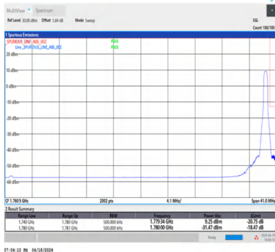
1-N66-15-40-H-2-DFT-PI2BPSK-Edge_1RB_Right-1@215-Ant1-1-seegraph-PASS-see graph
