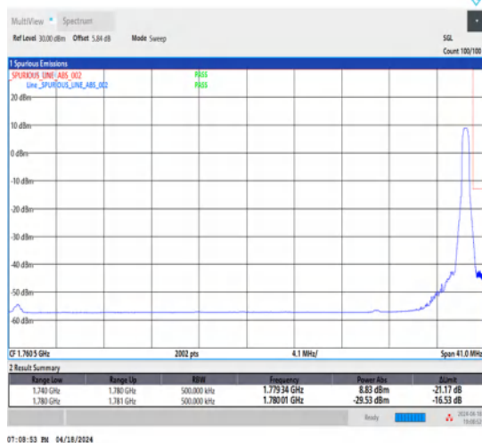
1-N66-15-40-H-5-CP-QPSK-Edge_1RB_Right-1@215-Ant1-1-seegraph-PASS-see graph
