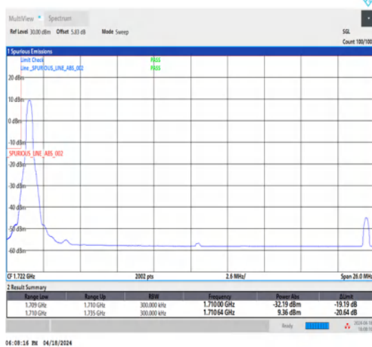
1-N66-15-25-L-4-CP-QPSK-Edge_1RB_Left-1@0-Ant1-1-seegraph-PASS-see graph
