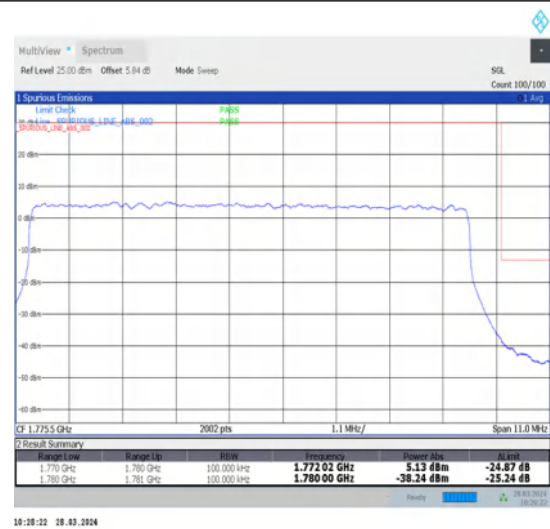
1-N66-15-10-H-3-DFT-PI2BPSK-Outer_Full-50@0-Ant1-1-seegraph-PASS-see graph
