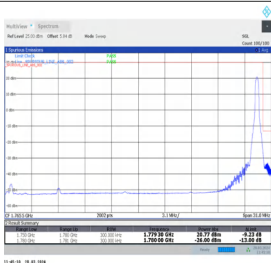
1-N66-15-30-H-5-CP-QPSK-Edge_1RB_Right-1@159-Ant1-1-seegraph-PASS-see graph
