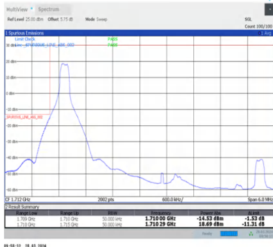
1-N66-15-5-L-1-DFT-PI2BPSK-Edge_1RB_Left-1@0-Ant1-1-seegraph-PASS-see graph
