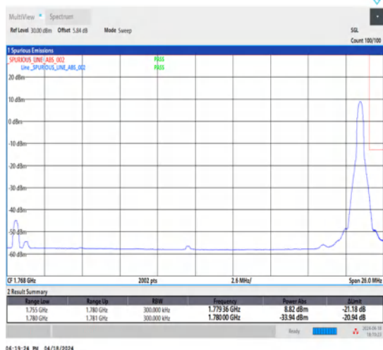
1-N66-15-25-H-5-CP-QPSK-Edge_1RB_Right-1@132-Ant1-1-seegraph-PASS-see graph
