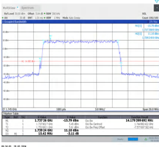
1-N66-15-15-M-9-CP-256QAM-Outet_Full-79@0-Ant1-14.179-15.420-≤15-PASS
