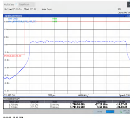
1-N66-15-5-L-3-DFT-PI2BPSK-Outer_Full-25@0-Ant1-1-seegraph-PASS-see graph
