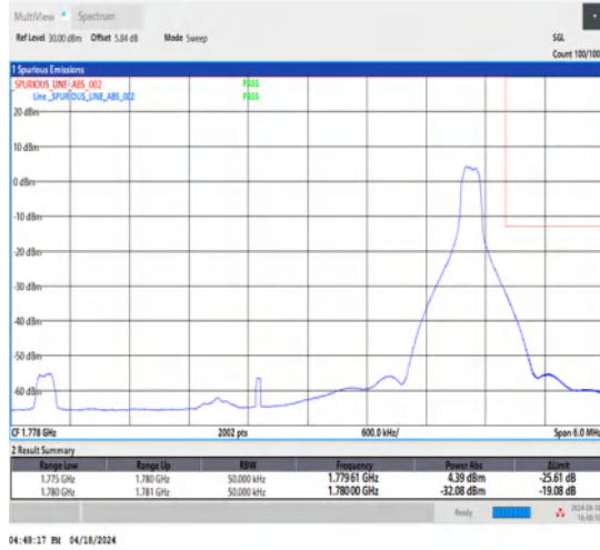
1-N66-15-5-H-2-DFT-PI2BPSK-Edge_1RB_Right-1@24-Ant1-1-seegraph-PASS-see graph
