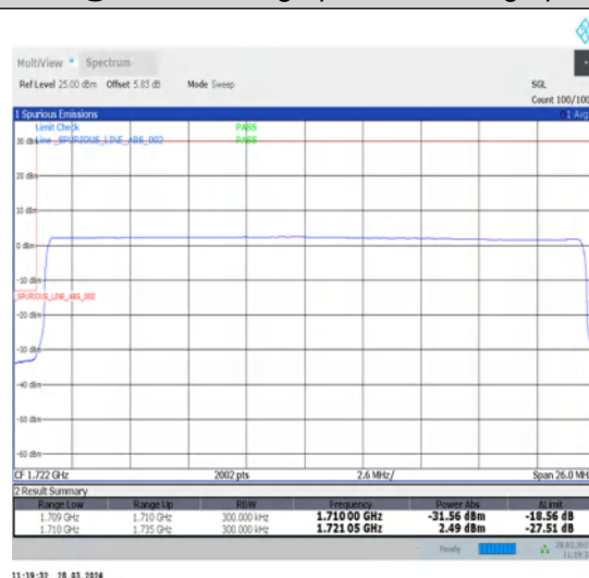
1-N66-15-25-L-6-CP-QPSK-Outer_Full-133@0-Ant1-1-seegraph-PASS-see graph
