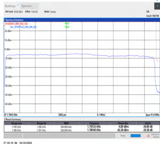
1-N66-15-40-H-3-DFT-PI2BPSK-Outer_Full-216@0-Ant1-1-seegraph-PASS-see graph
