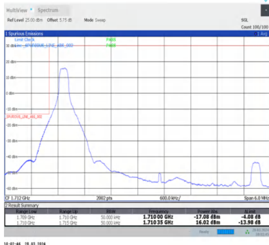
1-N66-15-5-L-4-CP-QPSK-Edge_1RB_Left-1@0-Ant1-1-seegraph-PASS-see graph
