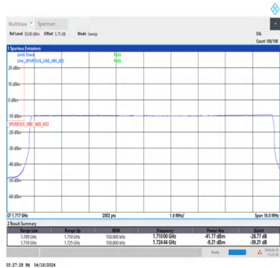
1-N66-15-15-L-6-CP-QPSK-Outer_Full-79@0-Ant1-1-seegraph-PASS-see graph
