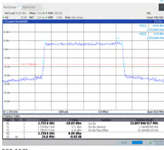
1-N66-15-25-M-9-CP-256QAM-Outer_Full-133@0-Ant1-23.808-24.800-≤25-PASS
