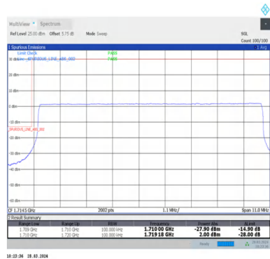
1-N66-15-10-L-6-CP-QPSK-Outer_Full-52@0-Ant1-1-seegraph-PASS-see graph
