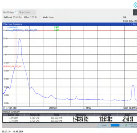
1-N66-15-10-L-4-CP-QPSK-Edge_1RB_Left-1@0-Ant1-1-seegraph-PASS-see graph
