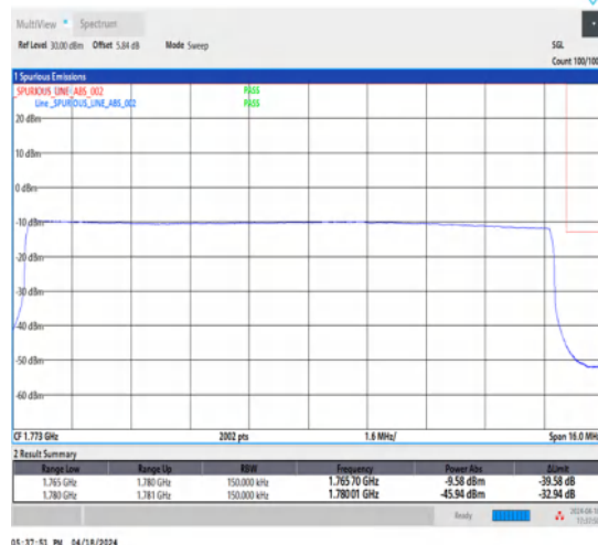
1-N66-15-15-H-6-CP-QPSK-Outer_Full-79@0-Ant1-1-seegraph-PASS-see graph
