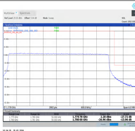
1-N66-15-5-H-6-CP-QPSK-Outer_Full-25@0-Ant1-1-seegraph-PASS-see graph
