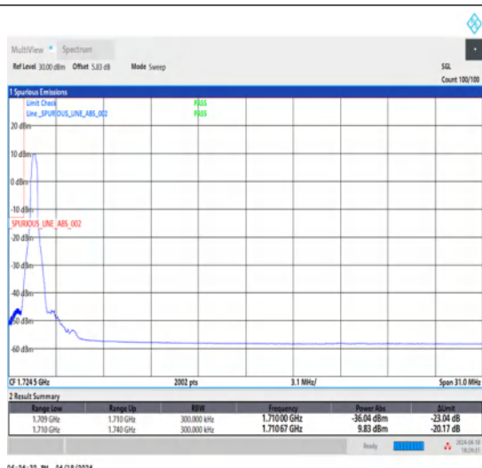
1-N66-15-30-L-1-DFT-PI2BPSK-Edge_1RB_Left-1@0-Ant1-1-seegraph-PASS-see graph
