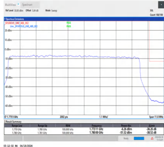
1-N66-15-10-H-3-DFT-PI2BPSK-Outer_Full-50@0-Ant1-1-seegraph-PASS-see graph
