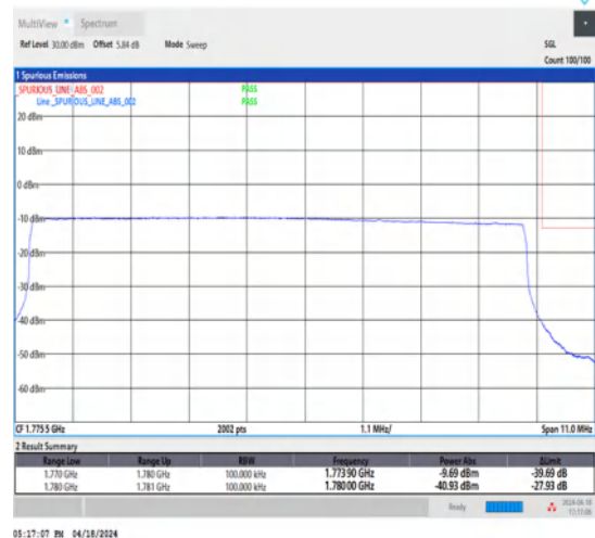
1-N66-15-10-H-6-CP-QPSK-Outer_Full-52@0-Ant1-1-seegraph-PASS-see graph
