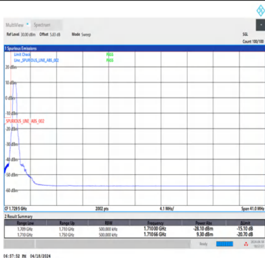
1-N66-15-40-L-4-CP-QPSK-Edge_1RB_Left-1@0-Ant1-1-seegraph-PASS-see graph
