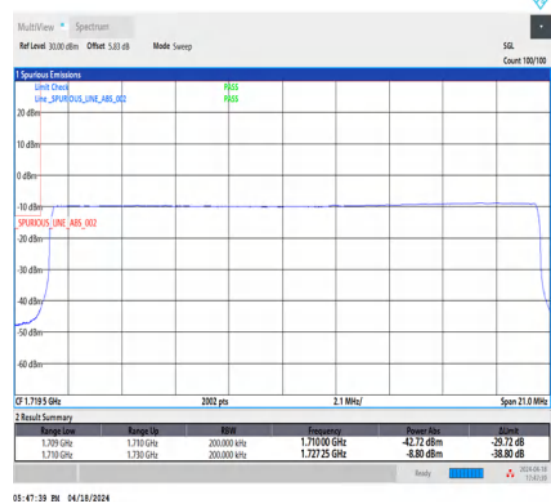
1-N66-15-20-L-6-CP-QPSK-Outer_Full-106@0-Ant1-1-seegraph-PASS-see graph
