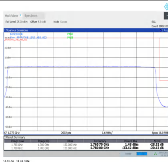
1-N66-15-15-H-6-CP-QPSK-Outer_Full-79@0-Ant1-1-seegraph-PASS-see graph
