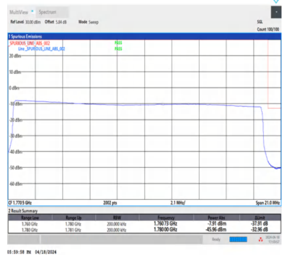
1-N66-15-20-H-6-CP-QPSK-Outer_Full-106@0-Ant1-1-seegraph-PASS-see graph
