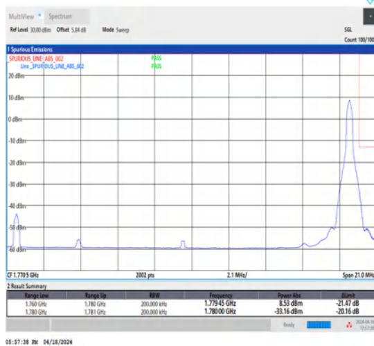
1-N66-15-20-H-5-CP-QPSK-Edge_1RB_Right-1@105-Ant1-1-seegraph-PASS-see graph
