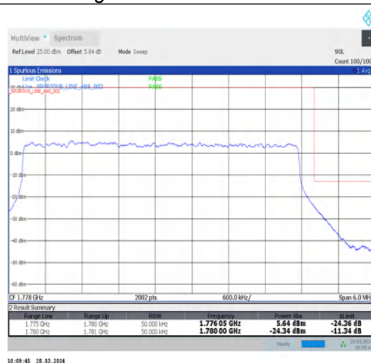
1-N66-15-5-H-3-DFT-PI2BPSK-Outer_Full-25@0-Ant1-1-seegraph-PASS-see graph
