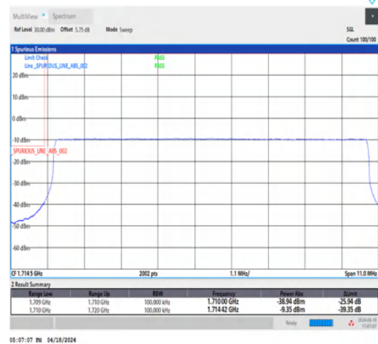
1-N66-15-10-L-6-CP-QPSK-Outer_Full-52@0-Ant1-1-seegraph-PASS-see graph
