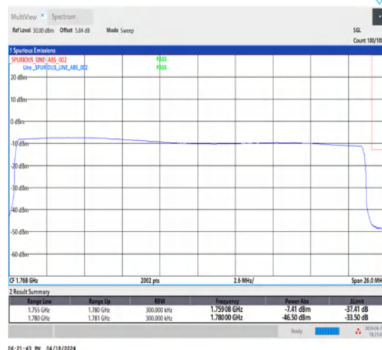
1-N66-15-25-H-6-CP-QPSK-Outer_Full-133@0-Ant1-1-seegraph-PASS-see graph
