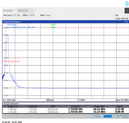
1-N66-15-40-L-4-CP-QPSK-Edge_1RB_Left-1@0-Ant1-1-seegraph-PASS-see graph
