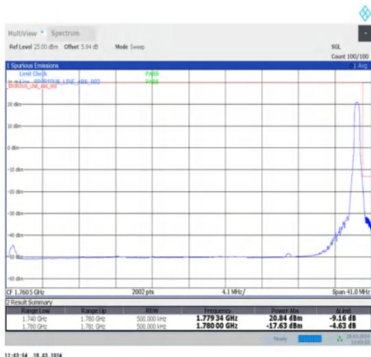
1-N66-15-40-H-5-CP-QPSK-Edge_1RB_Right-1@215-Ant1-1-seegraph-PASS-see graph
