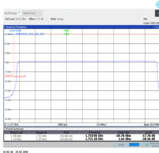
1-N66-15-15-L-6-CP-QPSK-Outer_Full-79@0-Ant1-1-seegraph-PASS-see graph
