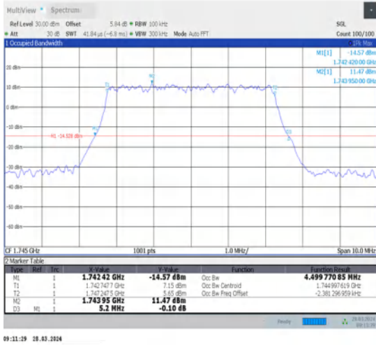
1-N66-15-5-M-5-DFT-256QAM-Outer_Full-25@0-Ant1.4.5-5.200-≤5-PASS
