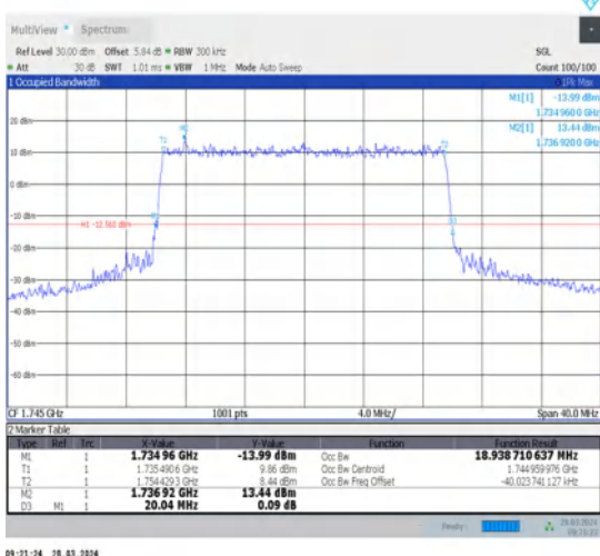
1-N66-15-20-M-8-CP-64QAM-Outer_Full-106@0-Ant1-18.939-20.040-≤20-PASS
