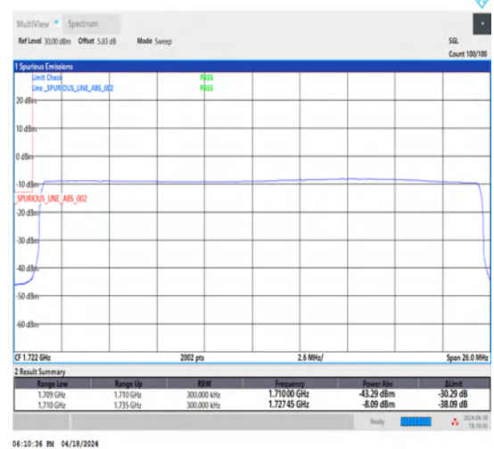
1-N66-15-25-L-6-CP-QPSK-Outer_Full-133@0-Ant1-1-seegraph-PASS-see graph
