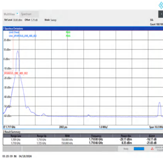
1-N66-15-15-L-4-CP-QPSK-Edge_1RB_Left-1@0-Ant1-1-seegraph-PASS-see graph
