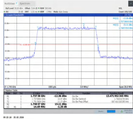
1-N66-15-15-M-4-DFT-64QAM-Outer_Full-75@0-Ant1-13.472-14.490-≤15-PASS
