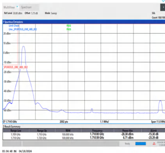
1-N66-15-10-L-4-CP-QPSK-Edge_1RB_Left-1@0-Ant1-1-seegraph-PASS-see graph
