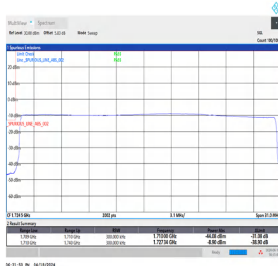
1-N66-15-30-L-6-CP-QPSK-Outer_Full-160@0-Ant1-1-seegraph-PASS-see graph
