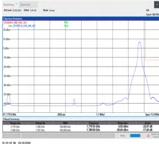
1-N66-15-10-H-2-DFT-PI2BPSK-Edge_1RB_Right-1@51-Ant1-1-seegraph-PASS-see graph
