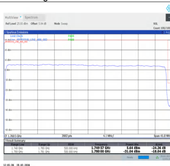
1-N66-15-40-H-3-DFT-PI2BPSK-Outer_Full-216@0-Ant1-1-seegraph-PASS-see graph
