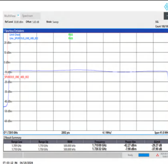
1-N66-15-40-L-6-CP-QPSK-Outer_Full-216@0-Ant1-1-seegraph-PASS-see graph
