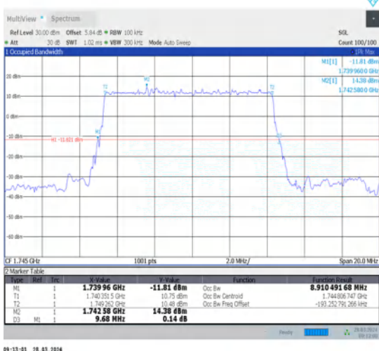
1-N66-15-10-M-2-DFT-PI2BPSK-Outer_Full-50@0-Ant1-8.91-9.680-≤10-PASS
