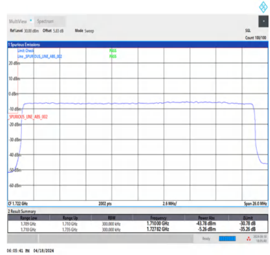
1-N66-15-25-L-3-DFT-PI2BPSK-Outer_Full-128@0-Ant1-1-seegraph-PASS-see graph
