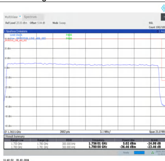
1-N66-15-30-H-3-DFT-PI2BPSK-Outer_Full-160@0-Ant1-1-seegraph-PASS-see graph
