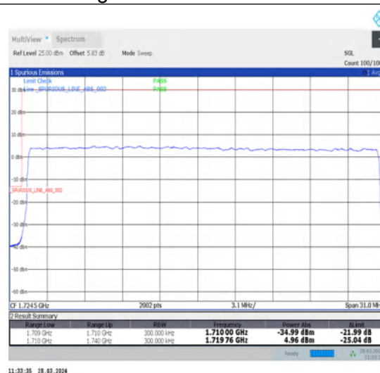
1-N66-15-30-L-3-DFT-PI2BPSK-Outer_Full-160@0-Ant1-1-seegraph-PASS-see graph
