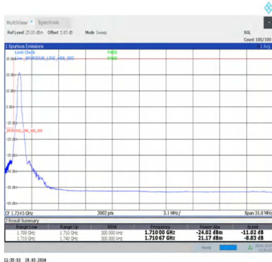
1-N66-15-30-L-4-CP-QPSK-Edge_1RB_Left-1@0-Ant1-1-seegraph-PASS-see graph
