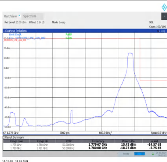
1-N66-15-5-H-5-CP-QPSK-Edge_1RB_Right-1@24-Ant1-1-seegraph-PASS-see graph
