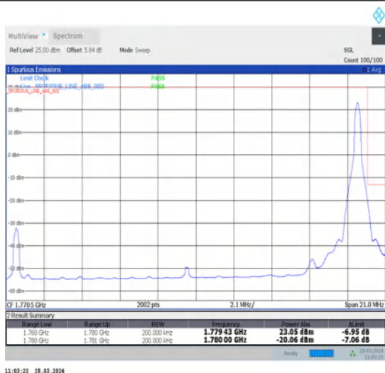
1-N66-15-20-H-2-DFT-PI2BPSK-Edge_1RB_Right-1@105-Ant1-1-seegraph-PASS-see graph
