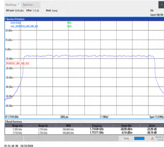
1-N66-15-10-L-3-DFT-PI2BPSK-Outer_Full-50@0-Ant1-1-seegraph-PASS-see graph
