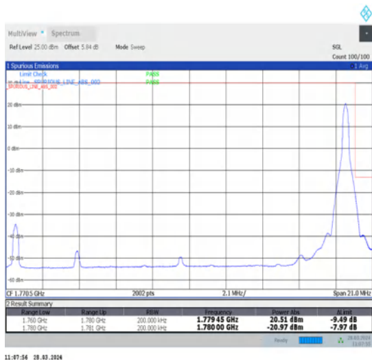
1-N66-15-20-H-5-CP-QPSK-Edge_1RB_Right-1@105-Ant1-1-seegraph-PASS-see graph
