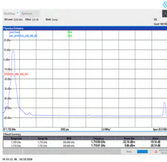
1-N66-15-25-L-1-DFT-PI2BPSK-Edge_1RB_Left-1@0-Ant1-1-seegraph-PASS-see graph
