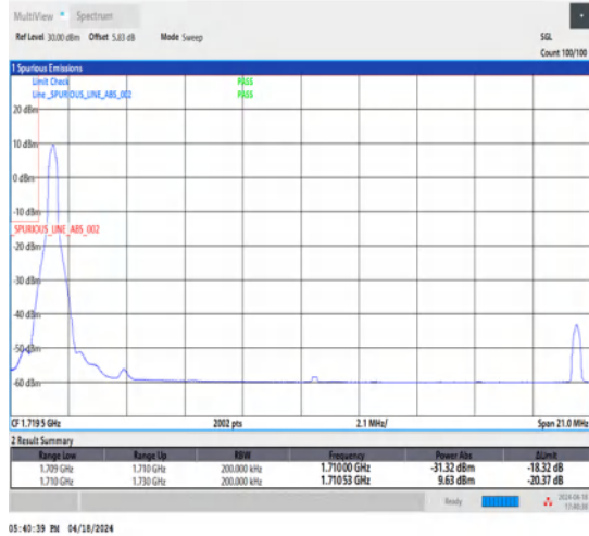
1-N66-15-20-L-1-DFT-PI2BPSK-Edge_1RB_Left-1@0-Ant1-1-seegraph-PASS-see graph
