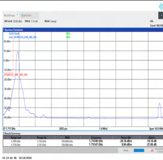
1-N66-15-15-L-1-DFT-PI2BPSK-Edge_1RB_Left-1@0-Ant1-1-seegraph-PASS-see graph
