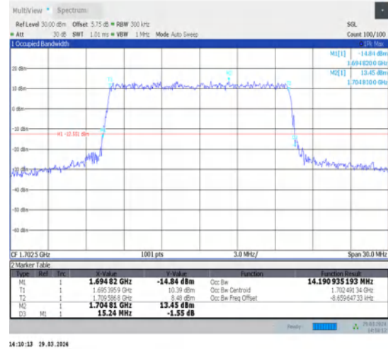
1-N70-15-15-M-8-CP-64QAM-Outet_Full-79@0-Ant1-14.191-15.240-≤15-PASS
