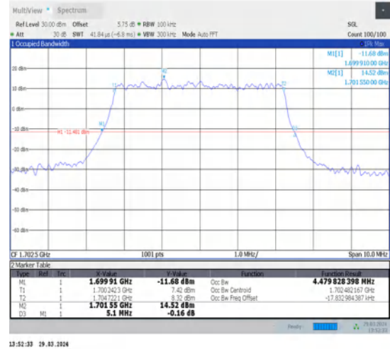
1-N70-15-5-M-6-CP-QPSK-Outer_Full-25@0-Ant1-4.48-5.100-≤5-PASS
