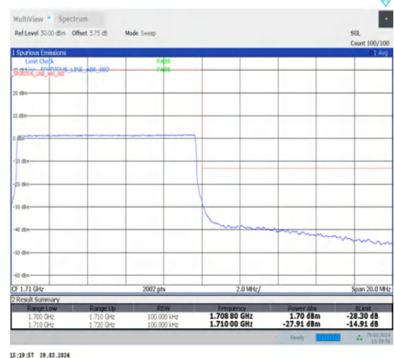
1-N70-15-10-H-6-CP-QPSK-Outer_Full-52@0-Ant1-1-seegraph-PASS-see graph
