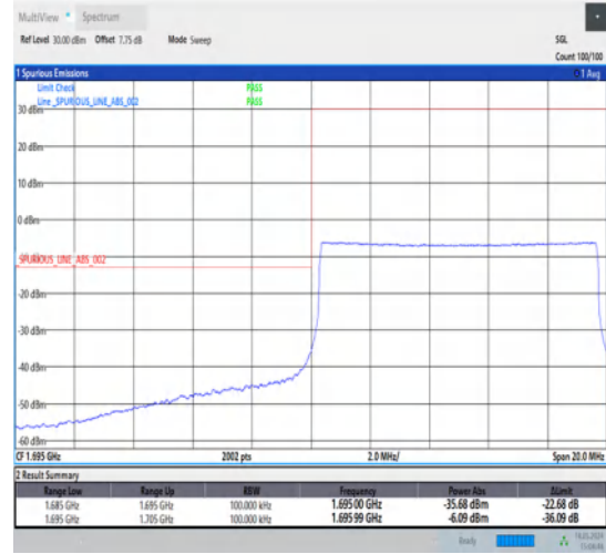
1-N70-15-10-L-6-CP-QPSK-Outer_Full-52@0-Ant1-1-seegraph-PASS-see graph
