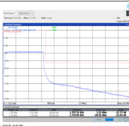
1-N70-15-5-H-6-CP-QPSK-Outer_Full-25@0-Ant1-1-seegraph-PASS-see graph
