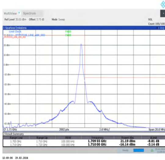
1-N70-15-10-H-2-DFT-PI2BPSK-Edge_1RB_Right-1@51-Ant1-1-seegraph-PASS-see graph
