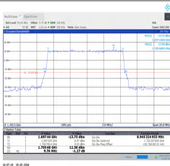
1-N70-15-10-M-3-DFT-16QAM-Out_Full-50@0-Ant1-8.945-9.760-≤10-PASS
