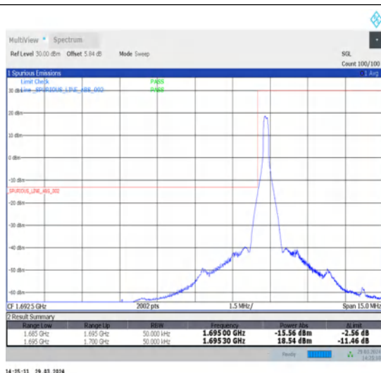
1-N70-15-5-L-1-DFT-PI2BPSK-Edge_1RB_Left-1@0-Ant1-1-seegraph-PASS-see graph
