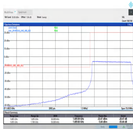
1-N70-15-5-L-6-CP-QPSK-Outer_Full-25@0-Ant1- 1-seegraph-PASS-see graph
