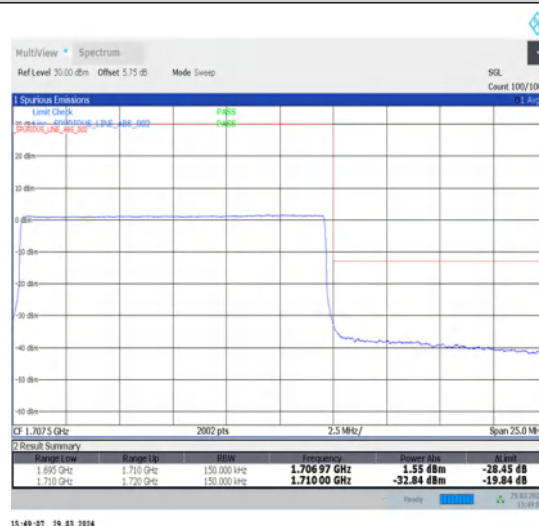
1-N70-15-15-H-6-CP-QPSK-Outer_Full-79@0-Ant1-1-seegraph-PASS-see graph
