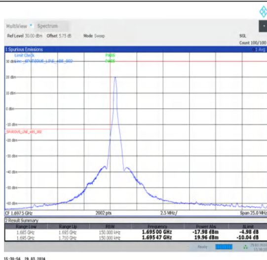
1-N70-15-15-L-4-CP-QPSK-Edge_1RB_Left-1@0-Ant1-1-seegraph-PASS-see graph
