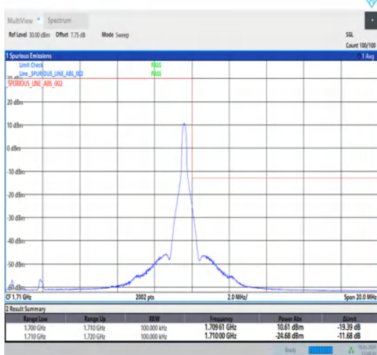
1-N70-15-10-H-5-CP-QPSK-Edge_1RB_Right-1@51-Ant1-1-seegraph-PASS-see graph
