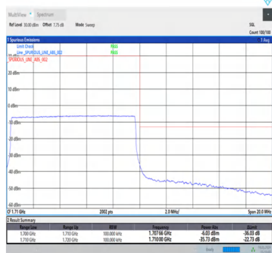
1-N70-15-10-H-6-CP-QPSK-Outer_Full-52@0-Ant1-1-seegraph-PASS-see graph
