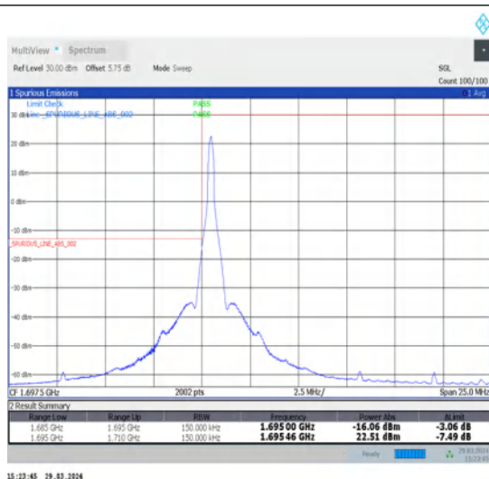
1-N70-15-15-L-1-DFT-PI2BPSK-Edge_1RB_Left-1@0-Ant1-1-seegraph-PASS-see graph
