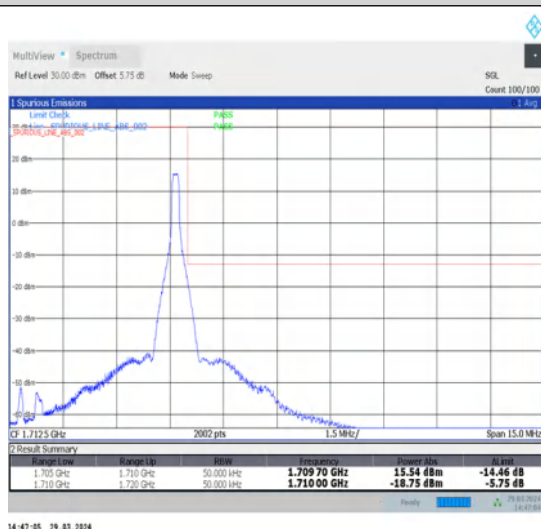
1-N70-15-5-H-5-CP-QPSK-Edge_1RB_Right-1@24-Ant1-1-seegraph-PASS-see graph
