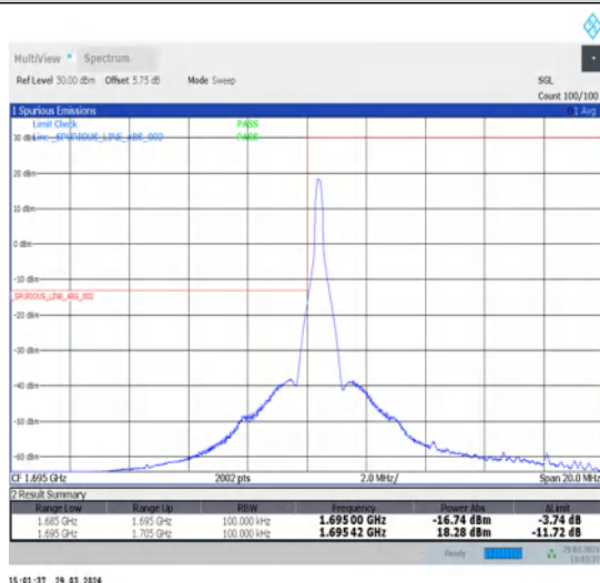
1-N70-15-10-L-4-CP-QPSK-Edge_1RB_Left-1@0-Ant1-1-seegraph-PASS-see graph
