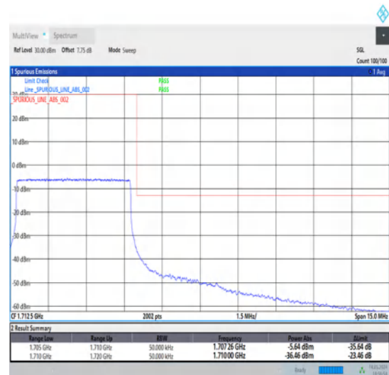
1-N70-15-5-H-6-CP-QPSK-Outer_Full-25@0- Ant1-1-seegraph-PASS-see graph
