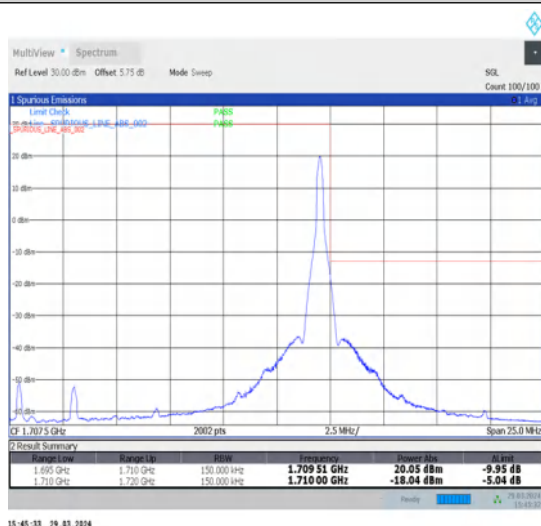
1-N70-15-15-H-5-CP-QPSK-Edge_1RB_Right-1@78-Ant1-1-seegraph-PASS-see graph
