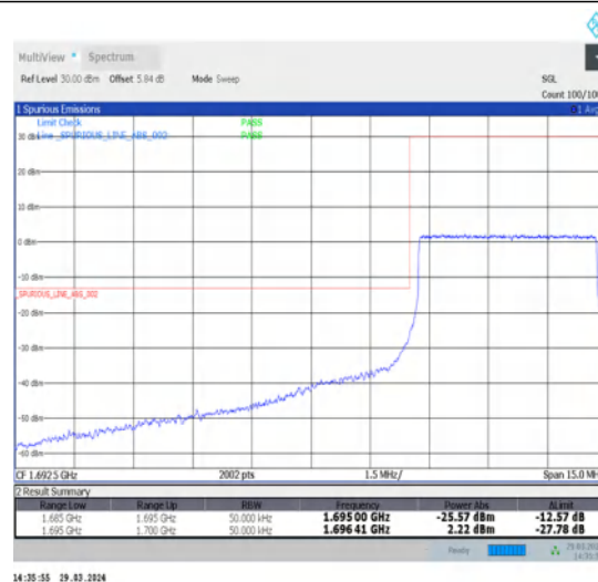
1-N70-15-5-L-6-CP-QPSK-Outer_Full-25@0-Ant1-1-seegraph-PASS-see graph
