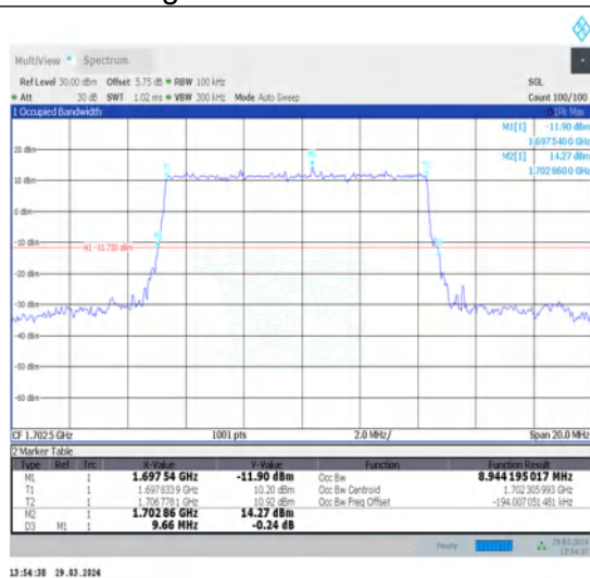
1-N70-15-10-M-1-DFT-QPSK-Out_Full-50@0-Ant1-8.944-9.660-≤10-PASS
