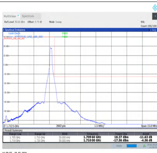
1-N70-15-5-H-2-DFT-PI2BPSK-Edge_1RB_Right-1@24-Ant1-1-seegraph-PASS-see graph
