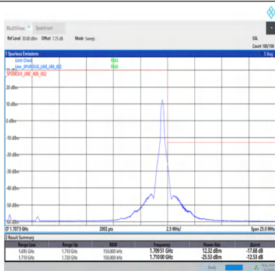
1-N70-15-15-H-5-CP-QPSK-Edge_1RB_Right-1@78-Ant1-1-seegraph-PASS-see graph
