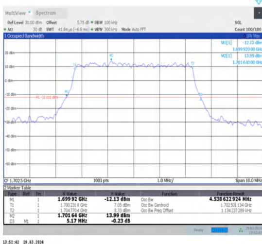
1-N70-15-5-M-7-CP-16QAM-Outer_Full-25@0-Ant1-4.539-5.170-≤5-PASS
