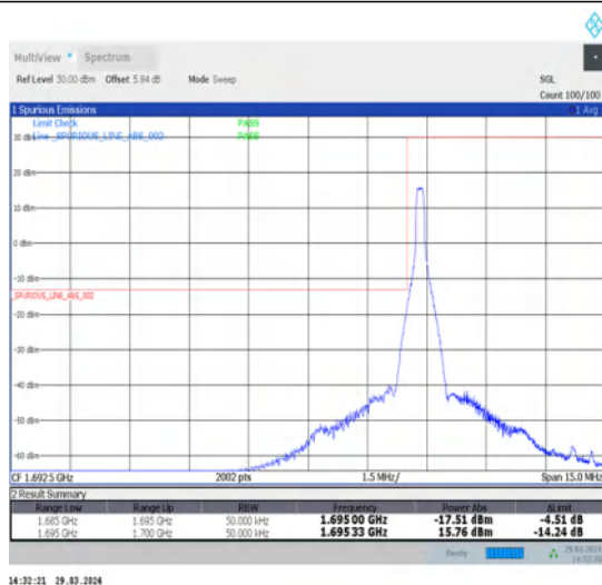
1-N70-15-5-L-4-CP-QPSK-Edge_1RB_Left-1@0-Ant1-1-seegraph-PASS-see graph
