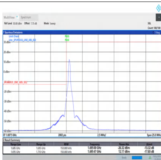
1-N70-15-15-L-4-CP-QPSK-Edge_1RB_Left-1@0-Ant1-1-seegraph-PASS-see graph
