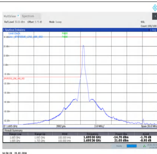
1-N70-15-10-L-1-DFT-PI2BPSK-Edge_1RB_Left-1@0-Ant1-1-seegraph-PASS-see graph
