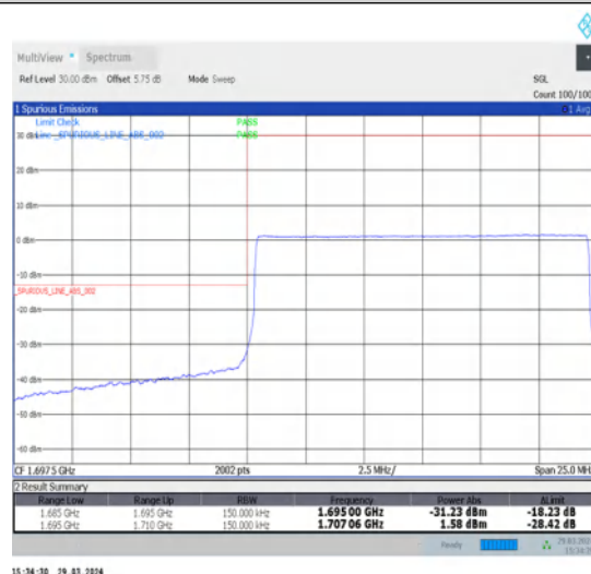
1-N70-15-15-L-6-CP-QPSK-Outer_Full-79@0-Ant1-1-seegraph-PASS-see graph
