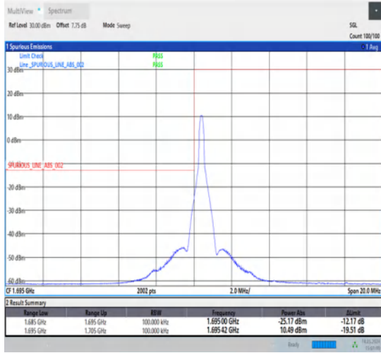
1-N70-15-10-L-4-CP-QPSK-Edge_1RB_Left-1@0-Ant1-1-seegraph-PASS-see graph
