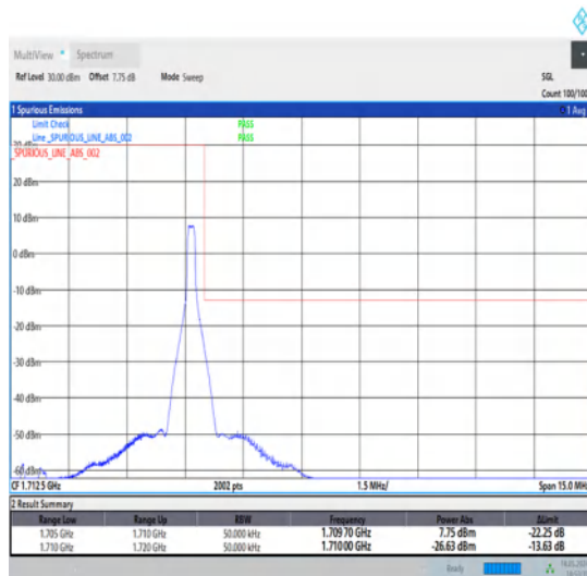
1-N70-15-5-H-5-CP-QPSK-Edge_1RB_Right-1@24- Ant1-1-seegraph-PASS-see graph
