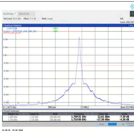
1-N70-15-15-H-2-DFT-PI2BPSK-Edge_1RB_Right-1@78-Ant1-1-seegraph-PASS-see graph
