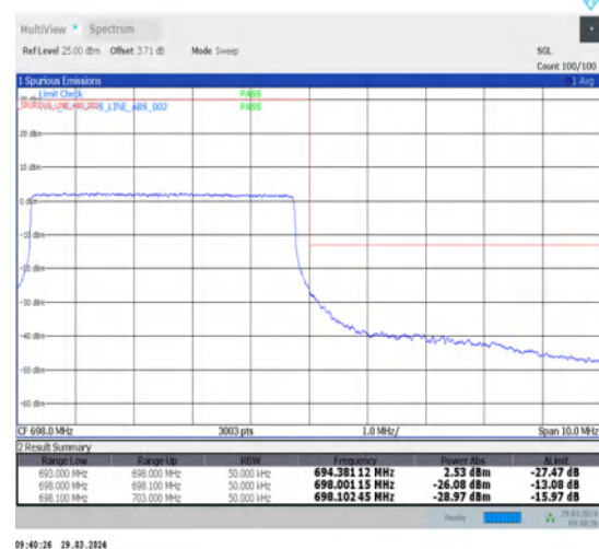
1-N71-15-5-H-6-CP-QPSK-Outer_Full-25@0-Ant1-1--PASS-see graph
