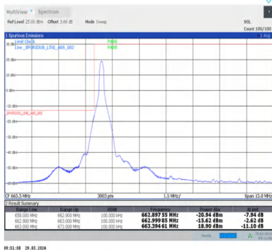
1-N71-15-10-L-4-CP-QPSK-Edge_1RB_Left-1@0-Ant1-1--PASS-see graph
