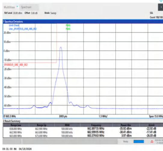
1-N71-15-10-L-1-DFT-PI2BPSK-Edge_1RB_Left-1@0-Ant1-1--PASS-see graph
