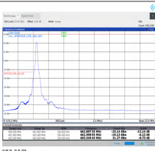
1-N71-15-20-L-4-CP-QPSK-Edge_1RB_Left-1@0-Ant1-1--PASS-see graph
