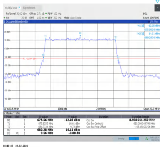
1-N71-15-10-M-3-DFT-16QAM-Outer_Full-50@0- Ant1-8.938-9.560-≤10-PASS
