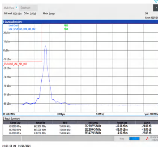
1-N71-15-15-L-4-CP-QPSK-Edge_1RB_Left-1@0-Ant1-1--PASS-see graph
