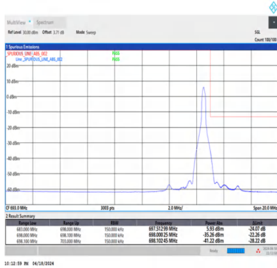
1-N71-15-15-H-2-DFT-PI2BPSK-Edge_1RB_Right-1@78-Ant1-1--PASS-see graph
