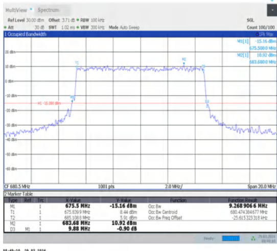
1-N71-15-10-M-8-CP-64QAM-Outer_Full-52@0- Ant1-9.269-9.880-≤10-PASS
