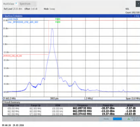
1-N71-15-10-L-1-DFT-PI2BPSK-Edge_1RB_Left-1@0-Ant1-1--PASS-see graph
