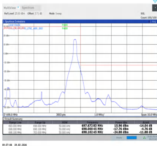
1-N71-15-5-H-5-CP-QPSK-Edge_1RB_Right-1@24-Ant1-1--PASS-see graph
