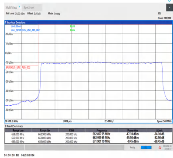
1-N71-15-20-L-3-DFT-PI2BPSK-Outer_Full-100@0-Ant1-1--PASS-see graph
