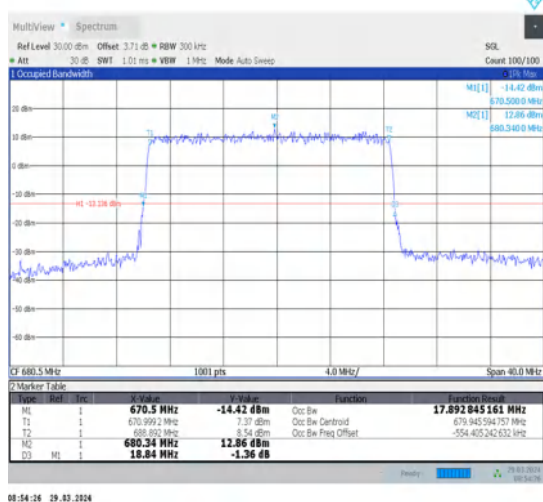
1-N71-15-20-M-5-DFT-256QAM-Outer_Full-100@0-Ant1-17.893-18.840-≤20-PASS
