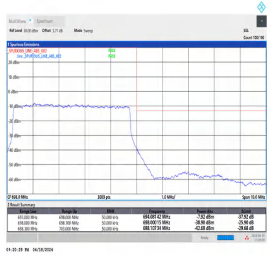
1-N71-15-5-H-3-DFT-PI2BPSK-Outer_Full-25@0-Ant1-1--PASS-see graph
