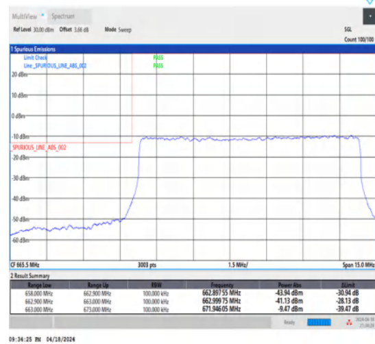
1-N71-15-10-L-3-DFT-PI2BPSK-Outer_Full-50@0-Ant1-1--PASS-see graph
