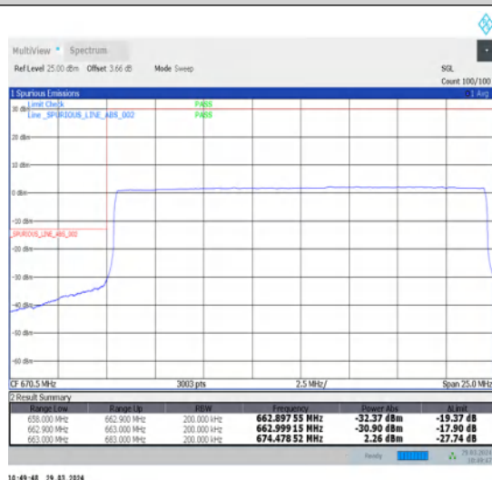
1-N71-15-20-L-6-CP-QPSK-Outer_Full-106@0-Ant1-1--PASS-see graph
