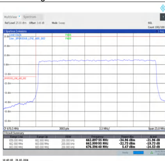
1-N71-15-20-L-3-DFT-PI2BPSK-Outer_Full-100@0-Ant1-1--PASS-see graph
