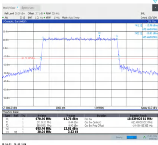
1-N71-15-20-M-8-CP-64QAM-Outer_Full-106@0-Ant1-18.939-20.040-≤20-PASS
