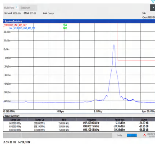
1-N71-15-15-H-5-CP-QPSK-Edge_1RB_Right-1@78-Ant1-1--PASS-see graph
