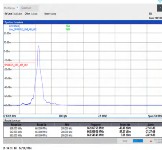
1-N71-15-20-L-4-CP-QPSK-Edge_1RB_Left-1@0-Ant1-1--PASS-see graph
