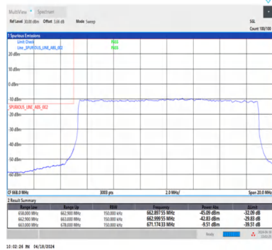
1-N71-15-15-L-3-DFT-PI2BPSK-Outer_Full-75@0-Ant1-1--PASS-see graph
