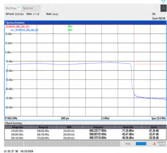
1-N71-15-20-H-6-CP-QPSK-Outer_Full-106@0-Ant1-1--PASS-see graph
