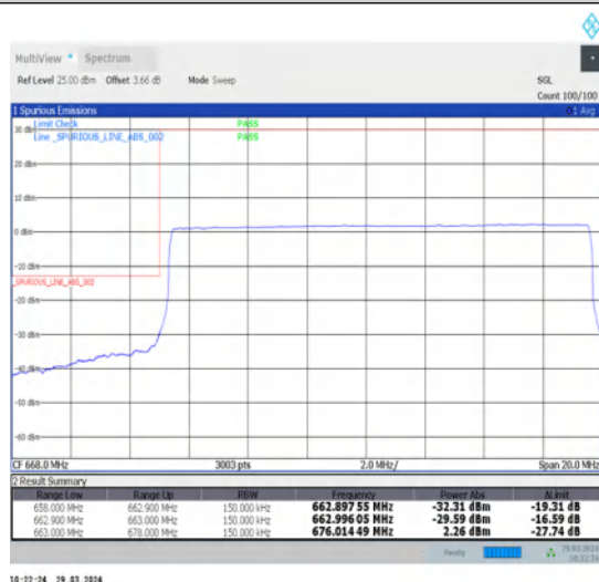
1-N71-15-15-L-6-CP-QPSK-Outer_Full-79@0-Ant1-1--PASS-see graph
