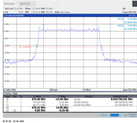
1-N71-15-10-M-1-DFT-QPSK-Outer_Full-50@0- Ant1-8.926-9.660-≤10-PASS
