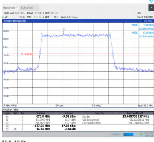
1-N71-15-15-M-1-DFT-QPSK-Outer_Full-75@0- Ant1-13.469-14.340-≤15-PASS
