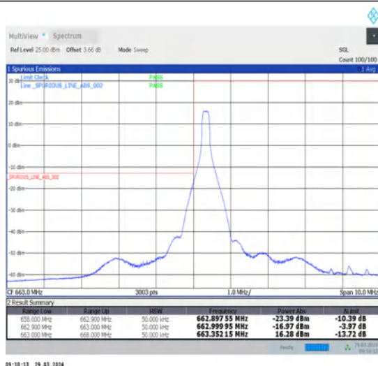
1-N71-15-5-L-4-CP-QPSK-Edge_1RB_Left-1@0-Ant1-1--PASS-see graph
