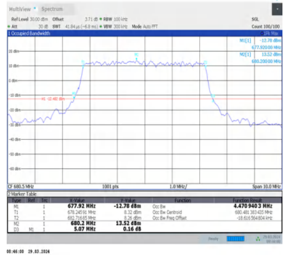
1-N71-15-5-M-6-CP-QPSK-Outer_Full-25@0-Ant1-4.471-5.070-≤5-PASS
