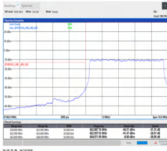
1-N71-15-5-L-3-DFT-PI2BPSK-Outer_Full-25@0-Ant1-1--PASS-see graph
