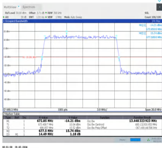
1-N71-15-15-M-4-DFT-64QAM-Outer_Full-75@0-Ant1-13.448-14.490-≤15-PASS
