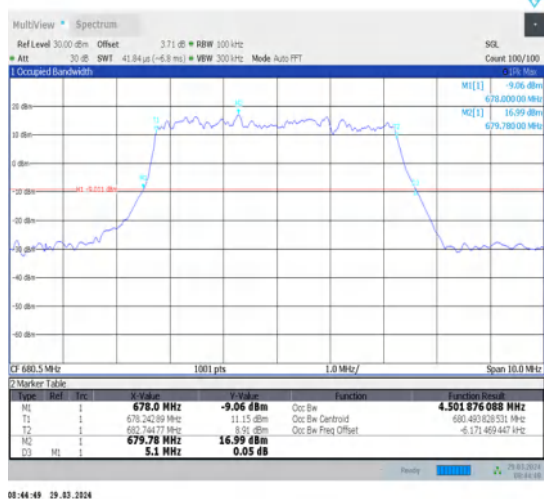
1-N71-15-5-M-1-DFT-QPSK-Outer_Full-25@0-Ant1-4.502-5.100-≤5-PASS
