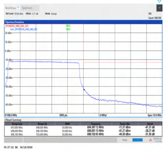
1-N71-15-5-H-6-CP-QPSK-Outer_Full-25@0-Ant1-1--PASS-see graph
