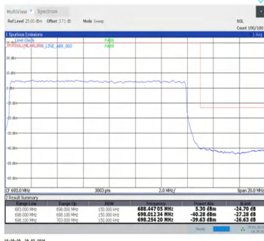
1-N71-15-15-H-3-DFT-PI2BPSK-Outer_Full-75@0-Ant1-1--PASS-see graph
