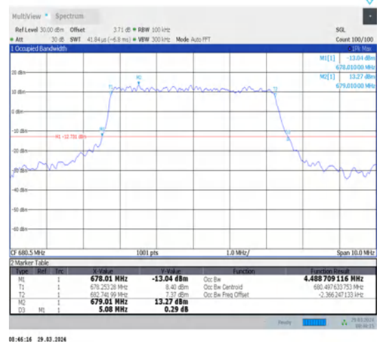
1-N71-15-5-M-8-CP-64QAM-Outer_Full-25@0-Ant1-4.489-5.080-≤5-PASS
