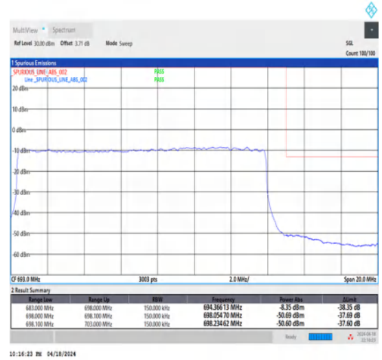
1-N71-15-15-H-3-DFT-PI2BPSK-Outer_Full-75@0-Ant1-1--PASS-see graph
