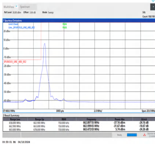
1-N71-15-15-L-1-DFT-PI2BPSK-Edge_1RB_Left-1@0-Ant1-1--PASS-see graph
