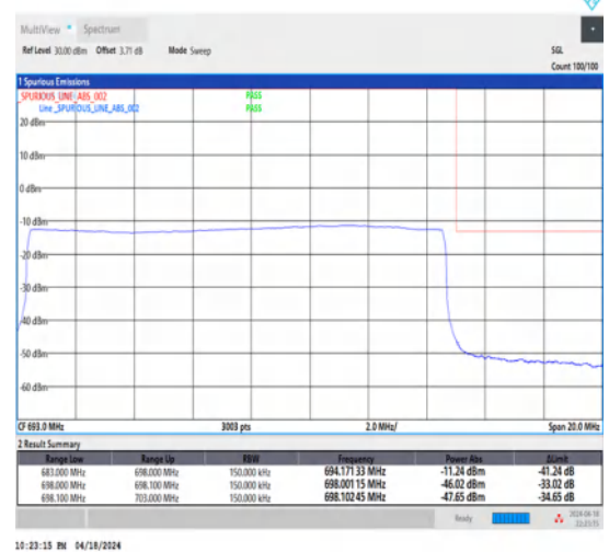
1-N71-15-15-H-6-CP-QPSK-Outer_Full-79@0-Ant1-1--PASS-see graph
