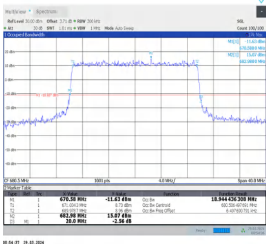
1-N71-15-20-M-6-CP-QPSK-Outer_Full-106@0-Ant1-18.944-20.000-≤20-PASS
