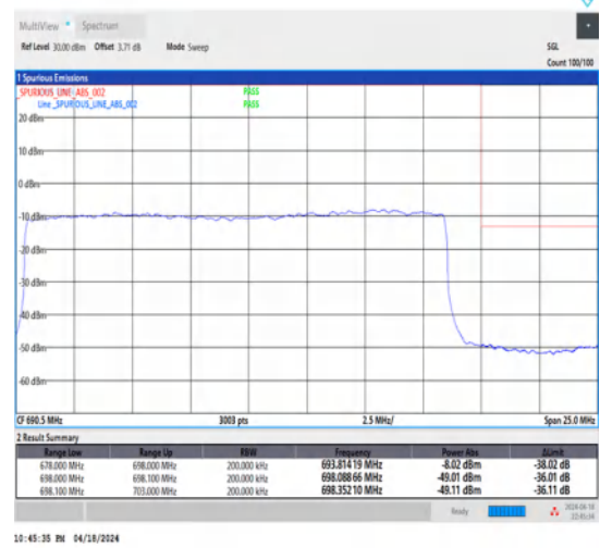
1-N71-15-20-H-3-DFT-PI2BPSK-Outer_Full-100@0-Ant1-1--PASS-see graph
