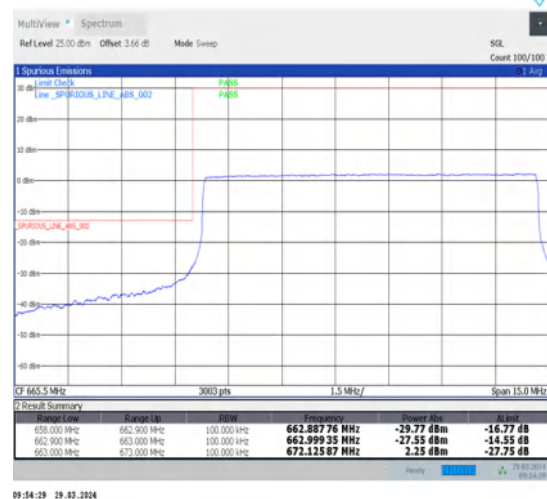
1-N71-15-10-L-6-CP-QPSK-Outer_Full-52@0-Ant1-1--PASS-see graph
