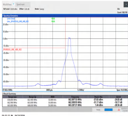
1-N71-15-5-L-1-DFT-PI2BPSK-Edge_1RB_Left-1@0-Ant1-1--PASS-see graph
