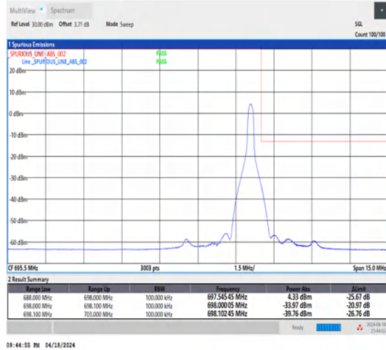
1-N71-15-10-H-2-DFT-PI2BPSK-Edge_1RB_Right-1@51-Ant1-1--PASS-see graph
