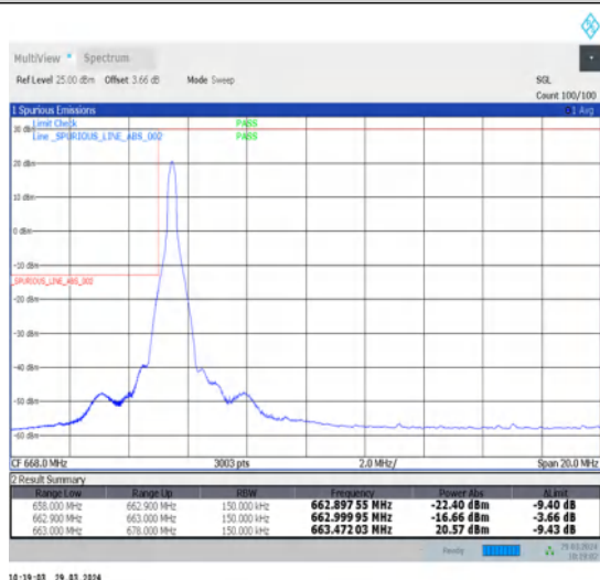
1-N71-15-15-L-4-CP-QPSK-Edge_1RB_Left-1@0-Ant1-1--PASS-see graph
