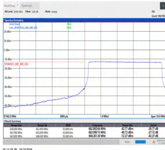
1-N71-15-5-L-6-CP-QPSK-Outer_Full-25@0-Ant1-1--PASS-see graph
