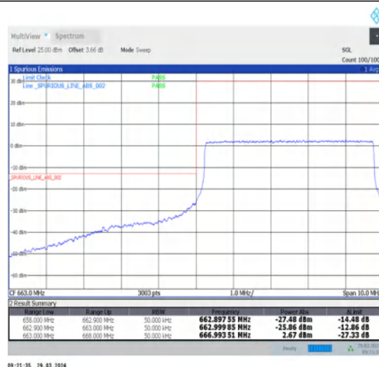
1-N71-15-5-L-6-CP-QPSK-Outer_Full-25@0-Ant1-1--PASS-see graph
