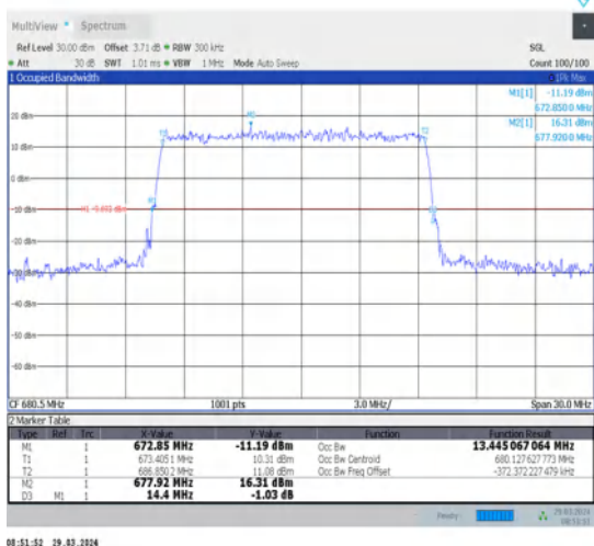
1-N71-15-15-M-3-DFT-16QAM-Outer_Full-75@0-Ant1-13.445-14.400-≤15-PASS
