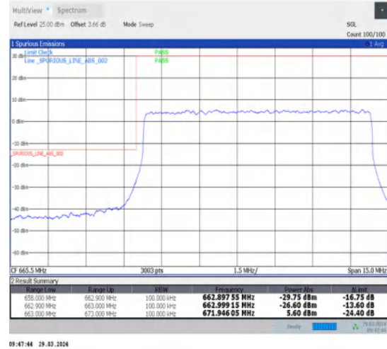
1-N71-15-10-L-3-DFT-PI2BPSK-Outer_Full-50@0-Ant1-1--PASS-see graph
