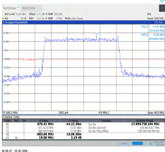
1-N71-15-20-M-4-DFT-64QAM-Outer_Full-100@0-Ant1-17.896-19.080-≤20-PASS
