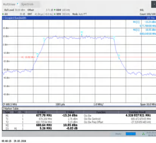
1-N71-15-5-M-9-CP-256QAM-Outer_Full-25@0- Ant1-4.527-5.260-≤5-PASS
