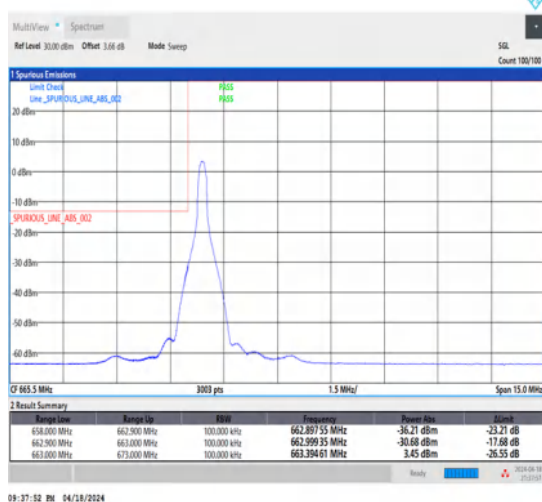
1-N71-15-10-L-4-CP-QPSK-Edge_1RB_Left-1@0-Ant1-1--PASS-see graph
