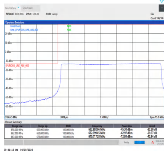
1-N71-15-10-L-6-CP-QPSK-Outer_Full-52@0-Ant1-1--PASS-see graph
