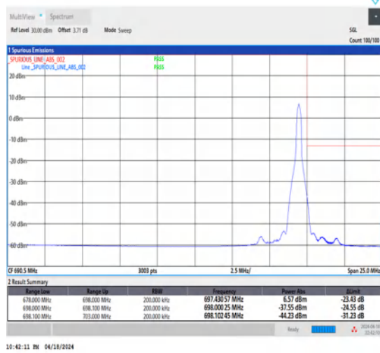
1-N71-15-20-H-2-DFT-PI2BPSK-Edge_1RB_Right-1@105-Ant1-1--PASS-see graph
