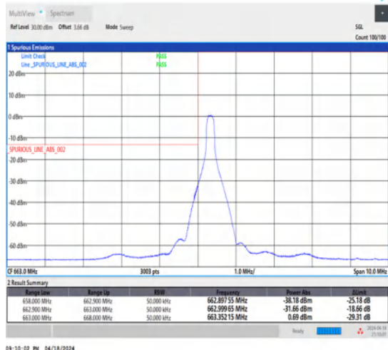
1-N71-15-5-L-4-CP-QPSK-Edge_1RB_Left-1@0-Ant1-1--PASS-see graph
