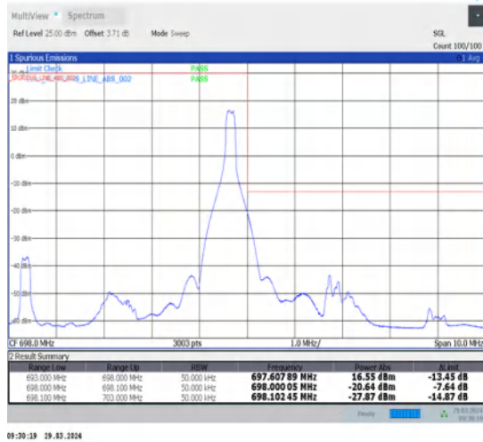
1-N71-15-5-H-2-DFT-PI2BPSK-Edge_1RB_Right-1@24-Ant1-1--PASS-see graph
