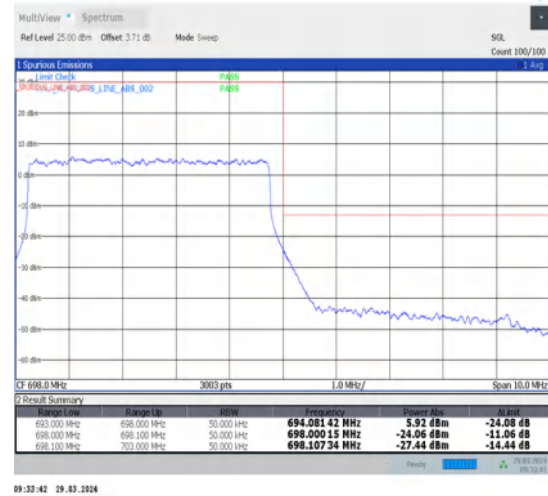
1-N71-15-5-H-3-DFT-PI2BPSK-Outer_Full-25@0-Ant1-1--PASS-see graph
