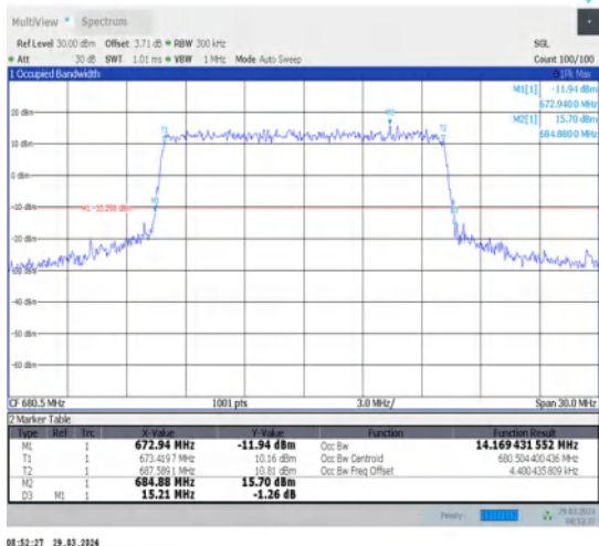
1-N71-15-15-M-7-CP-16QAM-Outer_Full-79@0-Ant1-14.169-15.210-≤15-PASS
