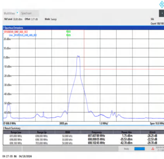
1-N71-15-5-H-2-DFT-PI2BPSK-Edge_1RB_Right-1@24-Ant1-1--PASS-see graph
