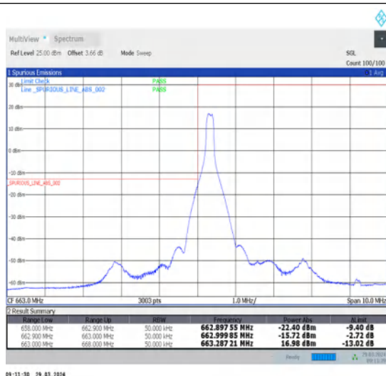
1-N71-15-5-L-1-DFT-PI2BPSK-Edge_1RB_Left-1@0-Ant1-1--PASS-see graph
