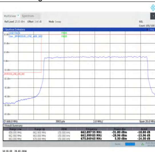
1-N71-15-15-L-3-DFT-PI2BPSK-Outer_Full-75@0-Ant1-1--PASS-see graph
