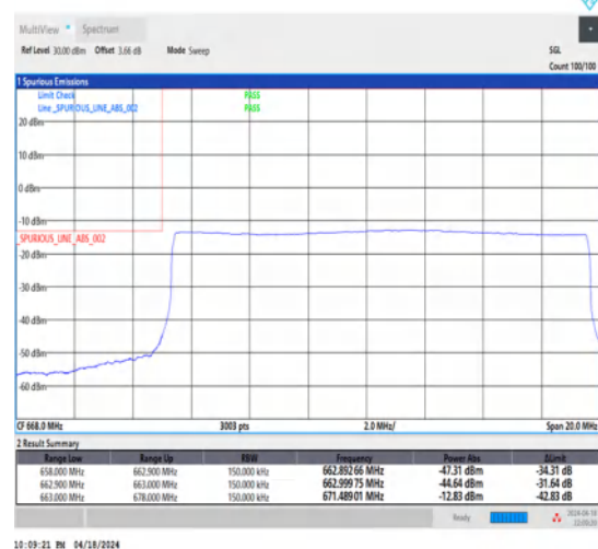
1-N71-15-15-L-6-CP-QPSK-Outer_Full-79@0-Ant1-1--PASS-see graph
