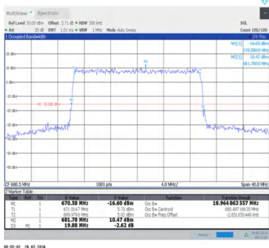
1-N71-15-20-M-9-CP-256QAM-Outer_Full-106@0-Ant1-18.965-19.880-≤20-PASS
