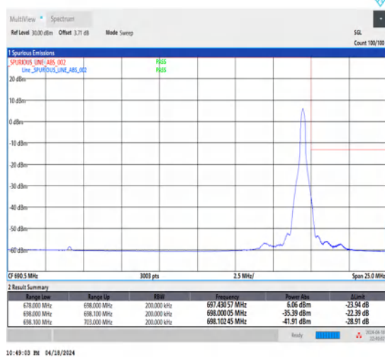
1-N71-15-20-H-5-CP-QPSK-Edge_1RB_Right-1@105-Ant1-1--PASS-see graph
