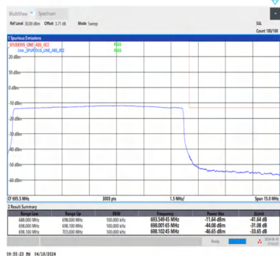
1-N71-15-10-H-6-CP-QPSK-Outer_Full-52@0-Ant1-1--PASS-see graph
