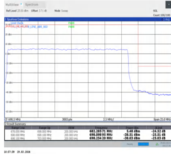
1-N71-15-20-H-3-DFT-PI2BPSK-Outer_Full-100@0-Ant1-1--PASS-see graph
