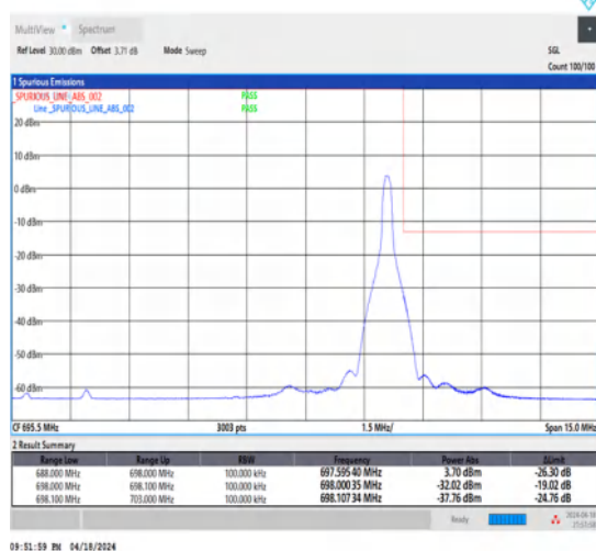
1-N71-15-10-H-5-CP-QPSK-Edge_1RB_Right-1@51-Ant1-1--PASS-see graph
