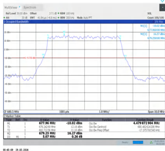
1-N71-15-5-M-2-DFT-PI2BPSK-Outer_Full-25@0-Ant1-4.48-5.070-≤5-PASS
