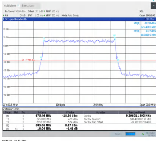
1-N71-15-10-M-9-CP-256QAM-Outer_Full-52@0- Ant1-9.296-10.040-≤10-PASS
