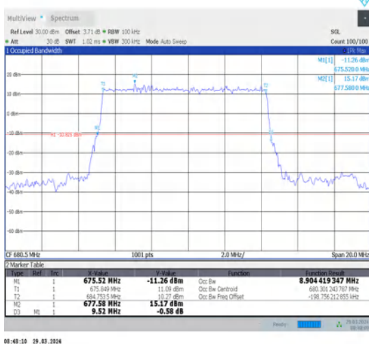
1-N71-15-10-M-2-DFT-PI2BPSK-Outer_Full-50@0- Ant1-8.904-9.520-≤10-PASS
