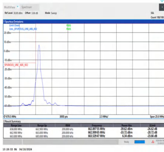
1-N71-15-20-L-1-DFT-PI2BPSK-Edge_1RB_Left-1@0-Ant1-1--PASS-see graph
