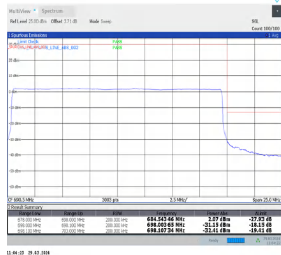
1-N71-15-20-H-6-CP-QPSK-Outer_Full-106@0-Ant1-1--PASS-see graph
