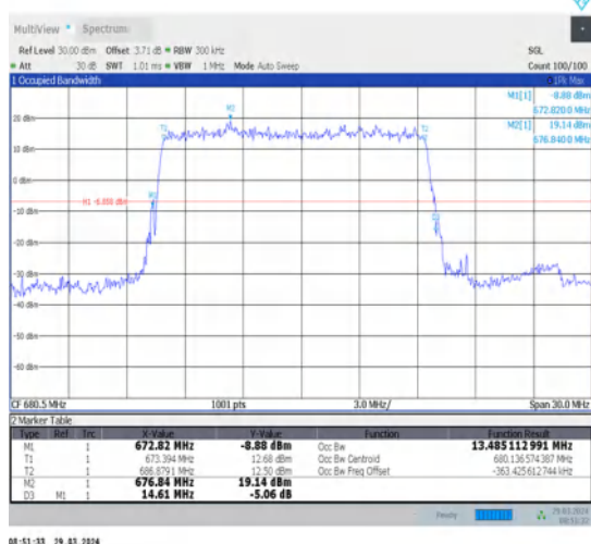
1-N71-15-15-M-2-DFT-PI2BPSK-Outer_Full-75@0- Ant1-13.485-14.610-≤15-PASS
