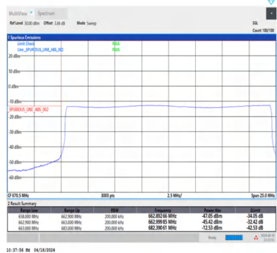
1-N71-15-20-L-6-CP-QPSK-Outer_Full-106@0-Ant1-1--PASS-see graph
