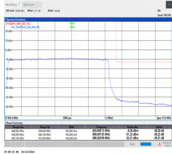
1-N71-15-10-H-3-DFT-PI2BPSK-Outer_Full-50@0-Ant1-1--PASS-see graph
