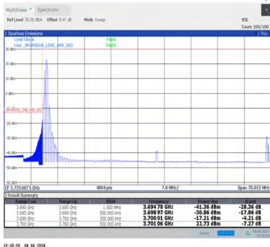
1-N77-3700-3980-30-60-L-1-DFT-PI2BPSK-Edge_1RB_Left-1@0-Ant1-1--PASS-see graph
