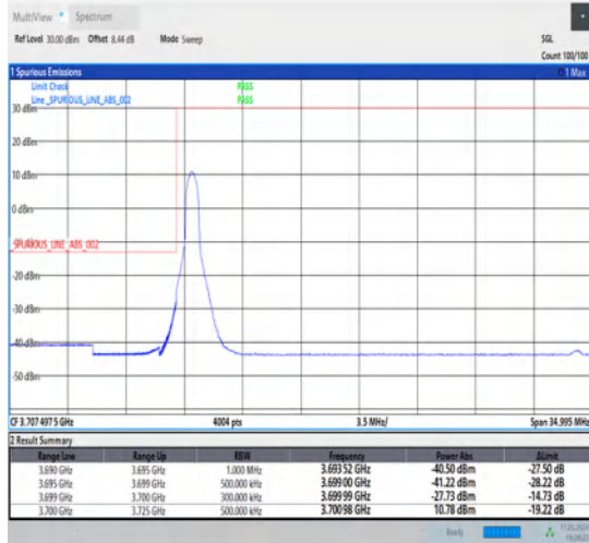
1-N77-3700-3980-30-25-L-1-DFT-PI2BPSK-Edge_1RB_Left-1@0-Ant1-1--PASS-see graph
