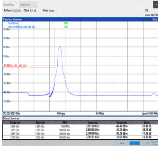
1-N77-3700-3980-30-20-L-1-DFT-PI2BPSK-Edge_1RB_Left-1@0-Ant1-1--PASS-see graph
