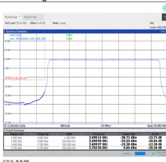
1-N77-3700-3980-30-30-L-3-DFT-PI2BPSK-Outer_Full-75@0-Ant1-1--PASS-see graph
