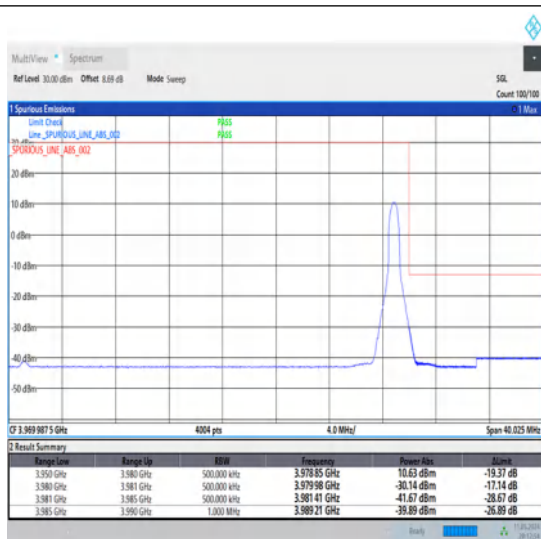
1-N77-3700-3980-30-30-H-2-DFT-PI2BPSK-Edge_1RB_Right-1@77-Ant1-1--PASS-see graph
