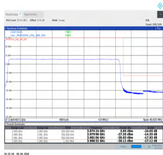
1-N77-3700-3980-30-30-H-6-CP-QPSK-Outer_Full-78@0-Ant1-1--PASS-see graph
