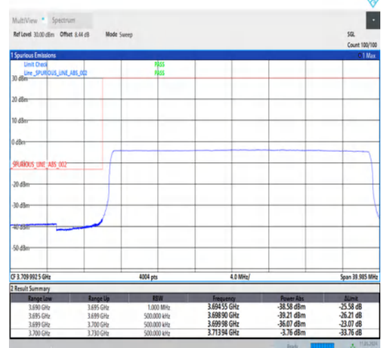
1-N77-3700-3980-30-30-L-6-CP-QPSK-Outer_Full-78@0-Ant1-1--PASS-see graph
