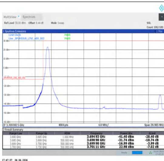
1-N77-3700-3980-30-30-L-1-DFT-PI2BPSK-Edge_1RB_Left-1@0-Ant1-1--PASS-see graph
