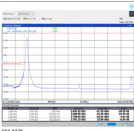
1-N77-3700-3980-30-50-L-1-DFT-PI2BPSK-Edge_1RB_Left-1@0-Ant1-1--PASS-see graph
