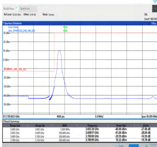
1-N77-3700-3980-30-20-L-4-CP-QPSK-Edge_1RB_Left-1@0-Ant1-1--PASS-see graph
