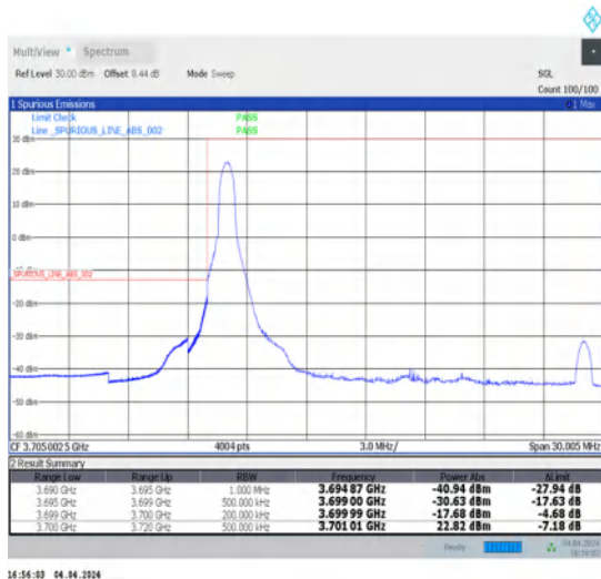
1-N77-3700-3980-30-20-L-4-CP-QPSK-Edge_1RB_Left-1@0-Ant1-1--PASS-see graph
