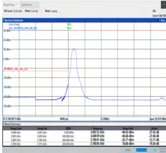
1-N77-3700-3980-30-15-L-1-DFT-PI2BPSK-Edge_1RB_Left-1@0-Ant1-1--PASS-see graph
