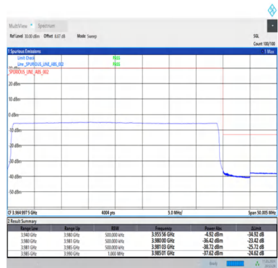
1-N77-3700-3980-30-40-H-6-CP-QPSK-Outer_Full-106@0-Ant1-1--PASS-see graph
