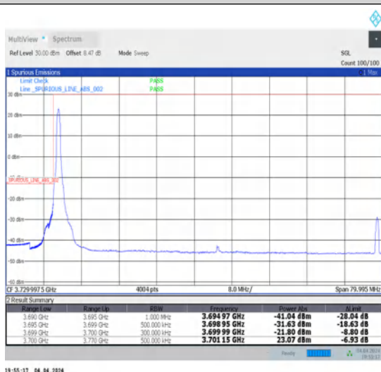
1-N77-3700-3980-30-70-L-4-CP-QPSK-Edge_1RB_Left-1@0-Ant1-1--PASS-see graph
