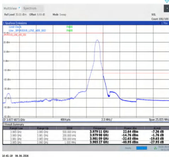
1-N77-3700-3980-30-15-H-5-CP-QPSK-Edge_1RB_Right-1@37-Ant1-1--PASS-see graph
