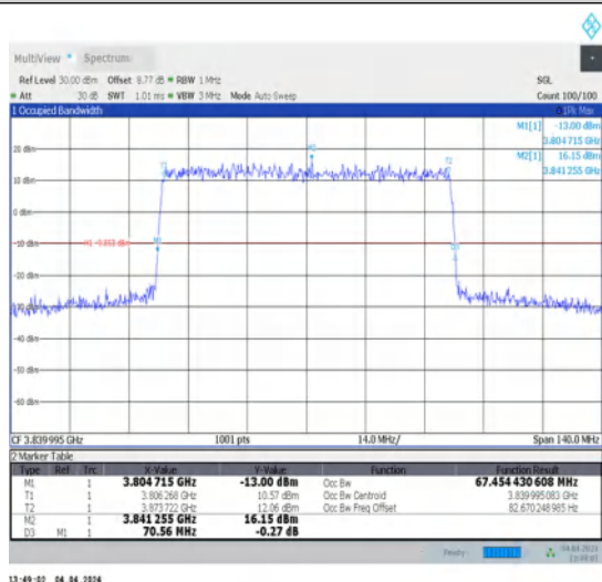
1-N77-3700-3980-30-70-M-6-CP-QPSK-Outer_Full-189@0-Ant1-67.454-70.560-≤70-PASS
