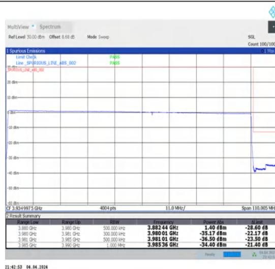
1-N77-3700-3980-30-100-H-6-CP-QPSK-Outer_Full-273@0-Ant1-1--PASS-see graph
