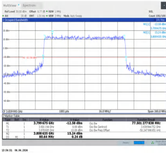
1-N77-3700-3980-30-80-M-7-CP-16QAM-Outer_Full-217@0-Ant1-77.501-80.640-≤80-PASS
