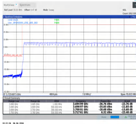
1-N77-3700-3980-30-60-L-3-DFT-PI2BPSK-Outer_Full-162@0-Ant1-1--PASS-see graph
