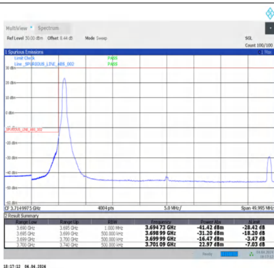
1-N77-3700-3980-30-40-L-1-DFT-PI2BPSK-Edge_1RB_Left-1@0-Ant1-1--PASS-see graph
