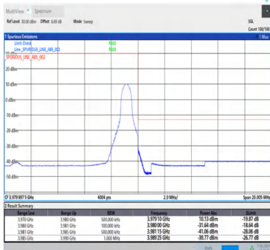
1-N77-3700-3980-30-10-H-5-CP-QPSK-Edge_1RB_Right-1@23-Ant1-1--PASS-see graph
