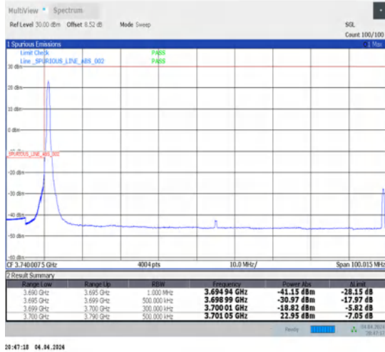
1-N77-3700-3980-30-90-L-1-DFT-PI2BPSK-Edge_1RB_Left-1@0-Ant1-1--PASS-see graph
