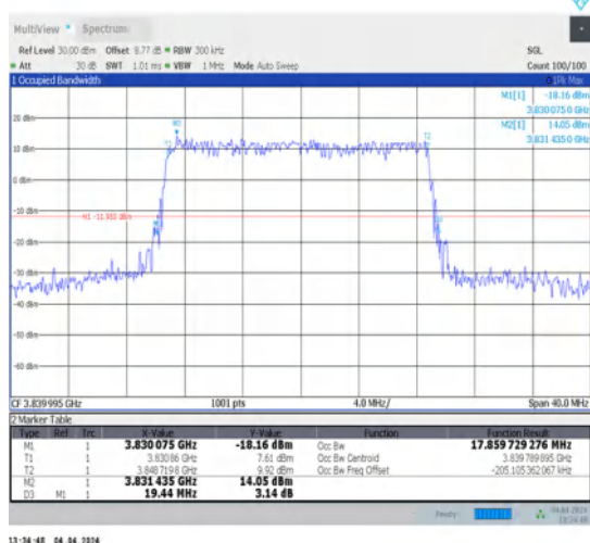
1-N77-3700-3980-30-20-M-5-DFT-256QAM-Outer_Full-50@0-Ant1-17.86-19.440-≤20-PASS
