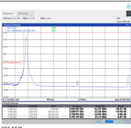
1-N77-3700-3980-30-50-L-4-CP-QPSK-Edge_1RB_Left-1@0-Ant1-1--PASS-see graph
