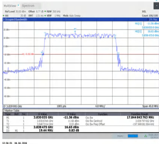
1-N77-3700-3980-30-20-M-3-DFT-16QAM-Outer_Full-50@0-Ant1-17.845-19.440-≤20-PASS
