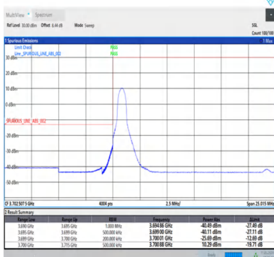
1-N77-3700-3980-30-15-L-4-CP-QPSK-Edge_1RB_Left-1@0-Ant1-1--PASS-see graph
