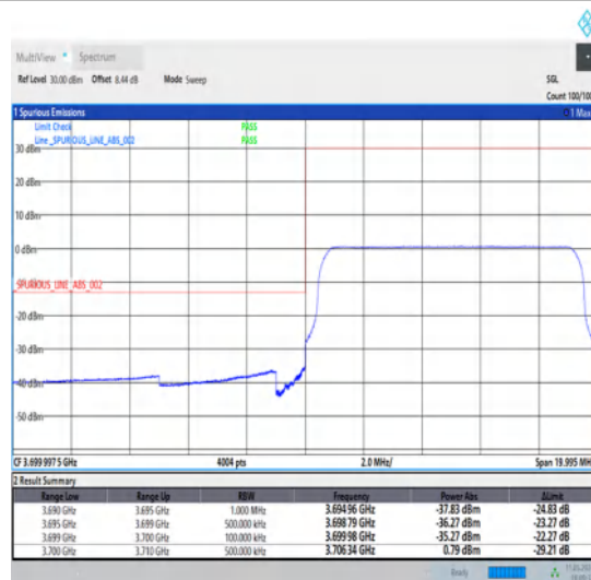
1-N77-3700-3980-30-10-L-6-CP-QPSK-Outer_Full-24@0-Ant1-1--PASS-see graph
