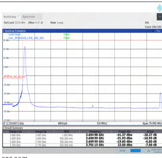
1-N77-3700-3980-30-70-L-1-DFT-PI2BPSK-Edge_1RB_Left-1@0-Ant1-1--PASS-see graph
