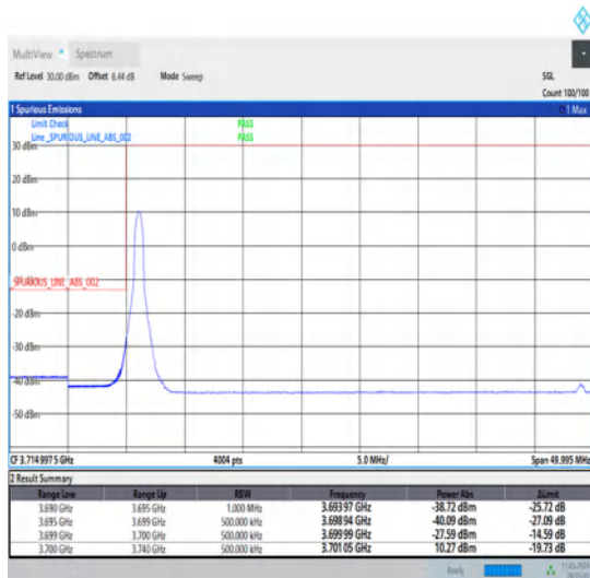
1-N77-3700-3980-30-40-L-4-CP-QPSK-Edge_1RB_Left-1@0-Ant1-1--PASS-see graph
