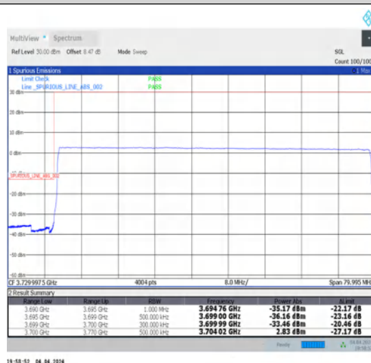
1-N77-3700-3980-30-70-L-6-CP-QPSK-Outer_Full-189@0-Ant1-1--PASS-see graph
