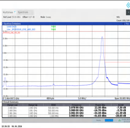
1-N77-3700-3980-30-40-H-2-DFT-PI2BPSK-Edge_1RB_Right-1@105-Ant1-1--PASS-see graph
