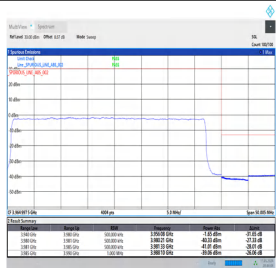
1-N77-3700-3980-30-40-H-3-DFT-PI2BPSK-Outer_Full-100@0-Ant1-1--PASS-see graph
