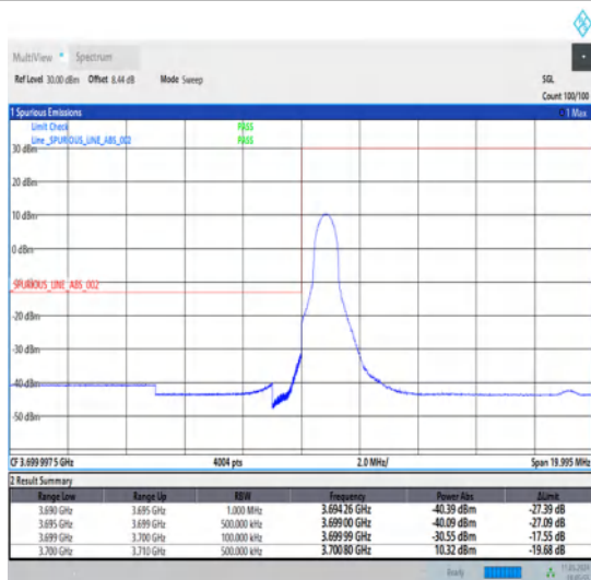
1-N77-3700-3980-30-10-L-4-CP-QPSK-Edge_1RB_Left-1@0-Ant1-1--PASS-see graph
