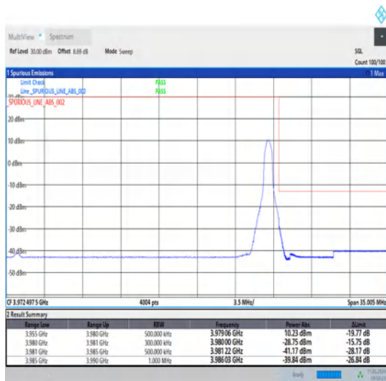
1-N77-3700-3980-30-25-H-5-CP-QPSK-Edge_1RB_Right-1@64-Ant1-1--PASS-see graph
