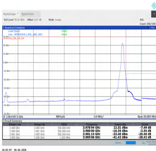
1-N77-3700-3980-30-40-H-5-CP-QPSK-Edge_1RB_Right-1@105-Ant1-1--PASS-see graph
