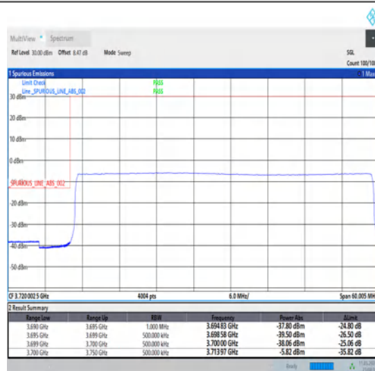
1-N77-3700-3980-30-50-L-6-CP-QPSK-Outer_Full-133@0-Ant1-1--PASS-see graph
