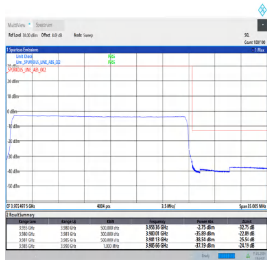
1-N77-3700-3980-30-25-H-6-CP-QPSK-Outer_Full-65@0-Ant1-1--PASS-see graph
