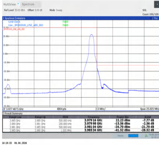
1-N77-3700-3980-30-15-H-2-DFT-PI2BPSK-Edge_1RB_Right-1@37-Ant1-1--PASS-see graph
