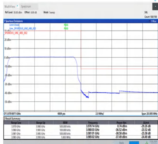
1-N77-3700-3980-30-10-H-6-CP-QPSK-Outer_Full-24@0-Ant1-1--PASS-see graph
