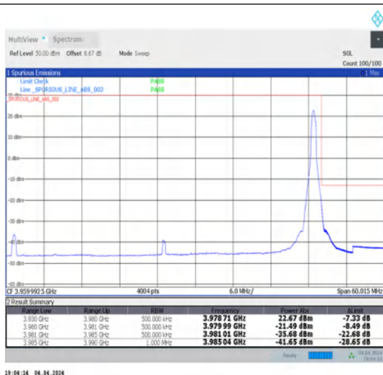
1-N77-3700-3980-30-50-H-2-DFT-PI2BPSK-Edge_1RB_Right-1@132-Ant1-1--PASS-see graph
