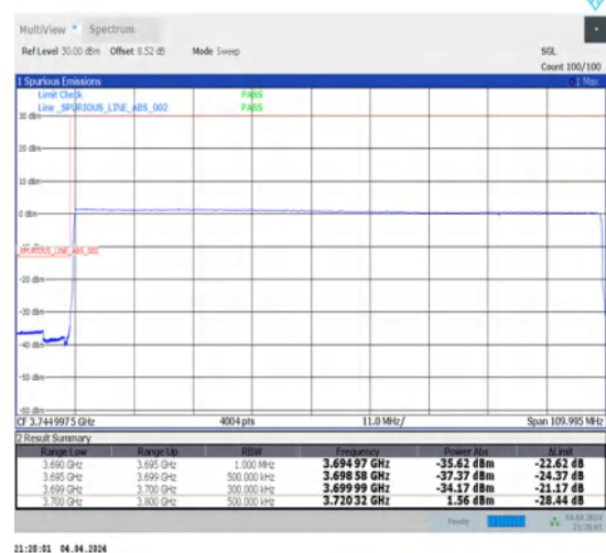
1-N77-3700-3980-30-100-L-6-CP-QPSK-Outer_Full-273@0-Ant1-1--PASS-see graph
