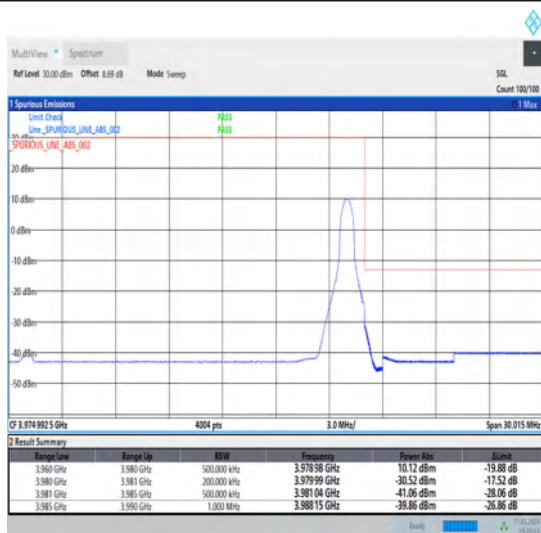
1-N77-3700-3980-30-20-H-5-CP-QPSK-Edge_1RB_Right-1@50-Ant1-1--PASS-see graph
