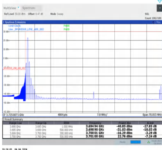
1-N77-3700-3980-30-60-L-4-CP-QPSK-Edge_1RB_Left-1@0-Ant1-1--PASS-see graph
