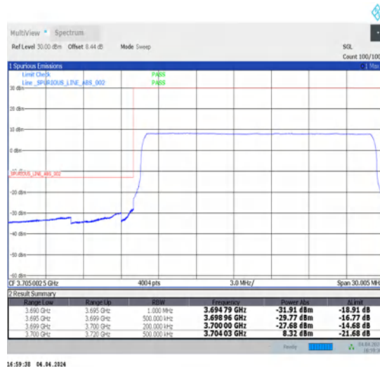
1-N77-3700-3980-30-20-L-6-CP-QPSK-Outer_Full-51@0-Ant1-1--PASS-see graph
