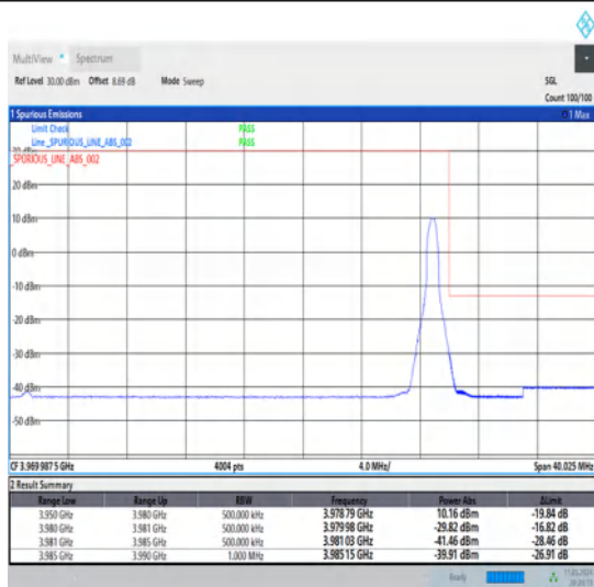
1-N77-3700-3980-30-30-H-5-CP-QPSK-Edge_1RB_Right-1@77-Ant1-1--PASS-see graph
