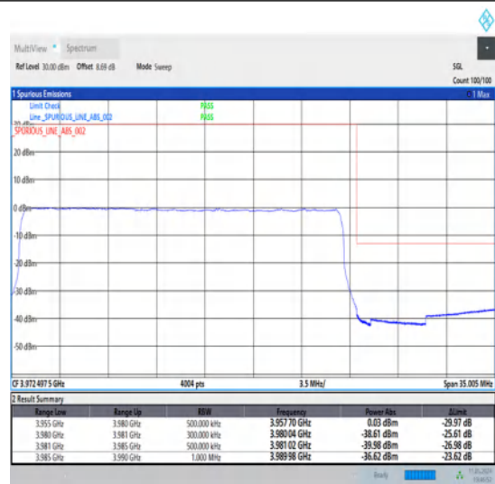
1-N77-3700-3980-30-25-H-3-DFT-PI2BPSK-Outer_Full-64@0-Ant1-1--PASS-see graph
