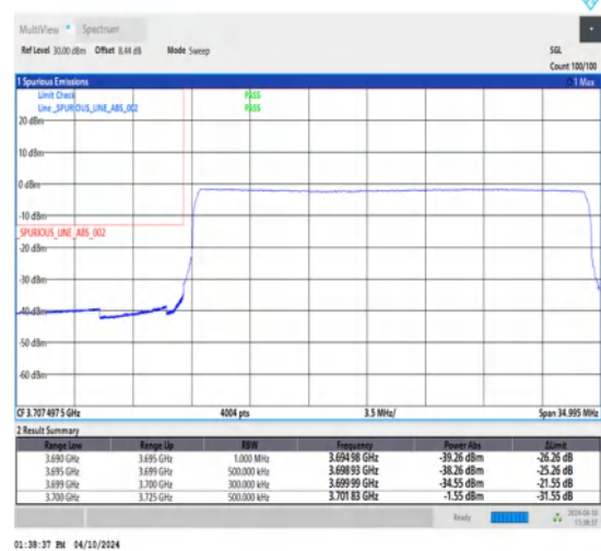
1-N77-3700-3980-30-25-L-6-CP-QPSK-Outer_Full-65@0-Ant1-1--PASS-see graph
