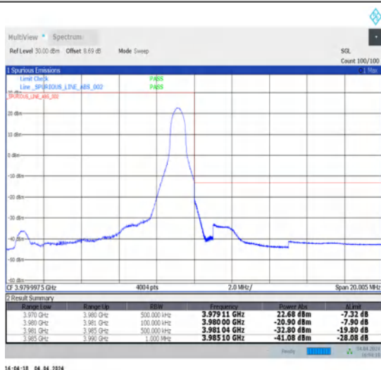
1-N77-3700-3980-30-10-H-5-CP-QPSK-Edge_1RB_Right-1@23-Ant1-1--PASS-see graph
