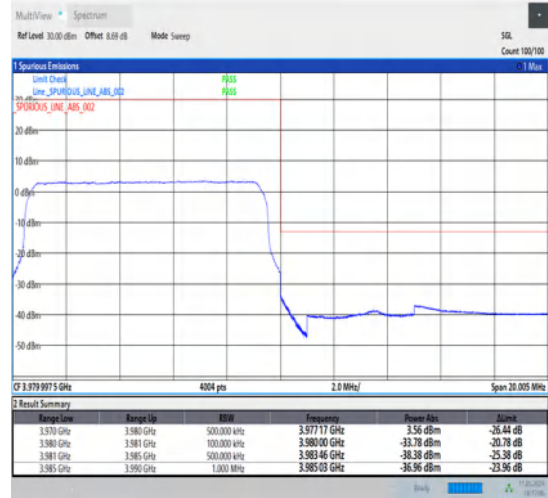
1-N77-3700-3980-30-10-H-3-DFT-PI2BPSK-Outer_Full-24@0-Ant1-1--PASS-see graph
