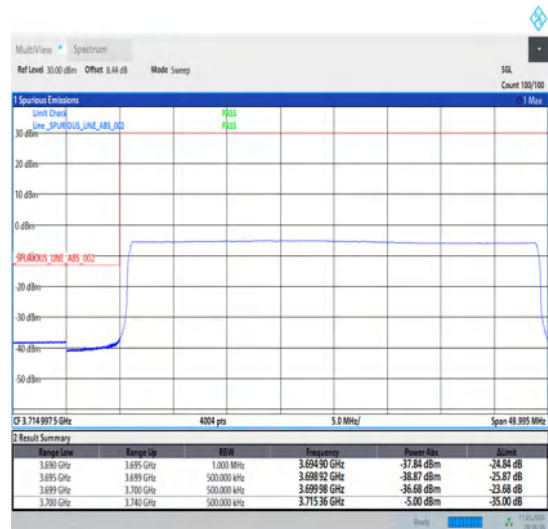
1-N77-3700-3980-30-40-L-6-CP-QPSK-Outer_Full-106@0-Ant1-1--PASS-see graph
