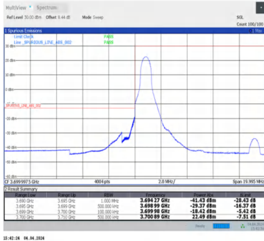
1-N77-3700-3980-30-10-L-1-DFT-PI2BPSK-Edge_1RB_Left-1@0-Ant1-1--PASS-see graph
