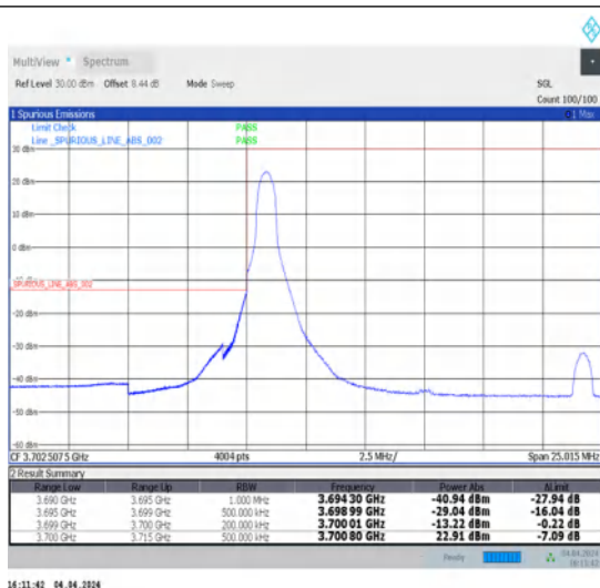
1-N77-3700-3980-30-15-L-1-DFT-PI2BPSK-Edge_1RB_Left-1@0-Ant1-1--PASS-see graph
