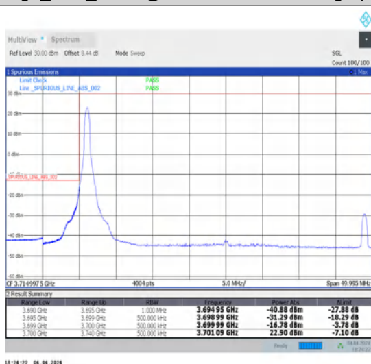
1-N77-3700-3980-30-40-L-4-CP-QPSK-Edge_1RB_Left-1@0-Ant1-1--PASS-see graph
