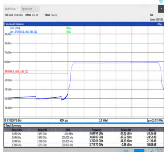
1-N77-3700-3980-30-15-L-6-CP-QPSK-Outer_Full-38@0-Ant1-1--PASS-see graph
