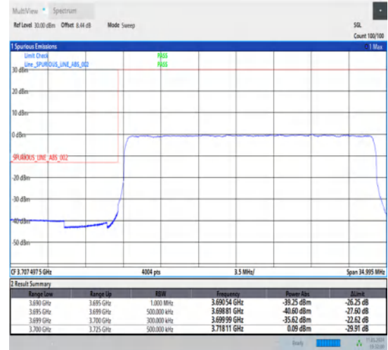
1-N77-3700-3980-30-25-L-3-DFT-PI2BPSK-Outer_Full-64@0-Ant1-1--PASS-see graph
