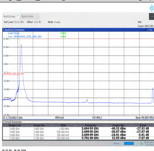
1-N77-3700-3980-30-80-L-4-CP-QPSK-Edge_1RB_Left-1@0-Ant1-1--PASS-see graph
