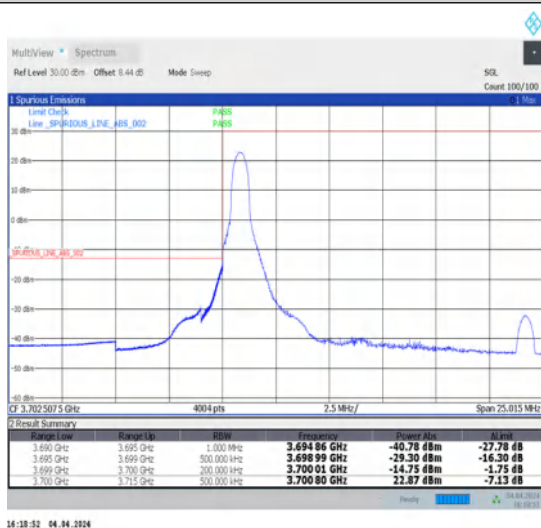
1-N77-3700-3980-30-15-L-4-CP-QPSK-Edge_1RB_Left-1@0-Ant1-1--PASS-see graph
