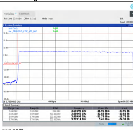
1-N77-3700-3980-30-80-L-3-DFT-PI2BPSK-Outer_Full-216@0-Ant1-1--PASS-see graph
