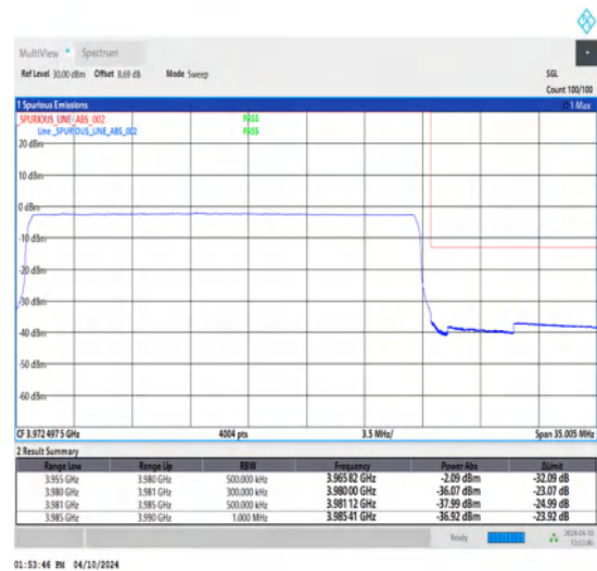
1-N77-3700-3980-30-25-H-6-CP-QPSK-Outer_Full-65@0-Ant1-1--PASS-see graph
