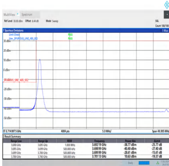
1-N77-3700-3980-30-40-L-1-DFT-PI2BPSK-Edge_1RB_Left-1@0-Ant1-1--PASS-see graph
