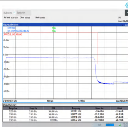
1-N77-3700-3980-30-30-H-6-CP-QPSK-Outer_Full-78@0-Ant1-1--PASS-see graph
