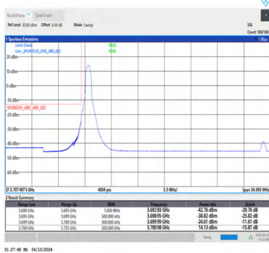
1-N77-3700-3980-30-25-L-1-DFT-PI2BPSK-Edge_1RB_Left-1@0-Ant1-1--PASS-see graph
