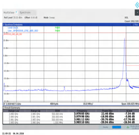
1-N77-3700-3980-30-90-H-5-CP-QPSK-Edge_1RB_Right-1@244-Ant1-1--PASS-see graph
