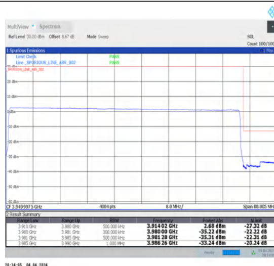
1-N77-3700-3980-30-70-H-6-CP-QPSK-Outer_Full-189@0-Ant1-1--PASS-see graph
