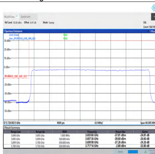
1-N77-3700-3980-30-50-L-3-DFT-PI2BPSK-Outer_Full-128@0-Ant1-1--PASS-see graph
