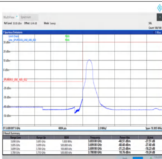
1-N77-3700-3980-30-10-L-1-DFT-PI2BPSK-Edge_1RB_Left-1@0-Ant1-1--PASS-see graph
