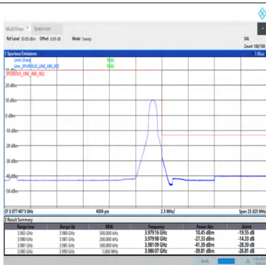
1-N77-3700-3980-30-15-H-2-DFT-PI2BPSK-Edge_1RB_Right-1@37-Ant1-1--PASS-see graph
