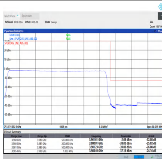
1-N77-3700-3980-30-20-H-6-CP-QPSK-Outer_Full-51@0-Ant1-1--PASS-see graph
