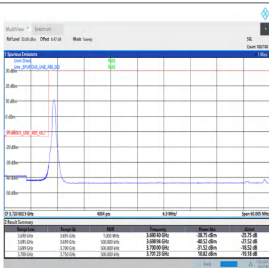
1-N77-3700-3980-30-50-L-1-DFT-PI2BPSK-Edge_1RB_Left-1@0-Ant1-1--PASS-see graph
