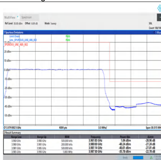
1-N77-3700-3980-30-20-H-3-DFT-PI2BPSK-Outer_Full-50@0-Ant1-1--PASS-see graph
