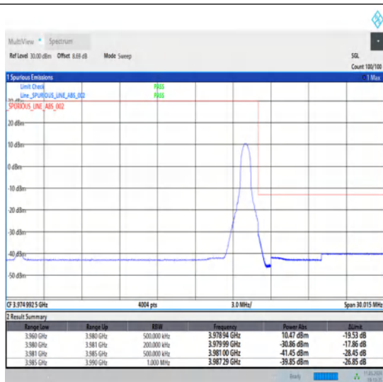
1-N77-3700-3980-30-20-H-2-DFT-PI2BPSK-Edge_1RB_Right-1@50-Ant1-1--PASS-see graph
