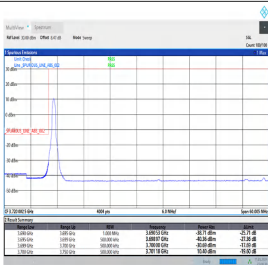
1-N77-3700-3980-30-50-L-4-CP-QPSK-Edge_1RB_Left-1@0-Ant1-1--PASS-see graph
