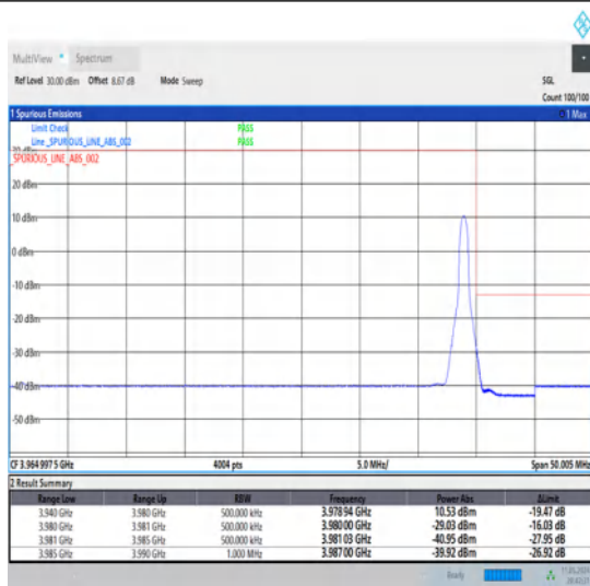
1-N77-3700-3980-30-40-H-2-DFT-PI2BPSK-Edge_1RB_Right-1@105-Ant1-1--PASS-see graph
