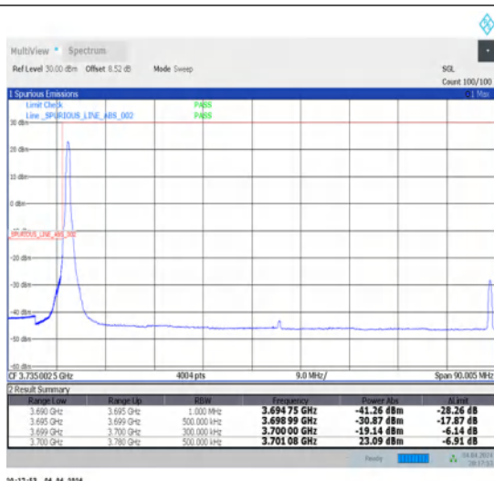
1-N77-3700-3980-30-80-L-1-DFT-PI2BPSK-Edge_1RB_Left-1@0-Ant1-1--PASS-see graph
