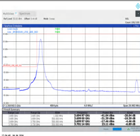
1-N77-3700-3980-30-30-L-4-CP-QPSK-Edge_1RB_Left-1@0-Ant1-1--PASS-see graph
