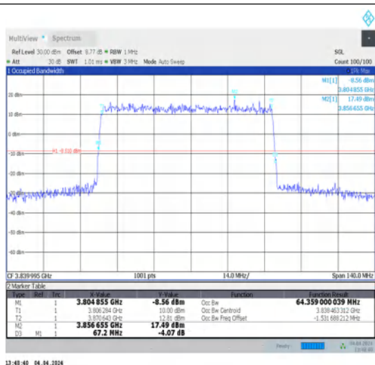
1-N77-3700-3980-30-70-M-4-DFT-64QAM-Outer_Full-180@0-Ant1-64.359-67.200-≤70-PASS
