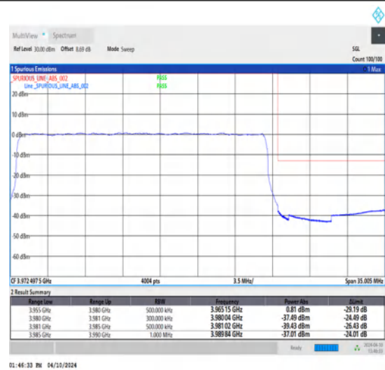
1-N77-3700-3980-30-25-H-3-DFT-PI2BPSK-Outer_Full-64@0-Ant1-1--PASS-see graph
