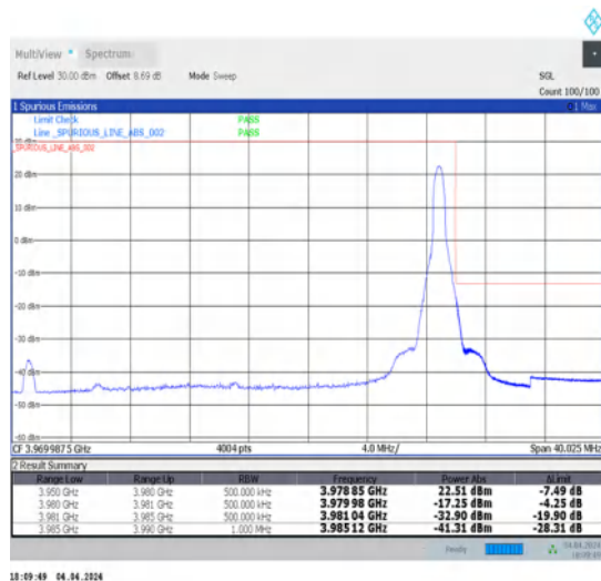
1-N77-3700-3980-30-30-H-5-CP-QPSK-Edge_1RB_Right-1@77-Ant1-1--PASS-see graph
