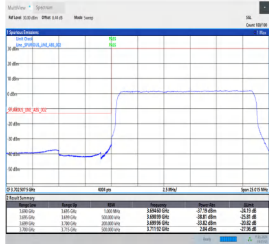
1-N77-3700-3980-30-15-L-3-DFT-PI2BPSK-Outer_Full-36@0-Ant1-1--PASS-see graph
