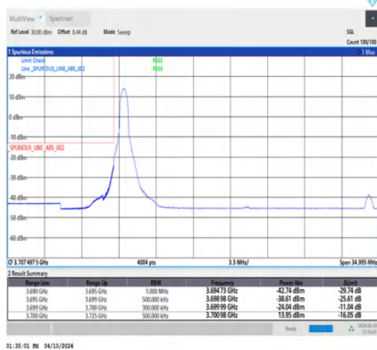
1-N77-3700-3980-30-25-L-4-CP-QPSK-Edge_1RB_Left-1@0-Ant1-1--PASS-see graph
