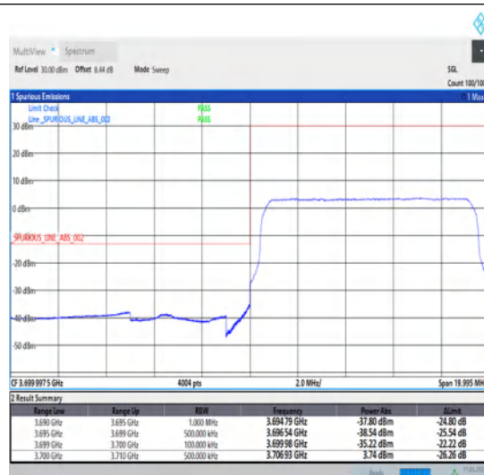
1-N77-3700-3980-30-10-L-3-DFT-PI2BPSK-Outer_Full-24@0-Ant1-1--PASS-see graph
