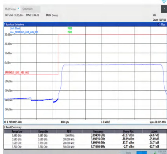
1-N77-3700-3980-30-20-L-6-CP-QPSK-Outer_Full-51@0-Ant1-1--PASS-see graph
