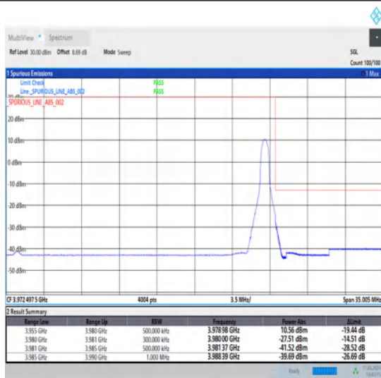
1-N77-3700-3980-30-25-H-2-DFT-PI2BPSK-Edge_1RB_Right-1@64-Ant1-1--PASS-see graph
