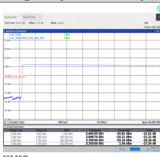
1-N77-3700-3980-30-80-L-6-CP-QPSK-Outer_Full-217@0-Ant1-1--PASS-see graph
