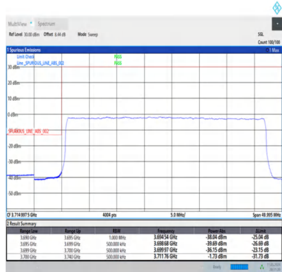
1-N77-3700-3980-30-40-L-3-DFT-PI2BPSK-Outer_Full-100@0-Ant1-1--PASS-see graph
