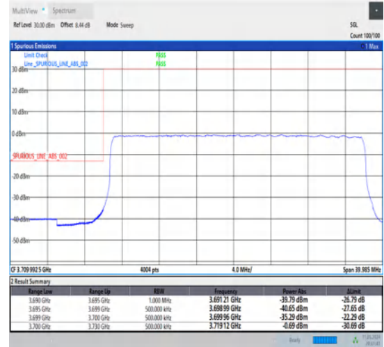
1-N77-3700-3980-30-30-L-3-DFT-PI2BPSK-Outer_Full-75@0-Ant1-1--PASS-see graph
