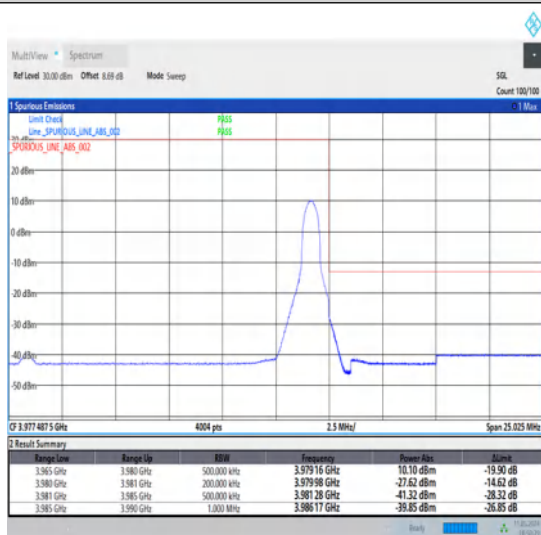
1-N77-3700-3980-30-15-H-5-CP-QPSK-Edge_1RB_Right-1@37-Ant1-1--PASS-see graph
