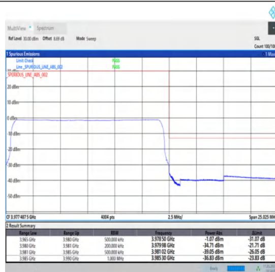
1-N77-3700-3980-30-15-H-6-CP-QPSK-Outer_Full-38@0-Ant1-1--PASS-see graph
