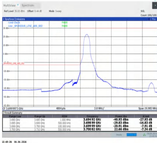
1-N77-3700-3980-30-10-L-4-CP-QPSK-Edge_1RB_Left-1@0-Ant1-1--PASS-see graph
