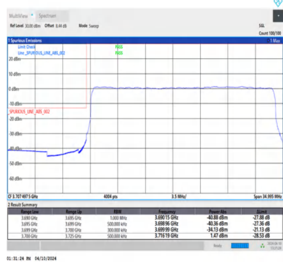
1-N77-3700-3980-30-25-L-3-DFT-PI2BPSK-Outer_Full-64@0-Ant1-1--PASS-see graph
