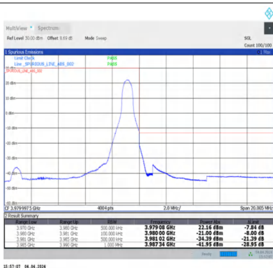
1-N77-3700-3980-30-10-H-2-DFT-PI2BPSK-Edge_1RB_Right-1@23-Ant1-1--PASS-see graph
