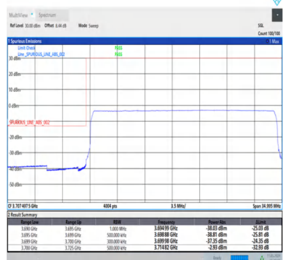
1-N77-3700-3980-30-25-L-6-CP-QPSK-Outer_Full-65@0-Ant1-1--PASS-see graph
