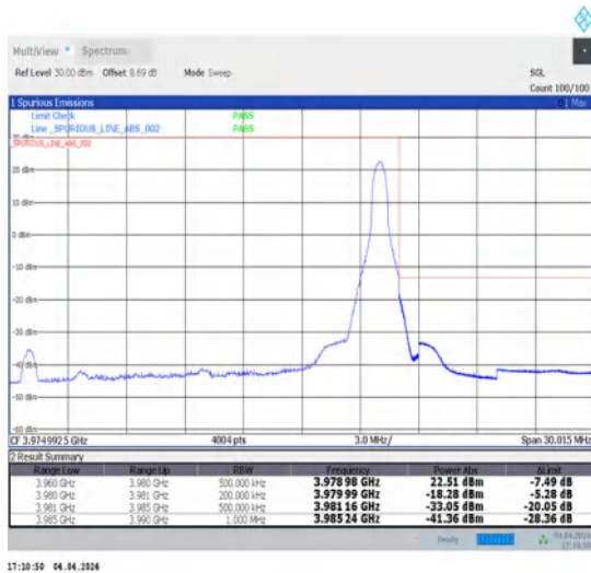
1-N77-3700-3980-30-20-H-5-CP-QPSK-Edge_1RB_Right-1@50-Ant1-1--PASS-see graph
