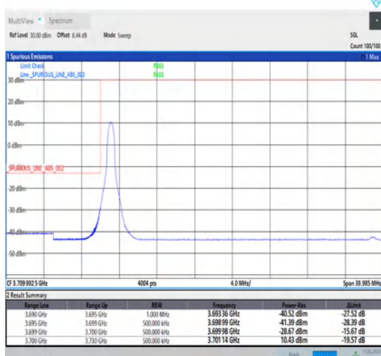
1-N77-3700-3980-30-30-L-4-CP-QPSK-Edge_1RB_Left-1@0-Ant1-1--PASS-see graph
