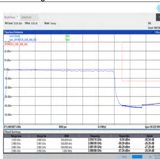
1-N77-3700-3980-30-30-H-3-DFT-PI2BPSK-Outer_Full-75@0-Ant1-1--PASS-see graph
