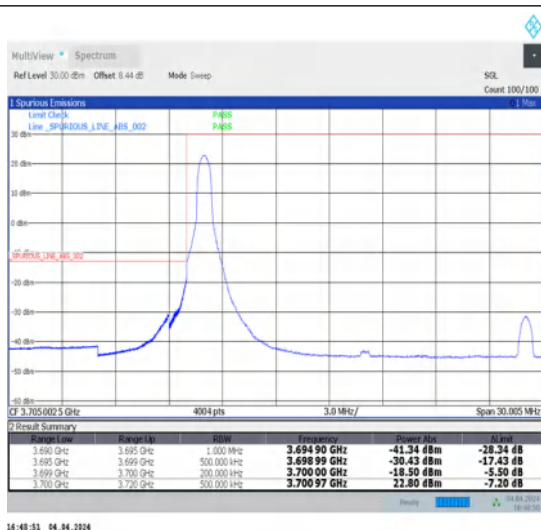
1-N77-3700-3980-30-20-L-1-DFT-PI2BPSK-Edge_1RB_Left-1@0-Ant1-1--PASS-see graph
