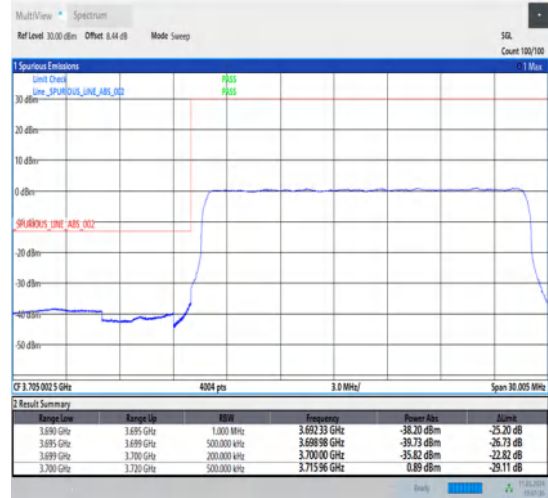
1-N77-3700-3980-30-20-L-3-DFT-PI2BPSK-Outer_Full-50@0-Ant1-1--PASS-see graph
