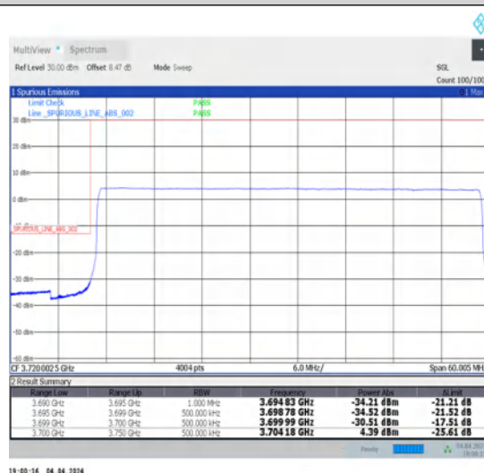
1-N77-3700-3980-30-50-L-6-CP-QPSK-Outer_Full-133@0-Ant1-1--PASS-see graph
