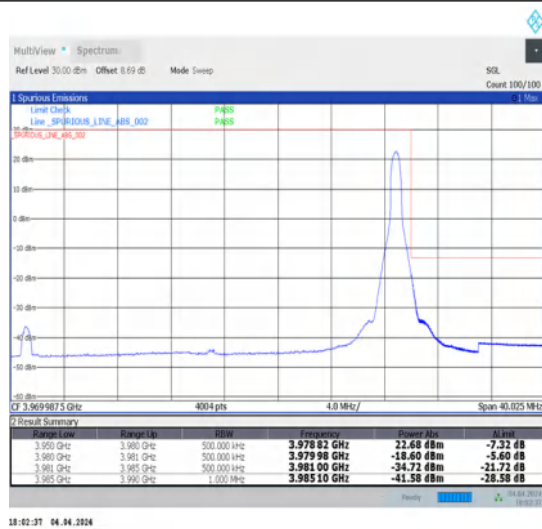
1-N77-3700-3980-30-30-H-2-DFT-PI2BPSK-Edge_1RB_Right-1@77-Ant1-1--PASS-see graph
