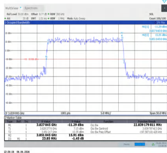
1-N77-3700-3980-30-25-M-4-DFT-64QAM-Outer_Full-64@0-Ant1-22.839-23.850-≤25-PASS
