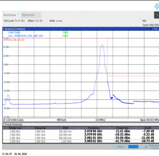
1-N77-3700-3980-30-20-H-2-DFT-PI2BPSK-Edge_1RB_Right-1@50-Ant1-1--PASS-see graph
