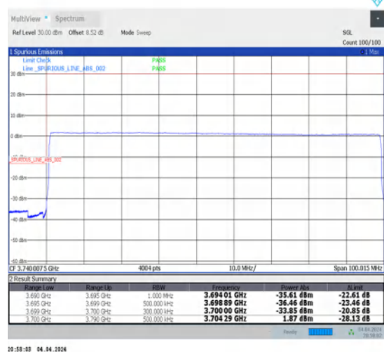
1-N77-3700-3980-30-90-L-6-CP-QPSK-Outer_Full-245@0-Ant1-1--PASS-see graph
