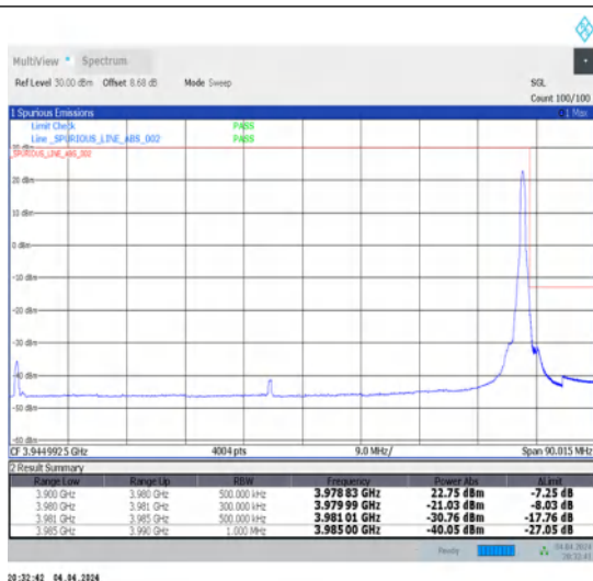
1-N77-3700-3980-30-80-H-2-DFT-PI2BPSK-Edge_1RB_Right-1@216-Ant1-1--PASS-see graph
