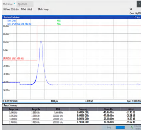
1-N77-3700-3980-30-30-L-1-DFT-PI2BPSK-Edge_1RB_Left-1@0-Ant1-1--PASS-see graph
