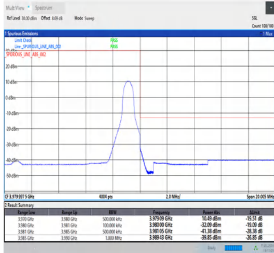
1-N77-3700-3980-30-10-H-2-DFT-PI2BPSK-Edge_1RB_Right-1@23-Ant1-1--PASS-see graph
