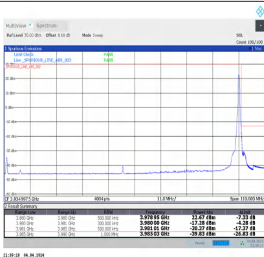
1-N77-3700-3980-30-100-H-5-CP-QPSK-Edge_1RB_Right-1@272-Ant1-1--PASS-see graph
