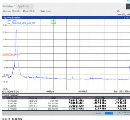
1-N77-3700-3980-30-90-L-4-CP-QPSK-Edge_1RB_Left-1@0-Ant1-1--PASS-see graph
