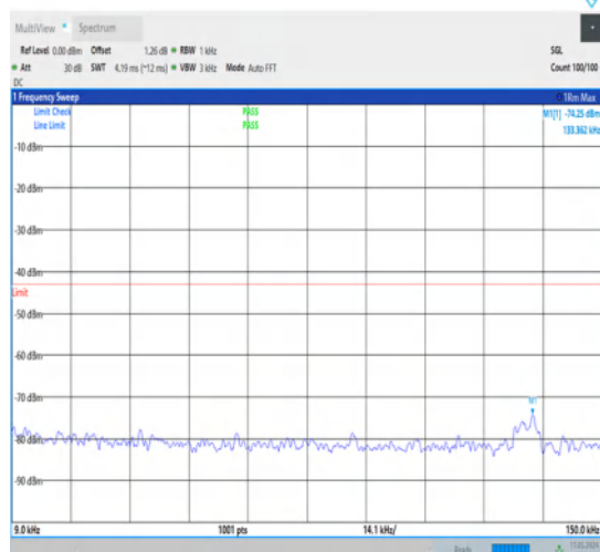
1-N77-3700-3980-30-100-L-1-DFT-QPSK- Edge_1RB_Left-1@0-0.009-0.15-Ant1-0.13--74.25-- 43-PASS
