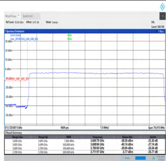
1-N77-3700-3980-30-60-L-3-DFT-PI2BPSK-Outer_Full-162@0-Ant1-1--PASS-see graph
