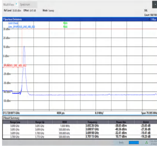
1-N77-3700-3980-30-70-L-1-DFT-PI2BPSK-Edge_1RB_Left-1@0-Ant1-1--PASS-see graph
