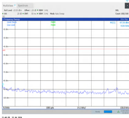
1-N77-3700-3980-30-100-M-1-DFT-PI2BPSK- Inner_1RB_Left-1@1-0.009-0.15-Ant1-0.02--87.26-- 43-PASS
