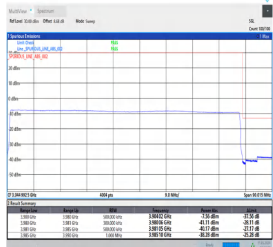
1-N77-3700-3980-30-80-H-6-CP-QPSK-Outer_Full-217@0-Ant1-1--PASS-see graph
