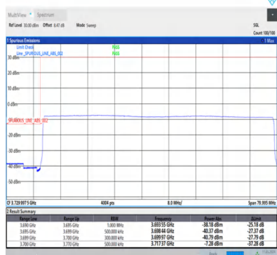
1-N77-3700-3980-30-70-L-6-CP-QPSK-Outer_Full-189@0-Ant1-1--PASS-see graph
