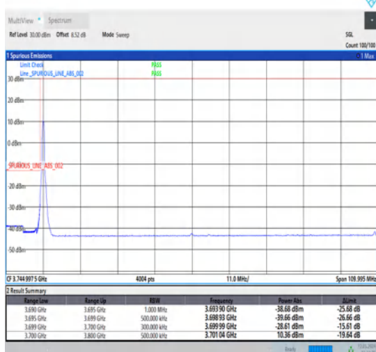
1-N77-3700-3980-30-100-L-4-CP-QPSK-Edge_1RB_Left-1@0-Ant1-1--PASS-see graph
