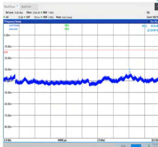
1-N77-3700-3980-30-100-L-1-DFT-QPSK- Edge_1RB_Left-1@0-6000-26000-Ant1-22124.46-- 33.25--13-PASS
