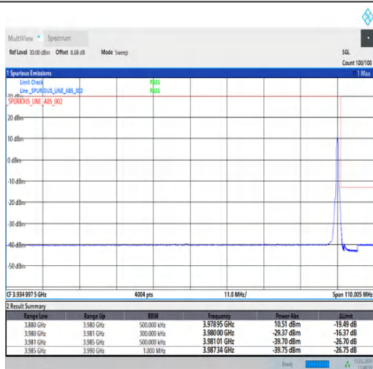
1-N77-3700-3980-30-100-H-5-CP-QPSK-Edge_1RB_Right-1@272-Ant1-1--PASS-see graph
