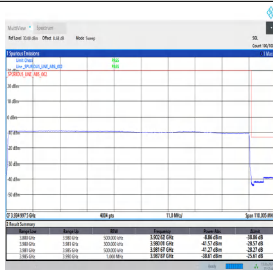
1-N77-3700-3980-30-100-H-6-CP-QPSK-Outer_Full-273@0-Ant1-1--PASS-see graph
