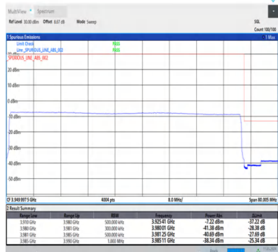
1-N77-3700-3980-30-70-H-6-CP-QPSK-Outer_Full-189@0-Ant1-1--PASS-see graph
