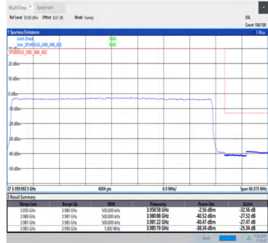
1-N77-3700-3980-30-50-H-3-DFT-PI2BPSK-Outer_Full-128@0-Ant1-1--PASS-see graph
