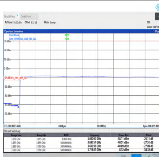
1-N77-3700-3980-30-90-L-6-CP-QPSK-Outer_Full-245@0-Ant1-1--PASS-see graph
