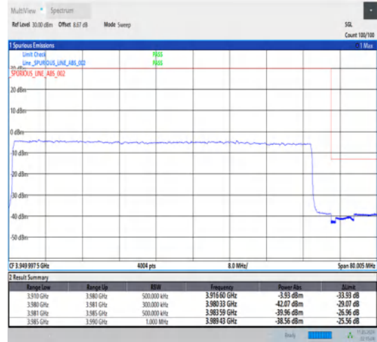
1-N77-3700-3980-30-70-H-3-DFT-PI2BPSK-Outer_Full-180@0-Ant1-1--PASS-see graph
