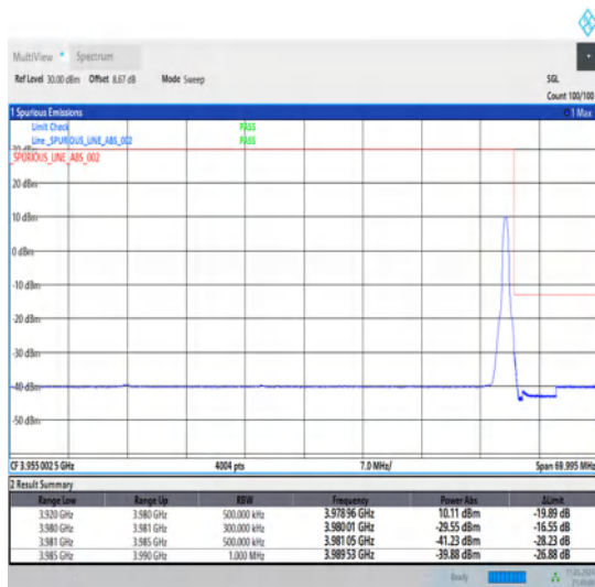
1-N77-3700-3980-30-60-H-5-CP-QPSK-Edge_1RB_Right-1@161-Ant1-1--PASS-see graph
