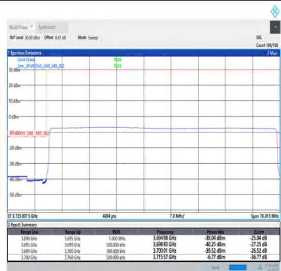
1-N77-3700-3980-30-60-L-6-CP-QPSK-Outer_Full-162@0-Ant1-1--PASS-see graph
