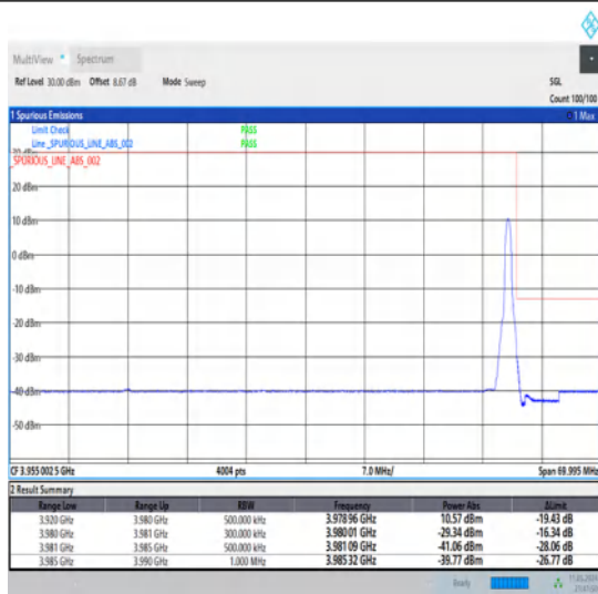
1-N77-3700-3980-30-60-H-2-DFT-PI2BPSK-Edge_1RB_Right-1@161-Ant1-1--PASS-see graph
