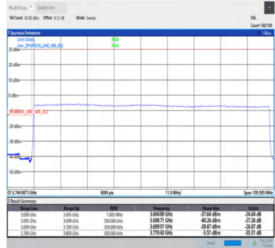
1-N77-3700-3980-30-100-L-3-DFT-PI2BPSK-Outer_Full-270@0-Ant1-1--PASS-see graph
