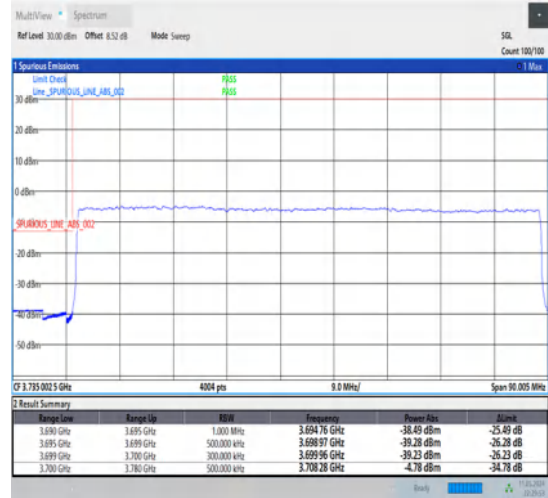
1-N77-3700-3980-30-80-L-3-DFT-PI2BPSK-Outer_Full-216@0-Ant1-1--PASS-see graph
