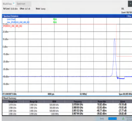
1-N77-3700-3980-30-70-H-2-DFT-PI2BPSK-Edge_1RB_Right-1@188-Ant1-1--PASS-see graph
