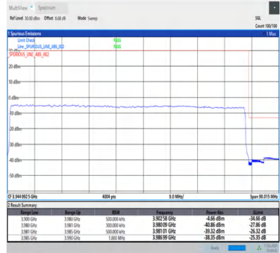
1-N77-3700-3980-30-80-H-3-DFT-PI2BPSK-Outer_Full-216@0-Ant1-1--PASS-see graph
