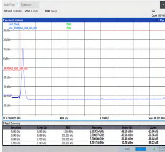
1-N77-3700-3980-30-80-L-1-DFT-PI2BPSK-Edge_1RB_Left-1@0-Ant1-1--PASS-see graph
