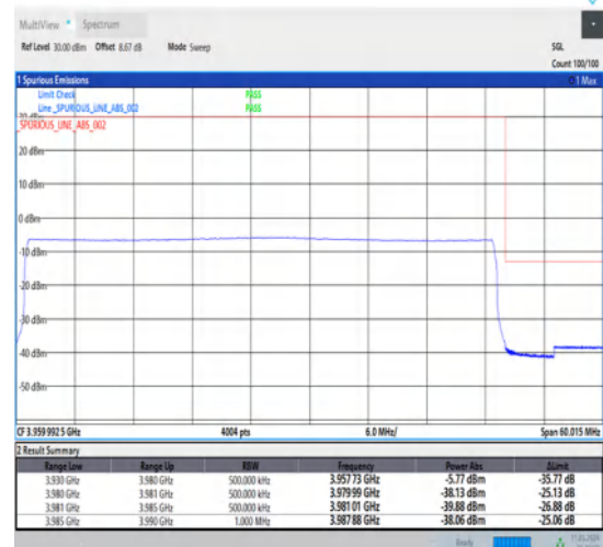
1-N77-3700-3980-30-50-H-6-CP-QPSK-Outer_Full-133@0-Ant1-1--PASS-see graph
