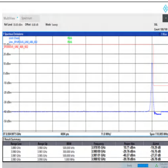
1-N77-3700-3980-30-100-H-2-DFT-PI2BPSK-Edge_1RB_Right-1@272-Ant1-1--PASS-see graph
