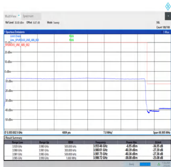
1-N77-3700-3980-30-60-H-6-CP-QPSK-Outer_Full-162@0-Ant1-1--PASS-see graph
