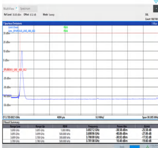
1-N77-3700-3980-30-80-L-4-CP-QPSK-Edge_1RB_Left-1@0-Ant1-1--PASS-see graph
