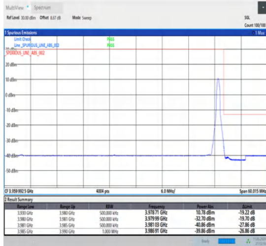
1-N77-3700-3980-30-50-H-2-DFT-PI2BPSK-Edge_1RB_Right-1@132-Ant1-1--PASS-see graph
