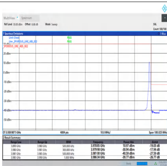
1-N77-3700-3980-30-90-H-2-DFT-PI2BPSK-Edge_1RB_Right-1@244-Ant1-1--PASS-see graph
