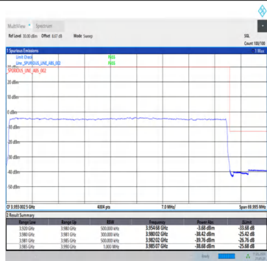
1-N77-3700-3980-30-60-H-3-DFT-PI2BPSK-Outer_Full-162@0-Ant1-1--PASS-see graph
