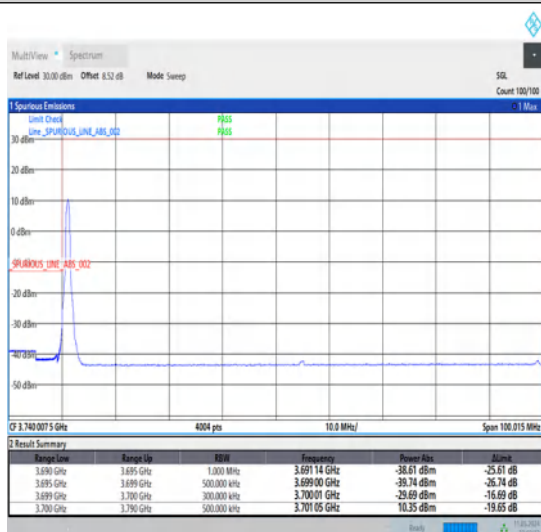
1-N77-3700-3980-30-90-L-4-CP-QPSK-Edge_1RB_Left-1@0-Ant1-1--PASS-see graph
