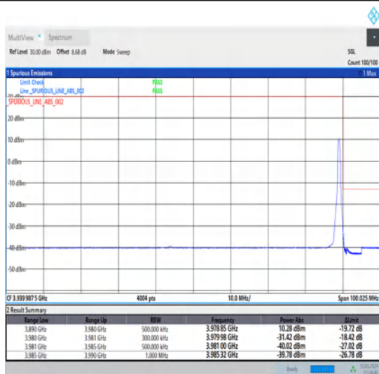
1-N77-3700-3980-30-90-H-5-CP-QPSK-Edge_1RB_Right-1@244-Ant1-1--PASS-see graph
