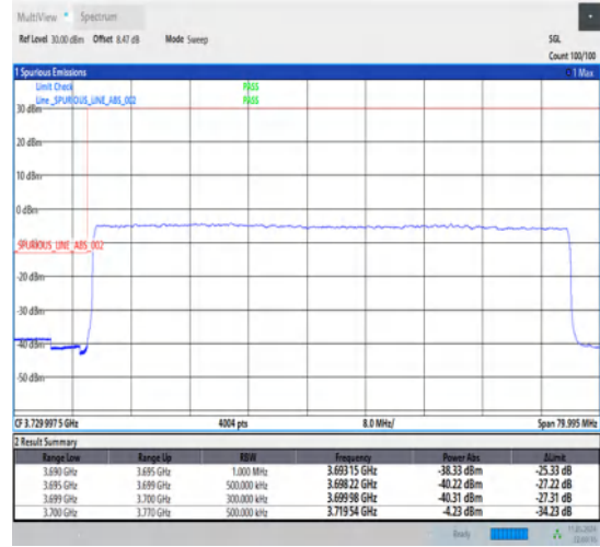
1-N77-3700-3980-30-70-L-3-DFT-PI2BPSK-Outer_Full-180@0-Ant1-1--PASS-see graph
