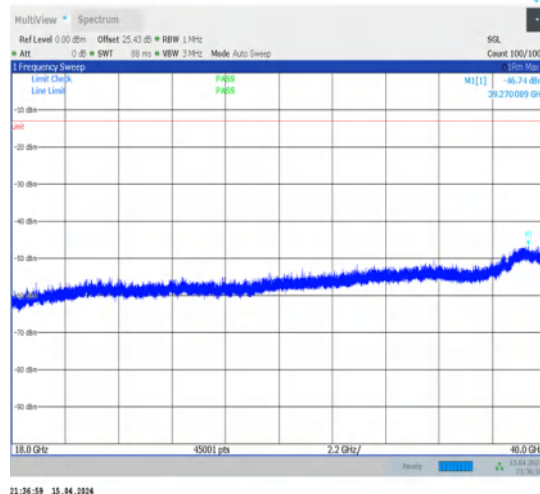
1-N77-3700-3980-30-100-L-1-DFT-PI2BPSK- Inner_1RB_Left-1@1-18000-40000-Ant1-18506.49-- 46.74--13-PASS
