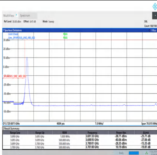
1-N77-3700-3980-30-60-L-4-CP-QPSK-Edge_1RB_Left-1@0-Ant1-1--PASS-see graph
