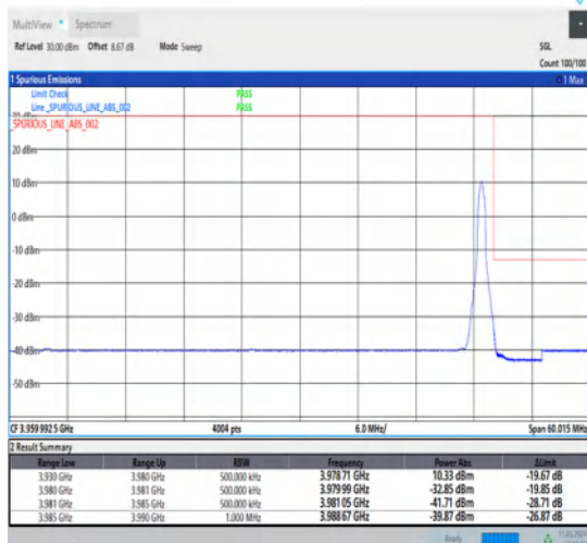
1-N77-3700-3980-30-50-H-5-CP-QPSK-Edge_1RB_Right-1@132-Ant1-1--PASS-see graph
