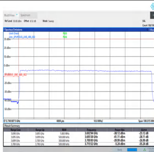
1-N77-3700-3980-30-90-L-3-DFT-PI2BPSK-Outer_Full-240@0-Ant1-1--PASS-see graph
