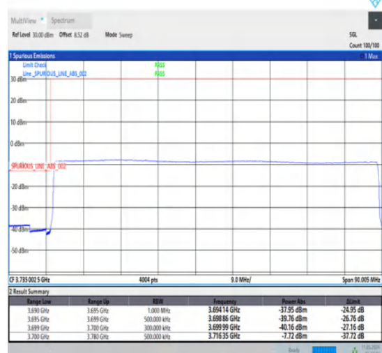
1-N77-3700-3980-30-80-L-6-CP-QPSK-Outer_Full-217@0-Ant1-1--PASS-see graph
