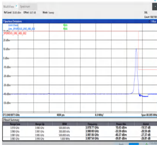
1-N77-3700-3980-30-70-H-5-CP-QPSK-Edge_1RB_Right-1@188-Ant1-1--PASS-see graph
