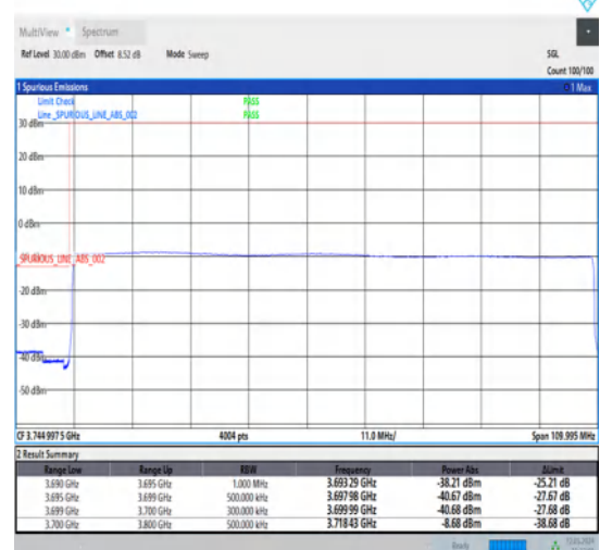
1-N77-3700-3980-30-100-L-6-CP-QPSK-Outer_Full-273@0-Ant1-1--PASS-see graph
