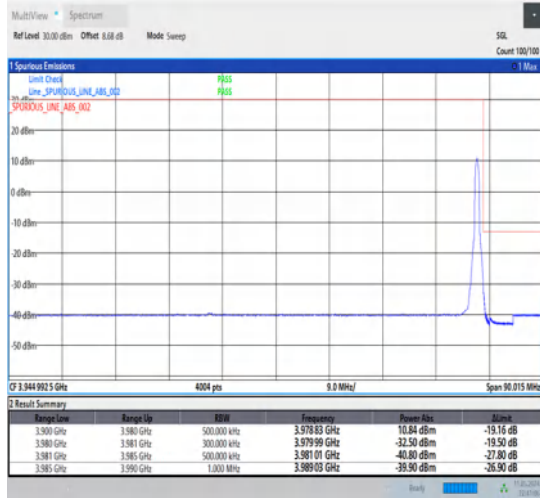
1-N77-3700-3980-30-80-H-2-DFT-PI2BPSK-Edge_1RB_Right-1@216-Ant1-1--PASS-see graph
