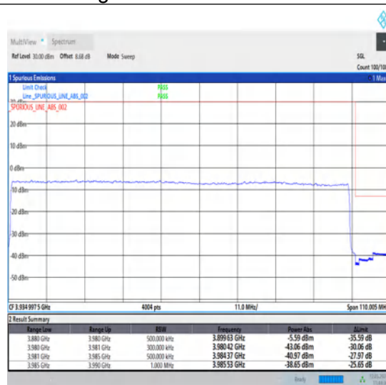
1-N77-3700-3980-30-100-H-3-DFT-PI2BPSK-Outer_Full-270@0-Ant1-1--PASS-see graph
