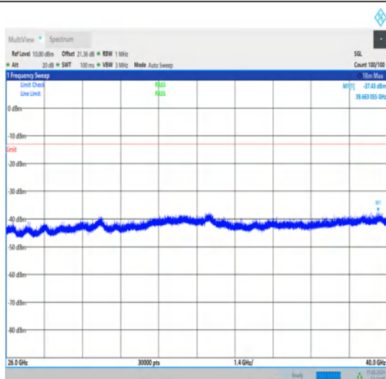
1-N77-3700-3980-30-100-L-1-DFT-QPSK- Edge_1RB_Left-1@0-26000-40000-Ant1-39663.06-- 37.43--13-PASS
