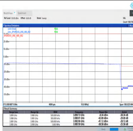
1-N77-3700-3980-30-90-H-6-CP-QPSK-Outer_Full-245@0-Ant1-1--PASS-see graph
