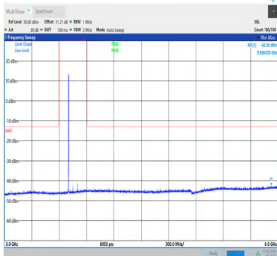
1-N77-3700-3980-30-100-L-1-DFT-QPSK- Edge_1RB_Left-1@0-3000-6000-Ant1-5926.02-- 42.58--13-PASS
