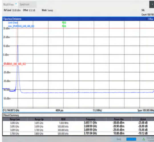
1-N77-3700-3980-30-100-L-1-DFT-PI2BPSK-Edge_1RB_Left-1@0-Ant1-1--PASS-see graph
