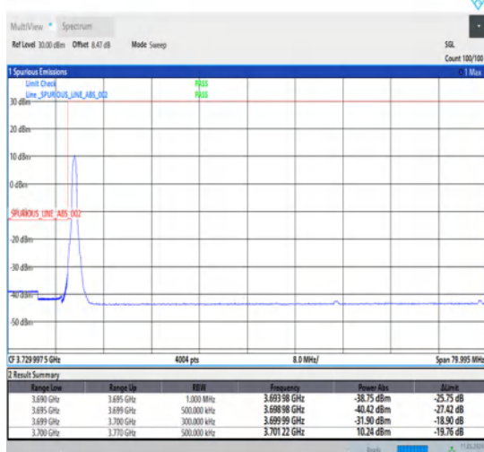
1-N77-3700-3980-30-70-L-4-CP-QPSK-Edge_1RB_Left-1@0-Ant1-1--PASS-see graph
