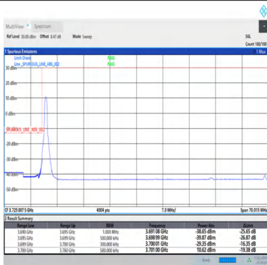
1-N77-3700-3980-30-60-L-1-DFT-PI2BPSK-Edge_1RB_Left-1@0-Ant1-1--PASS-see graph
