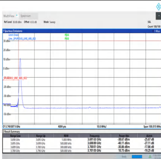
1-N77-3700-3980-30-90-L-1-DFT-PI2BPSK-Edge_1RB_Left-1@0-Ant1-1--PASS-see graph
