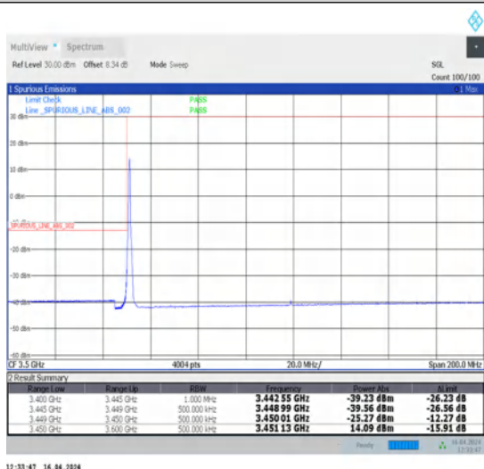
1-N78-3450-3550-30-70-L-4-CP-QPSK-Edge_1RB_Left-1@0-Ant1-1--PASS-see graph
