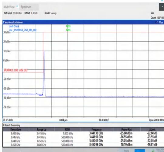
1-N78-3450-3550-30-100-L-4-CP-QPSK-Edge_1RB_Left-1@0-Ant1-1--PASS-see graph
