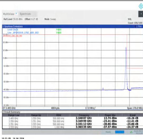
1-N78-3450-3550-30-30-H-5-CP-QPSK-Edge_1RB_Right-1@77-Ant1-1--PASS-see graph
