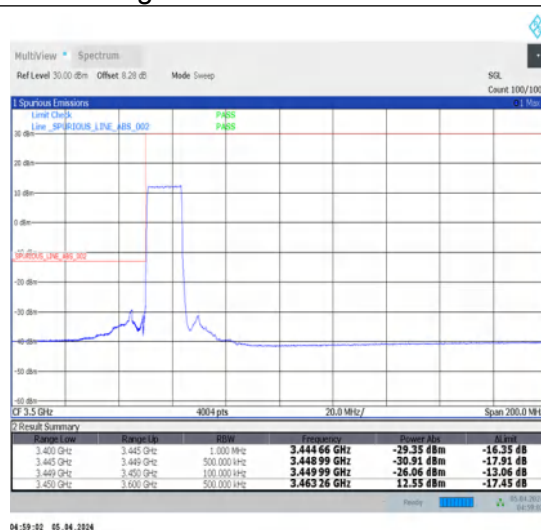
1-N78-3450-3550-30-15-L-3-DFT-PI2BPSK-Outer_Full-36@0-Ant1-1--PASS-see graph
