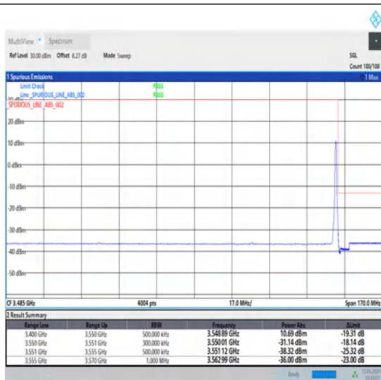
1-N78-3450-3550-30-40-H-2-DFT-PI2BPSK-Edge_1RB_Right-1@105-Ant1-1--PASS-see graph
