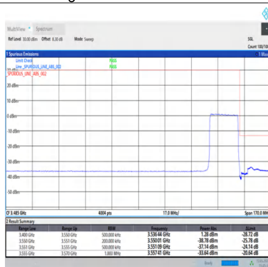
1-N78-3450-3550-30-20-H-3-DFT-PI2BPSK-Outer_Full-50@0-Ant1-1--PASS-see graph
