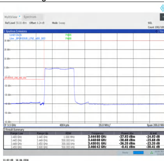
1-N78-3450-3550-30-40-L-3-DFT-PI2BPSK-Outer_Full-100@0-Ant1-1--PASS-see graph
