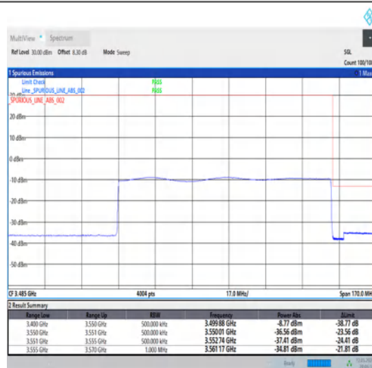
1-N78-3450-3550-30-100-H-6-CP-QPSK-Outer_Full-273@0-Ant1-1--PASS-see graph
