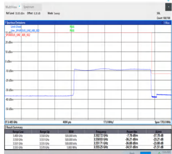
1-N78-3450-3550-30-80-H-6-CP-QPSK-Outer_Full-217@0-Ant1-1--PASS-see graph
