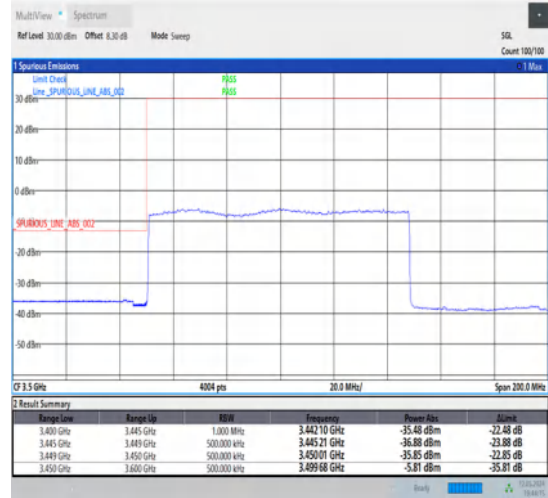
1-N78-3450-3550-30-100-L-3-DFT-PI2BPSK-Outer_Full-270@0-Ant1-1--PASS-see graph
