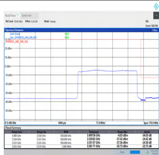
1-N78-3450-3550-30-70-H-3-DFT-PI2BPSK-Outer_Full-180@0-Ant1-1--PASS-see graph
