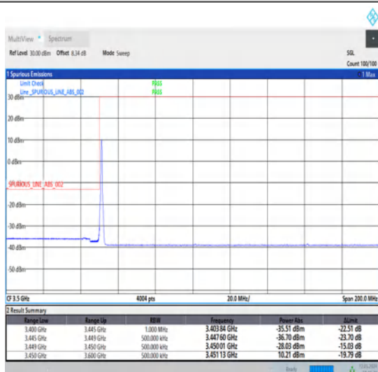
1-N78-3450-3550-30-70-L-4-CP-QPSK-Edge_1RB_Left-1@0-Ant1-1--PASS-see graph
