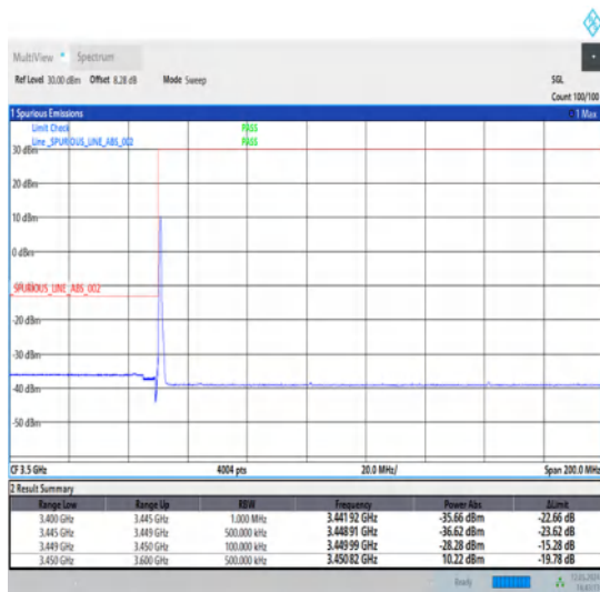
1-N78-3450-3550-30-15-L-4-CP-QPSK-Edge_1RB_Left-1@0-Ant1-1--PASS-see graph
