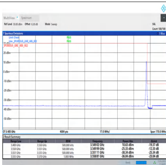
1-N78-3450-3550-30-60-H-2-DFT-PI2BPSK-Edge_1RB_Right-1@161-Ant1-1--PASS-see graph
