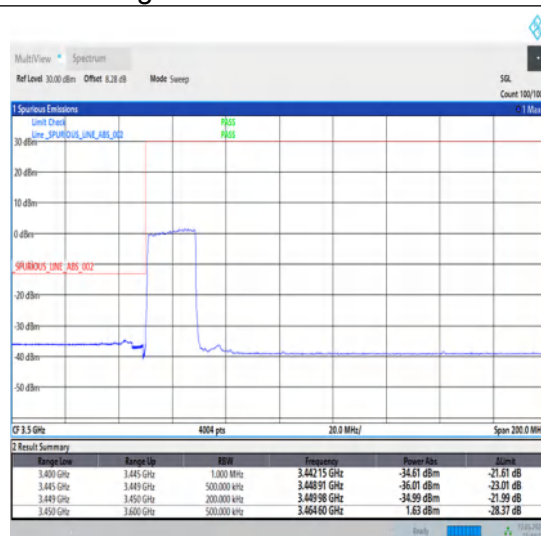
1-N78-3450-3550-30-20-L-3-DFT-PI2BPSK-Outer_Full-50@0-Ant1-1--PASS-see graph
