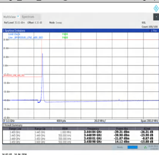
1-N78-3450-3550-30-100-L-4-CP-QPSK-Edge_1RB_Left-1@0-Ant1-1--PASS-see graph
