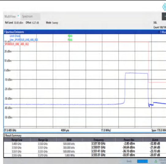
1-N78-3450-3550-30-25-H-6-CP-QPSK-Outer_Full-65@0-Ant1-1--PASS-see graph
