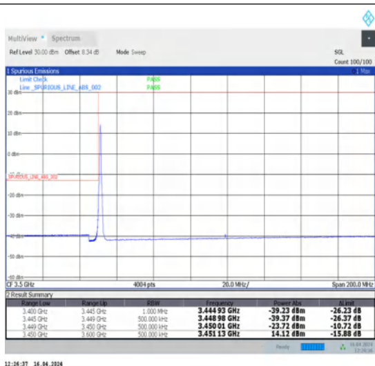
1-N78-3450-3550-30-70-L-1-DFT-PI2BPSK-Edge_1RB_Left-1@0-Ant1-1--PASS-see graph
