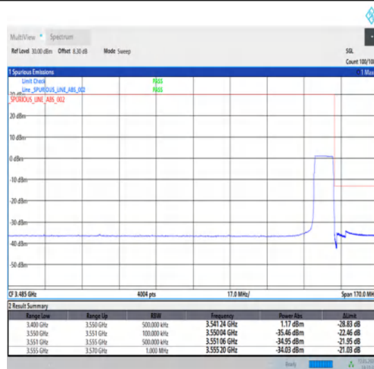
1-N78-3450-3550-30-10-H-6-CP-QPSK-Outer_Full-24@0-Ant1-1--PASS-see graph
