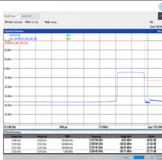
1-N78-3450-3550-30-30-H-6-CP-QPSK-Outer_Full-78@0-Ant1-1--PASS-see graph
