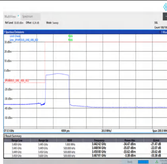
1-N78-3450-3550-30-30-L-6-CP-QPSK-Outer_Full-78@0-Ant1-1--PASS-see graph
