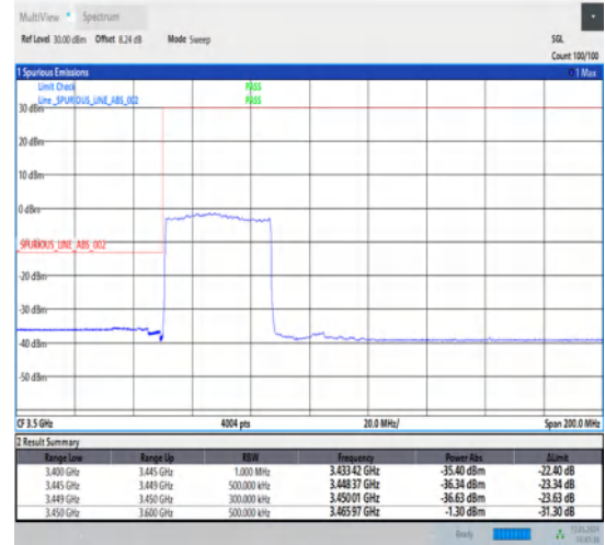
1-N78-3450-3550-30-40-L-3-DFT-PI2BPSK-Outer_Full-100@0-Ant1-1--PASS-see graph
