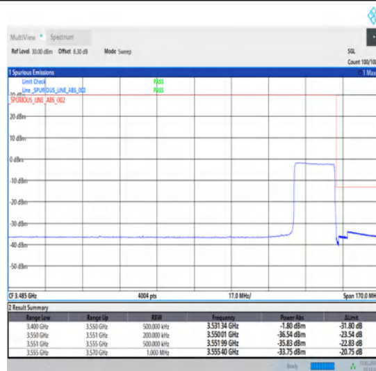
1-N78-3450-3550-30-20-H-6-CP-QPSK-Outer_Full-51@0-Ant1-1--PASS-see graph
