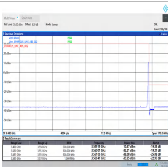
1-N78-3450-3550-30-10-H-2-DFT-PI2BPSK-Edge_1RB_Right-1@23-Ant1-1--PASS-see graph
