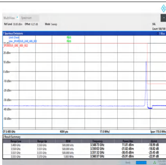
1-N78-3450-3550-30-50-H-2-DFT-PI2BPSK-Edge_1RB_Right-1@132-Ant1-1--PASS-see graph
