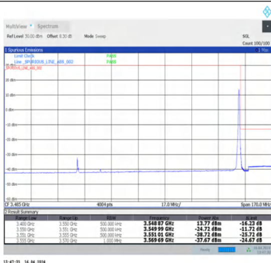
1-N78-3450-3550-30-90-H-5-CP-QPSK-Edge_1RB_Right-1@244-Ant1-1--PASS-see graph
