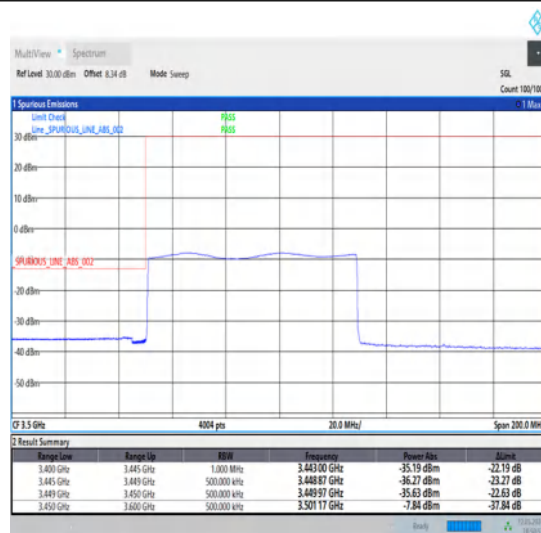
1-N78-3450-3550-30-80-L-6-CP-QPSK-Outer_Full-217@0-Ant1-1--PASS-see graph
