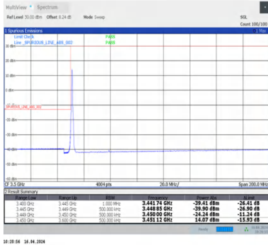
1-N78-3450-3550-30-30-L-1-DFT-PI2BPSK-Edge_1RB_Left-1@0-Ant1-1--PASS-see graph
