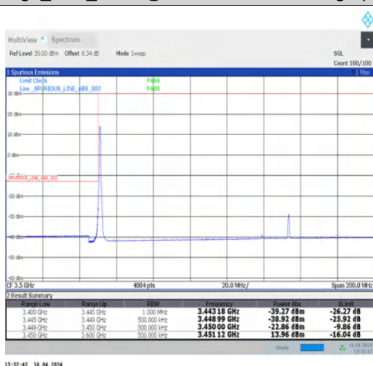
1-N78-3450-3550-30-90-L-4-CP-QPSK-Edge_1RB_Left-1@0-Ant1-1--PASS-see graph
