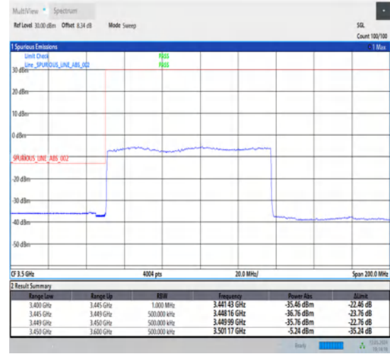
1-N78-3450-3550-30-90-L-3-DFT-PI2BPSK-Outer_Full-240@0-Ant1-1--PASS-see graph
