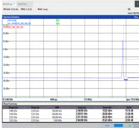
1-N78-3450-3550-30-80-H-2-DFT-PI2BPSK-Edge_1RB_Right-1@216-Ant1-1--PASS-see graph
