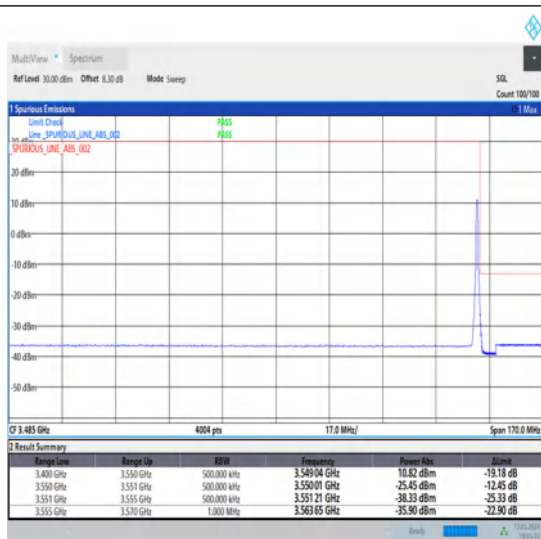
1-N78-3450-3550-30-100-H-2-DFT-PI2BPSK-Edge_1RB_Right-1@272-Ant1-1--PASS-see graph
