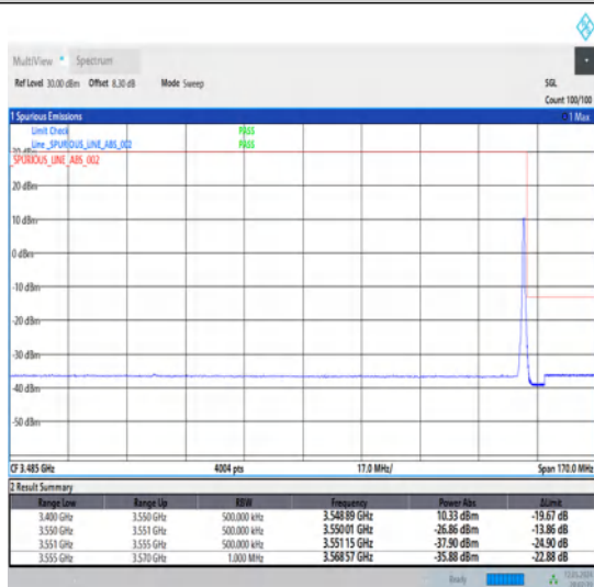
1-N78-3450-3550-30-100-H-5-CP-QPSK-Edge_1RB_Right-1@272-Ant1-1--PASS-see graph
