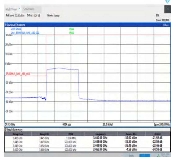
1-N78-3450-3550-30-40-L-6-CP-QPSK-Outer_Full-106@0-Ant1-1--PASS-see graph
