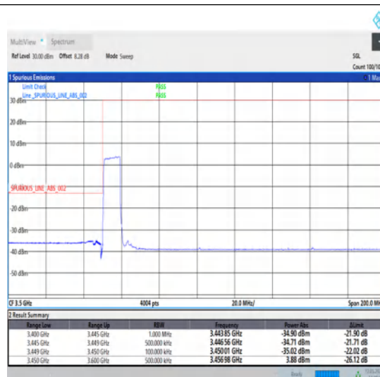
1-N78-3450-3550-30-10-L-3-DFT-PI2BPSK-Outer_Full-24@0-Ant1-1--PASS-see graph
