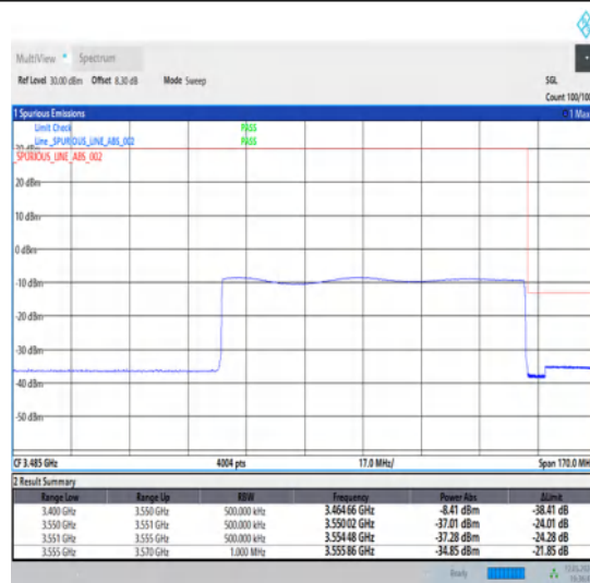
1-N78-3450-3550-30-90-H-6-CP-QPSK-Outer_Full-245@0-Ant1-1--PASS-see graph
