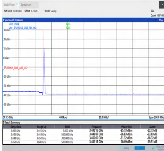
1-N78-3450-3550-30-40-L-1-DFT-PI2BPSK-Edge_1RB_Left-1@0-Ant1-1--PASS-see graph
