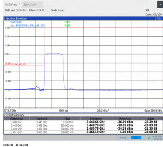
1-N78-3450-3550-30-25-L-3-DFT-PI2BPSK-Outer_Full-64@0-Ant1-1--PASS-see graph
