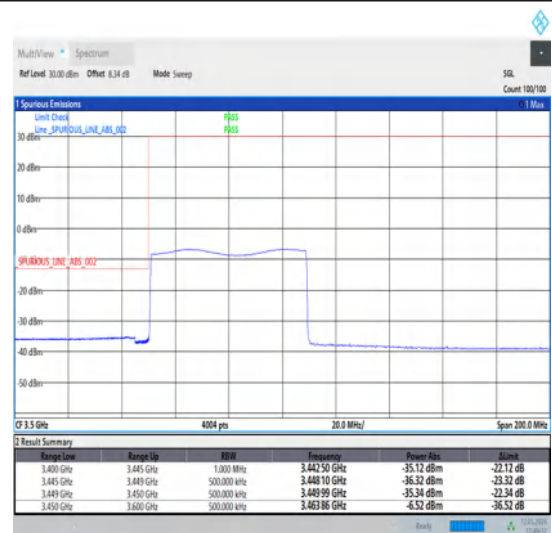
1-N78-3450-3550-30-60-L-6-CP-QPSK-Outer_Full-162@0-Ant1-1--PASS-see graph
