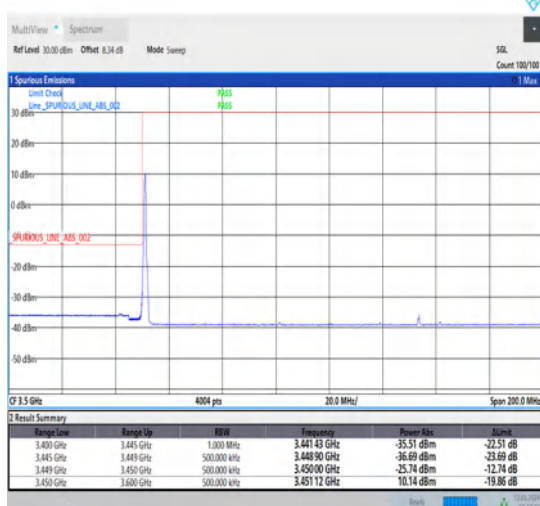
1-N78-3450-3550-30-90-L-4-CP-QPSK-Edge_1RB_Left-1@0-Ant1-1--PASS-see graph
