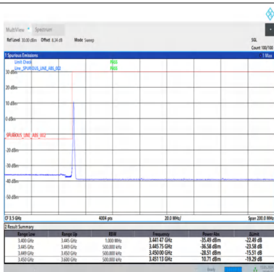
1-N78-3450-3550-30-70-L-1-DFT-PI2BPSK-Edge_1RB_Left-1@0-Ant1-1--PASS-see graph
