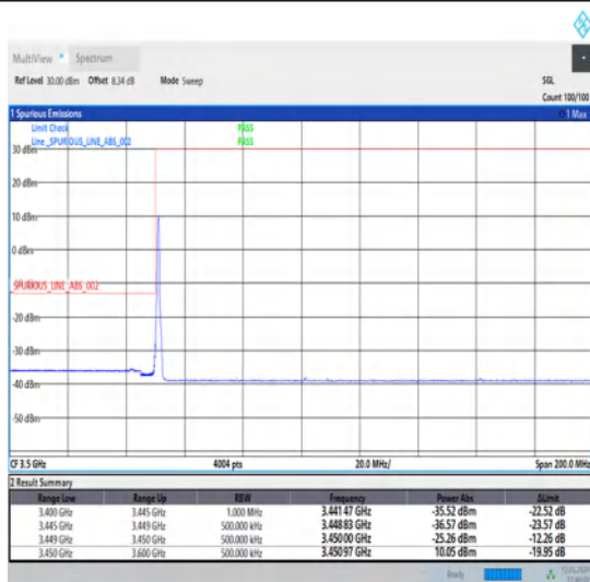
1-N78-3450-3550-30-60-L-4-CP-QPSK-Edge_1RB_Left-1@0-Ant1-1--PASS-see graph
