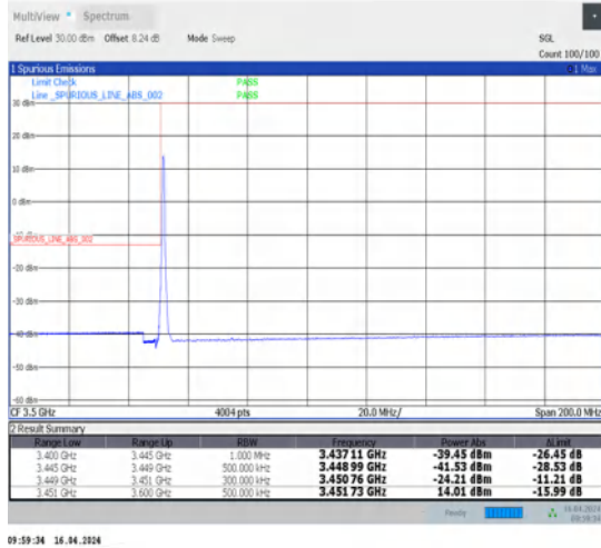
1-N78-3450-3550-30-25-L-1-DFT-PI2BPSK-Edge_1RB_Left-1@0-Ant1-1--PASS-see graph
