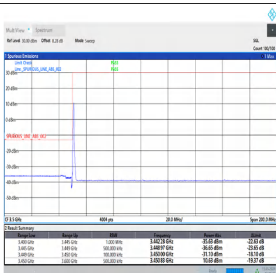
1-N78-3450-3550-30-10-L-1-DFT-PI2BPSK-Edge_1RB_Left-1@0-Ant1-1--PASS-see graph
