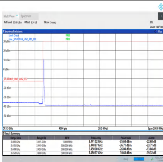
1-N78-3450-3550-30-60-L-1-DFT-PI2BPSK-Edge_1RB_Left-1@0-Ant1-1--PASS-see graph
