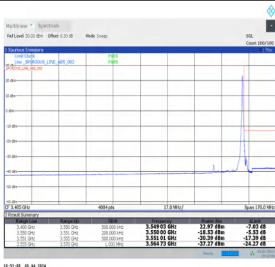
1-N78-3450-3550-30-20-H-5-CP-QPSK-Edge_1RB_Right-1@50-Ant1-1--PASS-see graph
