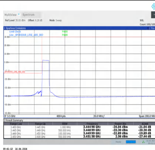
1-N78-3450-3550-30-10-L-6-CP-QPSK-Outer_Full-24@0-Ant1-1--PASS-see graph
