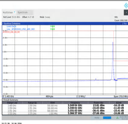
1-N78-3450-3550-30-25-H-5-CP-QPSK-Edge_1RB_Right-1@64-Ant1-1--PASS-see graph
