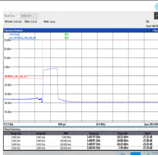
1-N78-3450-3550-30-20-L-6-CP-QPSK-Outer_Full-51@0-Ant1-1--PASS-see graph
