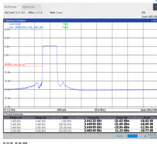
1-N78-3450-3550-30-20-L-3-DFT-PI2BPSK-Outer_Full-50@0-Ant1-1--PASS-see graph
