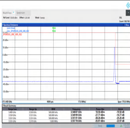
1-N78-3450-3550-30-90-H-5-CP-QPSK-Edge_1RB_Right-1@244-Ant1-1--PASS-see graph
