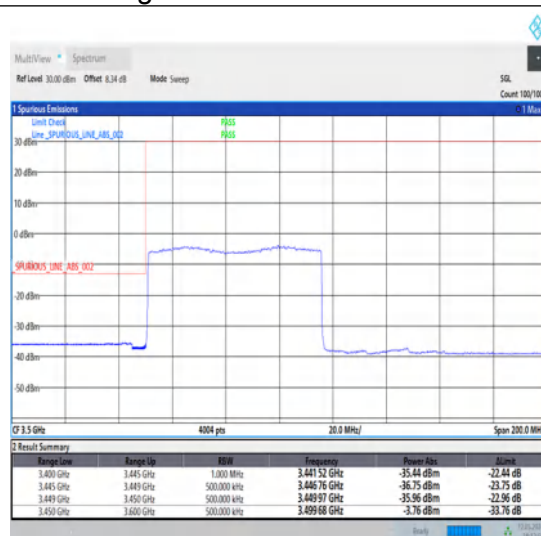
1-N78-3450-3550-30-70-L-3-DFT-PI2BPSK-Outer_Full-180@0-Ant1-1--PASS-see graph
