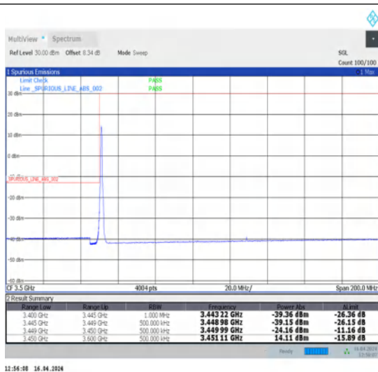
1-N78-3450-3550-30-80-L-1-DFT-PI2BPSK-Edge_1RB_Left-1@0-Ant1-1--PASS-see graph
