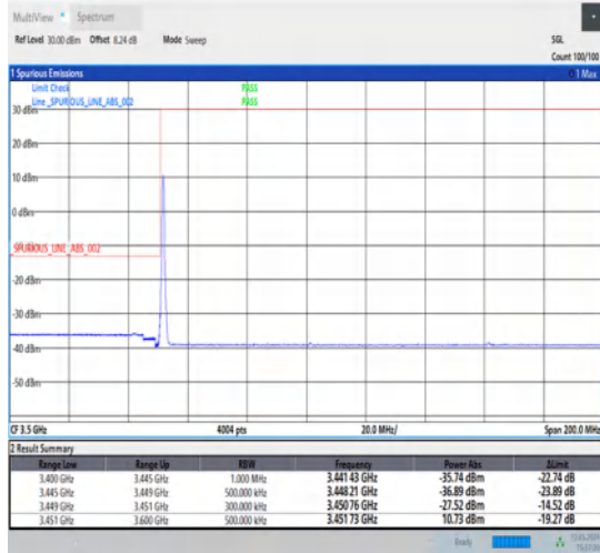
1-N78-3450-3550-30-25-L-1-DFT-PI2BPSK-Edge_1RB_Left-1@0-Ant1-1--PASS-see graph
