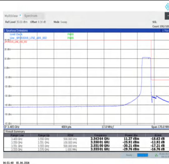
1-N78-3450-3550-30-10-H-6-CP-QPSK-Outer_Full-24@0-Ant1-1--PASS-see graph
