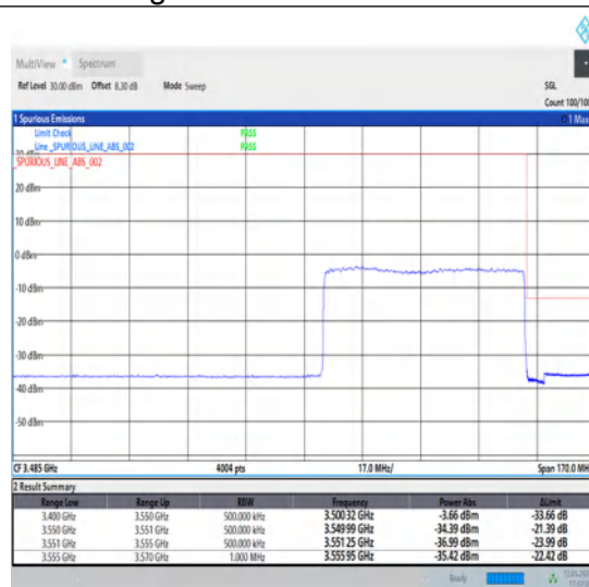
1-N78-3450-3550-30-60-H-3-DFT-PI2BPSK-Outer_Full-162@0-Ant1-1--PASS-see graph
