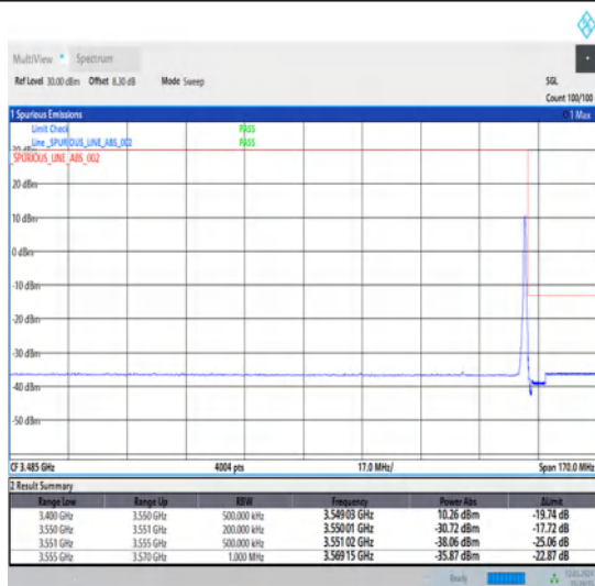
1-N78-3450-3550-30-20-H-5-CP-QPSK-Edge_1RB_Right-1@50-Ant1-1--PASS-see graph
