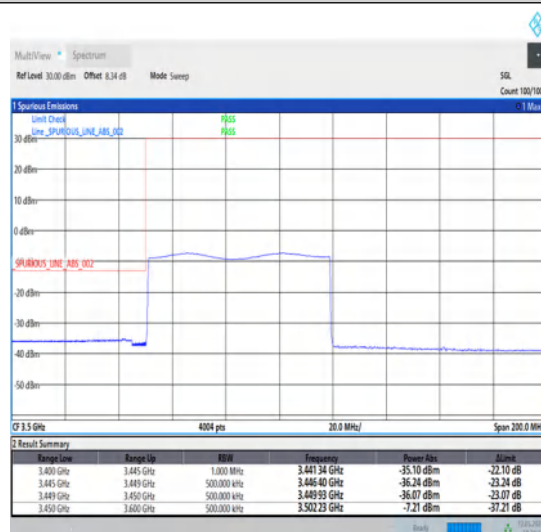
1-N78-3450-3550-30-70-L-6-CP-QPSK-Outer_Full-189@0-Ant1-1--PASS-see graph
