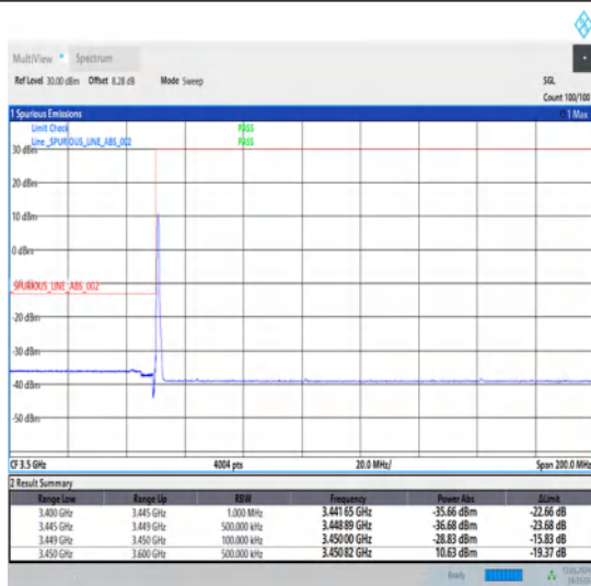
1-N78-3450-3550-30-15-L-1-DFT-PI2BPSK-Edge_1RB_Left-1@0-Ant1-1--PASS-see graph
