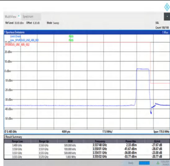
1-N78-3450-3550-30-15-H-3-DFT-PI2BPSK-Outer_Full-36@0-Ant1-1--PASS-see graph
