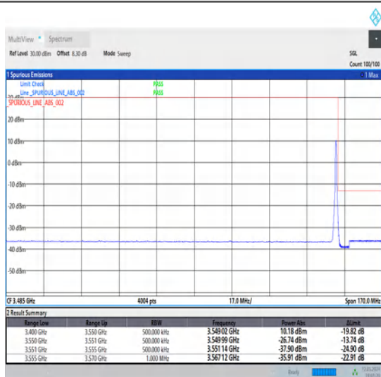
1-N78-3450-3550-30-60-H-5-CP-QPSK-Edge_1RB_Right-1@161-Ant1-1--PASS-see graph
