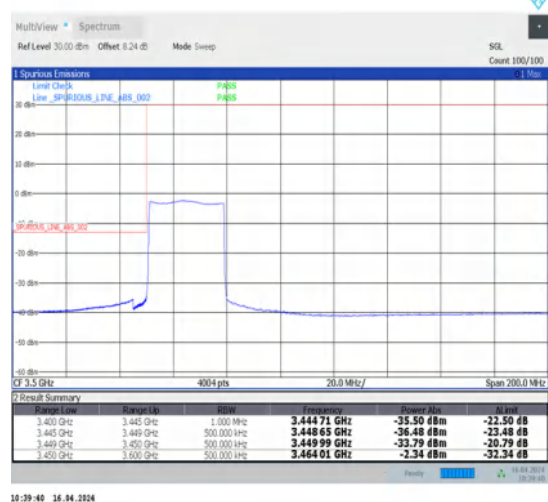
1-N78-3450-3550-30-30-L-6-CP-QPSK-Outer_Full-78@0-Ant1-1--PASS-see graph
