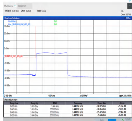
1-N78-3450-3550-30-50-L-6-CP-QPSK-Outer_Full-133@0-Ant1-1--PASS-see graph
