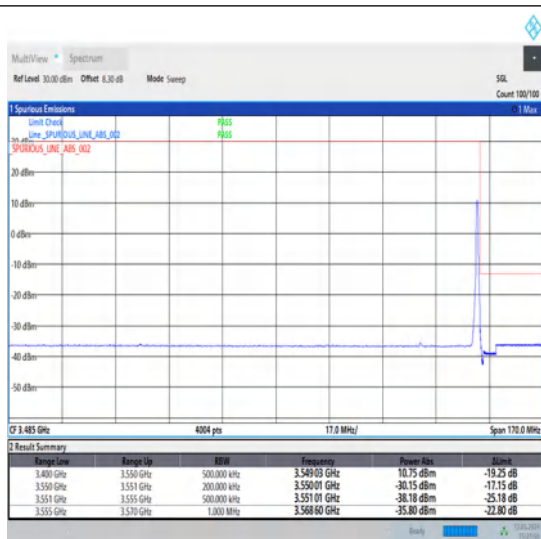
1-N78-3450-3550-30-20-H-2-DFT-PI2BPSK-Edge_1RB_Right-1@50-Ant1-1--PASS-see graph
