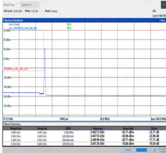
1-N78-3450-3550-30-50-L-1-DFT-PI2BPSK-Edge_1RB_Left-1@0-Ant1-1--PASS-see graph
