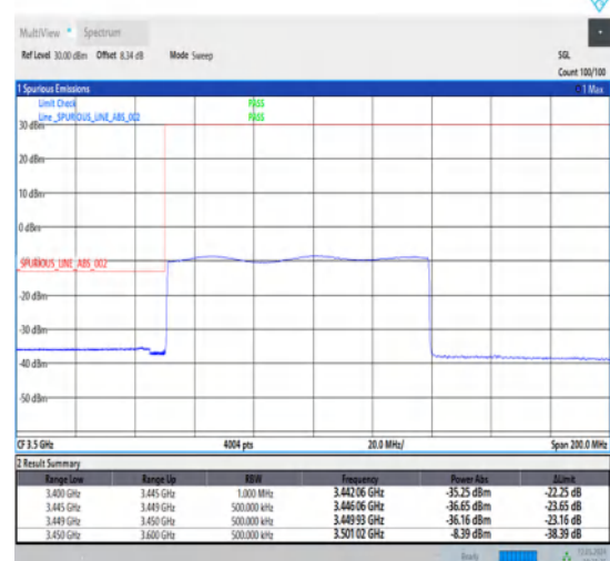
1-N78-3450-3550-30-90-L-6-CP-QPSK-Outer_Full-245@0-Ant1-1--PASS-see graph
