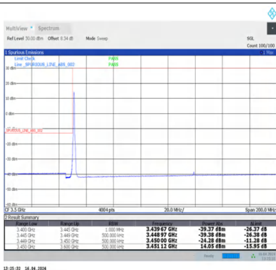
1-N78-3450-3550-30-90-L-1-DFT-PI2BPSK-Edge_1RB_Left-1@0-Ant1-1--PASS-see graph
