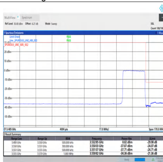
1-N78-3450-3550-30-25-H-3-DFT-PI2BPSK-Outer_Full-64@0-Ant1-1--PASS-see graph
