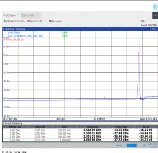
1-N78-3450-3550-30-40-H-5-CP-QPSK-Edge_1RB_Right-1@105-Ant1-1--PASS-see graph
