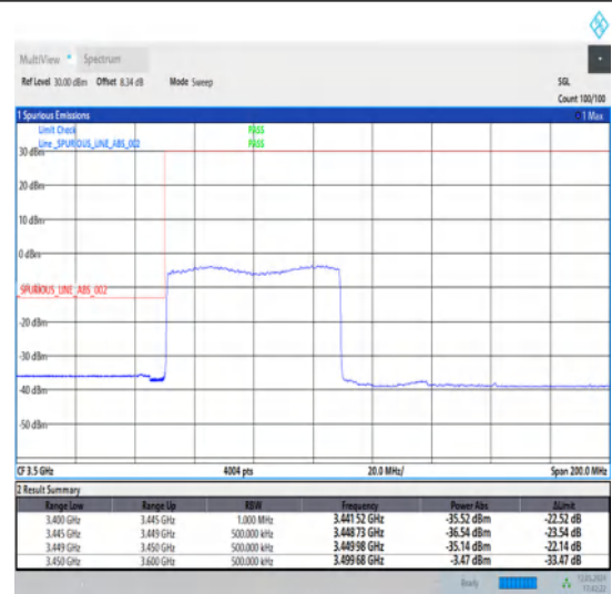
1-N78-3450-3550-30-60-L-3-DFT-PI2BPSK-Outer_Full-162@0-Ant1-1--PASS-see graph
