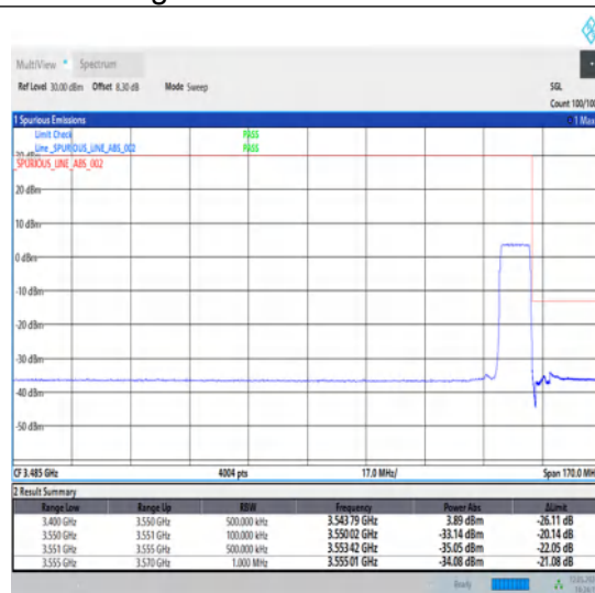
1-N78-3450-3550-30-10-H-3-DFT-PI2BPSK-Outer_Full-24@0-Ant1-1--PASS-see graph
