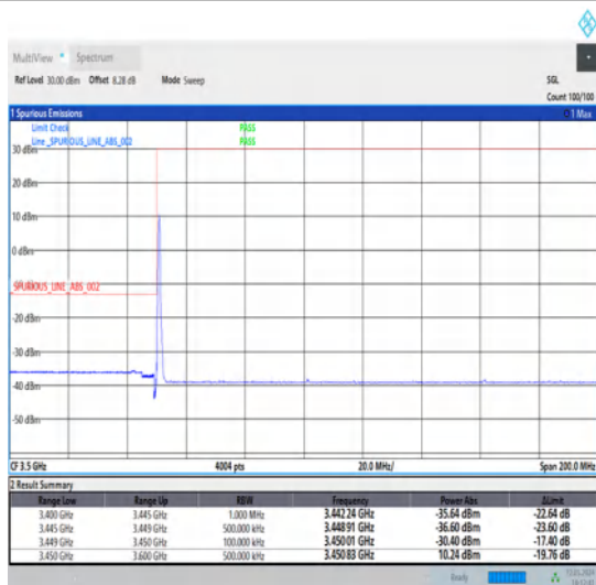
1-N78-3450-3550-30-10-L-4-CP-QPSK-Edge_1RB_Left-1@0-Ant1-1--PASS-see graph
