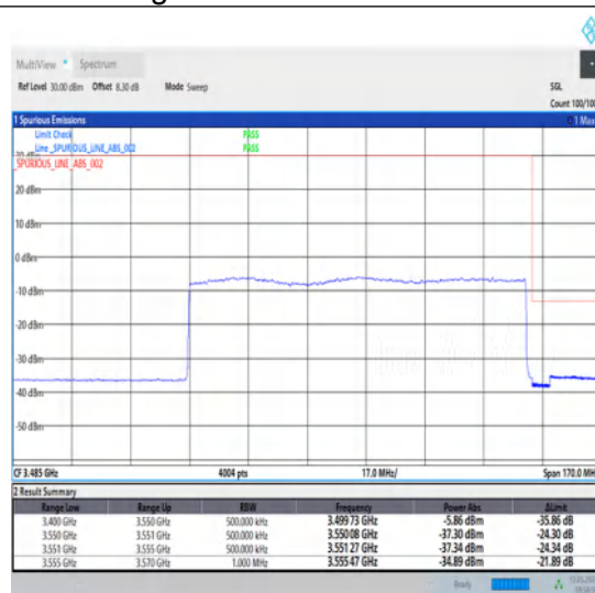
1-N78-3450-3550-30-100-H-3-DFT-PI2BPSK-Outer_Full-270@0-Ant1-1--PASS-see graph
