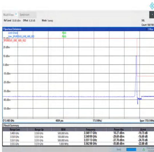
1-N78-3450-3550-30-15-H-5-CP-QPSK-Edge_1RB_Right-1@37-Ant1-1--PASS-see graph
