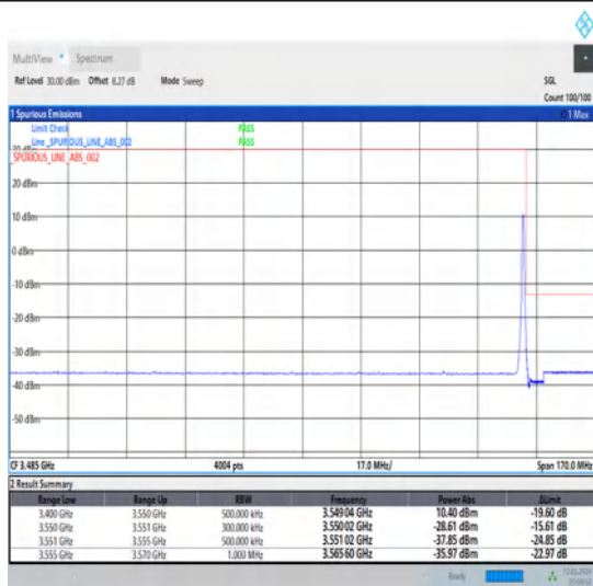
1-N78-3450-3550-30-25-H-5-CP-QPSK-Edge_1RB_Right-1@64-Ant1-1--PASS-see graph
