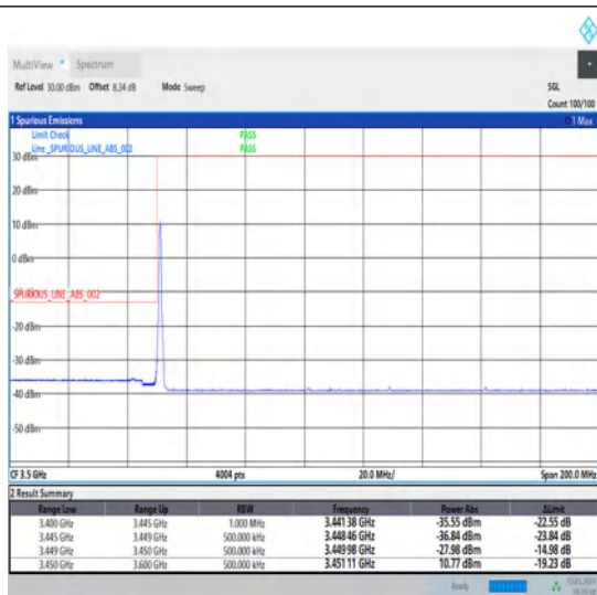
1-N78-3450-3550-30-80-L-1-DFT-PI2BPSK-Edge_1RB_Left-1@0-Ant1-1--PASS-see graph
