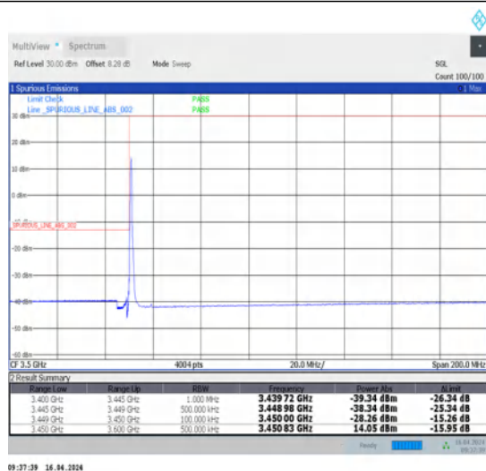
1-N78-3450-3550-30-10-L-4-CP-QPSK-Edge_1RB_Left-1@0-Ant1-1--PASS-see graph
