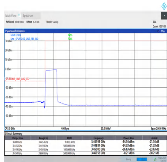
1-N78-3450-3550-30-15-L-6-CP-QPSK-Outer_Full-38@0-Ant1-1--PASS-see graph
