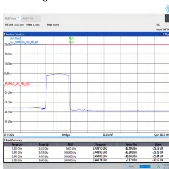
1-N78-3450-3550-30-30-L-3-DFT-PI2BPSK-Outer_Full-75@0-Ant1-1--PASS-see graph
