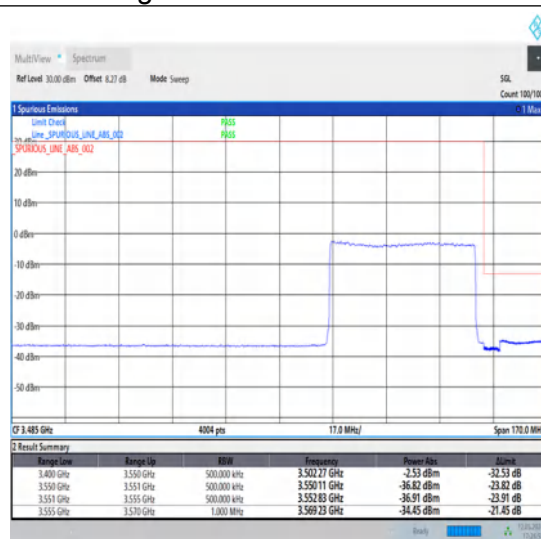
1-N78-3450-3550-30-50-H-3-DFT-PI2BPSK-Outer_Full-128@0-Ant1-1--PASS-see graph
