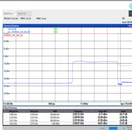
1-N78-3450-3550-30-60-H-6-CP-QPSK-Outer_Full-162@0-Ant1-1--PASS-see graph
