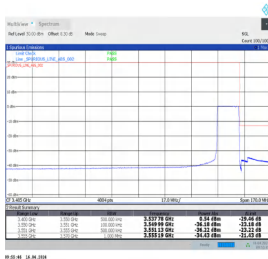
1-N78-3450-3550-30-15-H-6-CP-QPSK-Outer_Full-38@0-Ant1-1--PASS-see graph
