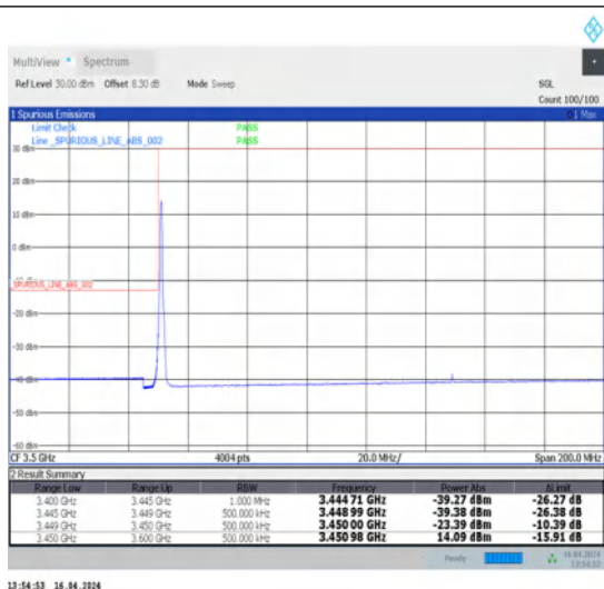
1-N78-3450-3550-30-100-L-1-DFT-PI2BPSK-Edge_1RB_Left-1@0-Ant1-1--PASS-see graph
