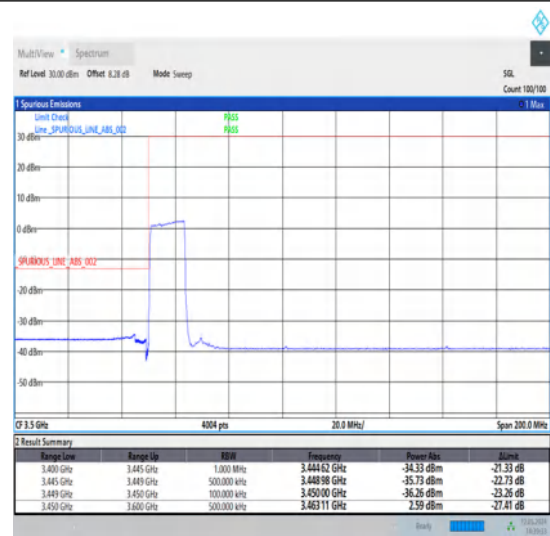
1-N78-3450-3550-30-15-L-3-DFT-PI2BPSK-Outer_Full-36@0-Ant1-1--PASS-see graph
