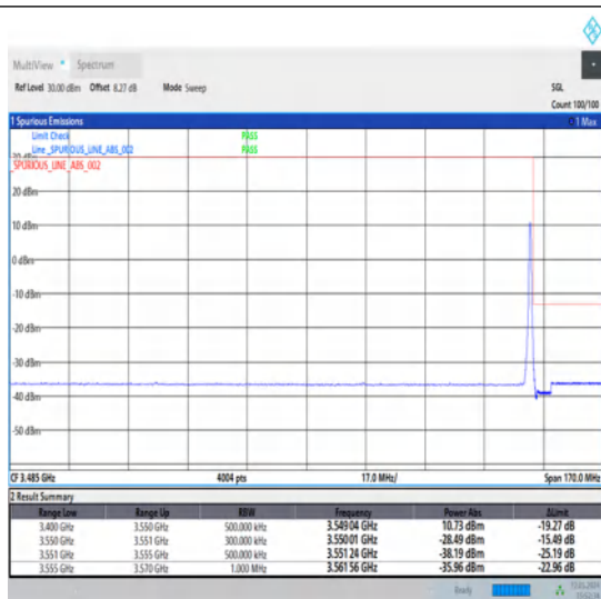
1-N78-3450-3550-30-25-H-2-DFT-PI2BPSK-Edge_1RB_Right-1@64-Ant1-1--PASS-see graph
