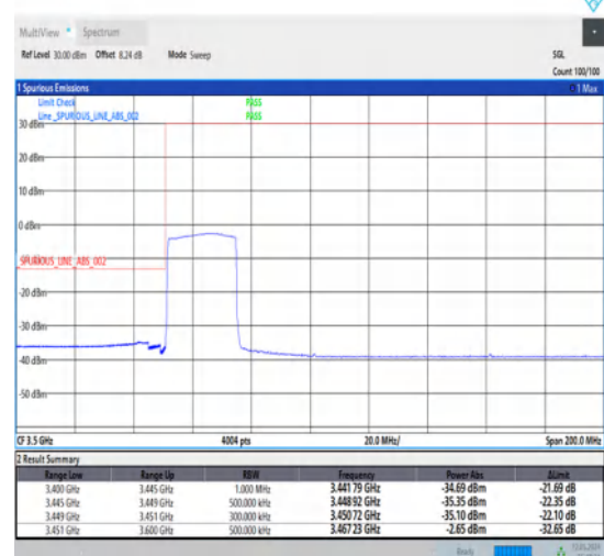
1-N78-3450-3550-30-25-L-6-CP-QPSK-Outer_Full-65@0-Ant1-1--PASS-see graph
