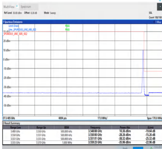
1-N78-3450-3550-30-80-H-5-CP-QPSK-Edge_1RB_Right-1@216-Ant1-1--PASS-see graph
