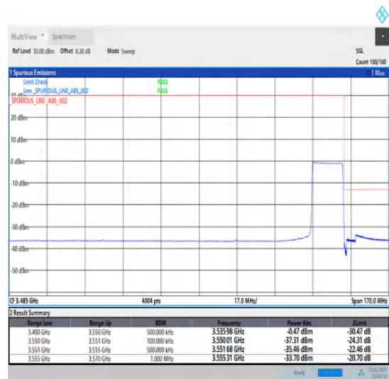
1-N78-3450-3550-30-15-H-6-CP-QPSK-Outer_Full-38@0-Ant1-1--PASS-see graph
