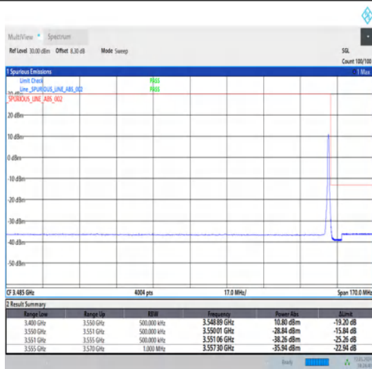
1-N78-3450-3550-30-70-H-2-DFT-PI2BPSK-Edge_1RB_Right-1@188-Ant1-1--PASS-see graph
