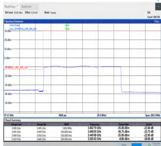
1-N78-3450-3550-30-100-L-6-CP-QPSK-Outer_Full-273@0-Ant1-1--PASS-see graph
