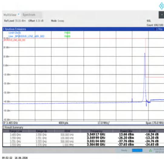
1-N78-3450-3550-30-15-H-5-CP-QPSK-Edge_1RB_Right-1@37-Ant1-1--PASS-see graph
