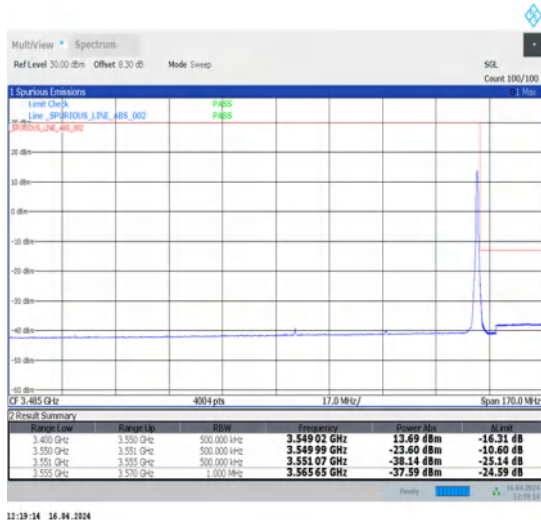
1-N78-3450-3550-30-60-H-5-CP-QPSK-Edge_1RB_Right-1@161-Ant1-1--PASS-see graph
