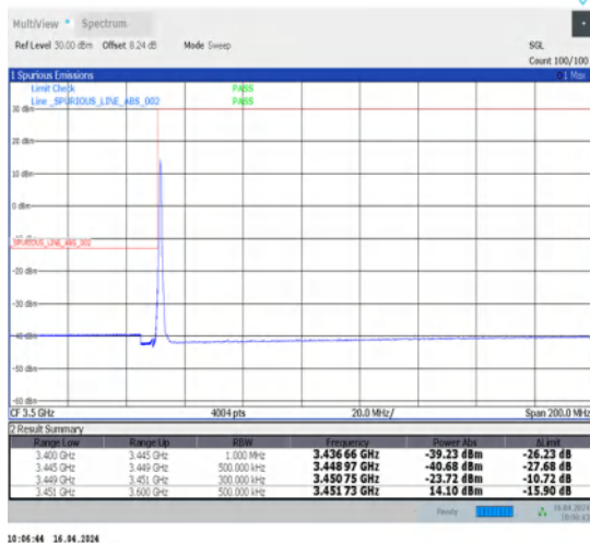
1-N78-3450-3550-30-25-L-4-CP-QPSK-Edge_1RB_Left-1@0-Ant1-1--PASS-see graph
