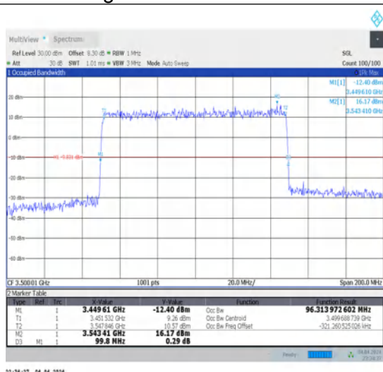
1-N78-3450-3550-30-100-M-3-DFT-16QAM-Outer_Full-270@0-Ant1-96.314-99.800-≤100-PASS
