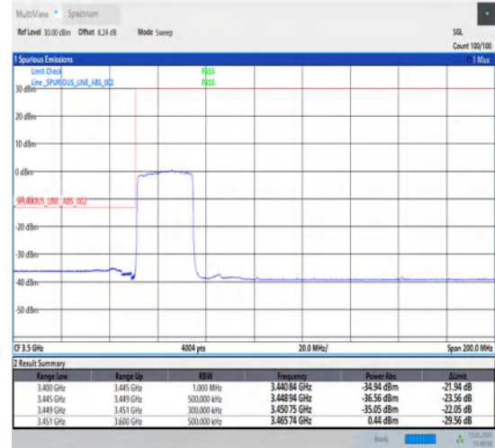
1-N78-3450-3550-30-25-L-3-DFT-PI2BPSK-Outer_Full-64@0-Ant1-1--PASS-see graph
