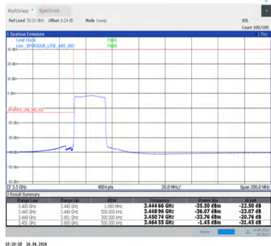
1-N78-3450-3550-30-25-L-6-CP-QPSK-Outer_Full-65@0-Ant1-1--PASS-see graph
