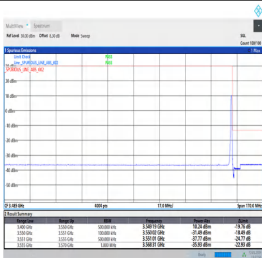
1-N78-3450-3550-30-10-H-5-CP-QPSK-Edge_1RB_Right-1@23-Ant1-1--PASS-see graph
