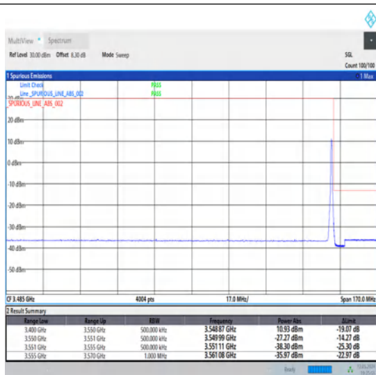
1-N78-3450-3550-30-90-H-2-DFT-PI2BPSK-Edge_1RB_Right-1@244-Ant1-1--PASS-see graph
