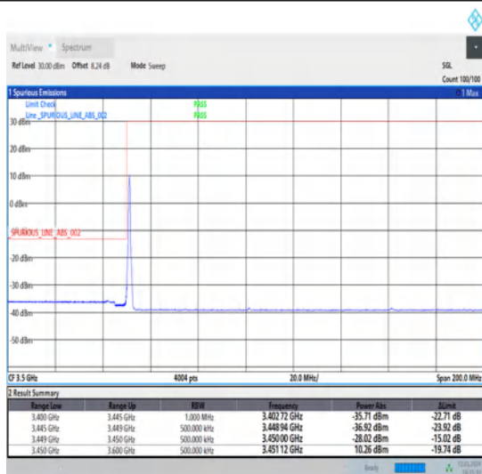
1-N78-3450-3550-30-30-L-4-CP-QPSK-Edge_1RB_Left-1@0-Ant1-1--PASS-see graph
