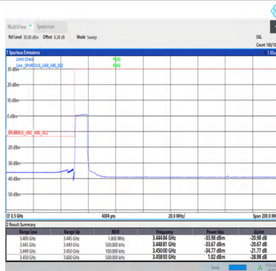
1-N78-3450-3550-30-10-L-6-CP-QPSK-Outer_Full-24@0-Ant1-1--PASS-see graph
