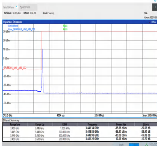
1-N78-3450-3550-30-50-L-4-CP-QPSK-Edge_1RB_Left-1@0-Ant1-1--PASS-see graph
