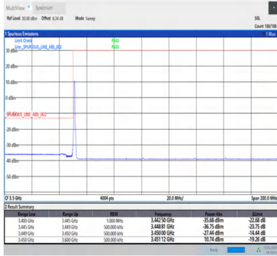
1-N78-3450-3550-30-90-L-1-DFT-PI2BPSK-Edge_1RB_Left-1@0-Ant1-1--PASS-see graph
