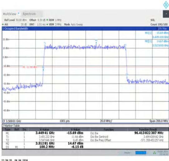
1-N78-3450-3550-30-100-M-4-DFT-64QAM-Outer_Full-270@0-Ant1-96.414-100.200-≤100-PASS
