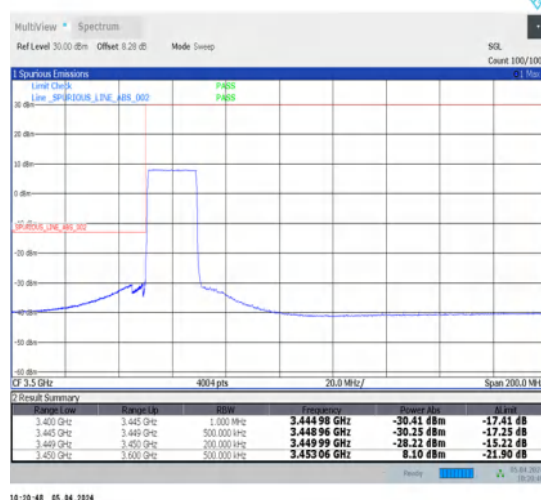
1-N78-3450-3550-30-20-L-6-CP-QPSK-Outer_Full-51@0-Ant1-1--PASS-see graph
