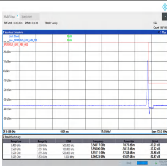
1-N78-3450-3550-30-15-H-2-DFT-PI2BPSK-Edge_1RB_Right-1@37-Ant1-1--PASS-see graph
