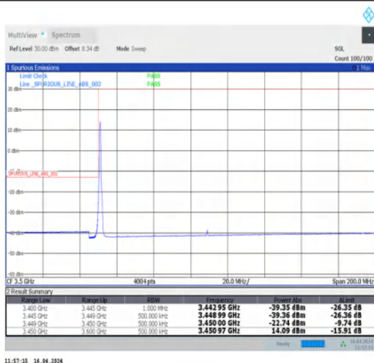
1-N78-3450-3550-30-60-L-1-DFT-PI2BPSK-Edge_1RB_Left-1@0-Ant1-1--PASS-see graph
