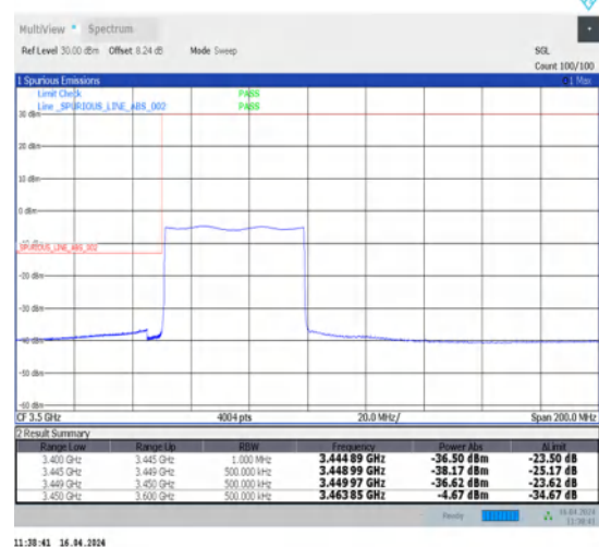
1-N78-3450-3550-30-50-L-6-CP-QPSK-Outer_Full-133@0-Ant1-1--PASS-see graph
