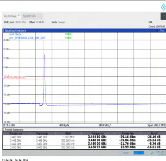
1-N78-3450-3550-30-60-L-4-CP-QPSK-Edge_1RB_Left-1@0-Ant1-1--PASS-see graph
