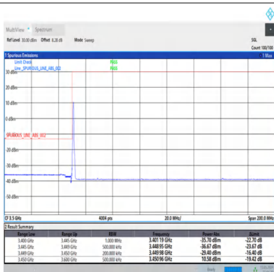
1-N78-3450-3550-30-20-L-1-DFT-PI2BPSK-Edge_1RB_Left-1@0-Ant1-1--PASS-see graph
