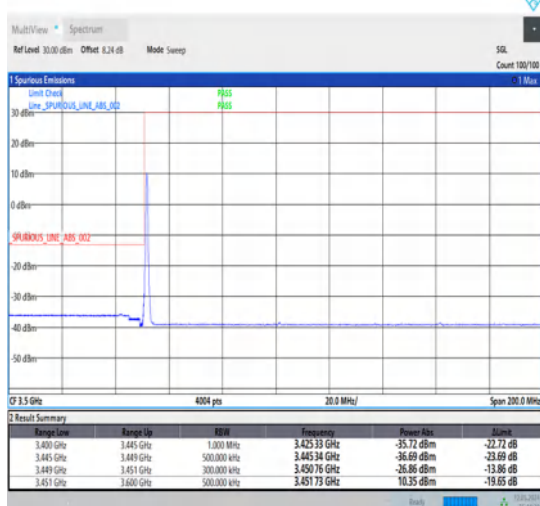
1-N78-3450-3550-30-25-L-4-CP-QPSK-Edge_1RB_Left-1@0-Ant1-1--PASS-see graph
