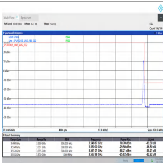
1-N78-3450-3550-30-30-H-2-DFT-PI2BPSK-Edge_1RB_Right-1@77-Ant1-1--PASS-see graph
