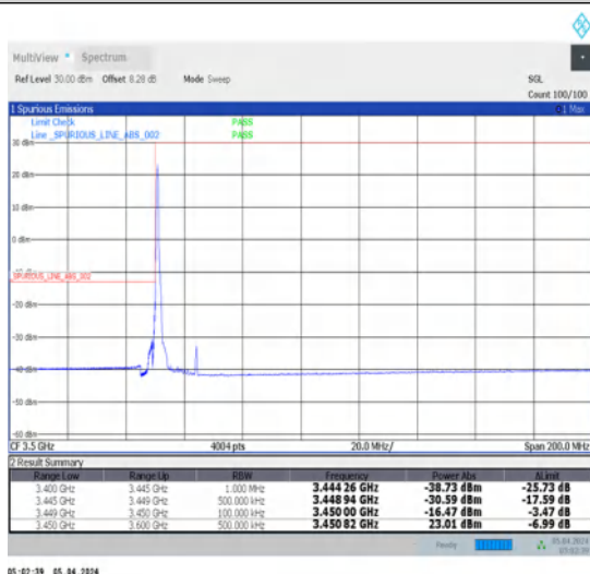
1-N78-3450-3550-30-15-L-4-CP-QPSK-Edge_1RB_Left-1@0-Ant1-1--PASS-see graph
