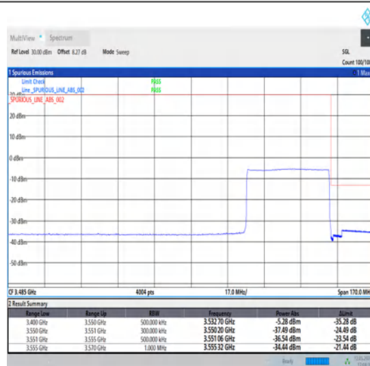
1-N78-3450-3550-30-40-H-6-CP-QPSK-Outer_Full-106@0-Ant1-1--PASS-see graph
