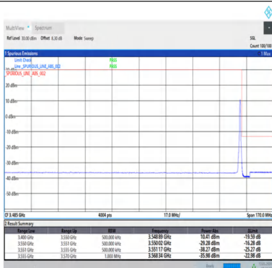
1-N78-3450-3550-30-70-H-5-CP-QPSK-Edge_1RB_Right-1@188-Ant1-1--PASS-see graph
