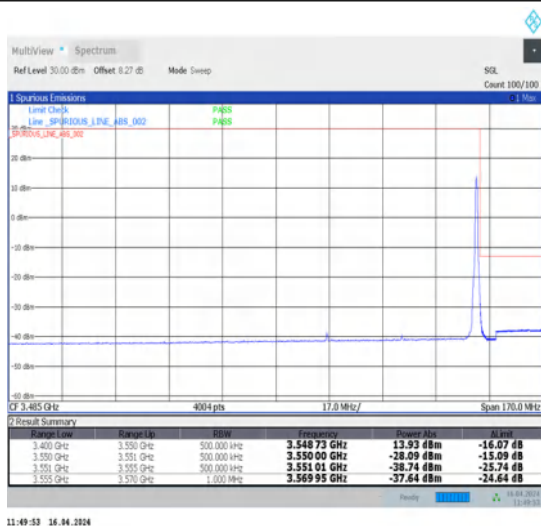
1-N78-3450-3550-30-50-H-5-CP-QPSK-Edge_1RB_Right-1@132-Ant1-1--PASS-see graph
