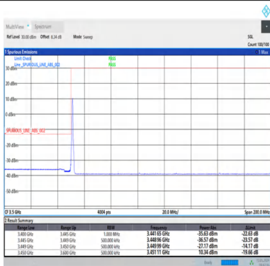
1-N78-3450-3550-30-80-L-4-CP-QPSK-Edge_1RB_Left-1@0-Ant1-1--PASS-see graph
