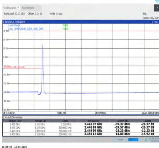
1-N78-3450-3550-30-30-L-4-CP-QPSK-Edge_1RB_Left-1@0-Ant1-1--PASS-see graph
