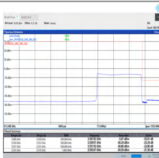
1-N78-3450-3550-30-50-H-6-CP-QPSK-Outer_Full-133@0-Ant1-1--PASS-see graph
