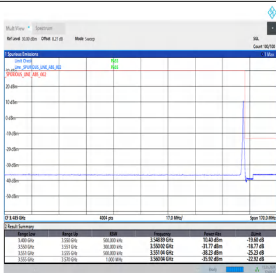
1-N78-3450-3550-30-40-H-5-CP-QPSK-Edge_1RB_Right-1@105-Ant1-1--PASS-see graph
