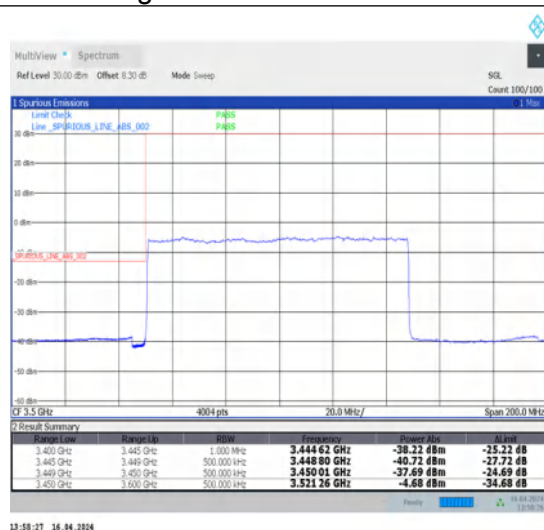
1-N78-3450-3550-30-100-L-3-DFT-PI2BPSK-Outer_Full-270@0-Ant1-1--PASS-see graph
