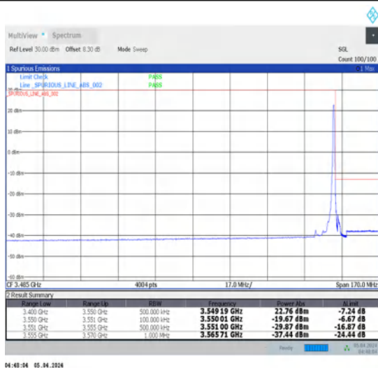
1-N78-3450-3550-30-10-H-5-CP-QPSK-Edge_1RB_Right-1@23-Ant1-1--PASS-see graph
