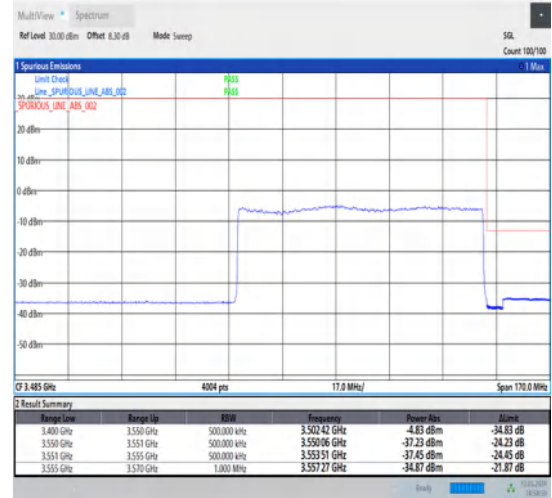
1-N78-3450-3550-30-80-H-3-DFT-PI2BPSK-Outer_Full-216@0-Ant1-1--PASS-see graph
