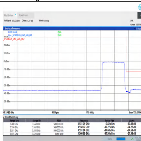
1-N78-3450-3550-30-30-H-3-DFT-PI2BPSK-Outer_Full-75@0-Ant1-1--PASS-see graph
