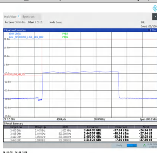
1-N78-3450-3550-30-100-L-6-CP-QPSK-Outer_Full-273@0-Ant1-1--PASS-see graph
