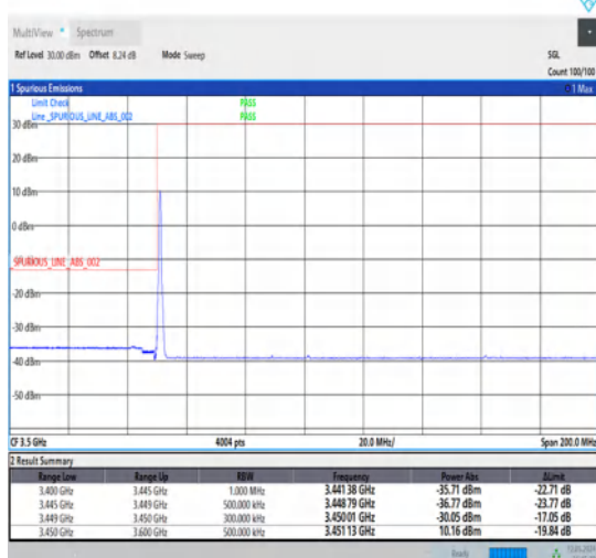
1-N78-3450-3550-30-40-L-4-CP-QPSK-Edge_1RB_Left-1@0-Ant1-1--PASS-see graph
