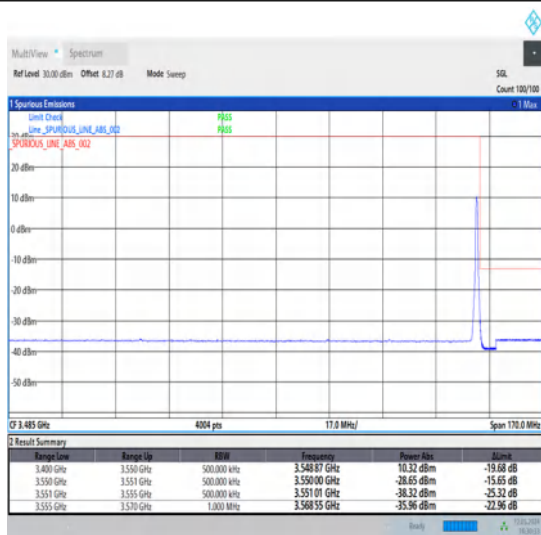
1-N78-3450-3550-30-30-H-5-CP-QPSK-Edge_1RB_Right-1@77-Ant1-1--PASS-see graph
