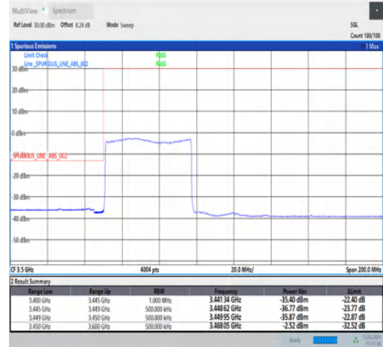
1-N78-3450-3550-30-50-L-3-DFT-PI2BPSK-Outer_Full-128@0-Ant1-1--PASS-see graph
