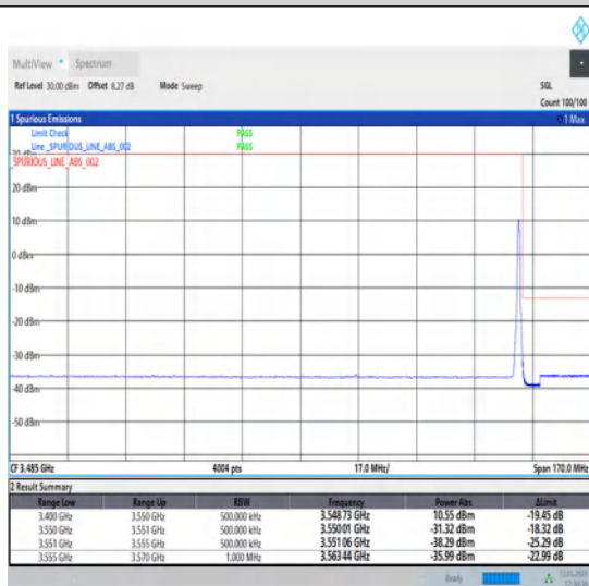
1-N78-3450-3550-30-50-H-5-CP-QPSK-Edge_1RB_Right-1@132-Ant1-1--PASS-see graph
