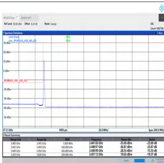
1-N78-3450-3550-30-30-L-1-DFT-PI2BPSK-Edge_1RB_Left-1@0-Ant1-1--PASS-see graph
