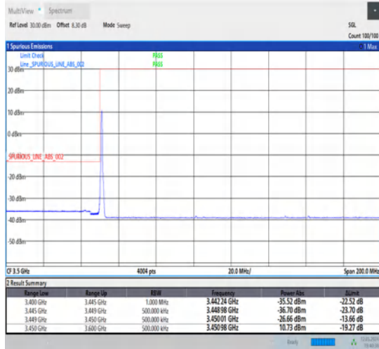
1-N78-3450-3550-30-100-L-1-DFT-PI2BPSK-Edge_1RB_Left-1@0-Ant1-1--PASS-see graph
