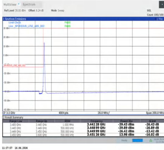
1-N78-3450-3550-30-50-L-1-DFT-PI2BPSK-Edge_1RB_Left-1@0-Ant1-1--PASS-see graph
