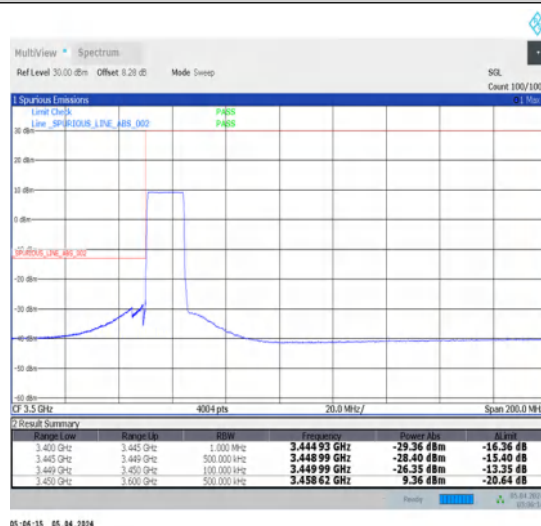
1-N78-3450-3550-30-15-L-6-CP-QPSK-Outer_Full-38@0-Ant1-1--PASS-see graph
