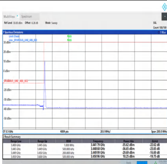
1-N78-3450-3550-30-20-L-4-CP-QPSK-Edge_1RB_Left-1@0-Ant1-1--PASS-see graph
