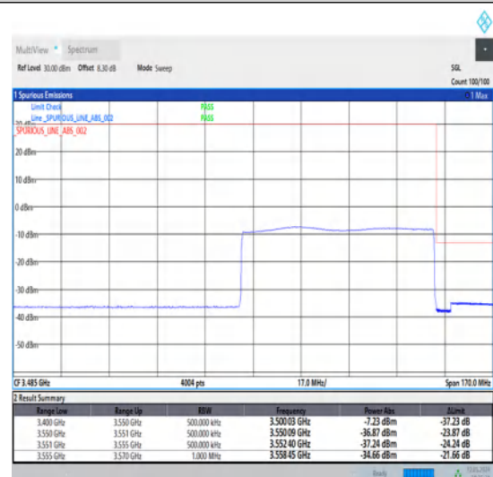
1-N78-3450-3550-30-70-H-6-CP-QPSK-Outer_Full-189@0-Ant1-1--PASS-see graph
