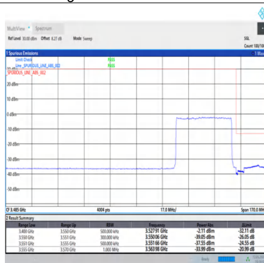
1-N78-3450-3550-30-40-H-3-DFT-PI2BPSK-Outer_Full-100@0-Ant1-1--PASS-see graph
