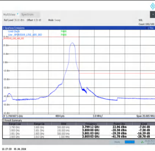
1-N78-3700-3800-N78-3700-380030-10-H-2-DFT-PI2BPSK-Edge_1RB_Right-1@23-Ant1-1--PASS-see graph
