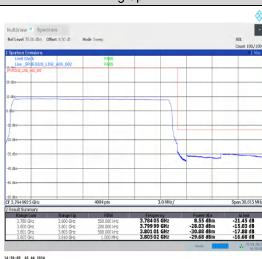
1-N78-3700-3800-N78-3700-380030-20-H-3-DFT-PI2BPSK-Outer_Full-50@0-Ant1-1--PASS-see graph
