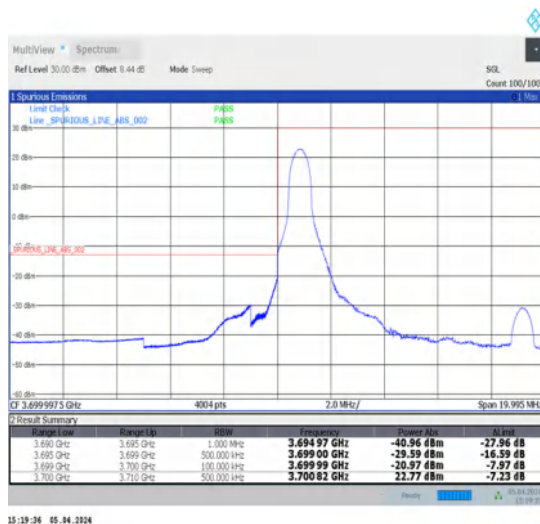
1-N78-3700-3800-N78-3700-380030-10-L-4-CP-QPSK-Edge_1RB_Left-1@0-Ant1-1--PASS-see graph
