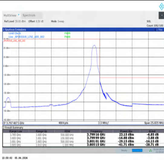
1-N78-3700-3800-N78-3700-380030-15-H-2-DFT-PI2BPSK-Edge_1RB_Right-1@37-Ant1-1--PASS-see graph
