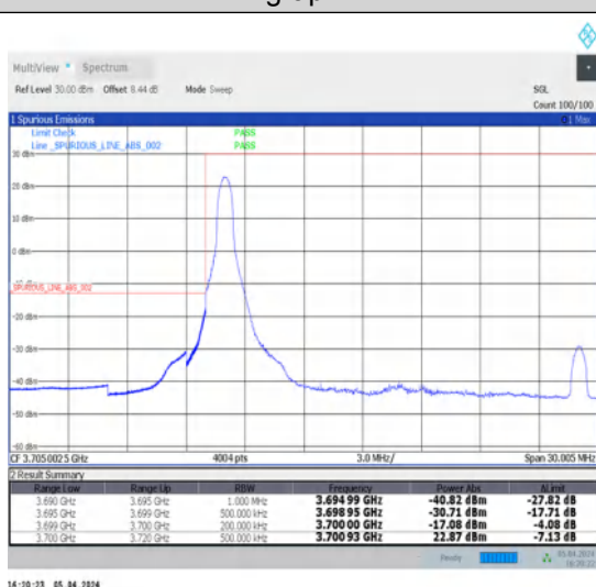
1-N78-3700-3800-N78-3700-380030-20-L-4-CP-QPSK-Edge_1RB_Left-1@0-Ant1-1--PASS-see graph
