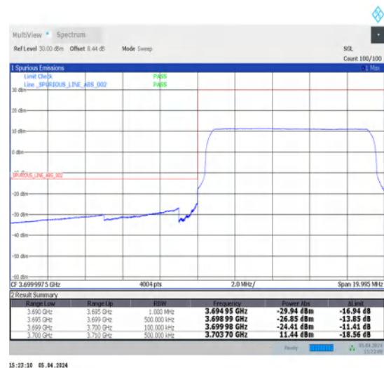
1-N78-3700-3800-N78-3700-380030-10-L-6-CP-QPSK-Outer_Full-24@0-Ant1-1--PASS-see graph
