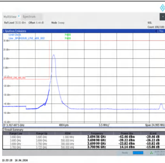
1-N78-3700-3800-N78-3700-380030-25-L-4-CP-QPSK-Edge_1RB_Left-1@0-Ant1-1--PASS-see graph
