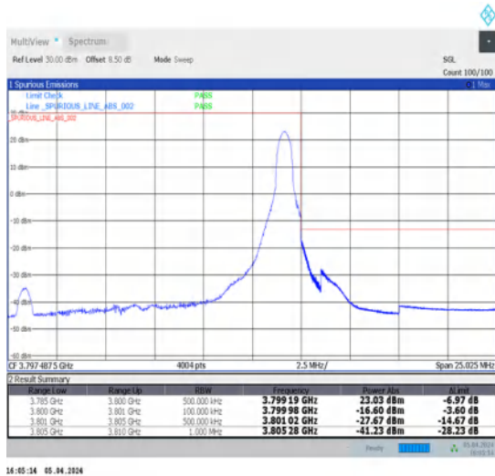
1-N78-3700-3800-N78-3700-380030-15-H-5-CP-QPSK-Edge_1RB_Right-1@37-Ant1-1--PASS-see graph
