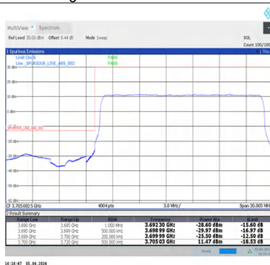
1-N78-3700-3800-N78-3700-380030-20-L-3-DFT-PI2BPSK-Outer_Full-50@0-Ant1-1--PASS-see graph
