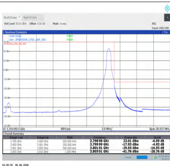
1-N78-3700-3800-N78-3700-380030-20-H-2-DFT-PI2BPSK-Edge_1RB_Right-1@50-Ant1-1--PASS-see graph
