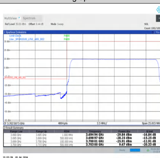
1-N78-3700-3800-N78-3700-380030-15-L-6-CP-QPSK-Outer_Full-38@0-Ant1-1--PASS-see graph
