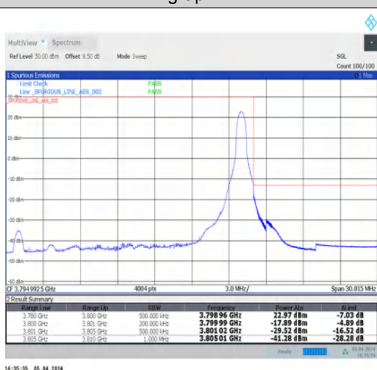
1-N78-3700-3800-N78-3700-380030-20-H-5-CP-QPSK-Edge_1RB_Right-1@50-Ant1-1--PASS-see graph
