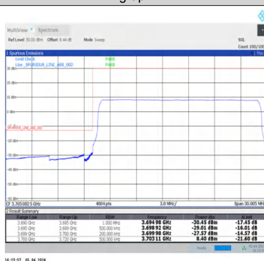
1-N78-3700-3800-N78-3700-380030-20-L-6-CP-QPSK-Outer_Full-51@0-Ant1-1--PASS-see graph
