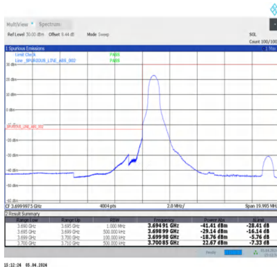
1-N78-3700-3800-N78-3700-380030-10-L-1-DFT-PI2BPSK-Edge_1RB_Left-1@0-Ant1-1--PASS-see graph
