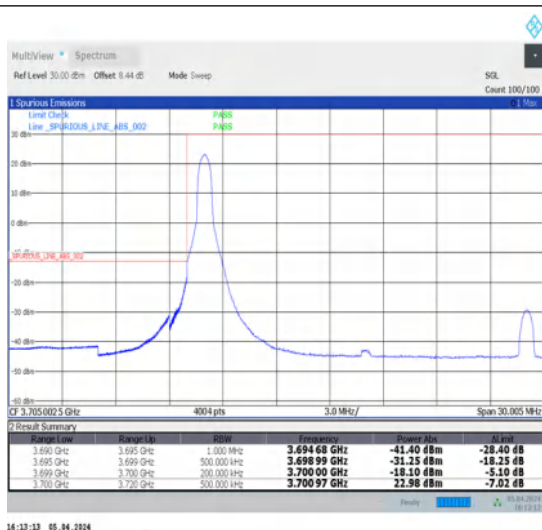
1-N78-3700-3800-N78-3700-380030-20-L-1-DFT-PI2BPSK-Edge_1RB_Left-1@0-Ant1-1--PASS-see graph
