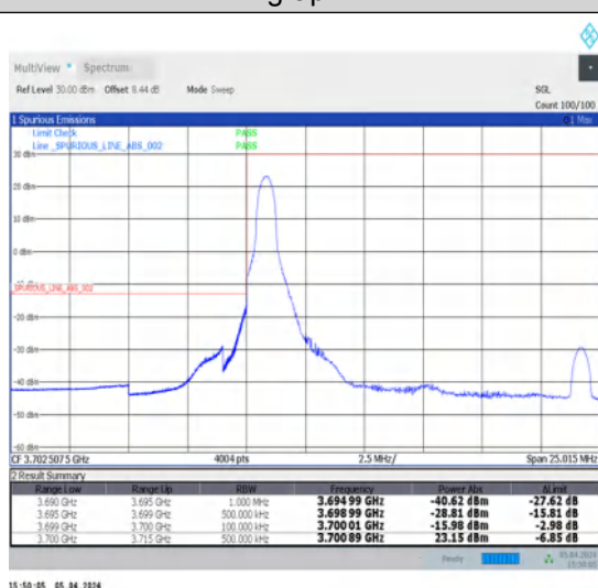
1-N78-3700-3800-N78-3700-380030-15-L-4-CP-QPSK-Edge_1RB_Left-1@0-Ant1-1--PASS-see graph
