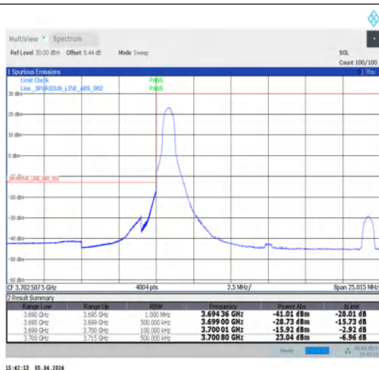
1-N78-3700-3800-N78-3700-380030-15-L-1-DFT-PI2BPSK-Edge_1RB_Left-1@0-Ant1-1--PASS-see graph
