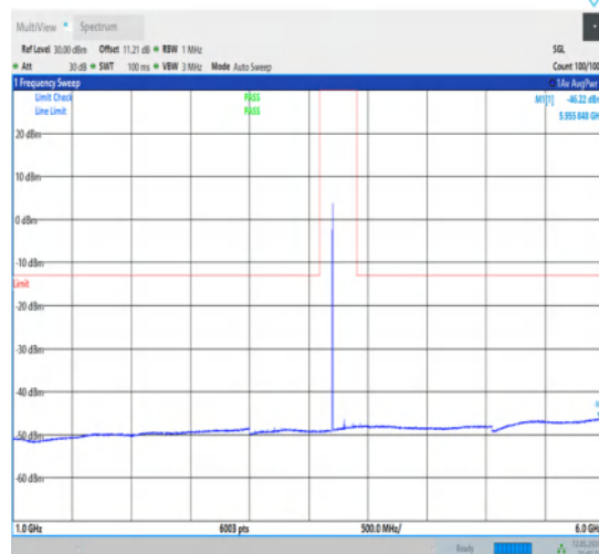
1-N78-3700-3800-30-100-H-1-DFT-QPSK- Edge_1RB_Left-1@0-1000-6000-Ant1-5955.85-- 46.22--13-PASS
