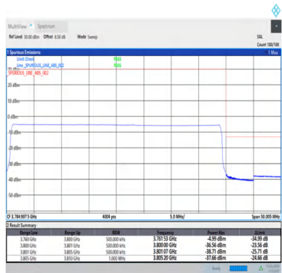
1-N78-3700-3800-30-40-H-6-CP-QPSK-Outer_Full-106@0-Ant1-1--PASS-see graph
