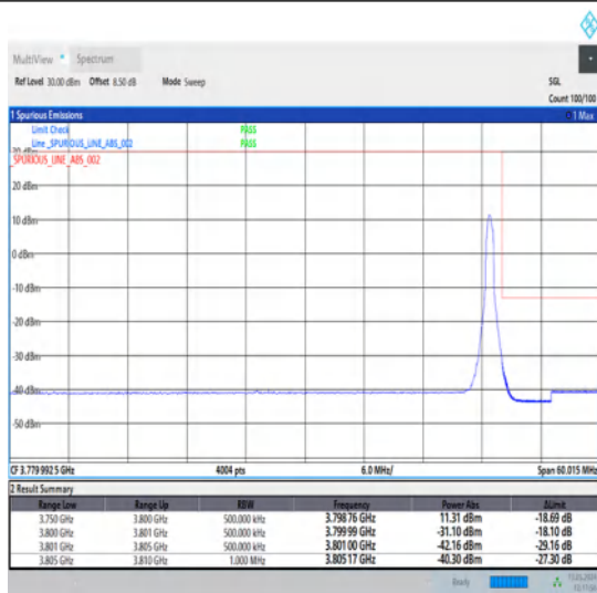
1-N78-3700-3800-30-50-H-2-DFT-PI2BPSK-Edge_1RB_Right-1@132-Ant1-1--PASS-see graph
