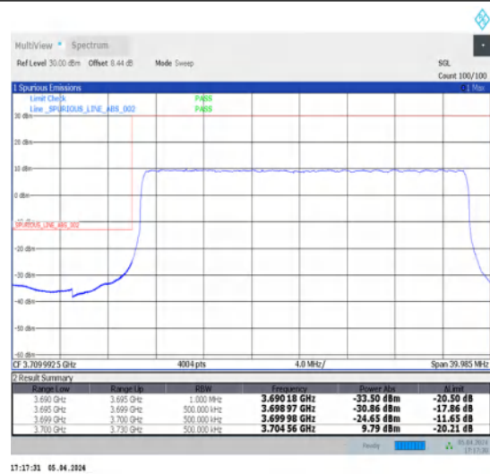
1-N78-3700-3800-N78-3700-380030-30-L-3-DFT-PI2BPSK-Outer_Full-75@0-Ant1-1--PASS-see graph
