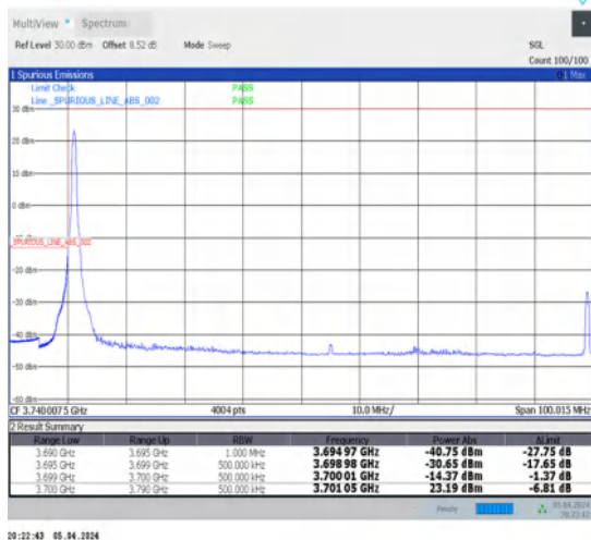
1-N78-3700-3800-N78-3700-380030-90-L-4-CP-QPSK-Edge_1RB_Left-1@0-Ant1-1--PASS-see graph
