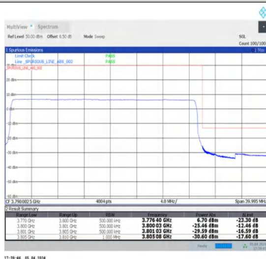
1-N78-3700-3800-N78-3700-380030-30-H-3-DFT-PI2BPSK-Outer_Full-75@0-Ant1-1--PASS-see graph
