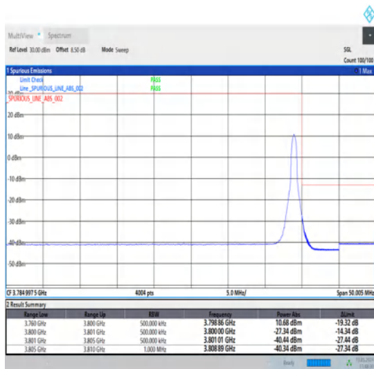
1-N78-3700-3800-30-40-H-5-CP-QPSK-Edge_1RB_Right-1@105-Ant1-1--PASS-see graph
