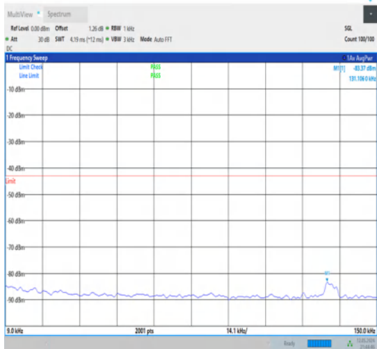
1-N78-3700-3800-30-100-H-1-DFT-QPSK- Edge_1RB_Left-1@0-0.009-0.15-Ant1-0.13--83.37-- 43-PASS
