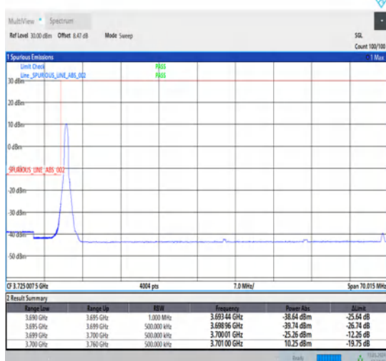
1-N78-3700-3800-30-60-L-4-CP-QPSK-Edge_1RB_Left-1@0-Ant1-1--PASS-see graph
