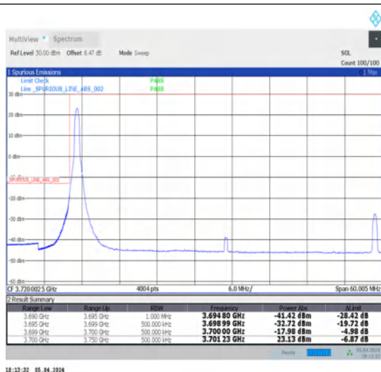
1-N78-3700-3800-N78-3700-380030-50-L-1-DFT-PI2BPSK-Edge_1RB_Left-1@0-Ant1-1--PASS-see graph
