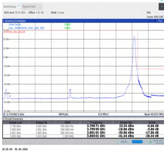
1-N78-3700-3800-N78-3700-380030-50-H-5-CP-QPSK-Edge_1RB_Right-1@132-Ant1-1--PASS-see graph
