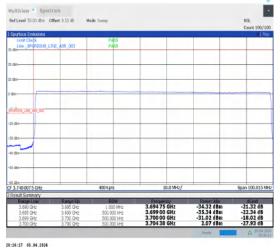
1-N78-3700-3800-N78-3700-380030-90-L-6-CP-QPSK-Outer_Full-245@0-Ant1-1--PASS-see graph
