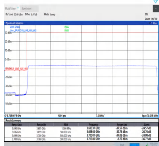
1-N78-3700-3800-30-60-L-6-CP-QPSK-Outer_Full-162@0-Ant1-1--PASS-see graph
