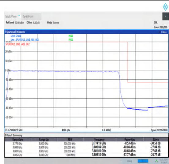
1-N78-3700-3800-30-30-H-3-DFT-PI2BPSK-Outer_Full-75@0-Ant1-1--PASS-see graph
