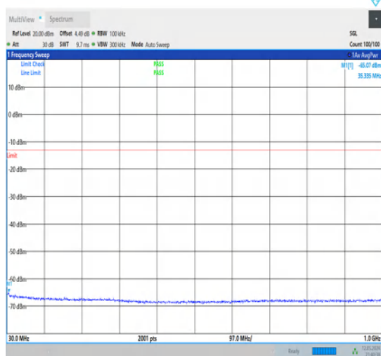
1-N78-3700-3800-30-100-L-1-DFT-QPSK- Edge_1RB_Left-1@0-30-1000-Ant1-35.34--65.07-- 13-PASS
