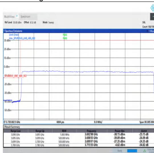
1-N78-3700-3800-30-80-L-3-DFT-PI2BPSK-Outer_Full-216@0-Ant1-1--PASS-see graph
