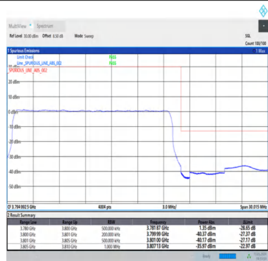
1-N78-3700-3800-30-20-H-3-DFT-PI2BPSK-Outer_Full-50@0-Ant1-1--PASS-see graph
