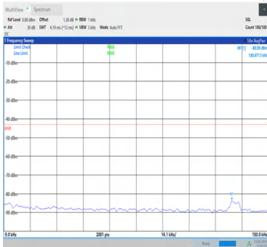
1-N78-3700-3800-30-100-M-1-DFT-QPSK- Edge_1RB_Left-1@0-0.009-0.15-Ant1-0.13--83.59-- 43-PASS
