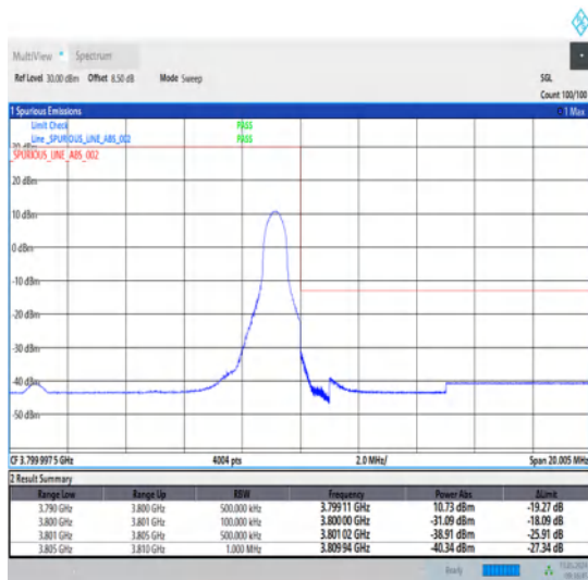
1-N78-3700-3800-30-10-H-5-CP-QPSK-Edge_1RB_Right-1@23-Ant1-1--PASS-see graph
