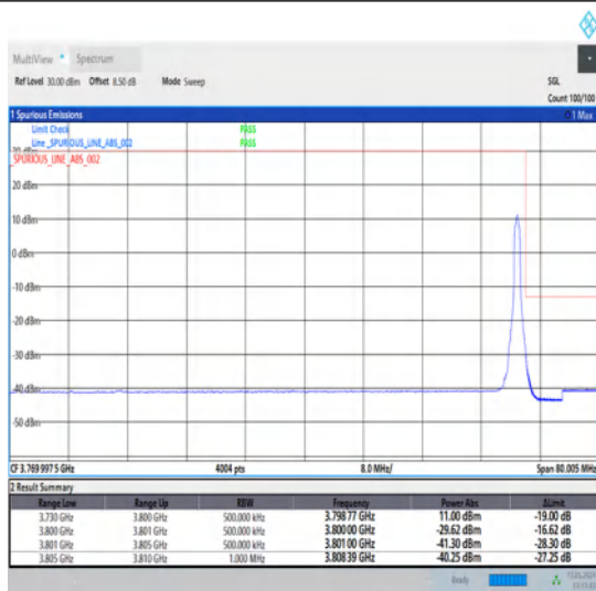
1-N78-3700-3800-30-70-H-2-DFT-PI2BPSK-Edge_1RB_Right-1@188-Ant1-1--PASS-see graph
