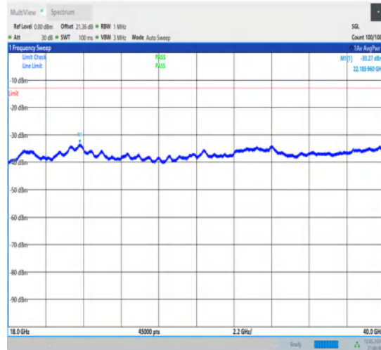
1-N78-3700-3800-30-100-H-1-DFT-QPSK- Edge_1RB_Left-1@0-18000-40000-Ant1-22185.96-- 33.27--13-PASS
