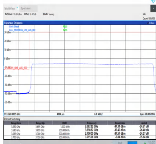
1-N78-3700-3800-30-50-L-6-CP-QPSK-Outer_Full-133@0-Ant1-1--PASS-see graph
