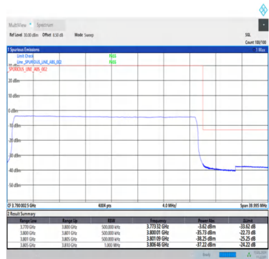
1-N78-3700-3800-30-30-H-6-CP-QPSK-Outer_Full-78@0-Ant1-1--PASS-see graph
