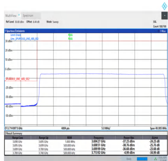
1-N78-3700-3800-30-40-L-6-CP-QPSK-Outer_Full-106@0-Ant1-1--PASS-see graph
