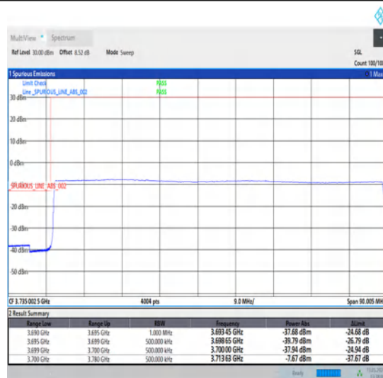
1-N78-3700-3800-30-80-L-6-CP-QPSK-Outer_Full-217@0-Ant1-1--PASS-see graph
