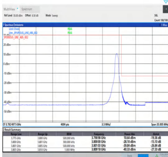
1-N78-3700-3800-30-25-H-5-CP-QPSK-Edge_1RB_Right-1@64-Ant1-1--PASS-see graph
