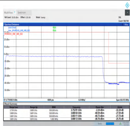
1-N78-3700-3800-30-50-H-3-DFT-PI2BPSK-Outer_Full-128@0-Ant1-1--PASS-see graph
