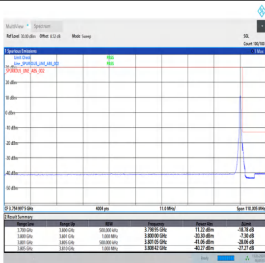
1-N78-3700-3800-30-100-H-2-DFT-PI2BPSK-Edge_1RB_Right-1@272-Ant1-1--PASS-see graph
