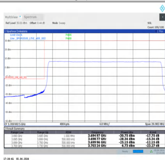
1-N78-3700-3800-N78-3700-380030-30-L-6-CP-QPSK-Outer_Full-78@0-Ant1-1--PASS-see graph
