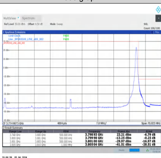
1-N78-3700-3800-N78-3700-380030-60-H-5-CP-QPSK-Edge_1RB_Right-1@161-Ant1-1--PASS-see graph
