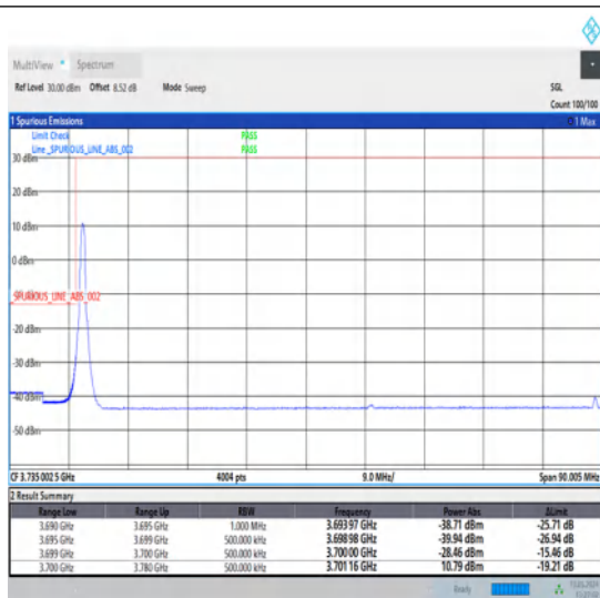
1-N78-3700-3800-30-80-L-1-DFT-PI2BPSK-Edge_1RB_Left-1@0-Ant1-1--PASS-see graph
