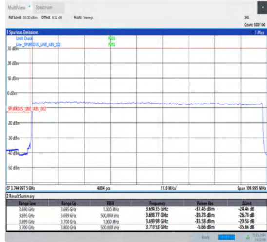
1-N78-3700-3800-30-100-L-3-DFT-PI2BPSK-Outer_Full-270@0-Ant1-1--PASS-see graph
