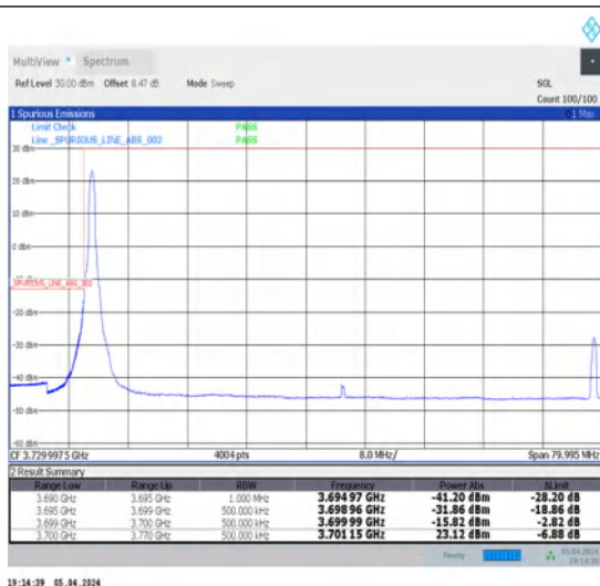
1-N78-3700-3800-N78-3700-380030-70-L-1-DFT-PI2BPSK-Edge_1RB_Left-1@0-Ant1-1--PASS-see graph
