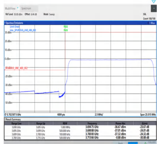
1-N78-3700-3800-30-15-L-6-CP-QPSK-Outer_Full-38@0-Ant1-1--PASS-see graph
