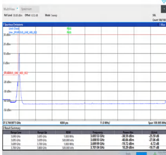
1-N78-3700-3800-30-100-L-4-CP-QPSK-Edge_1RB_Left-1@0-Ant1-1--PASS-see graph
