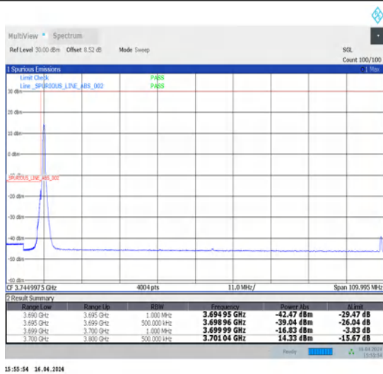
1-N78-3700-3800-N78-3700-380030-100-L-1-DFT-PI2BPSK-Edge_1RB_Left-1@0-Ant1-1--PASS-see graph
