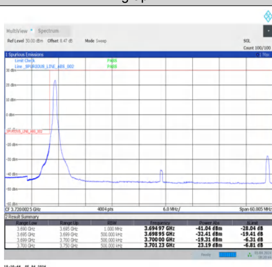
1-N78-3700-3800-N78-3700-380030-50-L-4-CP-QPSK-Edge_1RB_Left-1@0-Ant1-1--PASS-see graph
