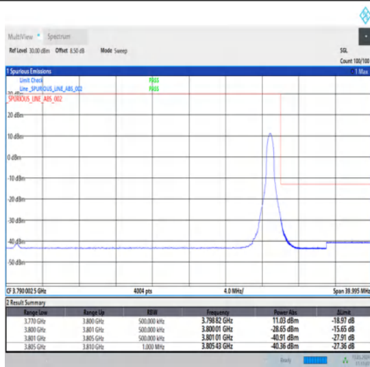
1-N78-3700-3800-30-30-H-2-DFT-PI2BPSK-Edge_1RB_Right-1@77-Ant1-1--PASS-see graph
