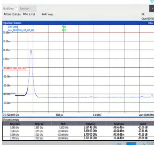
1-N78-3700-3800-30-50-L-4-CP-QPSK-Edge_1RB_Left-1@0-Ant1-1--PASS-see graph
