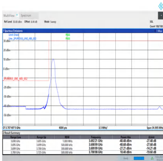
1-N78-3700-3800-30-25-L-4-CP-QPSK-Edge_1RB_Left-1@0-Ant1-1--PASS-see graph
