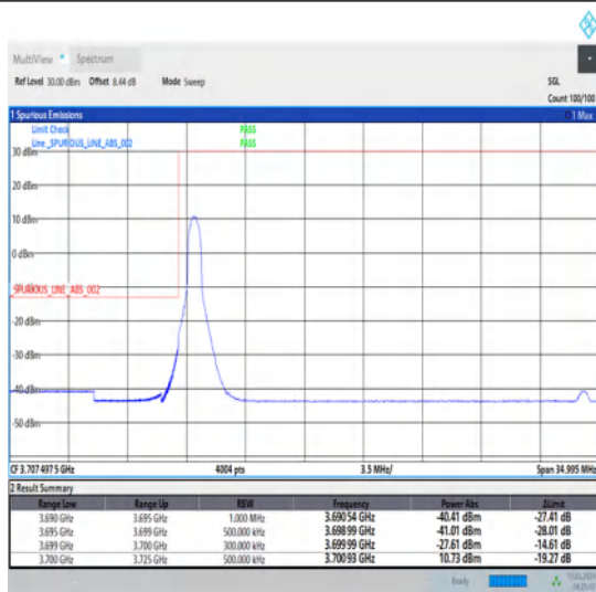
1-N78-3700-3800-30-25-L-1-DFT-PI2BPSK-Edge_1RB_Left-1@0-Ant1-1--PASS-see graph
