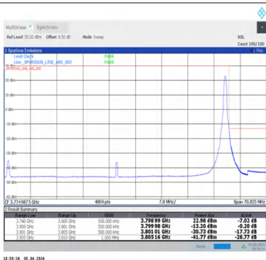
1-N78-3700-3800-N78-3700-380030-60-H-2-DFT-PI2BPSK-Edge_1RB_Right-1@161-Ant1-1--PASS-see graph
