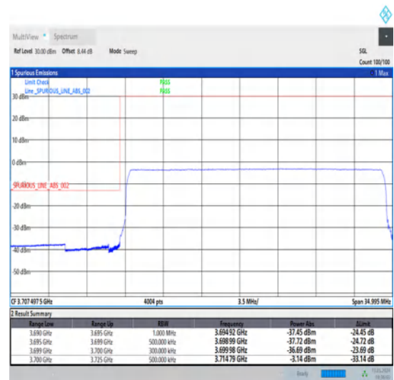
1-N78-3700-3800-30-25-L-6-CP-QPSK-Outer_Full-65@0-Ant1-1--PASS-see graph
