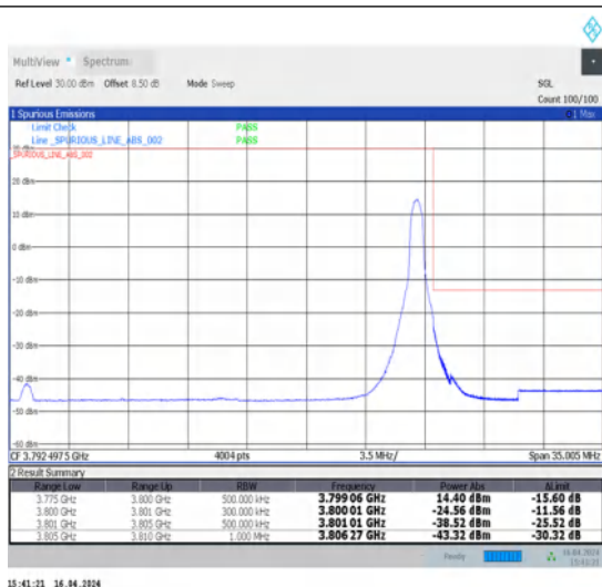
1-N78-3700-3800-N78-3700-380030-25-H-2-DFT-PI2BPSK-Edge_1RB_Right-1@64-Ant1-1--PASS-see graph
