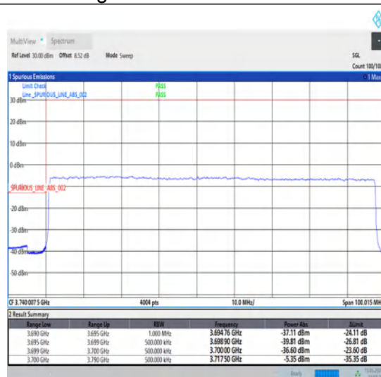
1-N78-3700-3800-30-90-L-3-DFT-PI2BPSK-Outer_Full-240@0-Ant1-1--PASS-see graph
