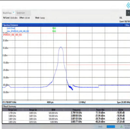
1-N78-3700-3800-30-10-H-2-DFT-PI2BPSK-Edge_1RB_Right-1@23-Ant1-1--PASS-see graph
