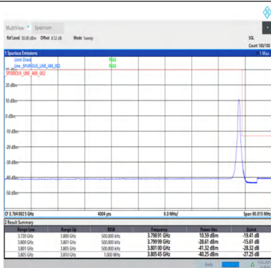
1-N78-3700-3800-30-80-H-5-CP-QPSK-Edge_1RB_Right-1@216-Ant1-1--PASS-see graph
