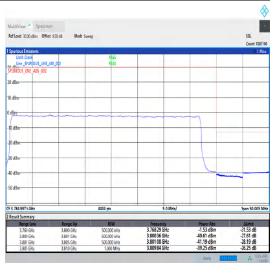
1-N78-3700-3800-30-40-H-3-DFT-PI2BPSK-Outer_Full-100@0-Ant1-1--PASS-see graph
