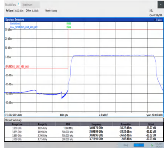
1-N78-3700-3800-30-15-L-3-DFT-PI2BPSK-Outer_Full-36@0-Ant1-1--PASS-see graph
