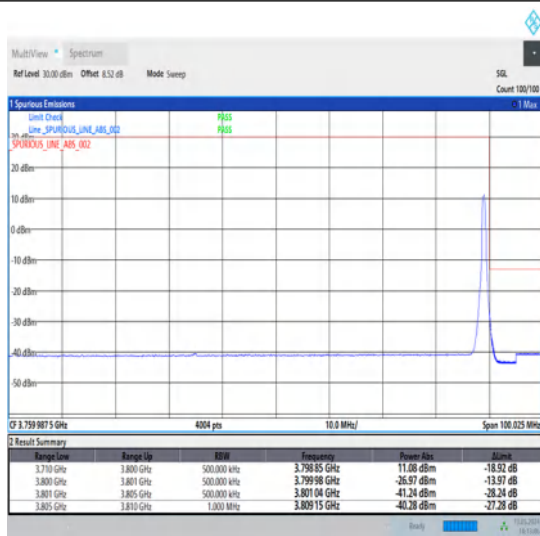
1-N78-3700-3800-30-90-H-2-DFT-PI2BPSK-Edge_1RB_Right-1@244-Ant1-1--PASS-see graph
