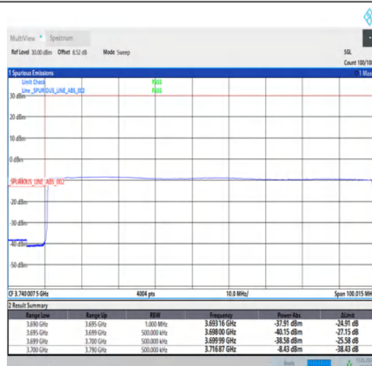
1-N78-3700-3800-30-90-L-6-CP-QPSK-Outer_Full-245@0-Ant1-1--PASS-see graph
