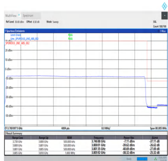
1-N78-3700-3800-30-70-H-6-CP-QPSK-Outer_Full-189@0-Ant1-1--PASS-see graph
