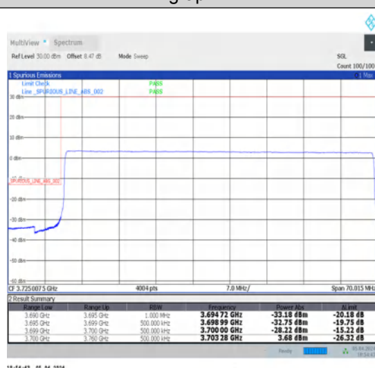
1-N78-3700-3800-N78-3700-380030-60-L-6-CP-QPSK-Outer_Full-162@0-Ant1-1--PASS-see graph
