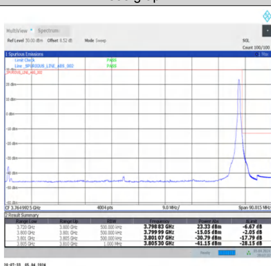
1-N78-3700-3800-N78-3700-380030-80-H-5-CP-QPSK-Edge_1RB_Right-1@216-Ant1-1--PASS-see graph
