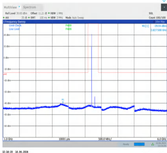
1-N78-3700-3800-N78-3700-380030-100-H-1-DFT-PI2BPSK-Inner_1RB_Left-1@1-1000-6000-Ant1-2742.00--39.94--13-PASS
