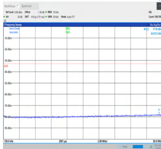
1-N78-3700-3800-30-100-H-1-DFT-QPSK- Edge_1RB_Left-1@0-0.15-30-Ant1-29.37--77.33--33- PASS
