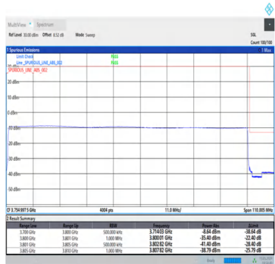
1-N78-3700-3800-30-100-H-6-CP-QPSK-Outer_Full-273@0-Ant1-1--PASS-see graph
