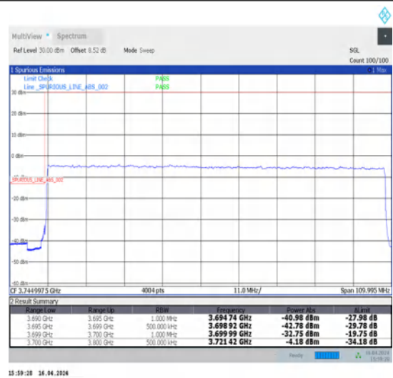
1-N78-3700-3800-N78-3700-380030-100-L-3-DFT-PI2BPSK-Outer_Full-270@0-Ant1-1--PASS-see graph
