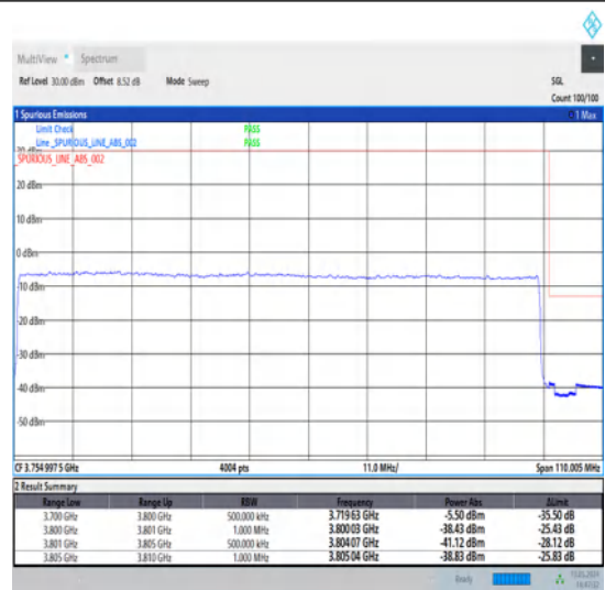
1-N78-3700-3800-30-100-H-3-DFT-PI2BPSK-Outer_Full-270@0-Ant1-1--PASS-see graph
