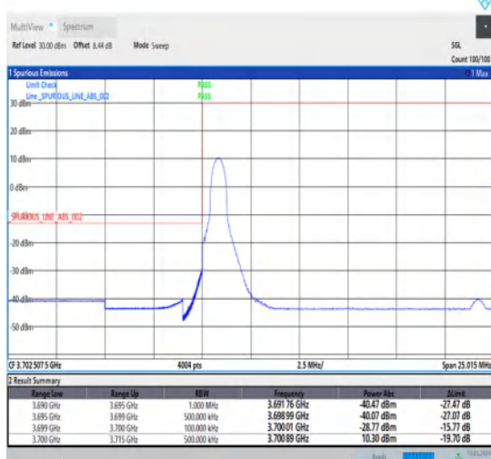
1-N78-3700-3800-30-15-L-4-CP-QPSK-Edge_1RB_Left-1@0-Ant1-1--PASS-see graph
