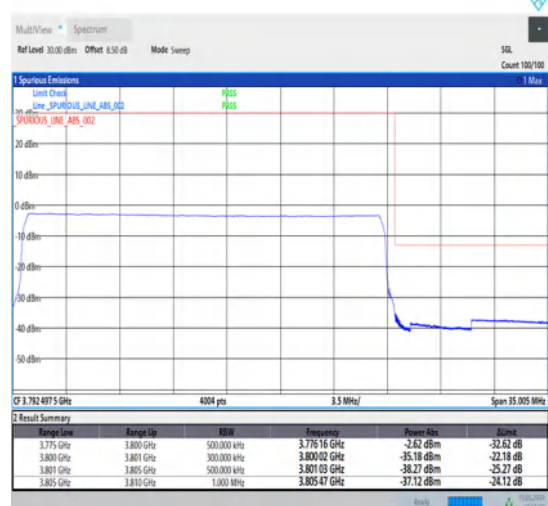
1-N78-3700-3800-30-25-H-6-CP-QPSK-Outer_Full-65@0-Ant1-1--PASS-see graph
