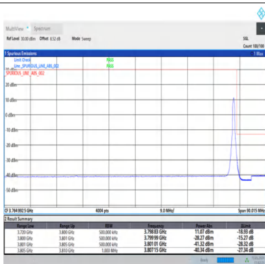
1-N78-3700-3800-30-80-H-2-DFT-PI2BPSK-Edge_1RB_Right-1@216-Ant1-1--PASS-see graph
