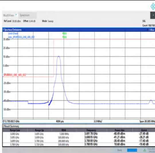
1-N78-3700-3800-30-20-L-1-DFT-PI2BPSK-Edge_1RB_Left-1@0-Ant1-1--PASS-see graph
