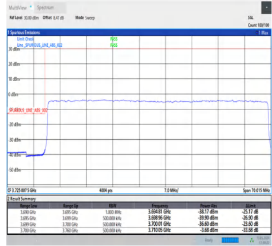
1-N78-3700-3800-30-60-L-3-DFT-PI2BPSK-Outer_Full-162@0-Ant1-1--PASS-see graph
