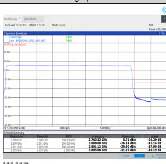
1-N78-3700-3800-N78-3700-380030-40-H-3-DFT-PI2BPSK-Outer_Full-100@0-Ant1-1--PASS-see graph
