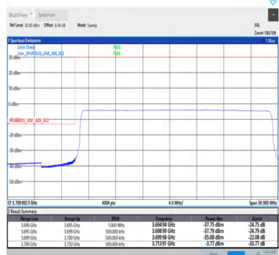
1-N78-3700-3800-30-30-L-6-CP-QPSK-Outer_Full-78@0-Ant1-1--PASS-see graph
