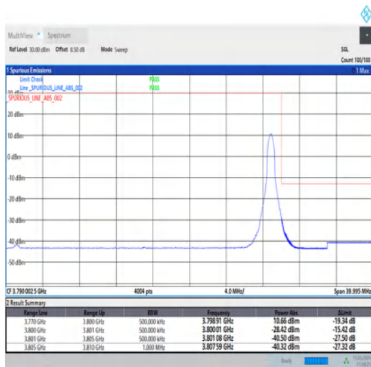
1-N78-3700-3800-30-30-H-5-CP-QPSK-Edge_1RB_Right-1@77-Ant1-1--PASS-see graph
