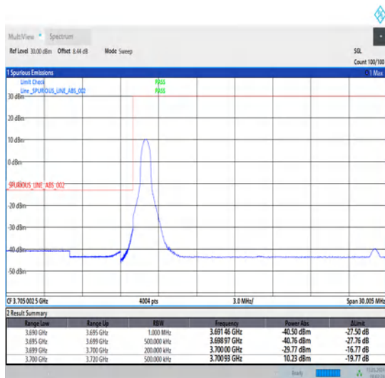
1-N78-3700-3800-30-20-L-4-CP-QPSK-Edge_1RB_Left-1@0-Ant1-1--PASS-see graph
