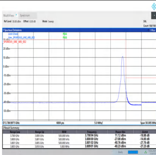
1-N78-3700-3800-30-40-H-2-DFT-PI2BPSK-Edge_1RB_Right-1@105-Ant1-1--PASS-see graph
