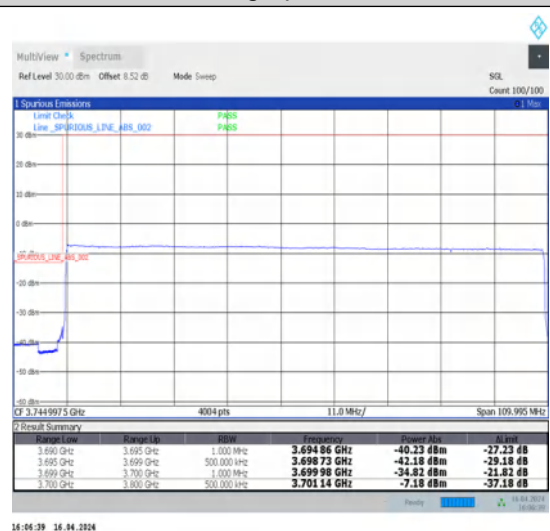
1-N78-3700-3800-N78-3700-380030-100-L-6-CP-QPSK-Outer_Full-273@0-Ant1-1--PASS-see graph
