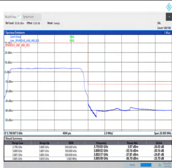
1-N78-3700-3800-30-10-H-3-DFT-PI2BPSK-Outer_Full-24@0-Ant1-1--PASS-see graph
