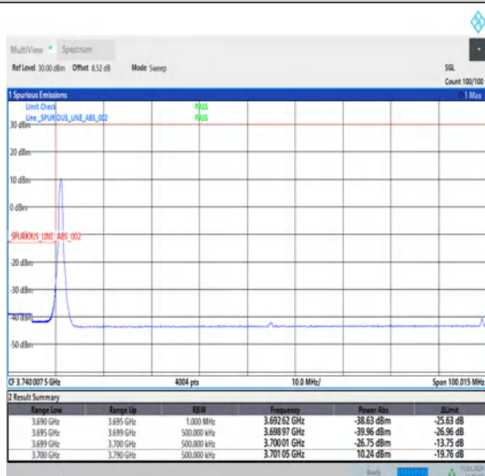
1-N78-3700-3800-30-90-L-4-CP-QPSK-Edge_1RB_Left-1@0-Ant1-1--PASS-see graph
