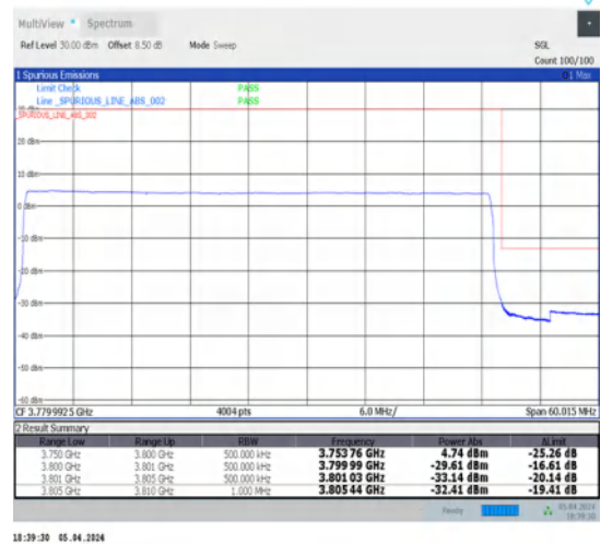
1-N78-3700-3800-N78-3700-380030-50-H-6-CP-QPSK-Outer_Full-133@0-Ant1-1--PASS-see graph
