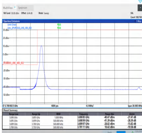
1-N78-3700-3800-30-30-L-4-CP-QPSK-Edge_1RB_Left-1@0-Ant1-1--PASS-see graph
