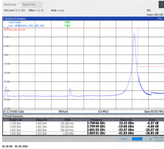
1-N78-3700-3800-N78-3700-380030-50-H-2-DFT-PI2BPSK-Edge_1RB_Right-1@132-Ant1-1--PASS-see graph
