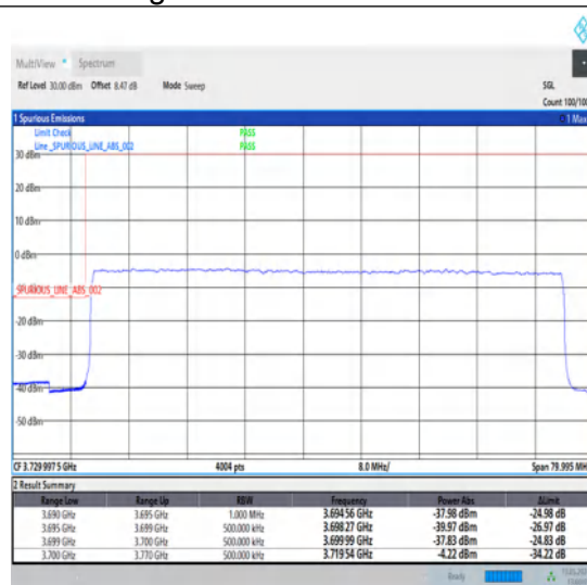
1-N78-3700-3800-30-70-L-3-DFT-PI2BPSK-Outer_Full-180@0-Ant1-1--PASS-see graph
