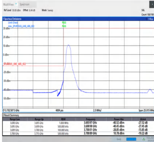
1-N78-3700-3800-30-15-L-1-DFT-PI2BPSK-Edge_1RB_Left-1@0-Ant1-1--PASS-see graph
