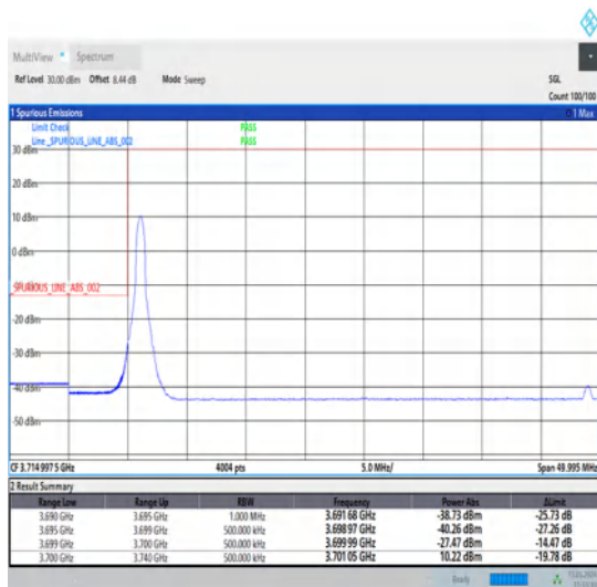
1-N78-3700-3800-30-40-L-4-CP-QPSK-Edge_1RB_Left-1@0-Ant1-1--PASS-see graph
