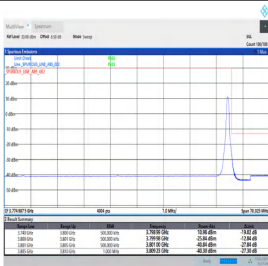
1-N78-3700-3800-30-60-H-2-DFT-PI2BPSK-Edge_1RB_Right-1@161-Ant1-1--PASS-see graph
