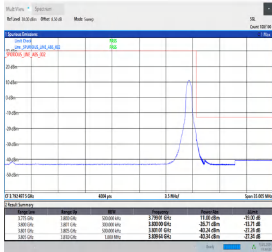
1-N78-3700-3800-30-25-H-2-DFT-PI2BPSK-Edge_1RB_Right-1@64-Ant1-1--PASS-see graph
