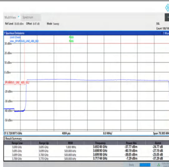
1-N78-3700-3800-30-70-L-6-CP-QPSK-Outer_Full-189@0-Ant1-1--PASS-see graph
