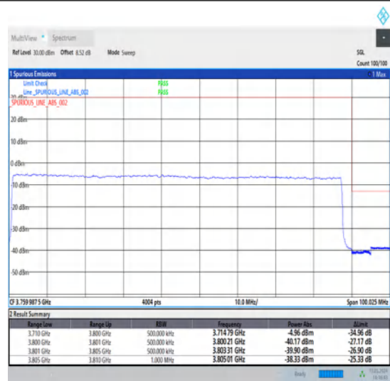
1-N78-3700-3800-30-90-H-3-DFT-PI2BPSK-Outer_Full-240@0-Ant1-1--PASS-see graph
