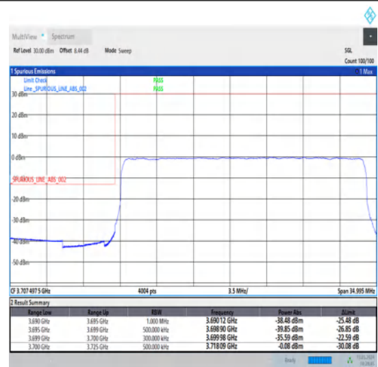
1-N78-3700-3800-30-25-L-3-DFT-PI2BPSK-Outer_Full-64@0-Ant1-1--PASS-see graph
