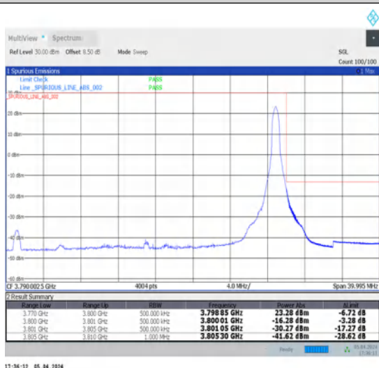
1-N78-3700-3800-N78-3700-380030-30-H-5-CP-QPSK-Edge_1RB_Right-1@77-Ant1-1--PASS-see graph
