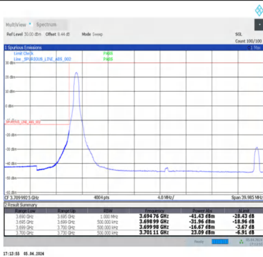
1-N78-3700-3800-N78-3700-380030-30-L-1-DFT-PI2BPSK-Edge_1RB_Left-1@0-Ant1-1--PASS-see graph
