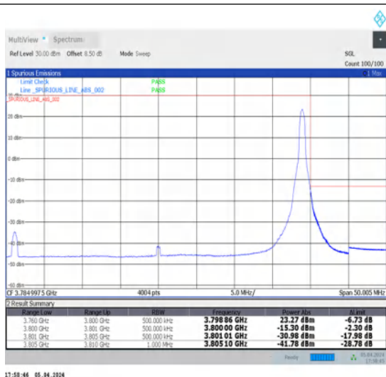
1-N78-3700-3800-N78-3700-380030-40-H-2-DFT-PI2BPSK-Edge_1RB_Right-1@105-Ant1-1--PASS-see graph
