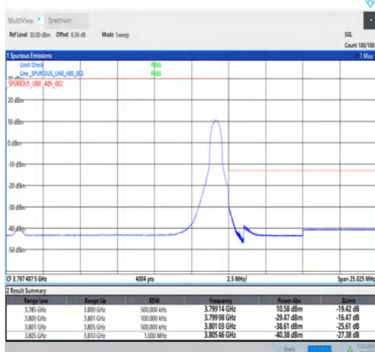
1-N78-3700-3800-30-15-H-5-CP-QPSK-Edge_1RB_Right-1@37-Ant1-1--PASS-see graph
