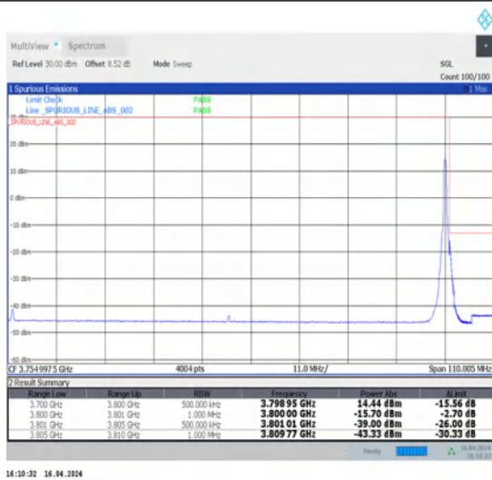
1-N78-3700-3800-N78-3700-380030-100-H-2-DFT-PI2BPSK-Edge_1RB_Right-1@272-Ant1-1--PASS-see graph
