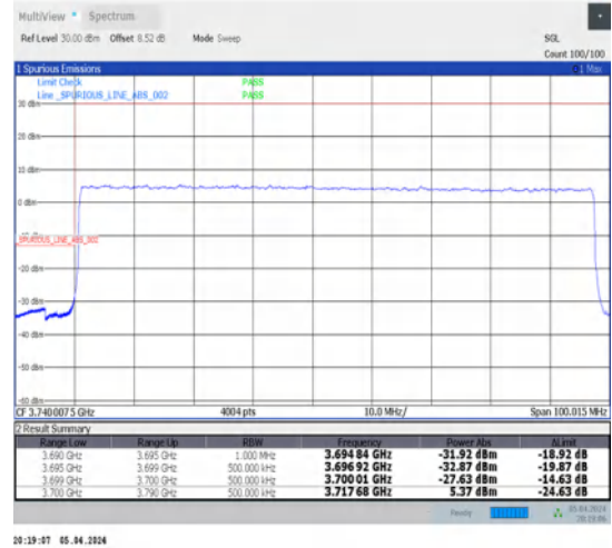
1-N78-3700-3800-N78-3700-380030-90-L-3-DFT-PI2BPSK-Outer_Full-240@0-Ant1-1--PASS-see graph
