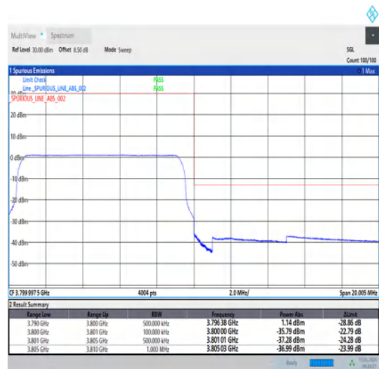
1-N78-3700-3800-30-10-H-6-CP-QPSK-Outer_Full-24@0-Ant1-1--PASS-see graph
