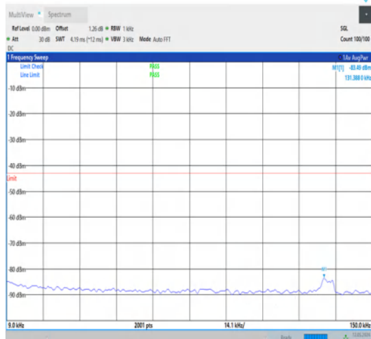
1-N78-3700-3800-30-100-L-1-DFT-QPSK- Edge_1RB_Left-1@0-0.009-0.15-Ant1-0.13--83.49-- 43-PASS
