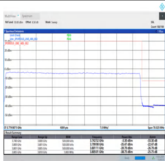
1-N78-3700-3800-30-60-H-3-DFT-PI2BPSK-Outer_Full-162@0-Ant1-1--PASS-see graph
