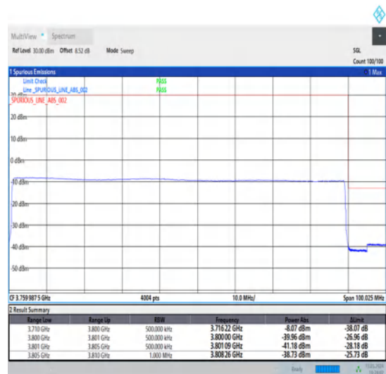
1-N78-3700-3800-30-90-H-6-CP-QPSK-Outer_Full-245@0-Ant1-1--PASS-see graph
