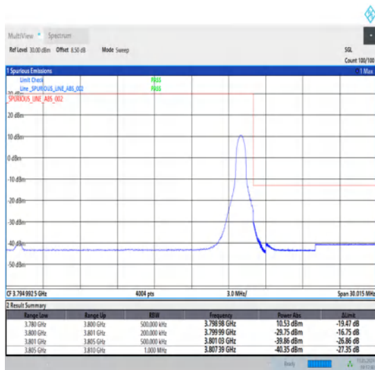
1-N78-3700-3800-30-20-H-5-CP-QPSK-Edge_1RB_Right-1@50-Ant1-1--PASS-see graph
