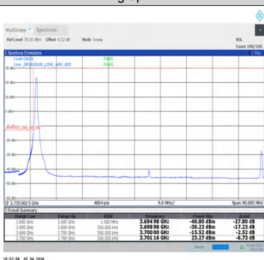
1-N78-3700-3800-N78-3700-380030-80-L-4-CP-QPSK-Edge_1RB_Left-1@0-Ant1-1--PASS-see graph
