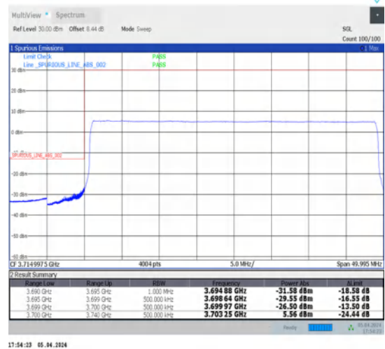
1-N78-3700-3800-N78-3700-380030-40-L-6-CP-QPSK-Outer_Full-106@0-Ant1-1--PASS-see graph
