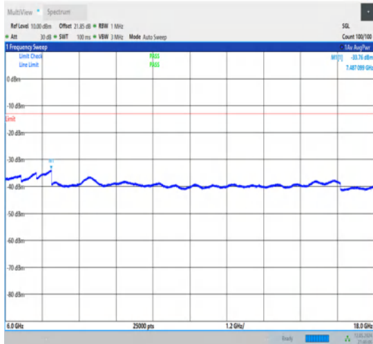
1-N78-3700-3800-30-100-H-1-DFT-QPSK- Edge_1RB_Left-1@0-6000-18000-Ant1-7487.10-- 33.76--13-PASS
