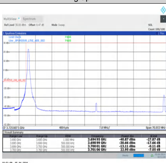
1-N78-3700-3800-N78-3700-380030-60-L-4-CP-QPSK-Edge_1RB_Left-1@0-Ant1-1--PASS-see graph
