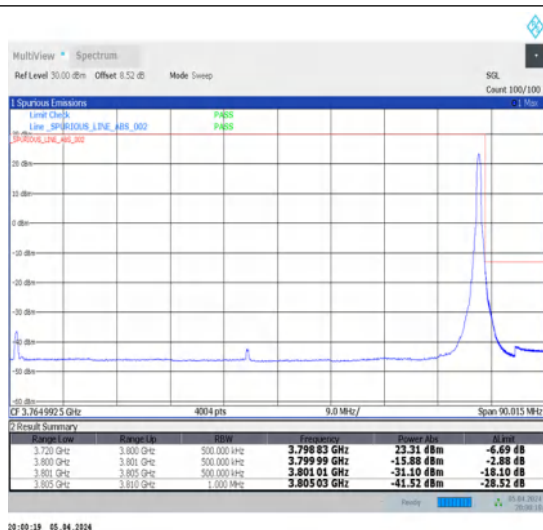
1-N78-3700-3800-N78-3700-380030-80-H-2-DFT-PI2BPSK-Edge_1RB_Right-1@216-Ant1-1--PASS-see graph
