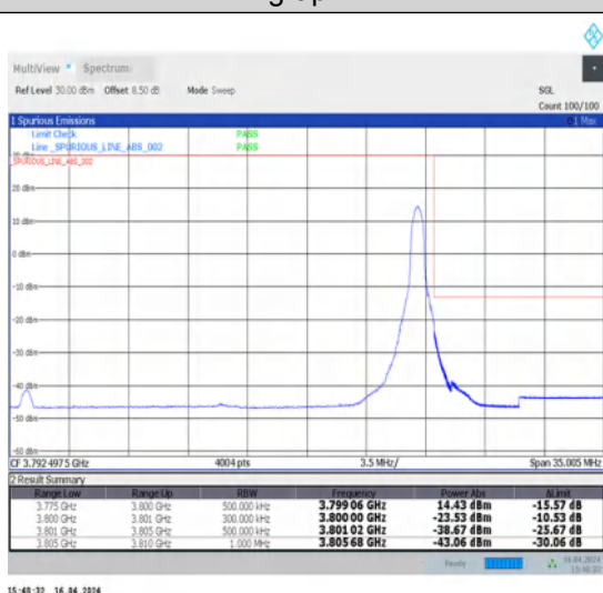
1-N78-3700-3800-N78-3700-380030-25-H-5-CP-QPSK-Edge_1RB_Right-1@64-Ant1-1--PASS-see graph
