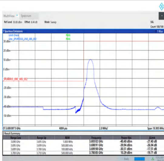
1-N78-3700-3800-30-10-L-4-CP-QPSK-Edge_1RB_Left-1@0-Ant1-1--PASS-see graph
