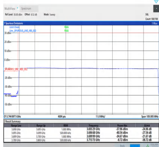
1-N78-3700-3800-30-100-L-6-CP-QPSK-Outer_Full-273@0-Ant1-1--PASS-see graph
