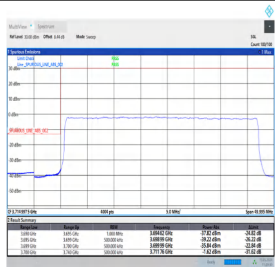
1-N78-3700-3800-30-40-L-3-DFT-PI2BPSK-Outer_Full-100@0-Ant1-1--PASS-see graph
