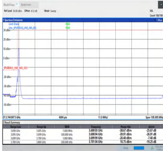
1-N78-3700-3800-30-100-L-1-DFT-PI2BPSK-Edge_1RB_Left-1@0-Ant1-1--PASS-see graph
