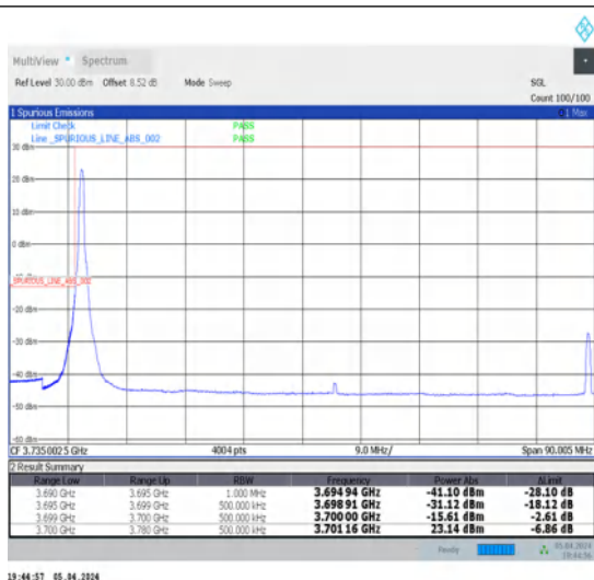
1-N78-3700-3800-N78-3700-380030-80-L-1-DFT-PI2BPSK-Edge_1RB_Left-1@0-Ant1-1--PASS-see graph
