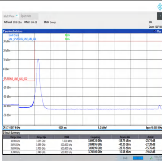
1-N78-3700-3800-30-40-L-1-DFT-PI2BPSK-Edge_1RB_Left-1@0-Ant1-1--PASS-see graph
