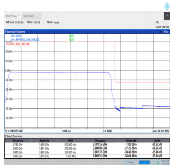
1-N78-3700-3800-30-20-H-6-CP-QPSK-Outer_Full-51@0-Ant1-1--PASS-see graph
