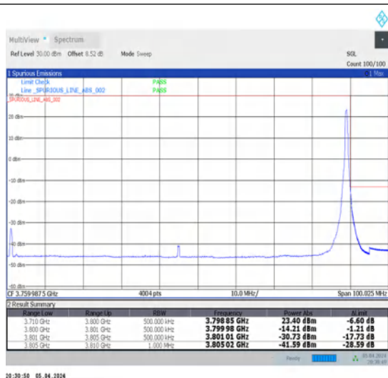
1-N78-3700-3800-N78-3700-380030-90-H-2-DFT-PI2BPSK-Edge_1RB_Right-1@244-Ant1-1--PASS-see graph
