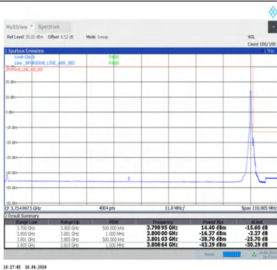
1-N78-3700-3800-N78-3700-380030-100-H-5-CP-QPSK-Edge_1RB_Right-1@272-Ant1-1--PASS-see graph
