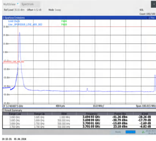
1-N78-3700-3800-N78-3700-380030-90-L-1-DFT-PI2BPSK-Edge_1RB_Left-1@0-Ant1-1--PASS-see graph
