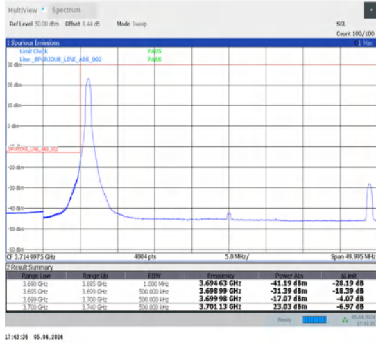
1-N78-3700-3800-N78-3700-380030-40-L-1-DFT-PI2BPSK-Edge_1RB_Left-1@0-Ant1-1--PASS-see graph
