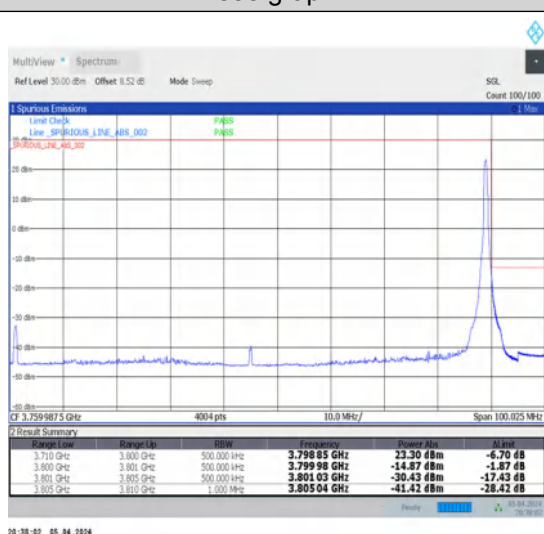
1-N78-3700-3800-N78-3700-380030-90-H-5-CP-QPSK-Edge_1RB_Right-1@244-Ant1-1--PASS-see graph
