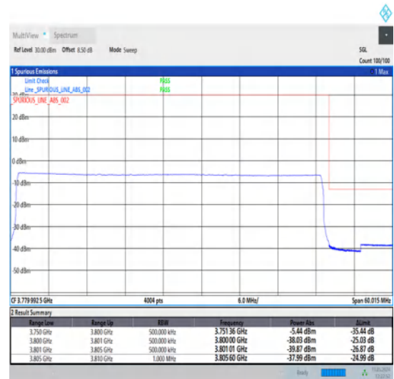
1-N78-3700-3800-30-50-H-6-CP-QPSK-Outer_Full-133@0-Ant1-1--PASS-see graph
