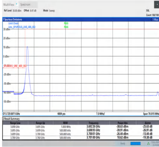
1-N78-3700-3800-30-60-L-1-DFT-PI2BPSK-Edge_1RB_Left-1@0-Ant1-1--PASS-see graph
