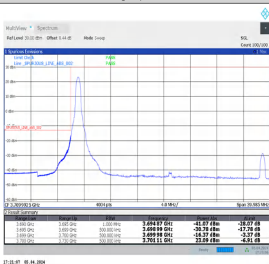
1-N78-3700-3800-N78-3700-380030-30-L-4-CP-QPSK-Edge_1RB_Left-1@0-Ant1-1--PASS-see graph
