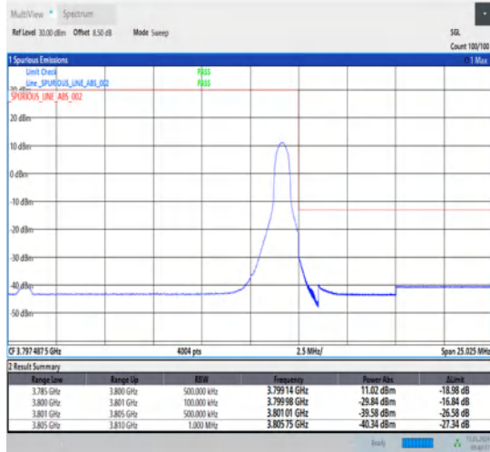
1-N78-3700-3800-30-15-H-2-DFT-PI2BPSK-Edge_1RB_Right-1@37-Ant1-1--PASS-see graph
