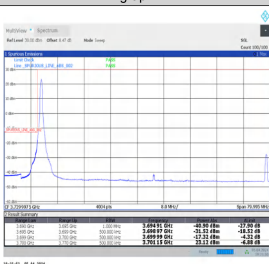
1-N78-3700-3800-N78-3700-380030-70-L-4-CP-QPSK-Edge_1RB_Left-1@0-Ant1-1--PASS-see graph
