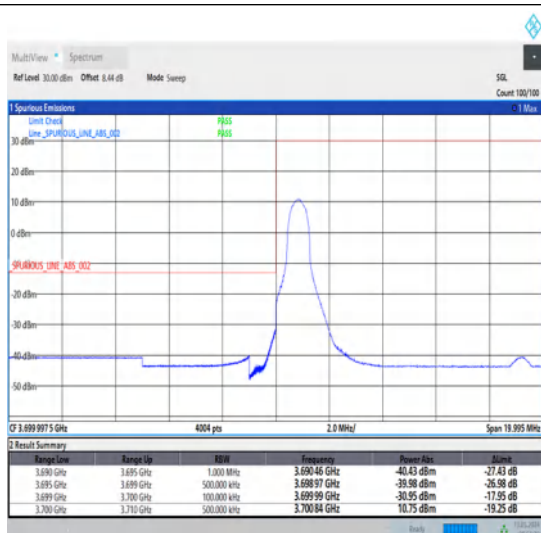
1-N78-3700-3800-30-10-L-1-DFT-PI2BPSK-Edge_1RB_Left-1@0-Ant1-1--PASS-see graph
