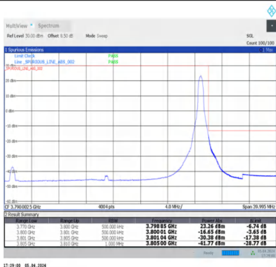
1-N78-3700-3800-N78-3700-380030-30-H-2-DFT-PI2BPSK-Edge_1RB_Right-1@77-Ant1-1--PASS-see graph
