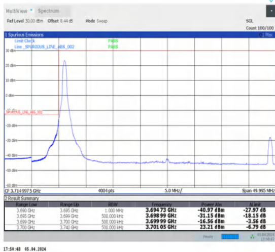
1-N78-3700-3800-N78-3700-380030-40-L-4-CP-QPSK-Edge_1RB_Left-1@0-Ant1-1--PASS-see graph
