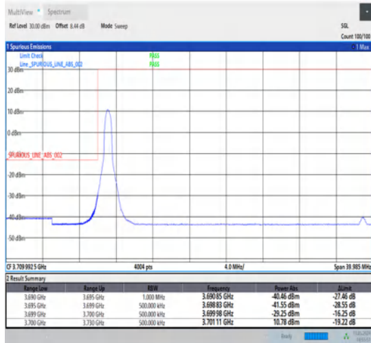
1-N78-3700-3800-30-30-L-1-DFT-PI2BPSK-Edge_1RB_Left-1@0-Ant1-1--PASS-see graph
