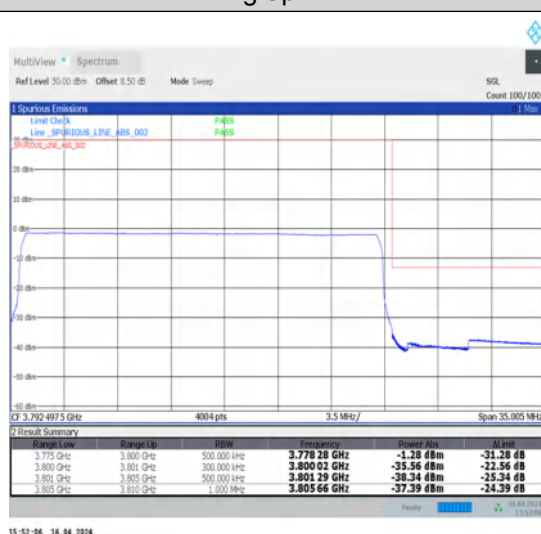
1-N78-3700-3800-N78-3700-380030-25-H-3-DFT-PI2BPSK-Outer_Full-64@0-Ant1-1--PASS-see graph
