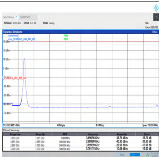
1-N78-3700-3800-30-70-L-1-DFT-PI2BPSK-Edge_1RB_Left-1@0-Ant1-1--PASS-see graph
