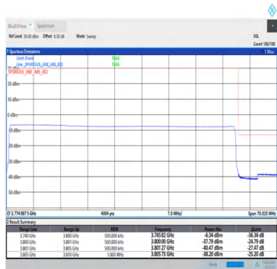
1-N78-3700-3800-30-60-H-6-CP-QPSK-Outer_Full-162@0-Ant1-1--PASS-see graph
