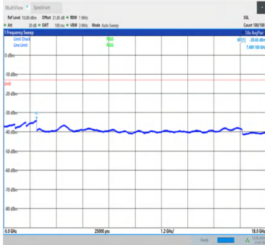
1-N78-3700-3800-30-100-L-1-DFT-QPSK- Edge_1RB_Left-1@0-6000-18000-Ant1-7499.10-- 33.65--13-PASS
