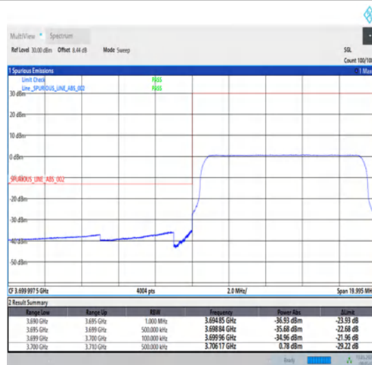
1-N78-3700-3800-30-10-L-6-CP-QPSK-Outer_Full-24@0-Ant1-1--PASS-see graph
