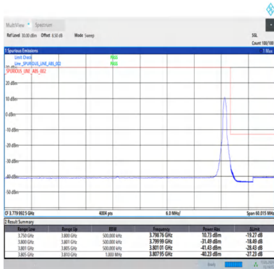
1-N78-3700-3800-30-50-H-5-CP-QPSK-Edge_1RB_Right-1@132-Ant1-1--PASS-see graph
