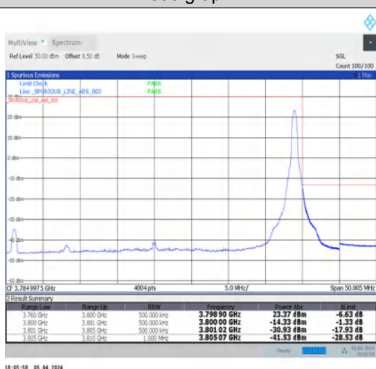
1-N78-3700-3800-N78-3700-380030-40-H-5-CP-QPSK-Edge_1RB_Right-1@105-Ant1-1--PASS-see graph
