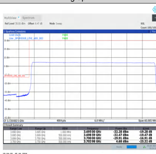
1-N78-3700-3800-N78-3700-380030-50-L-6-CP-QPSK-Outer_Full-133@0-Ant1-1--PASS-see graph
