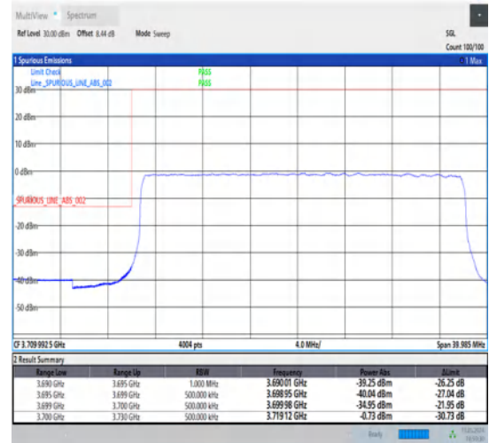
1-N78-3700-3800-30-30-L-3-DFT-PI2BPSK-Outer_Full-75@0-Ant1-1--PASS-see graph
