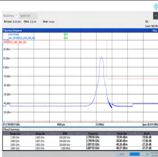
1-N78-3700-3800-30-20-H-2-DFT-PI2BPSK-Edge_1RB_Right-1@50-Ant1-1--PASS-see graph
