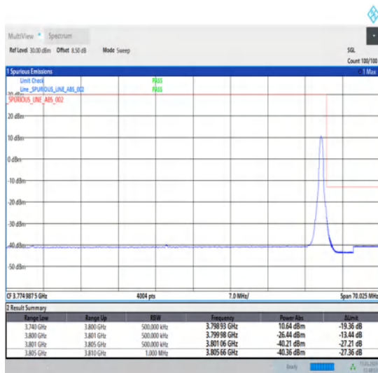
1-N78-3700-3800-30-60-H-5-CP-QPSK-Edge_1RB_Right-1@161-Ant1-1--PASS-see graph
