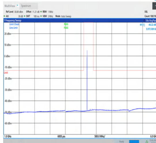
1-N78-3700-3800-30-100-M-1-DFT-QPSK- Edge_1RB_Left-1@0-1000-6000-Ant1-5972.51-- 46.22--13-PASS
