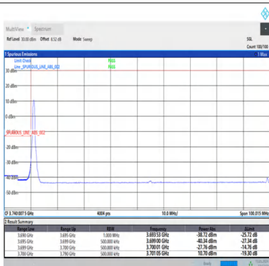
1-N78-3700-3800-30-90-L-1-DFT-PI2BPSK-Edge_1RB_Left-1@0-Ant1-1--PASS-see graph
