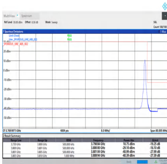
1-N78-3700-3800-30-70-H-5-CP-QPSK-Edge_1RB_Right-1@188-Ant1-1--PASS-see graph
