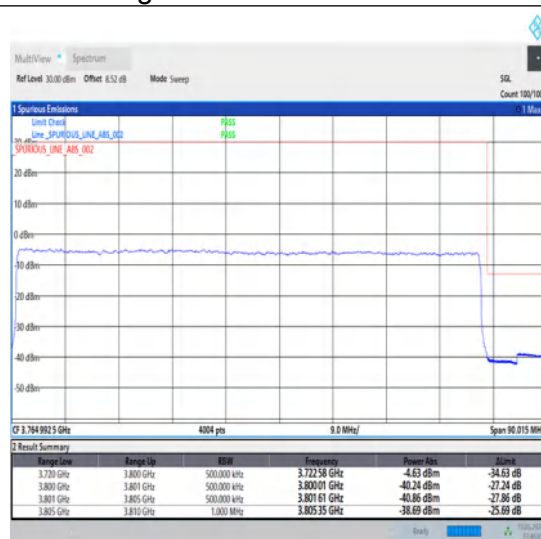
1-N78-3700-3800-30-80-H-3-DFT-PI2BPSK-Outer_Full-216@0-Ant1-1--PASS-see graph
