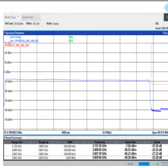
1-N78-3700-3800-30-80-H-6-CP-QPSK-Outer_Full-217@0-Ant1-1--PASS-see graph
