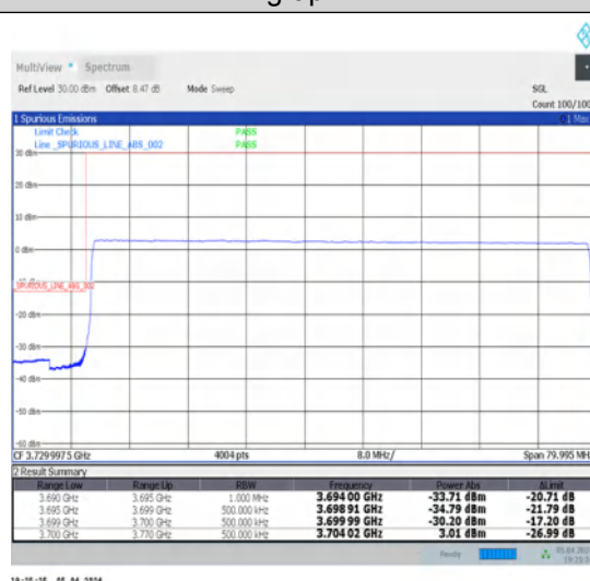
1-N78-3700-3800-N78-3700-380030-70-L-6-CP-QPSK-Outer_Full-189@0-Ant1-1--PASS-see graph
