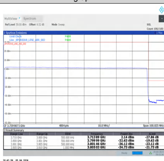
1-N78-3700-3800-N78-3700-380030-90-H-3-DFT-PI2BPSK-Outer_Full-240@0-Ant1-1--PASS-see graph
