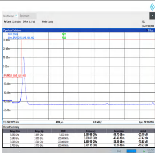
1-N78-3700-3800-30-70-L-4-CP-QPSK-Edge_1RB_Left-1@0-Ant1-1--PASS-see graph
