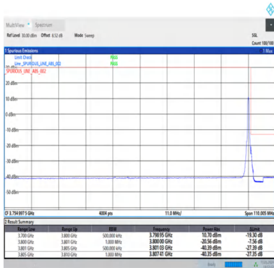
1-N78-3700-3800-30-100-H-5-CP-QPSK-Edge_1RB_Right-1@272-Ant1-1--PASS-see graph
