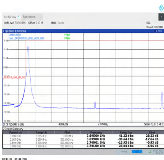
1-N78-3700-3800-N78-3700-380030-60-L-1-DFT-PI2BPSK-Edge_1RB_Left-1@0-Ant1-1--PASS-see graph
