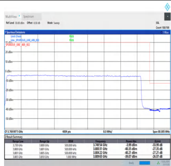
1-N78-3700-3800-30-70-H-3-DFT-PI2BPSK-Outer_Full-180@0-Ant1-1--PASS-see graph
