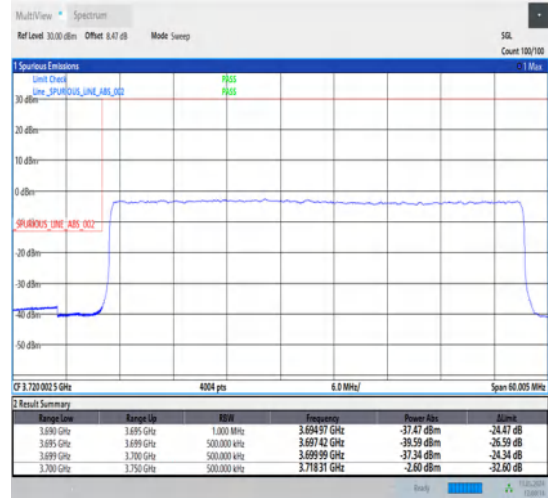
1-N78-3700-3800-30-50-L-3-DFT-PI2BPSK-Outer_Full-128@0-Ant1-1--PASS-see graph
