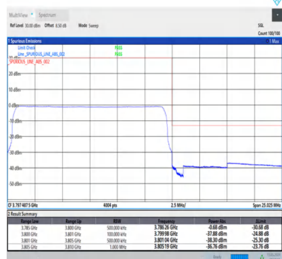
1-N78-3700-3800-30-15-H-6-CP-QPSK-Outer_Full-38@0-Ant1-1--PASS-see graph
