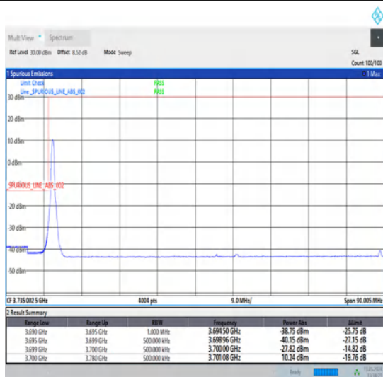
1-N78-3700-3800-30-80-L-4-CP-QPSK-Edge_1RB_Left-1@0-Ant1-1--PASS-see graph
