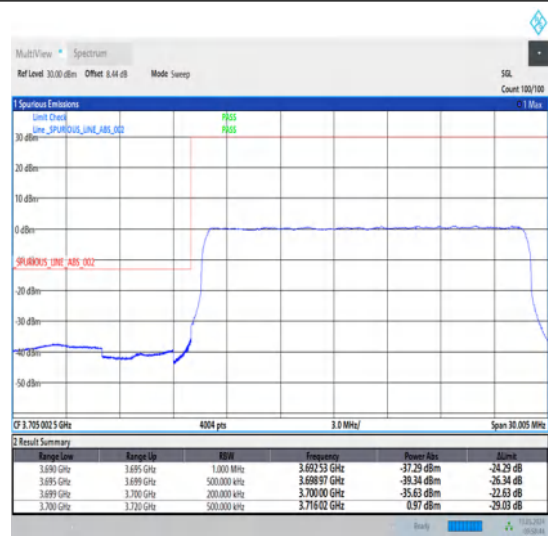
1-N78-3700-3800-30-20-L-3-DFT-PI2BPSK-Outer_Full-50@0-Ant1-1--PASS-see graph
