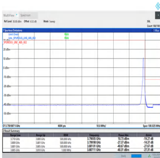
1-N78-3700-3800-30-90-H-5-CP-QPSK-Edge_1RB_Right-1@244-Ant1-1--PASS-see graph
