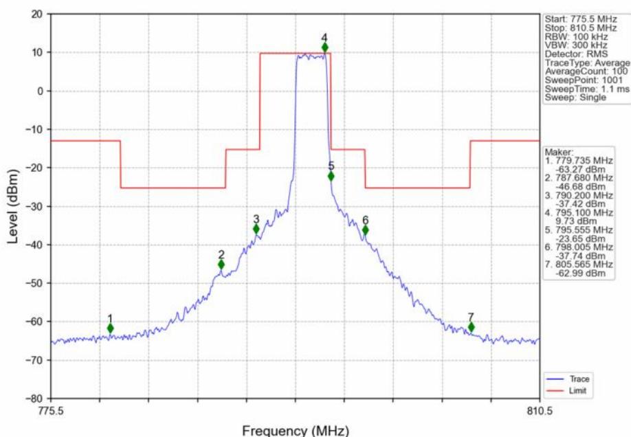
Band14_5MHz_QPSK_MCH_793MHz_RB_25_0_NTNV
