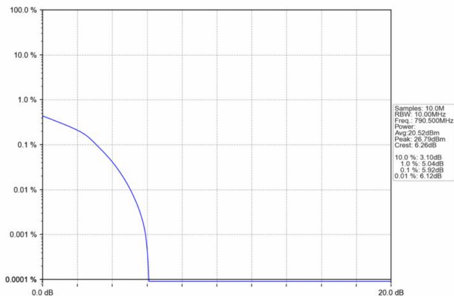
Band14_5MHz_64QAM_LCH_790.5MHz_RB_25_0_NTNV
