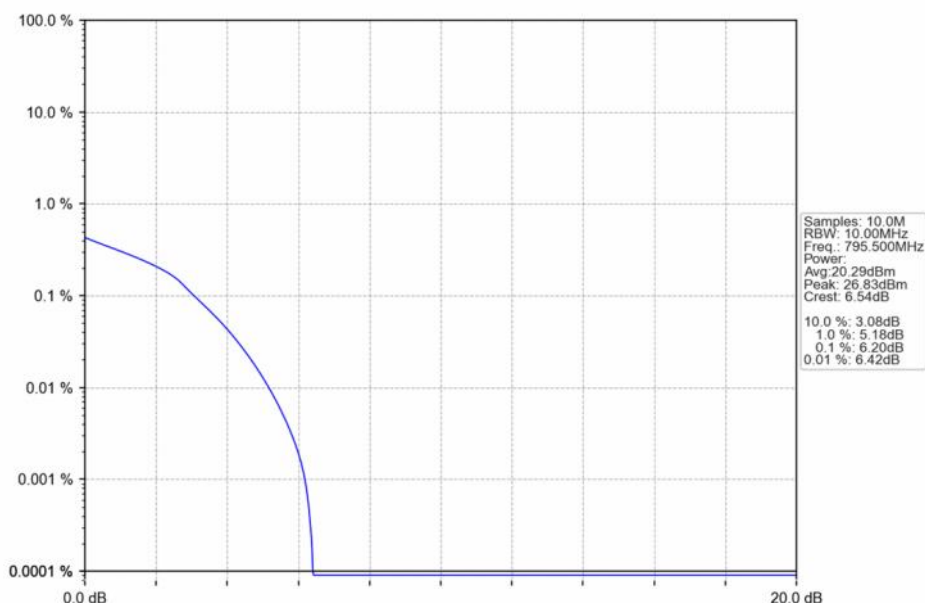
Band14_5MHz_64QAM_HCH_795.5MHz_RB_25_0_NTNV
