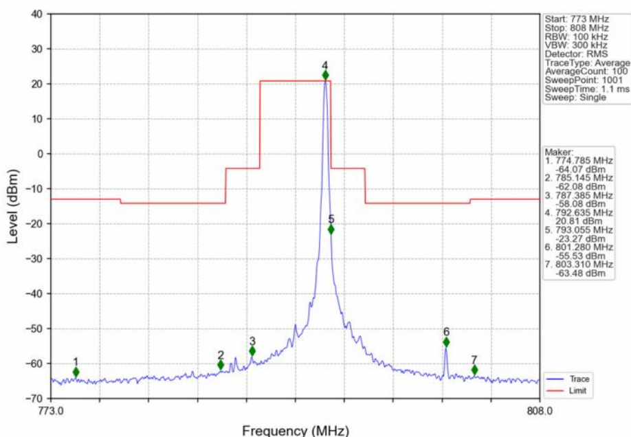
Band14_5MHz_QPSK_LCH_790.5MHz_RB_12_0_NTNV
