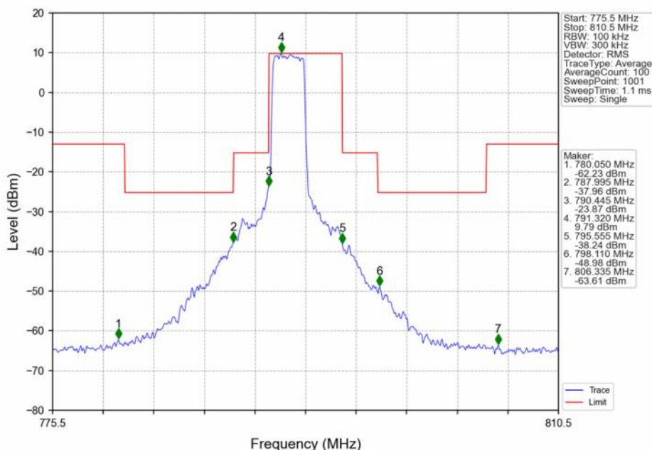
Band14_5MHz_QPSK_MCH_793MHz_RB_12_6_NTNV
