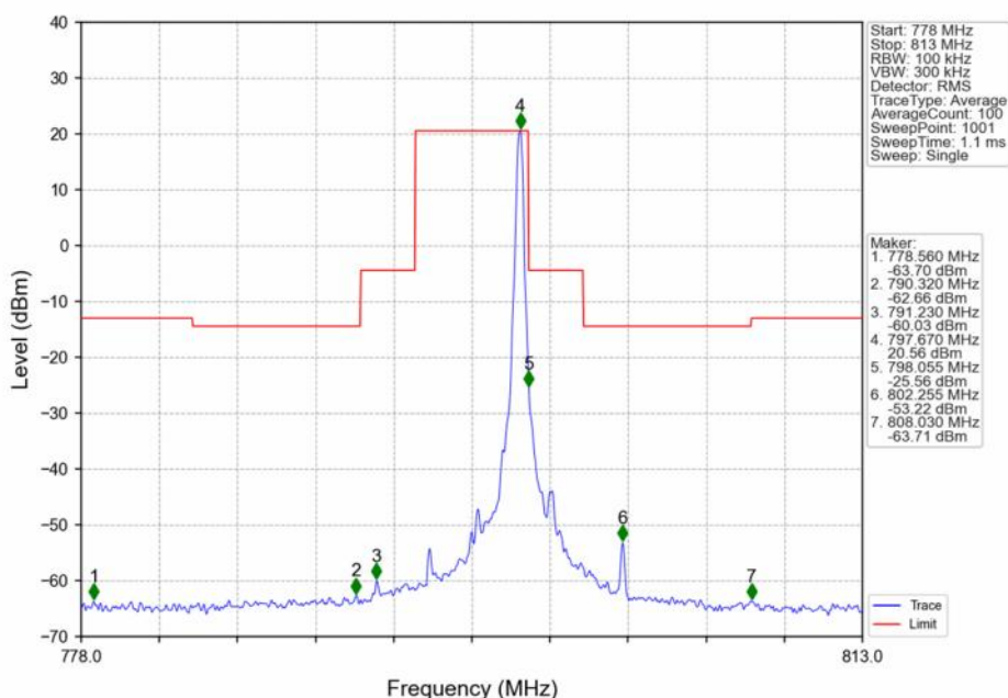
Band14_5MHz_QPSK_HCH_795.5MHz_RB_12_0_NTNV
