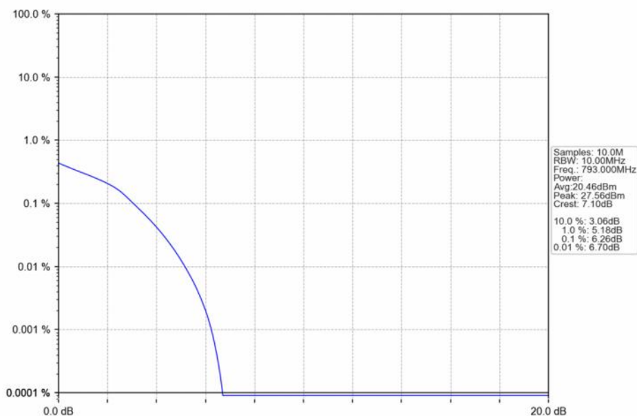
Band14_10MHz_64QAM_MCH_793MHz_RB_50_0_NTNV
