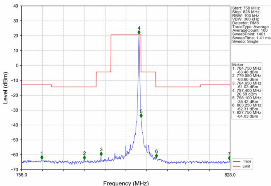
Band14_10MHz_QPSK_MCH_793MHz_RB_25_0_NTNV
