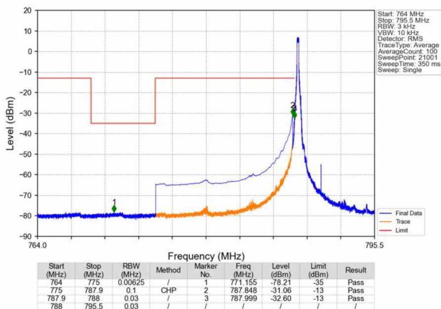
Band14_5MHz_QPSK_LCH_790.5MHz_RB_1_0_NTNV
