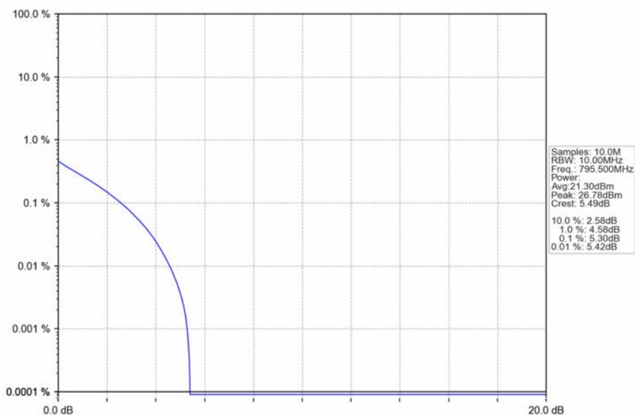
Band14_5MHz_QPSK_HCH_795.5MHz_RB_25_0_NTNV
