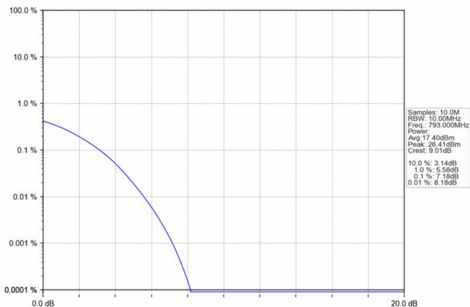
Band14_5MHz_256QAM_MCH_793MHz_RB_25_0_NTNV
