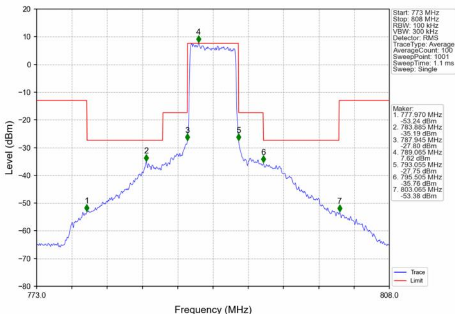
Band14_5MHz_QPSK_MCH_793MHz_RB_1_0_NTNV
