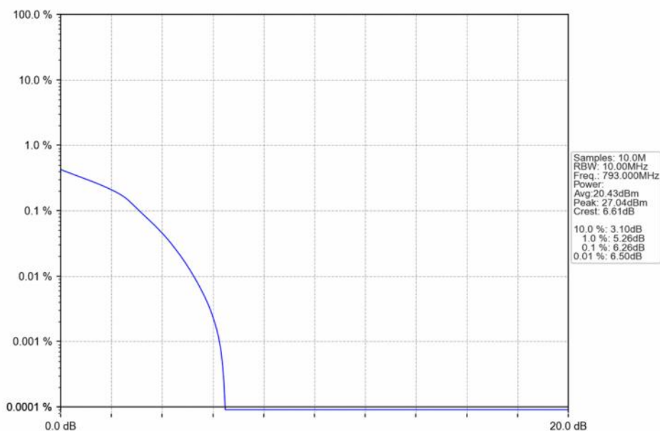
Band14_5MHz_16QAM_MCH_793MHz_RB_25_0_NTNV
