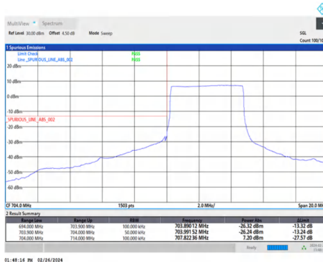
Band17-5MHz-QPSK-23755-25RB#0
