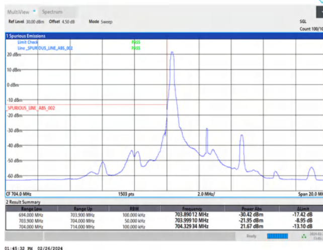
Band17-5MHz-QPSK-23755-25RB#0
