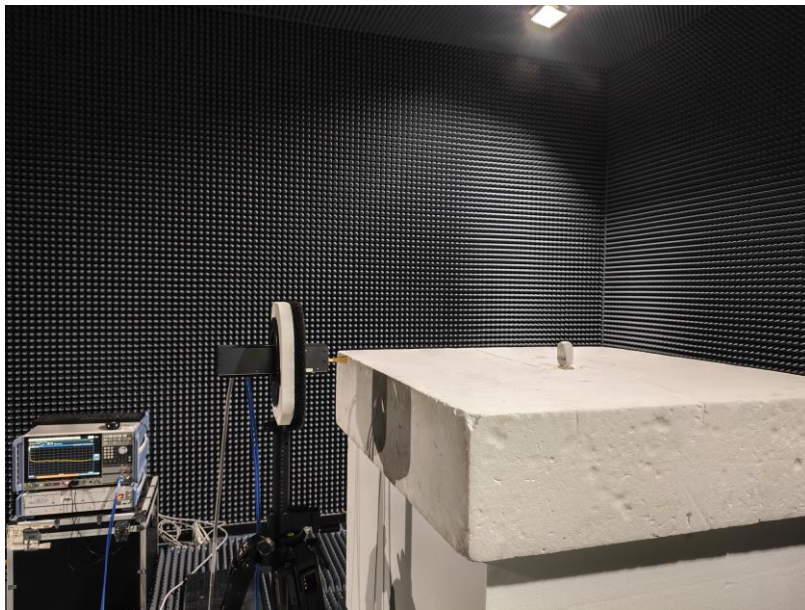
Radiated Emission 90-100 GHz
