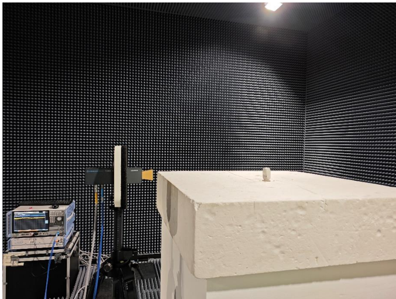
Radiated Emission 42-60GHz
