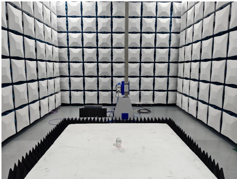
Radiated Emission 18-26.5GHz
