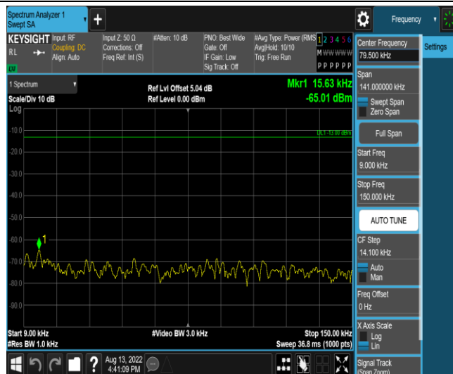
Band13-5MHz-QPSK-23255-1RB#0-Range1:0.009~0.15MHz
