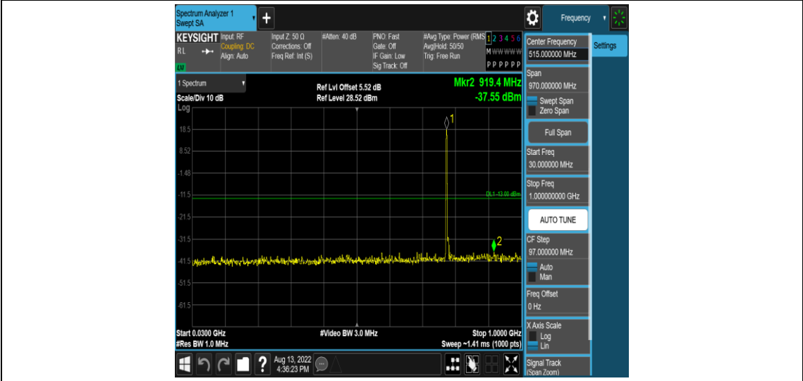
Band13-5MHz-QPSK-23230-1RB#0-Range3:30~1000MHz
