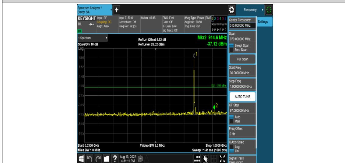
Band13-5MHz-QPSK-23205-1RB#0-Range3:30~1000MHz
