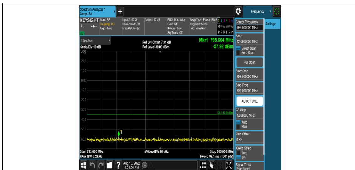
Band13-5MHz-QPSK-23205-1RB#0-Range6:793~805MHz
