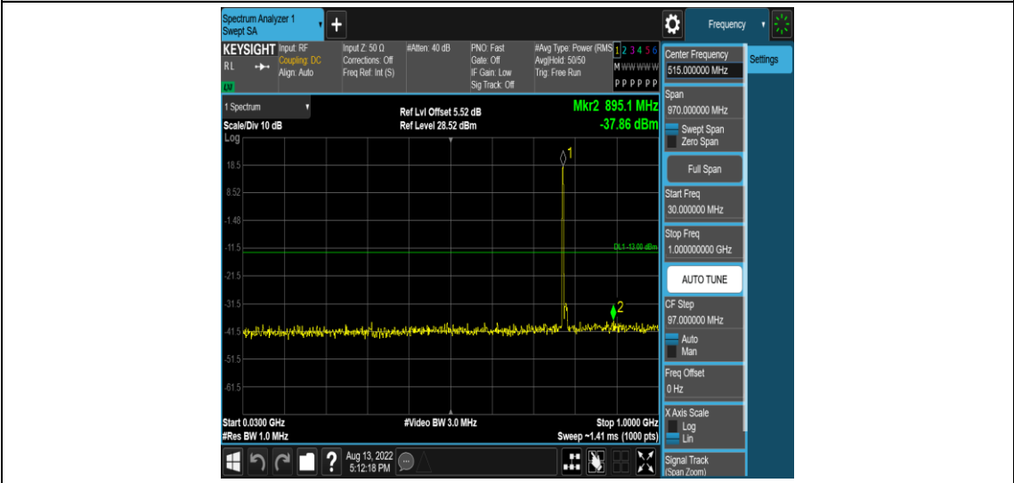
Band13-10MHz-16QAM-23230-1RB#0-Range3:30~1000MHz
