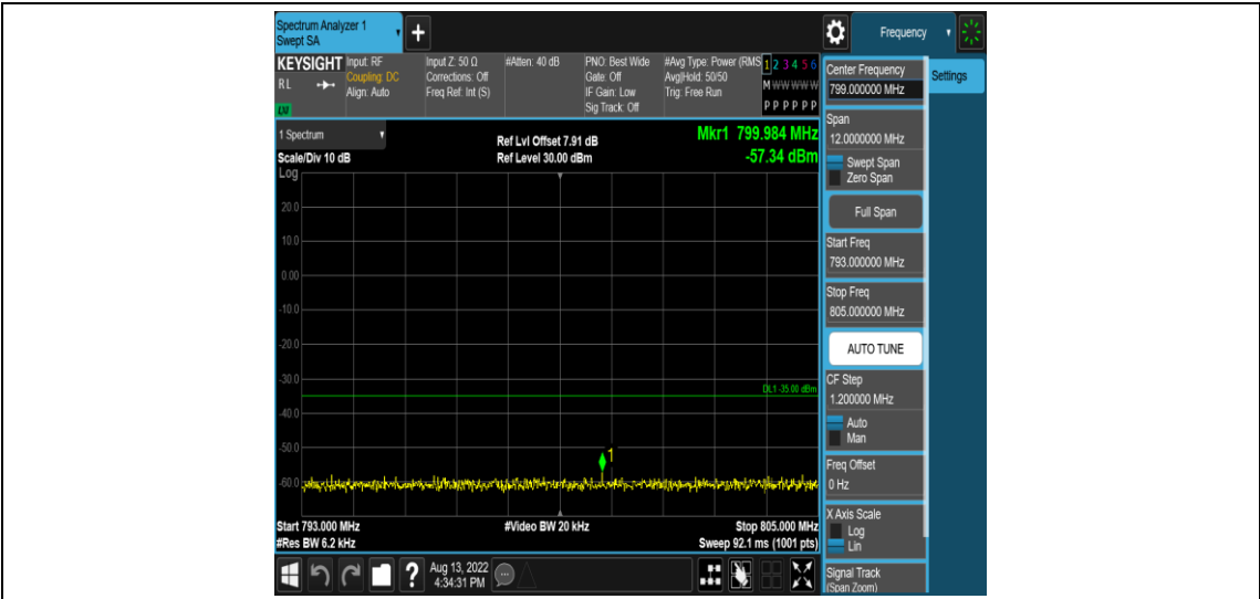
Band13-5MHz-16QAM-23205-1RB#0-Range6:793~805MHz
