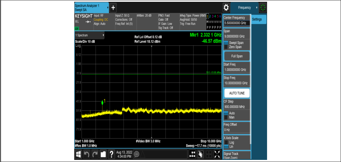
Band13-5MHz-16QAM-23205-1RB#0-Range4:1000~10000MHz
