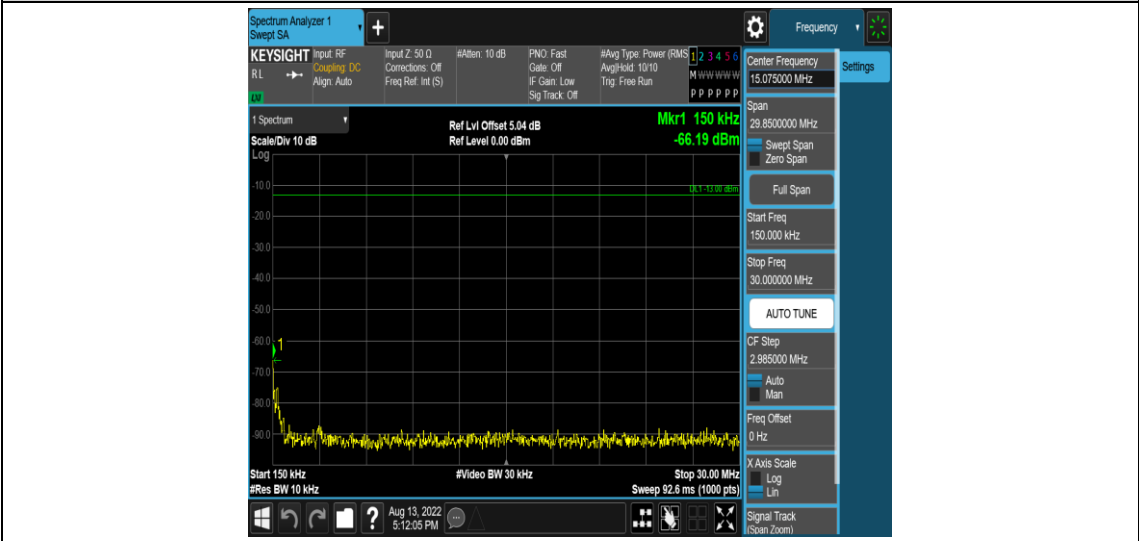
Band13-10MHz-16QAM-23230-1RB#0-Range2:0.15~30MHz
