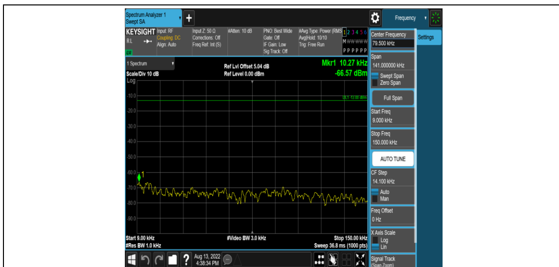
Band13-5MHz-16QAM-23230-1RB#0-Range1:0.009~0.15MHz
