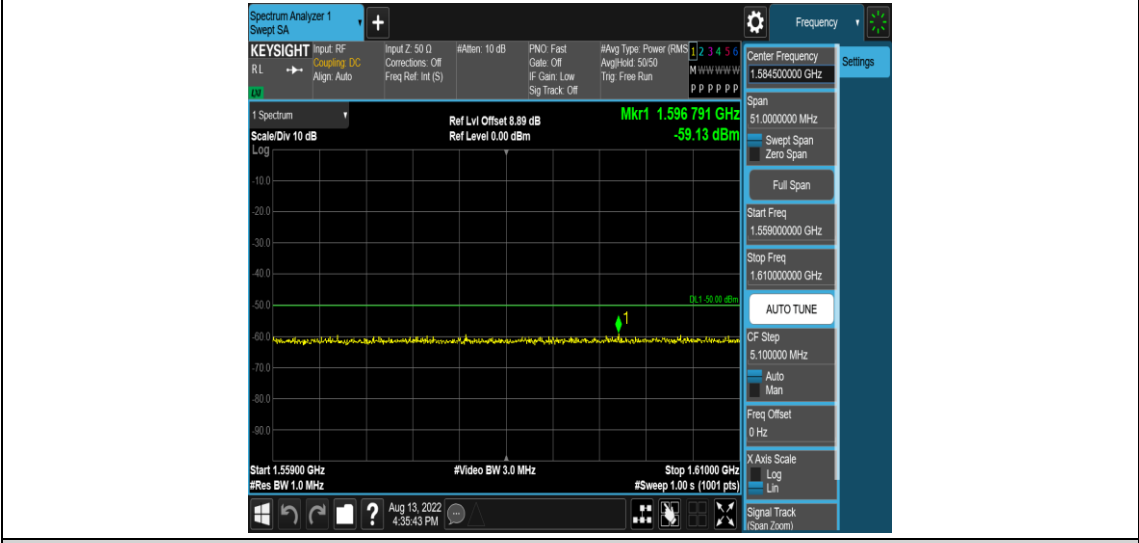
Band13-5MHz-16QAM-23205-1RB#0-Range7:1559~1610MHz
