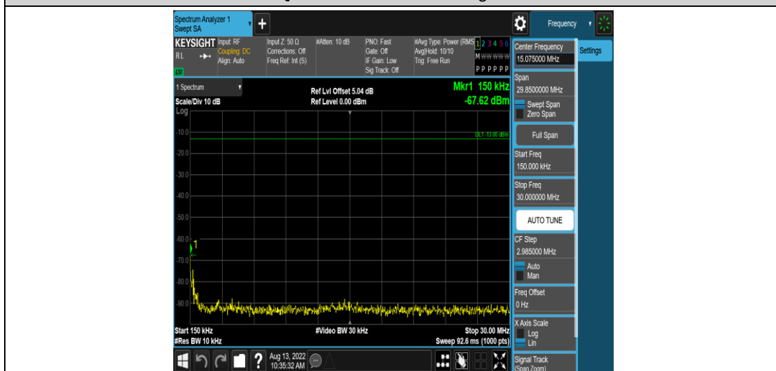
Band2-3MHz-16QAM-18900-1RB#0-Range2:0.15~30MHz
