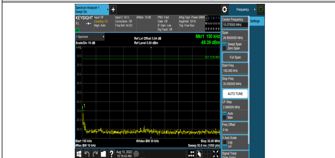
Band2-1.4MHz-16QAM-19193-1RB#0-Range2:0.15~30MHz
