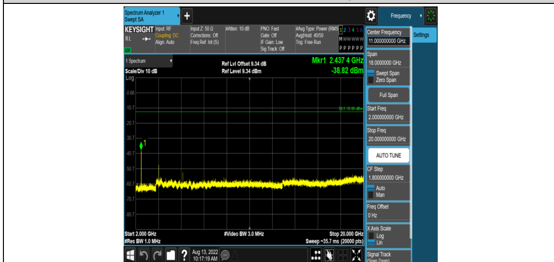
Band2-1.4MHz-16QAM-19193-1RB#0-Range5:2000~20000MHz
