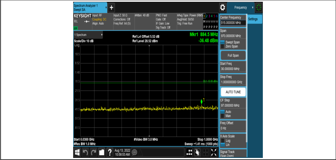
Band2-5MHz-QPSK-19175-1RB#0-Range3:30~1000MHz
