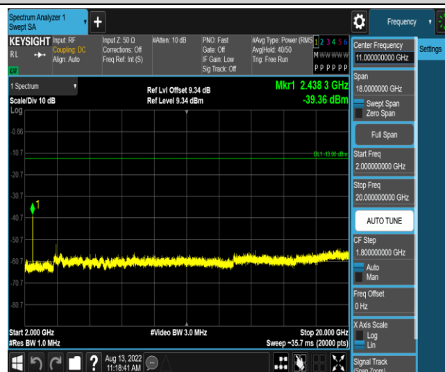
Band2-10MHz-QPSK-18900-1RB#0-Range5:2000~20000MHz
