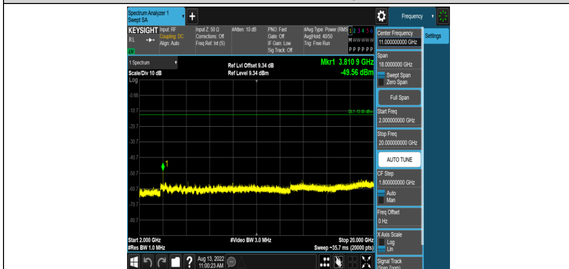
Band2-5MHz-16QAM-19175-1RB#0-Range5:2000~20000MHz
