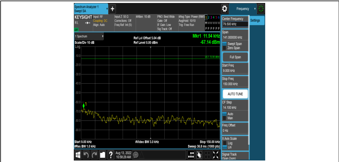
Band2-5MHz-QPSK-19175-1RB#0-Range1:0.009~0.15MHz
