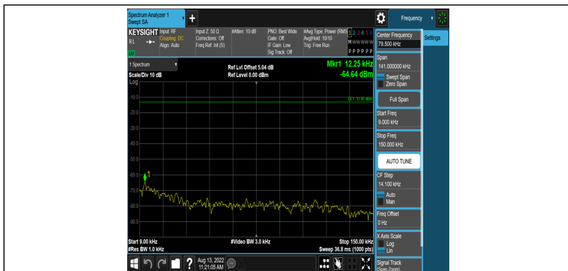
Band2-10MHz-16QAM-19150-1RB#0-Range1:0.009~0.15MHz
