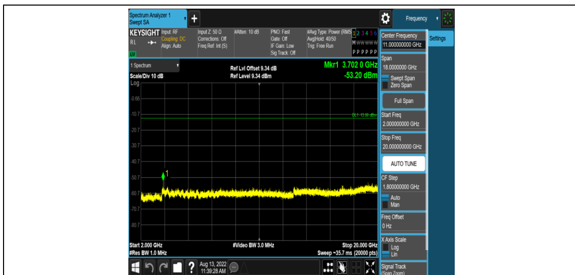
Band2-15MHz-16QAM-18675-1RB#0-Range5:2000~20000MHz
