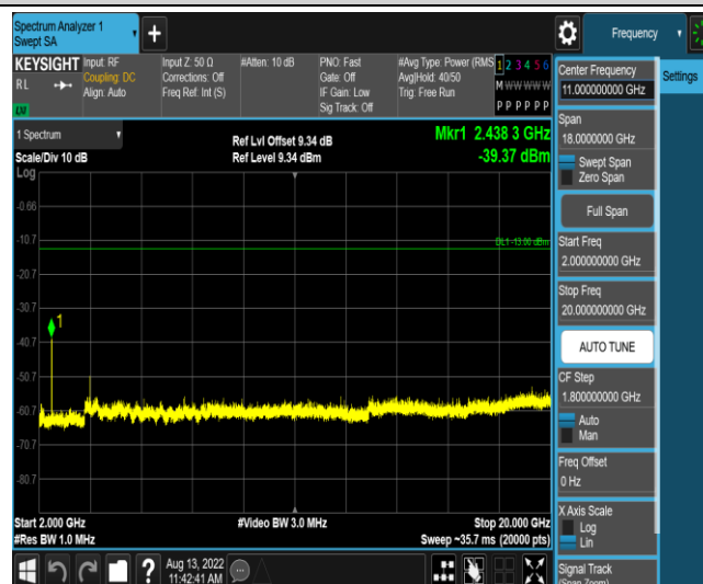
Band2-15MHz-QPSK-19125-1RB#0-Range5:2000~20000MHz
