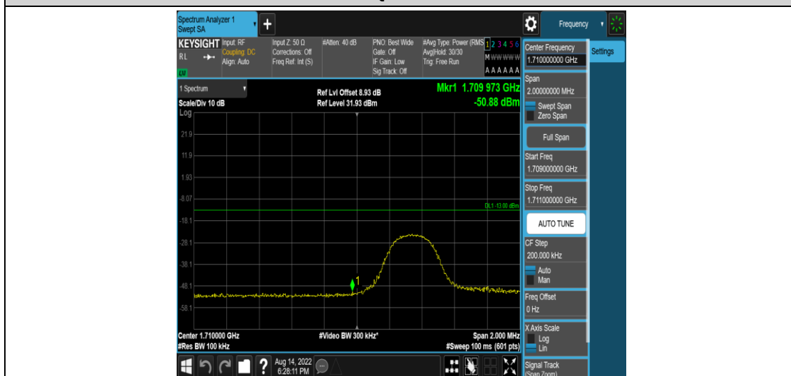
Band4-5MHz-QPSK-19975-1RB#24
