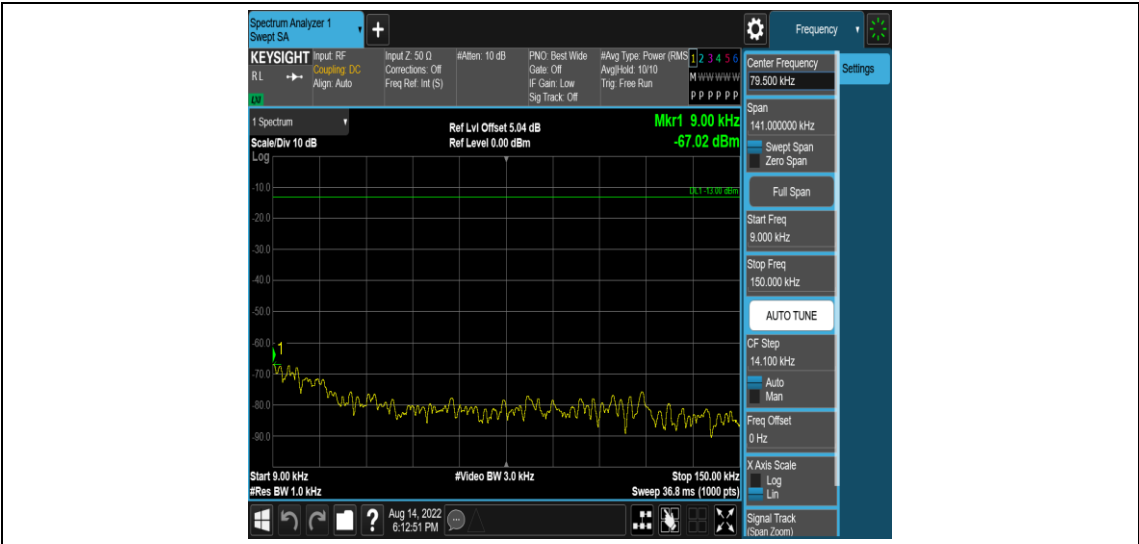
Band4-3MHz-QPSK-20385-1RB#0-Range1:0.009~0.15MHz
