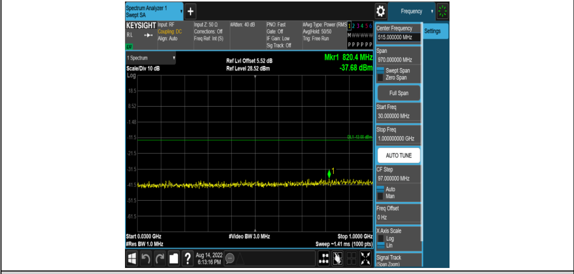
Band4-3MHz-QPSK-20385-1RB#0-Range3:30~1000MHz
