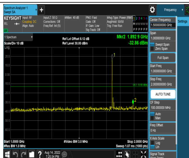
Band4-15MHz-QPSK-20325-1RB#0-Range4:1000~2000MHz
