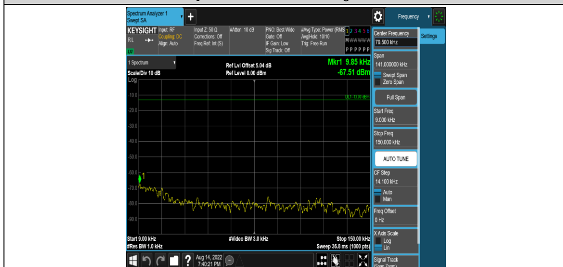
Band4-20MHz-QPSK-20175-1RB#0-Range1:0.009~0.15MHz
