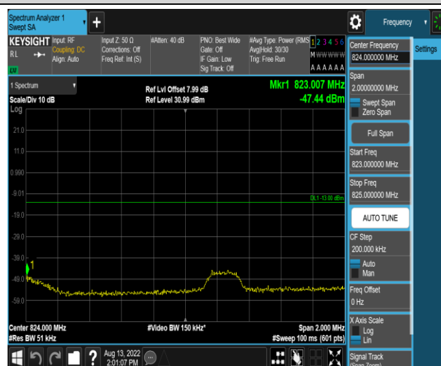
Band5-3MHz-16QAM-20415-1RB#14
