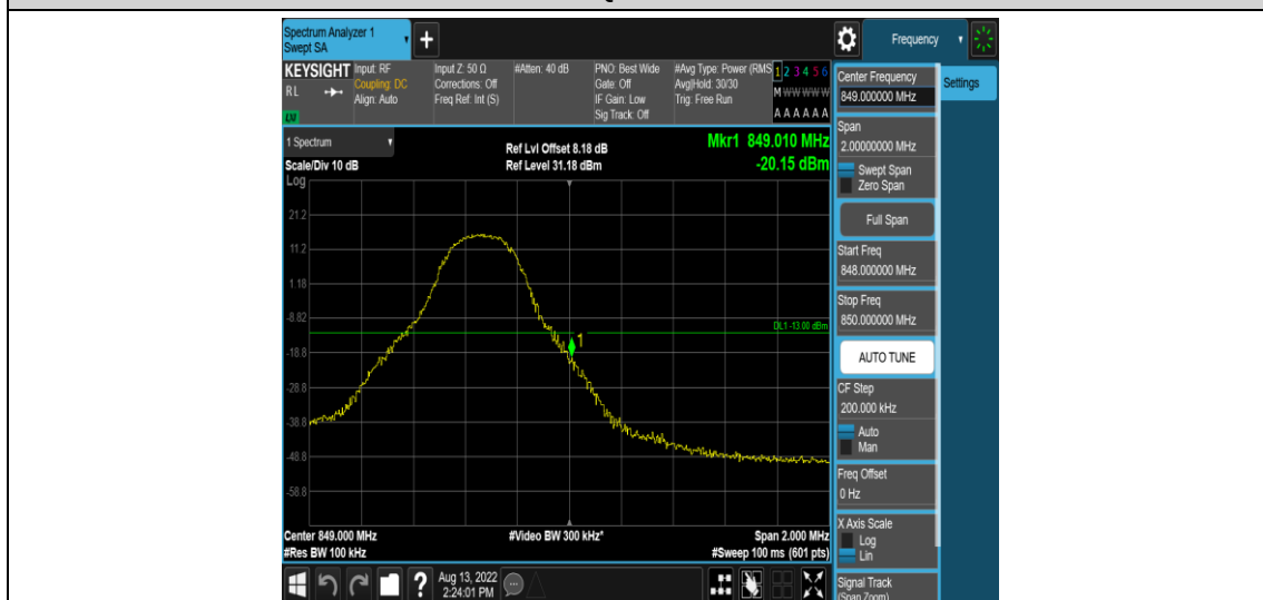
Band5-5MHz-QPSK-20625-1RB#24
