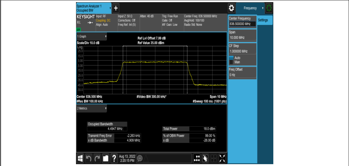
Band5-5MHz-QPSK-20525-25RB#0
