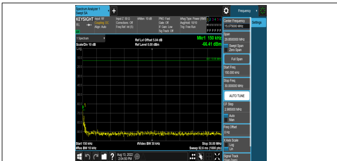
Band5-3MHz-16QAM-20415-1RB#0-Range2:0.15~30MHz
