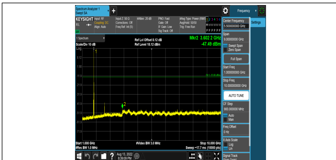
Band66-10MHz-16QAM-132322-1RB#0-Range4:1000~10000MHz
