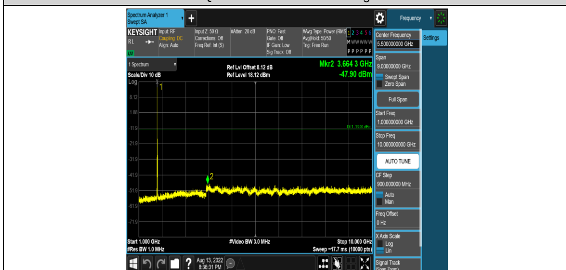
Band66-10MHz-QPSK-132022-1RB#0-Range4:1000~10000MHz
