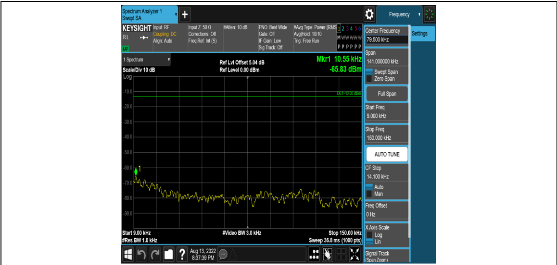
Band66-10MHz-QPSK-132322-1RB#0-Range1:0.009~0.15MHz
