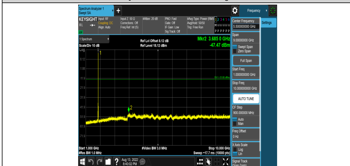
Band66-10MHz-QPSK-132622-1RB#0-Range4:1000~10000MHz
