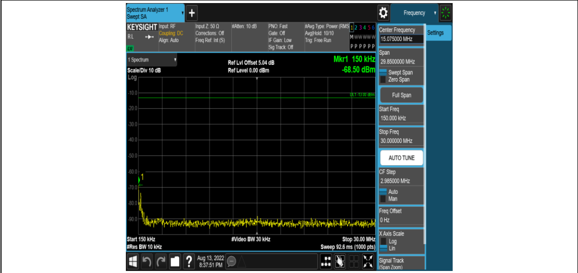
Band66-10MHz-QPSK-132322-1RB#0-Range2:0.15~30MHz
