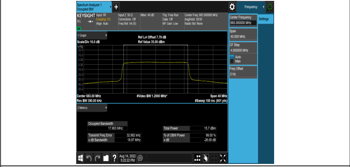
Band71-20MHz-16QAM-133322-100RB#0
