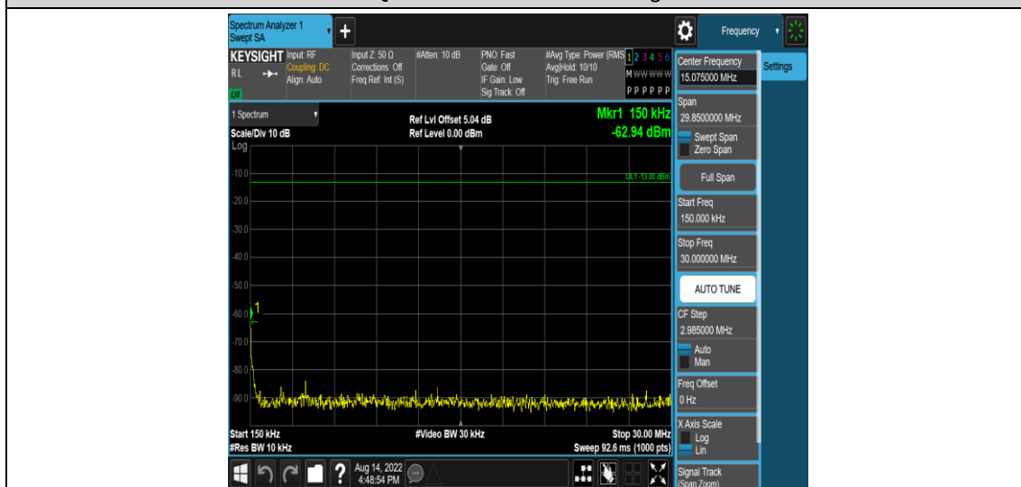
Band71-10MHz-16QAM-133422-1RB#0-Range2:0.15~30MHz
