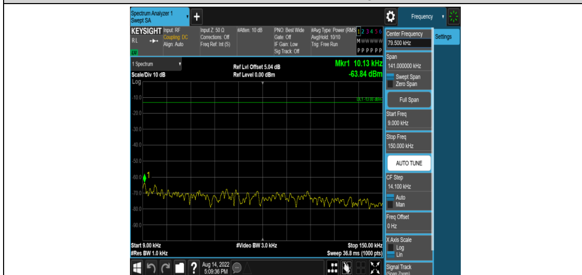
Band71-15MHz-16QAM-133397-1RB#0-Range1:0.009~0.15MHz
