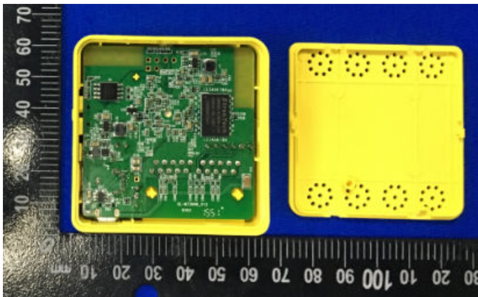
EUT - Open View
