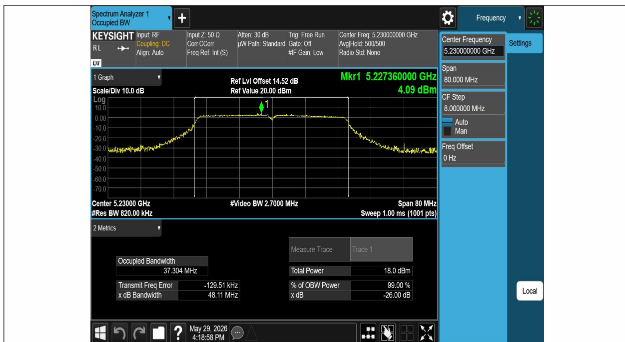
11N40SISO-Ant1-5230
