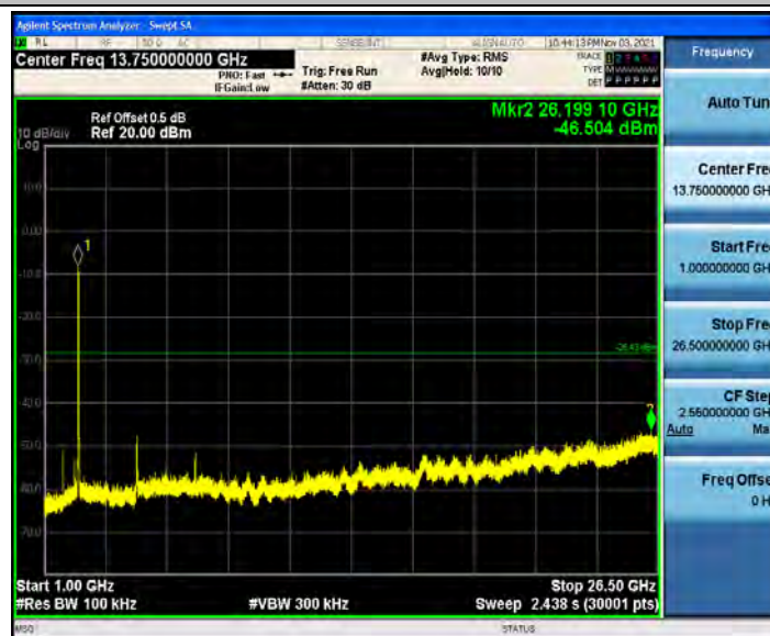
802.11n(HT40)_Ant2_2422_0~Reference
