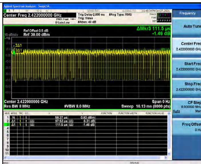
802.11n(HT40) Ant2 2422
