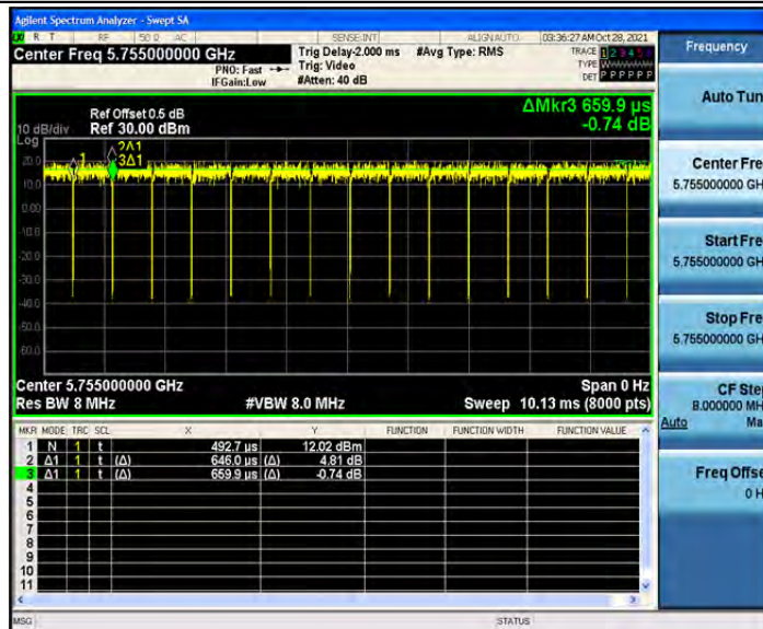
802.11n(HT40)_Ant2_5755
