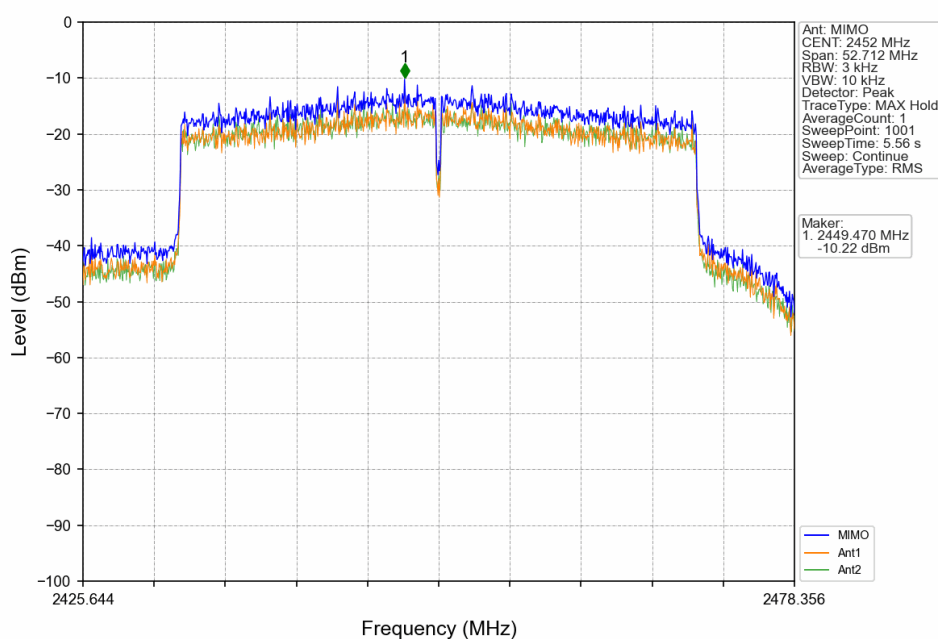
802.11ax(HEW40)_HCH_2452MHz_RU484_Left_MIMO_NTNV
