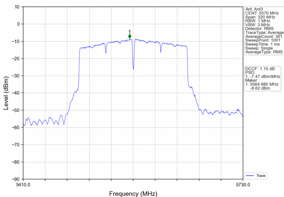
802.11ac(VHT160)_MCH_5570MHz_Ant3_NTNV
