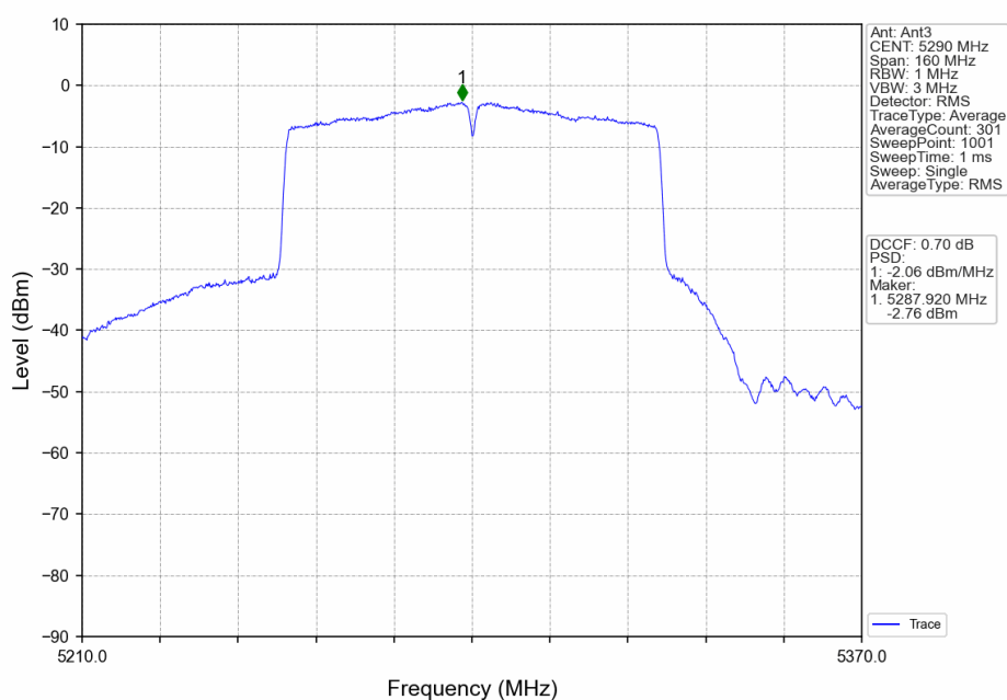
802.11ac(VHT80)_MCH_5290MHz_Ant3_NTNV
