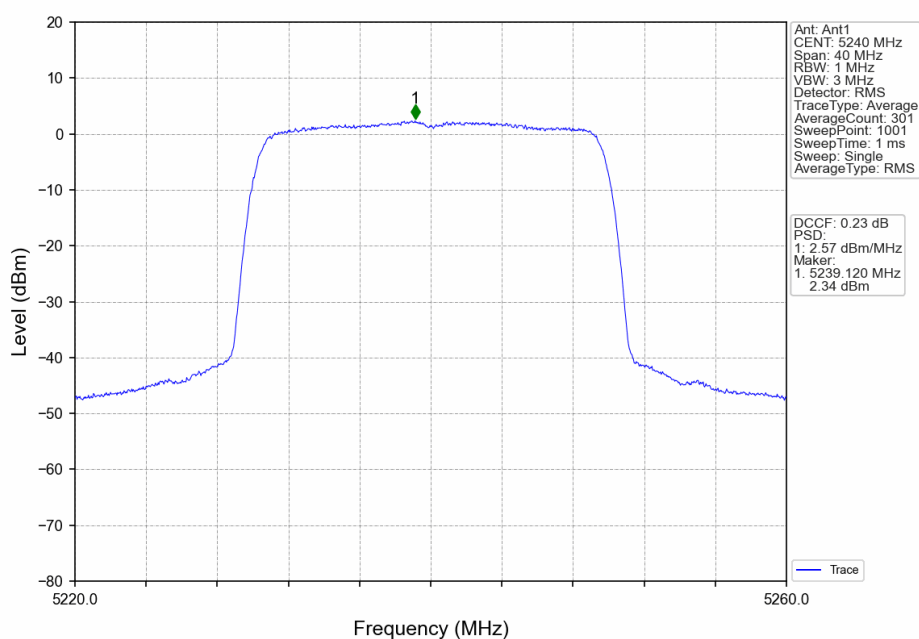
802.11ax(HEW20)_HCH_5240MHz_RU242_Left_Ant1_NTNV
