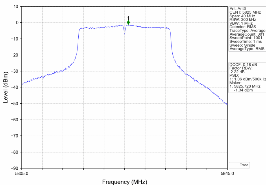
802.11n(HT20)_HCH_5825MHz_Ant3_NTNV
