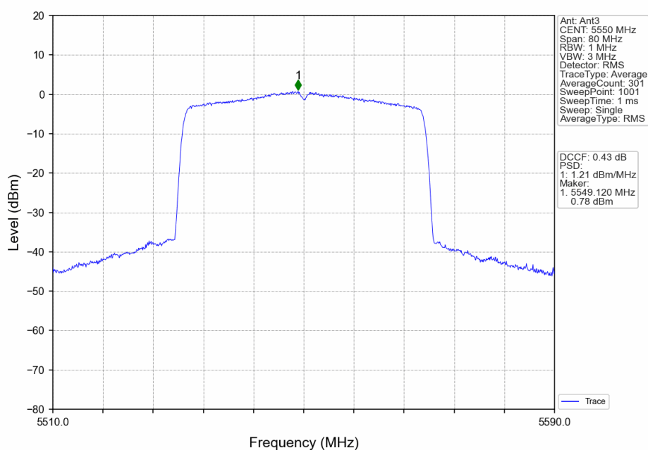
802.11ax(HEW40)_MCH_5550MHz_RU484_Left_Ant3_NTNV
