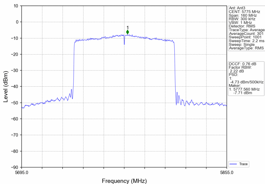
802.11ax(HEW80)_MCH_5775MHz_RU996_Left_Ant3_NTNV
