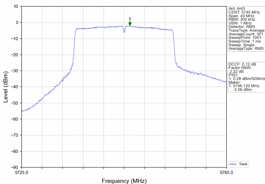
802.11ax(HEW20)_LCH_5745MHz_RU242_Left_Ant3_NTNV
