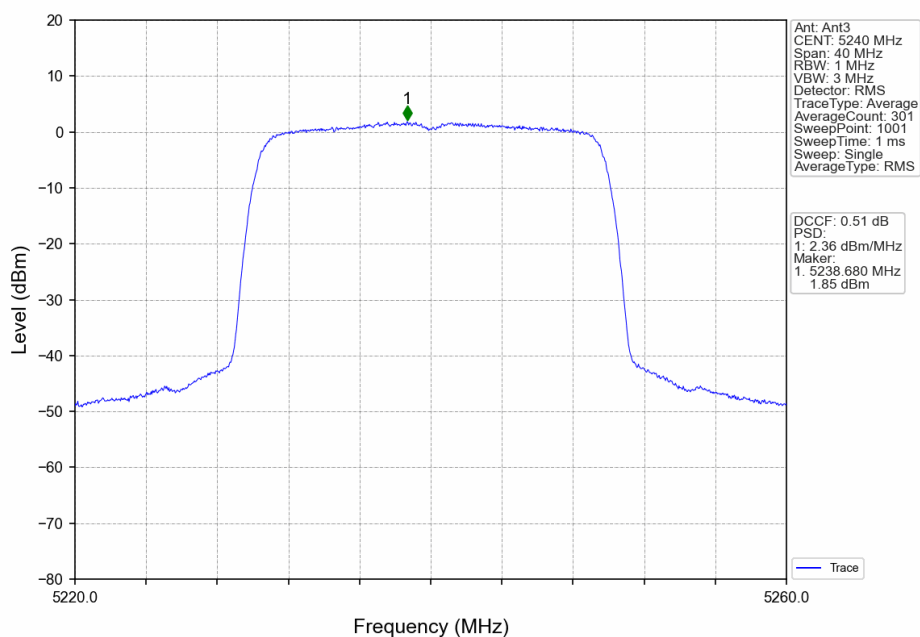
802.11ax(HEW20)_HCH_5240MHz_RU242_Left_Ant3_NTNV
