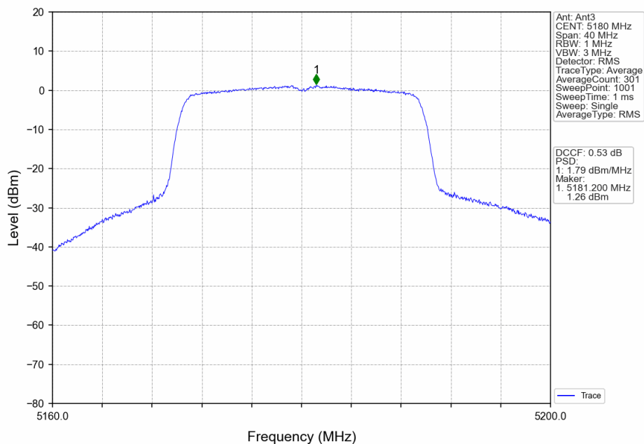
802.11ax(HEW20)_LCH_5180MHz_RU242_Left_Ant3_NTNV
