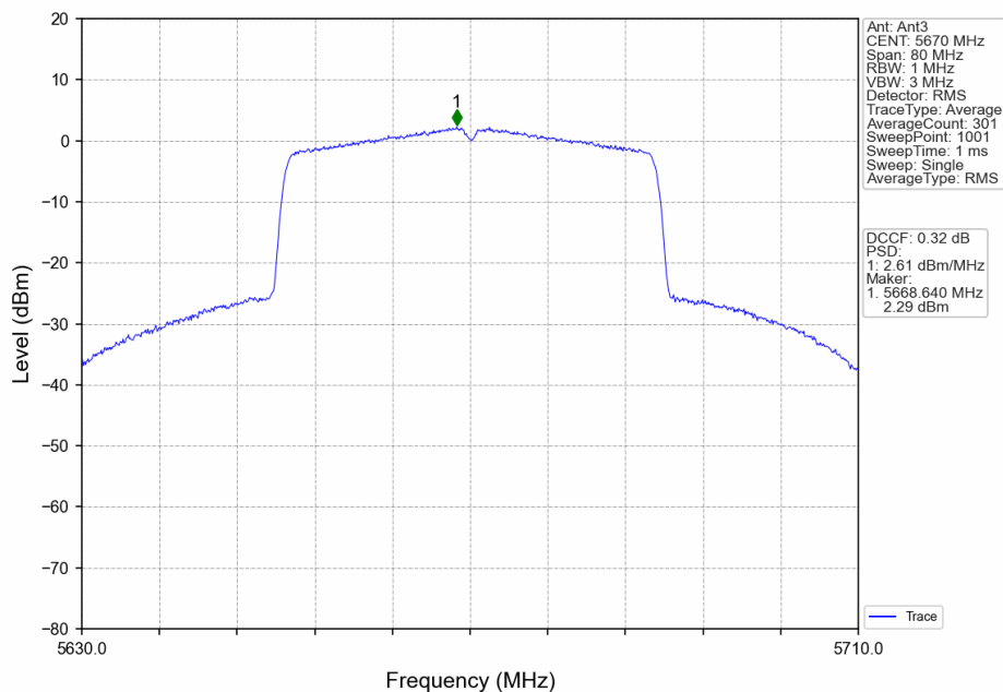
802.11ax(HEW40)_HCH_5670MHz_RU484_Left_Ant3_NTNV
