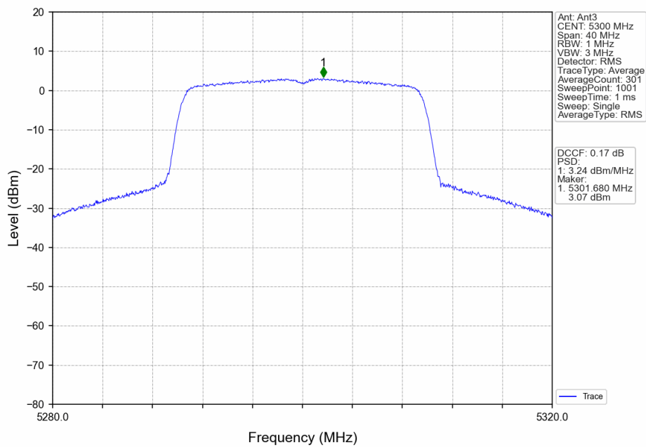
802.11ax(HEW20)_MCH_5300MHz_RU242_Left_Ant3_NTNV
